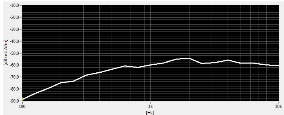
Figure 7-3 Worst-case ABM2 Plot for UMTS
