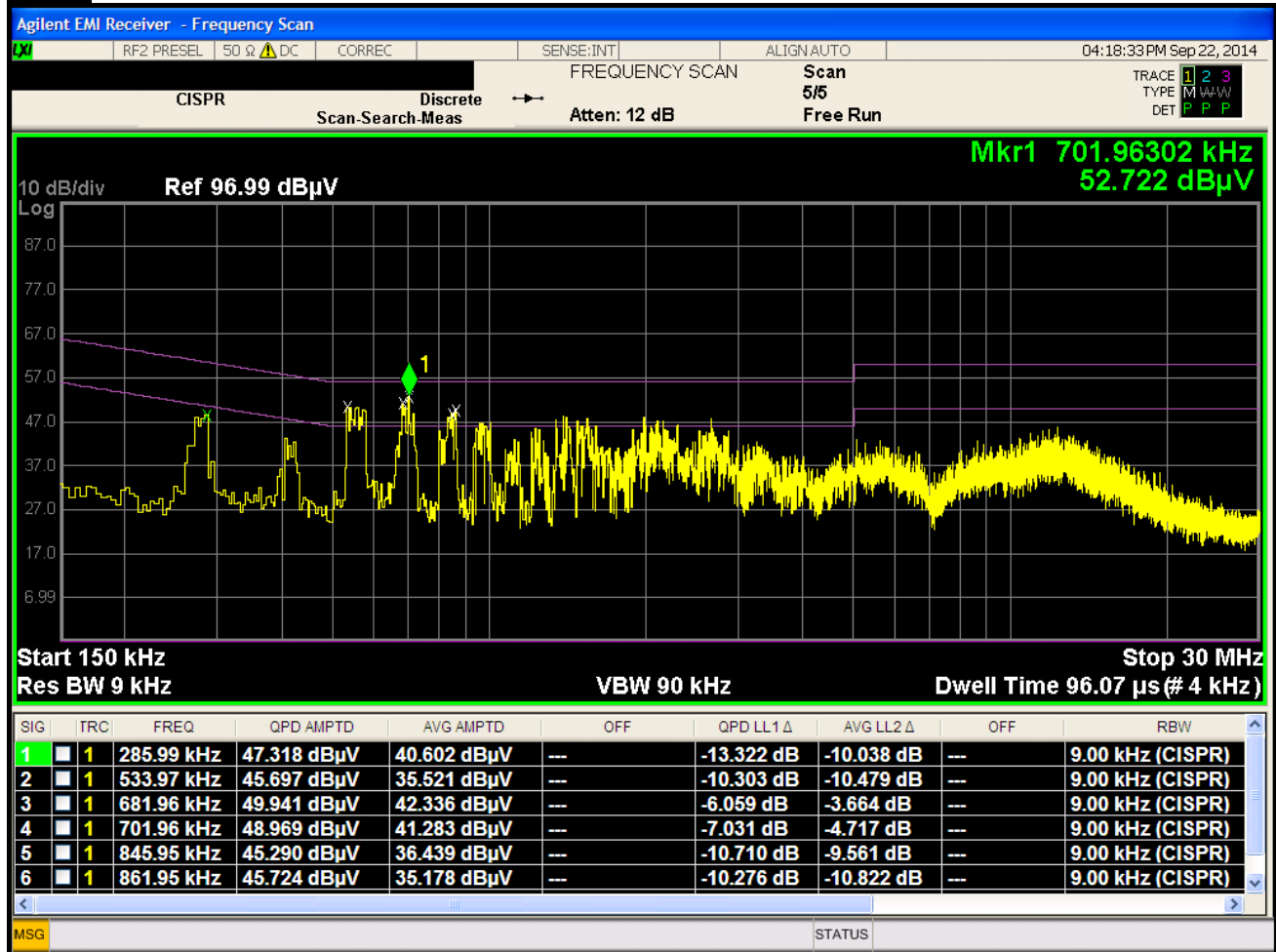
Plot 6-143. Line Conducted Plot with 802.11a (L1)
