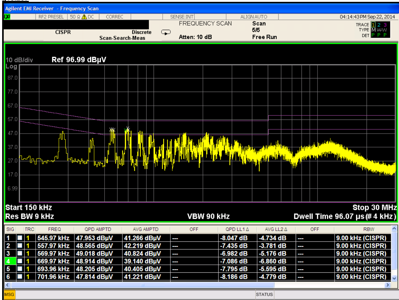
Plot 6-144. Line Conducted Plot with 802.11a (N)
