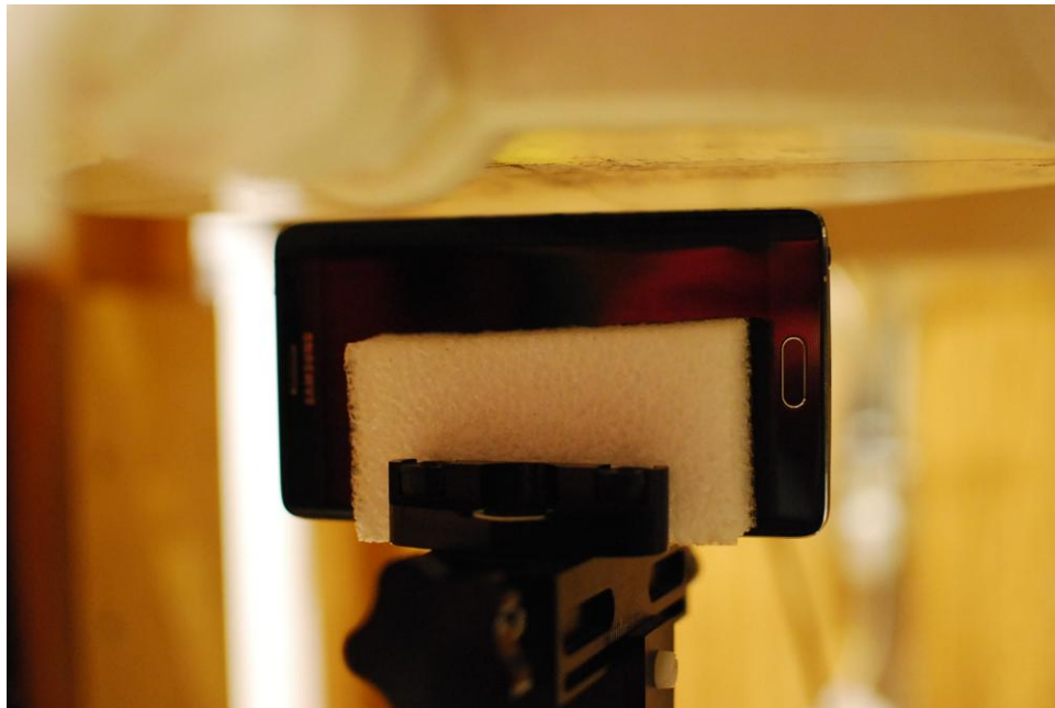
SAR Test Setup Photo 14 – Right Edge at 1.0 cm
