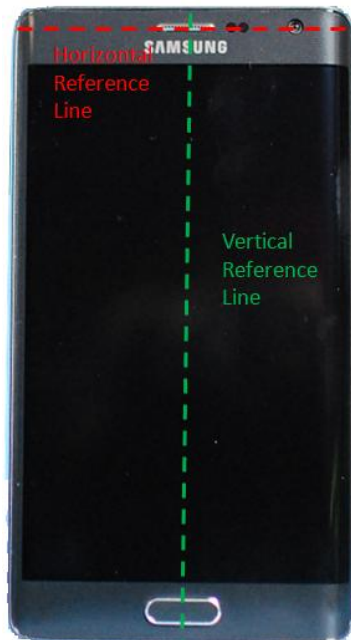
SAR Test Setup Photo 17 – Horizontal and Vertical Reference Lines
