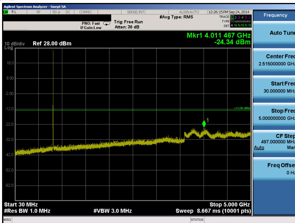
Plot 6-35. Conducted Spurious Plot (Band 5 – 5.0MHz QPSK – RB Size 1, RB Offset 0 – Mid Channel)
