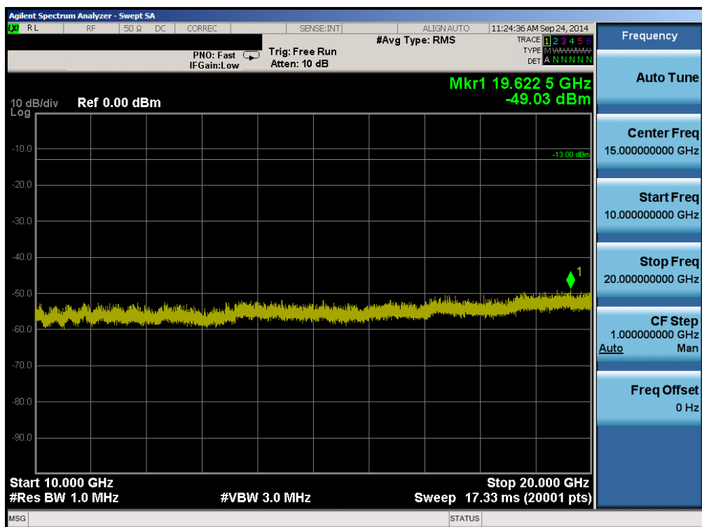
Plot 6-42. Conducted Spurious Plot (Band 4 – 10.0MHz QPSK – RB Size 1, RB Offset 0 – Mid Channel)
