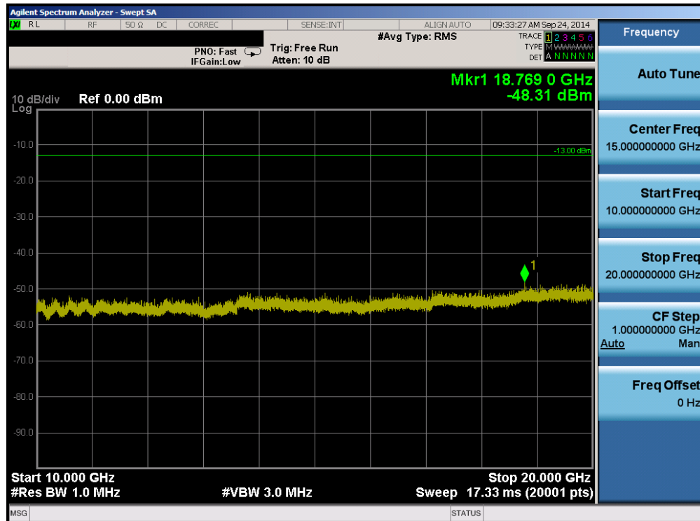
Plot 6-48. Conducted Spurious Plot (Band 2 – 5.0MHz QPSK – RB Size 1, RB Offset 0 – Mid Channel)
