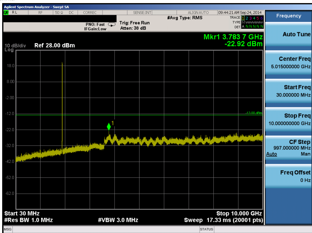
Plot 6-49. Conducted Spurious Plot (Band 2 – 5.0MHz QPSK – RB Size 1, RB Offset 0 – High Channel)
