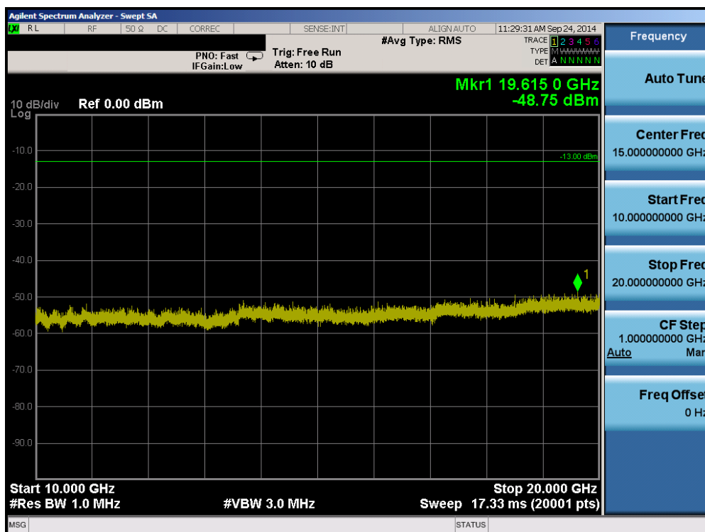
Plot 6-40. Conducted Spurious Plot (Band 4 – 10.0MHz QPSK – RB Size 1, RB Offset 0 – Low Channel)
