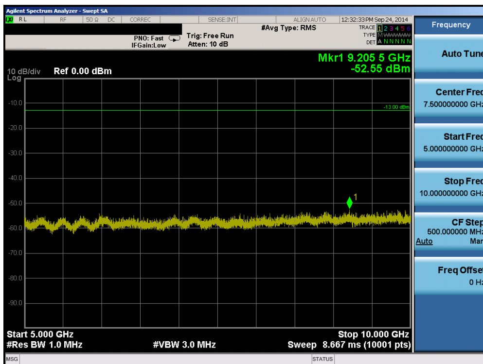
Plot 6-38. Conducted Spurious Plot (Band 5 – 5.0MHz QPSK – RB Size 1, RB Offset 0 – High Channel)
