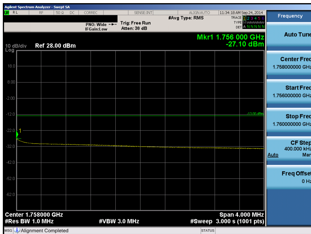
Plot 6-74. Upper Extended Band Edge Plot (Band 4 – 10.0MHz QPSK – RB Size 50)
