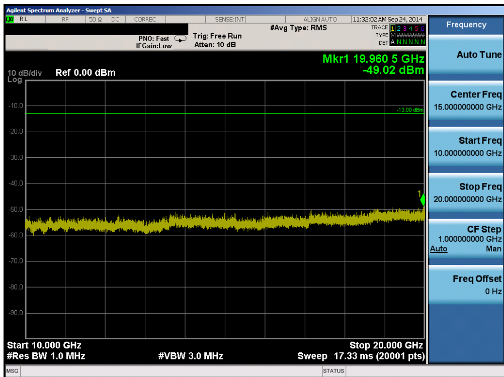
Plot 6-44. Conducted Spurious Plot (Band 4 – 10.0MHz QPSK – RB Size 1, RB Offset 0 – High Channel)
