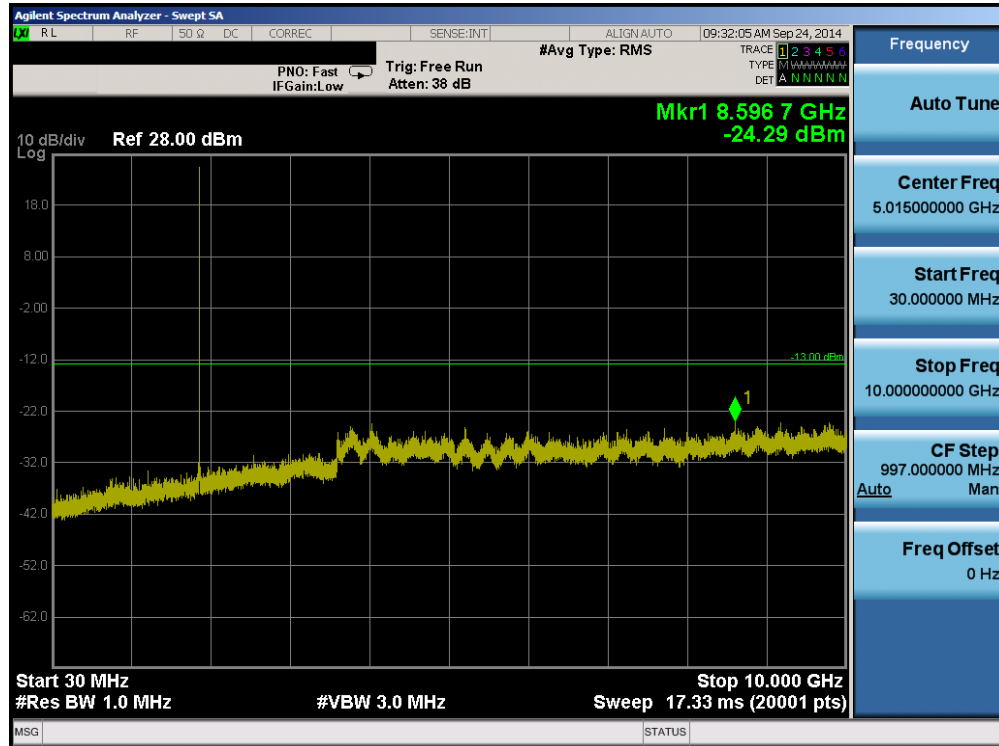
Plot 6-47. Conducted Spurious Plot (Band 2 – 5.0MHz QPSK – RB Size 1, RB Offset 0 – Mid Channel)
