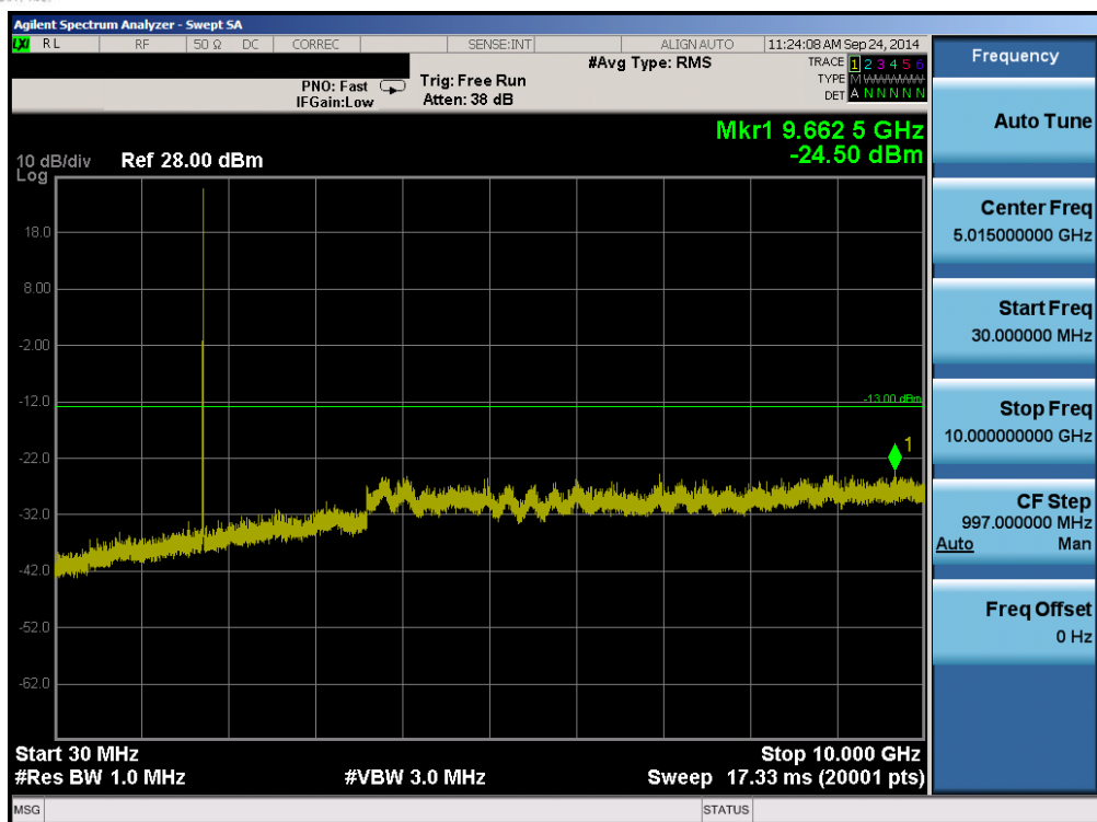
Plot 6-41. Conducted Spurious Plot (Band 4 – 10.0MHz QPSK – RB Size 1, RB Offset 0 – Mid Channel)
