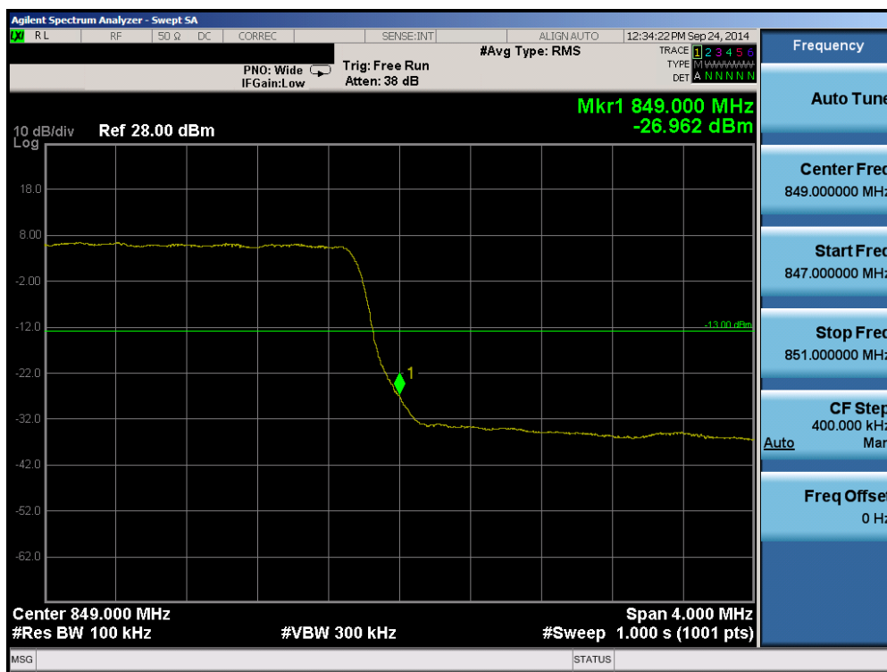
Plot 6-56. Upper Band Edge Plot (Band 5 – 5.0MHz QPSK – RB Size 25)
