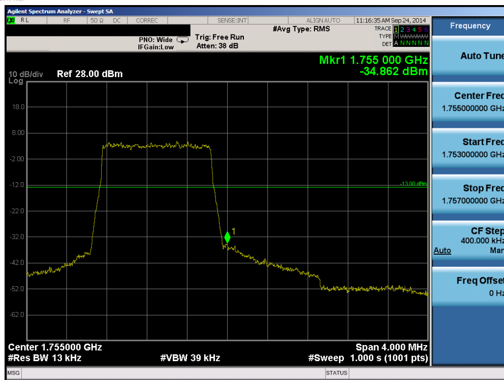
Plot 6-61. Upper Band Edge Plot (Band 4 – 1.4MHz QPSK – RB Size 6)
