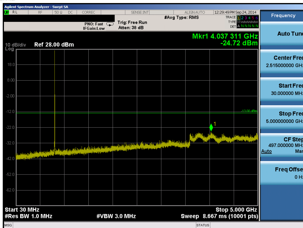
Plot 6-33. Conducted Spurious Plot (Band 5 – 5.0MHz QPSK – RB Size 1, RB Offset 0 – Low Channel)
