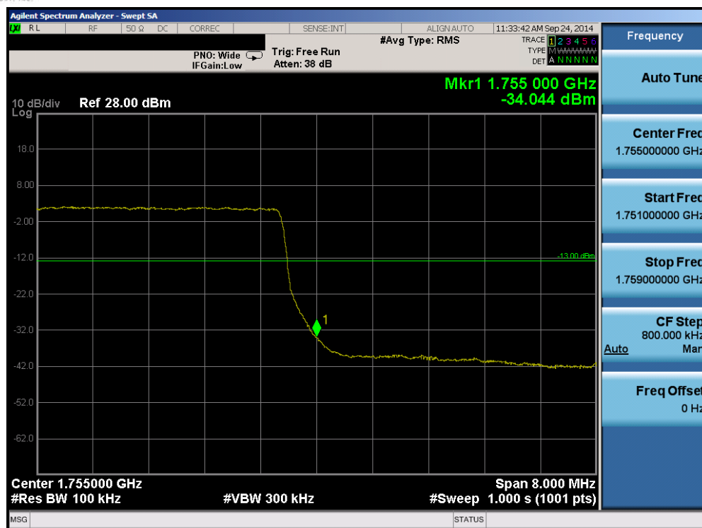
Plot 6-73. Upper Band Edge Plot (Band 4 – 10.0MHz QPSK – RB Size 50)
