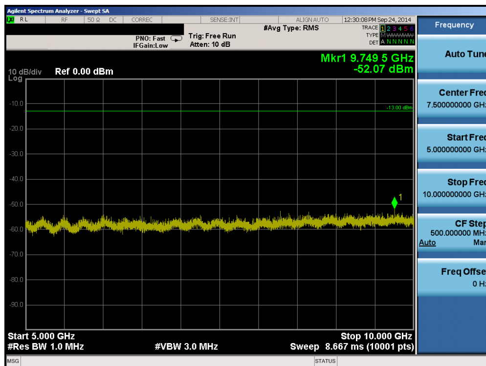
Plot 6-34. Conducted Spurious Plot (Band 5 – 5.0MHz QPSK – RB Size 1, RB Offset 0 – Low Channel)
