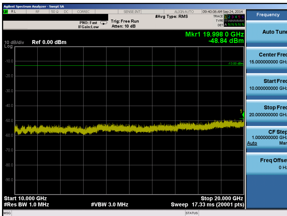
Plot 6-46. Conducted Spurious Plot (Band 2 – 5.0MHz QPSK – RB Size 1, RB Offset 0 – Low Channel)
