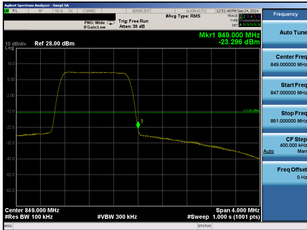
Plot 6-52. Upper Band Edge Plot (Band 5 – 1.4MHz QPSK – RB Size 6)
