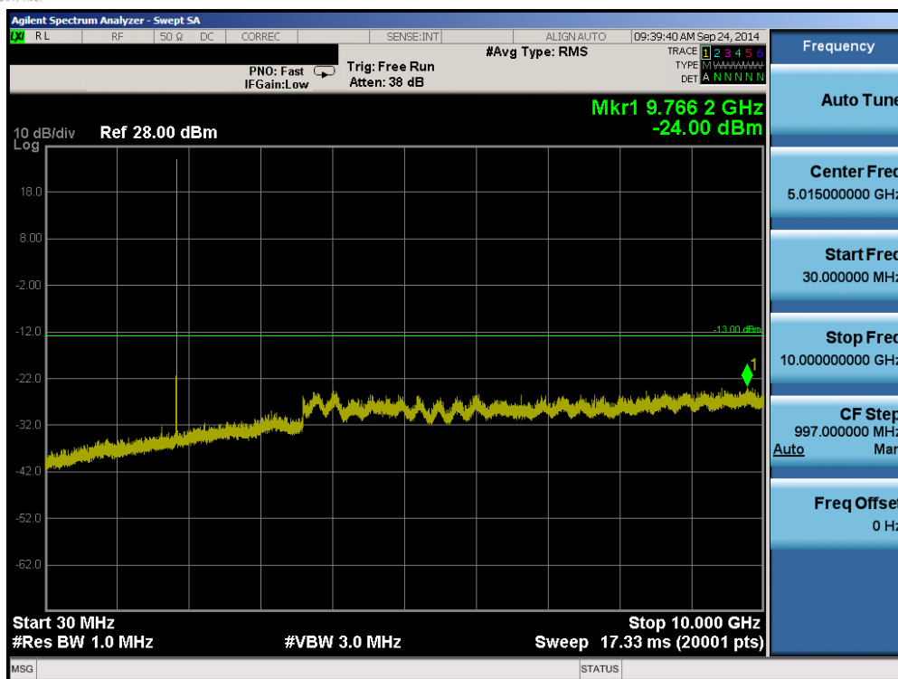
Plot 6-45. Conducted Spurious Plot (Band 2 – 5.0MHz QPSK – RB Size 1, RB Offset 0 – Low Channel)
