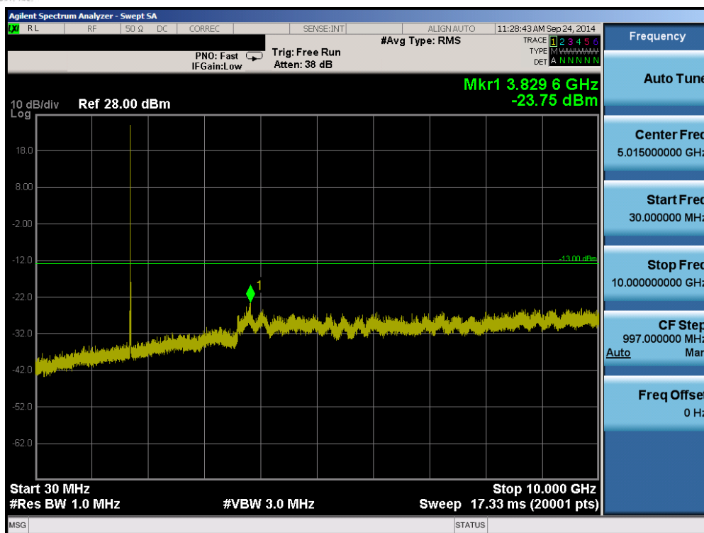
Plot 6-39. Conducted Spurious Plot (Band 4 – 10.0MHz QPSK – RB Size 1, RB Offset 0– Low Channel)
