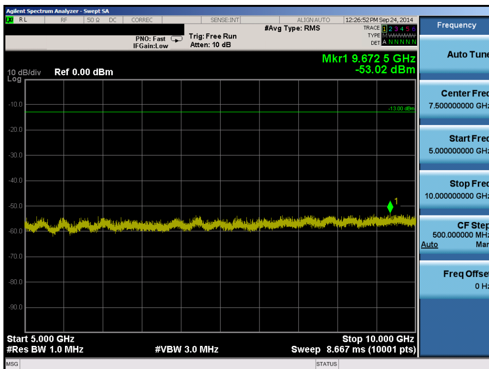
Plot 6-36. Conducted Spurious Plot (Band 5 – 5.0MHz QPSK – RB Size 1, RB Offset 0 – Mid Channel)
