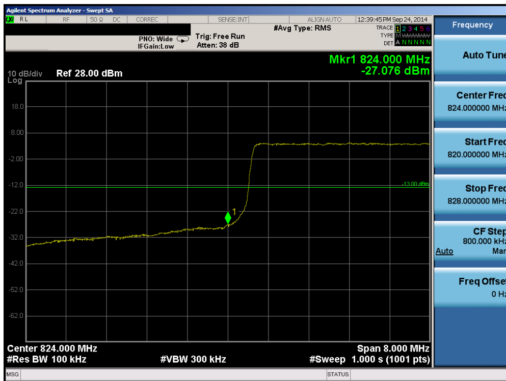
Plot 6-57. Lower Band Edge Plot (Band 5 - 10.0MHz QPSK - RB Size 50)
