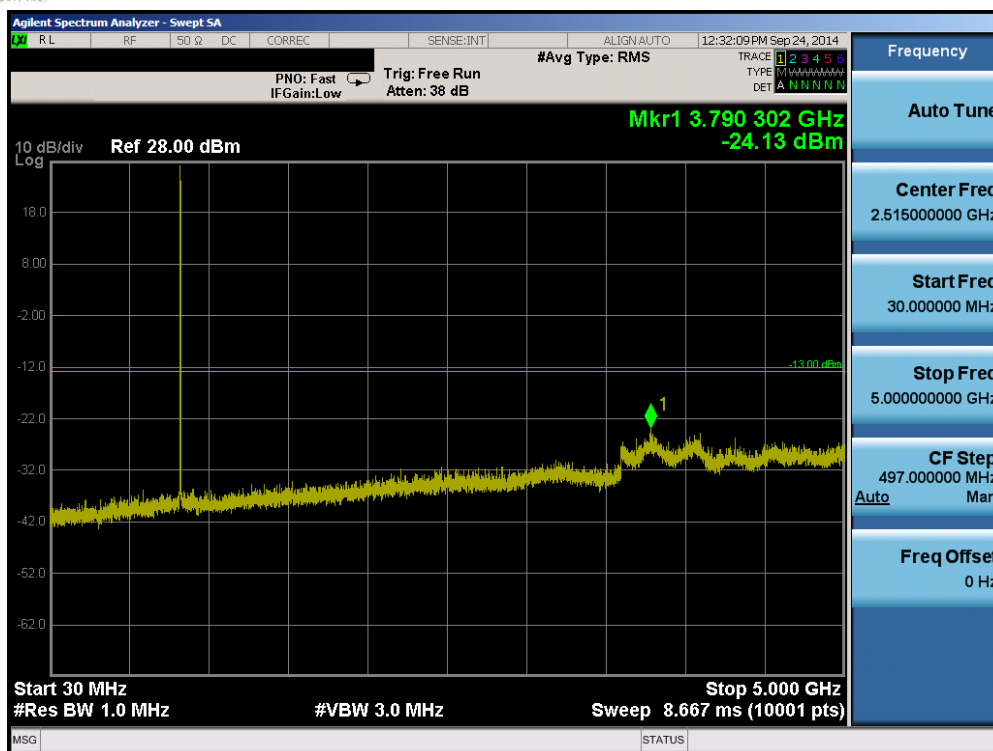
Plot 6-37. Conducted Spurious Plot (Band 5 – 5.0MHz QPSK – RB Size 1, RB Offset 0 – High Channel)
