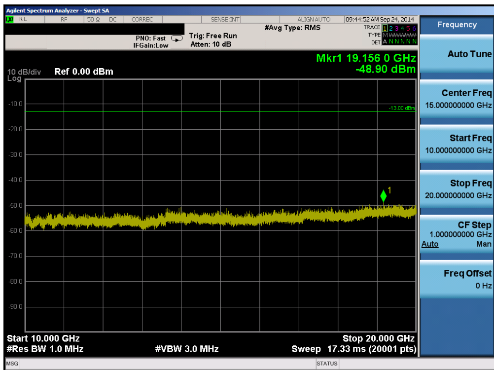
Plot 6-50. Conducted Spurious Plot (Band 2 – 5.0MHz QPSK – RB Size 1, RB Offset 0 – High Channel)
