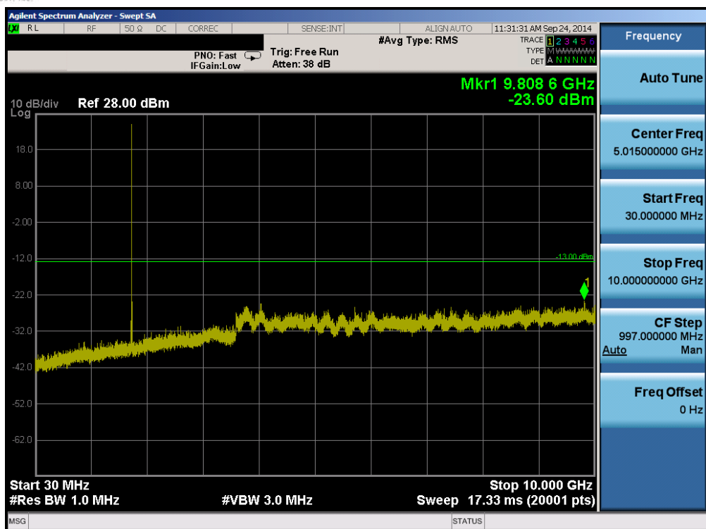
Plot 6-43. Conducted Spurious Plot (Band 4 – 10.0MHz QPSK – RB Size 1, RB Offset 0 – High Channel)
