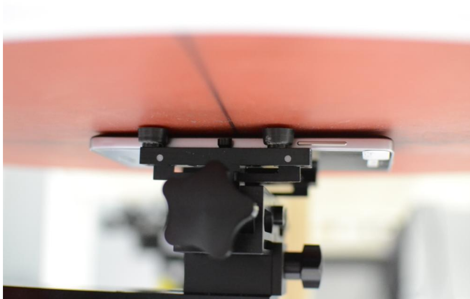
SAR Test Setup Photo 5 – Back Side at 0.0 cm (Extremity)
