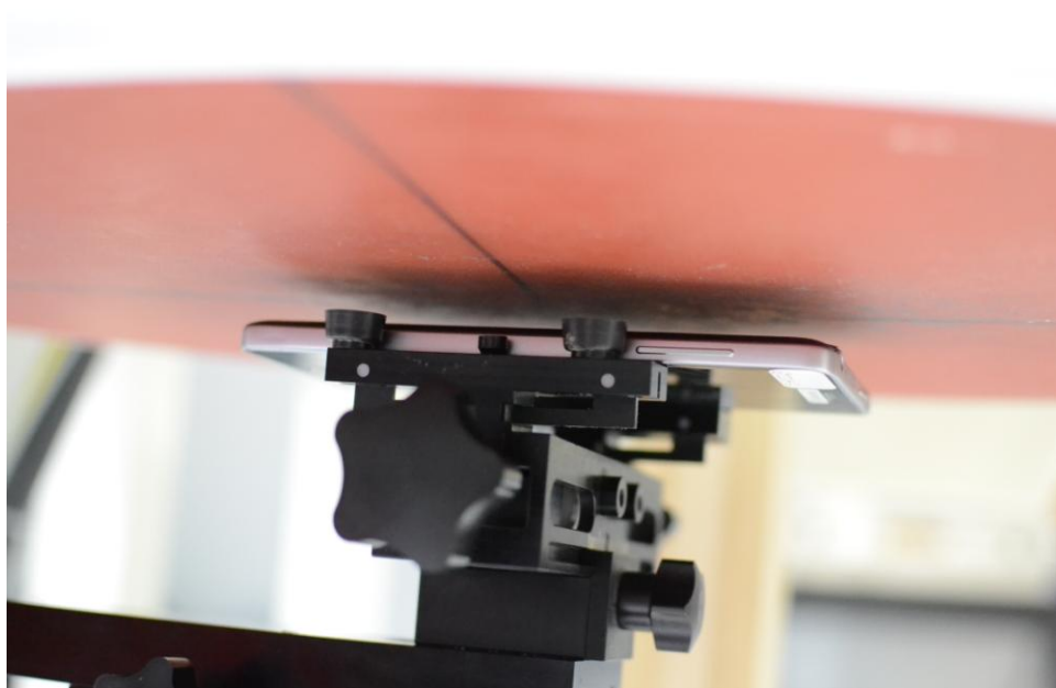
SAR Test Setup Photo 6 – Back Side at 1.0 cm (Body-worn and Hotspot)
