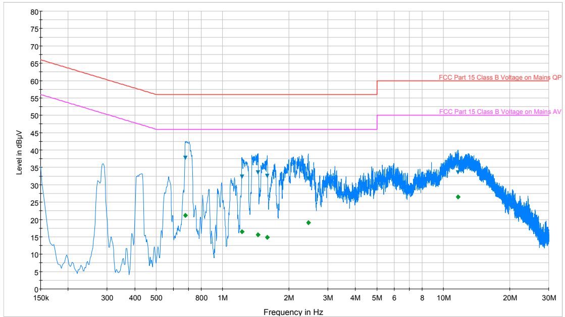
Plot 6-6. Line-Conducted Test Plot (L1)
