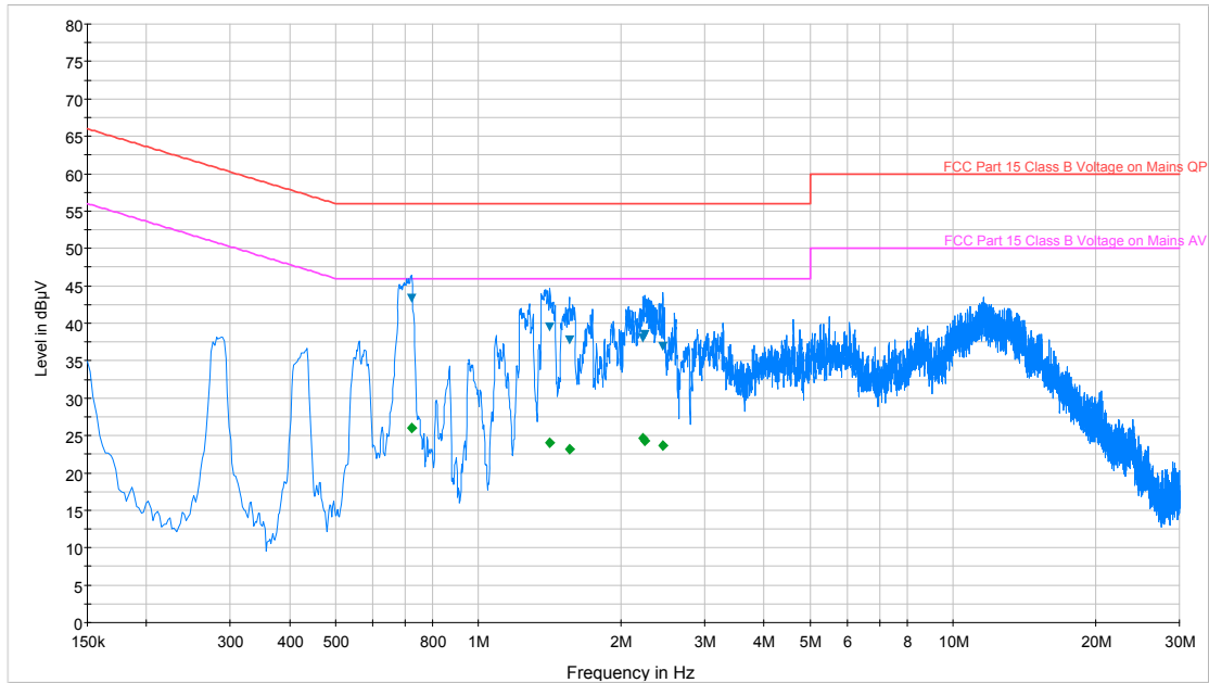
Plot 6-7. Line-Conducted Test Plot (N)
