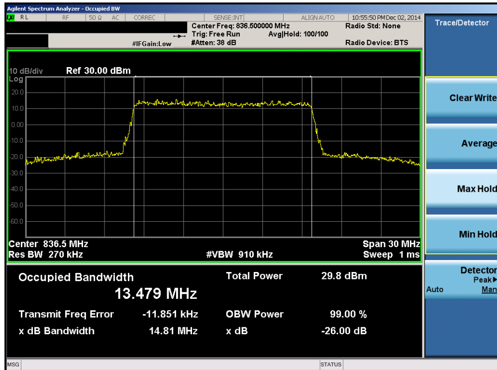
Plot 6-2. Occupied Bandwidth Plot (Band 26 – 15.0MHz 16-QAM – RB Size 75)
