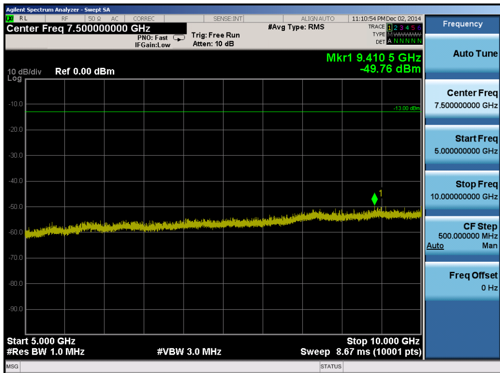
Plot 6-8. Conducted Spurious Plot (Band 26 – 15.0MHz QPSK – RB Size 1, RB Offset 0 – High Channel)
