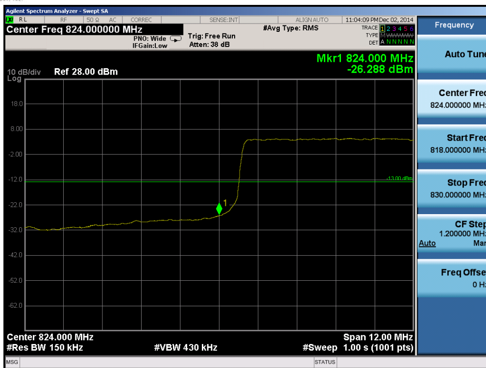
Plot 6-9. Lower Band Edge Plot (Band 26 – 15.0MHz QPSK – RB Size 75)
