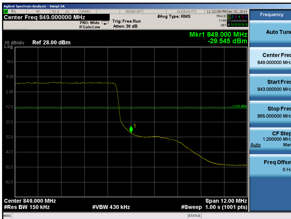
Plot 6-10. Upper Band Edge Plot (Band 26 – 15.0MHz QPSK – RB Size 75)
