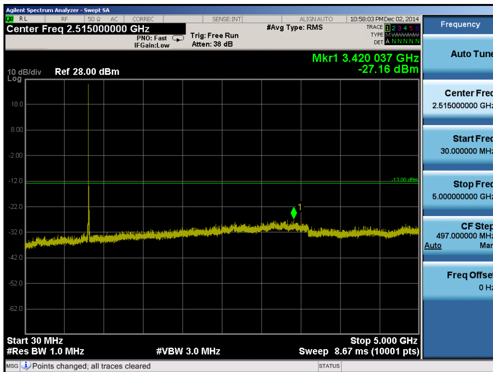
Plot 6-5. Conducted Spurious Plot (Band 26 – 15.0MHz QPSK – RB Size 1, RB Offset 0 – Mid Channel)
