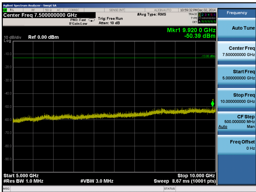
Plot 6-4. Conducted Spurious Plot (Band 26 – 15.0MHz QPSK – RB Size 1, RB Offset 0 – Low Channel)
