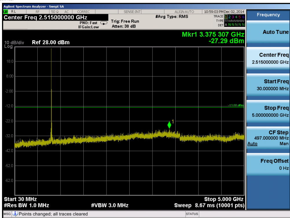
Plot 6-3. Conducted Spurious Plot (Band 26 – 15.0MHz QPSK – RB Size 1, RB Offset 0 – Low Channel)
