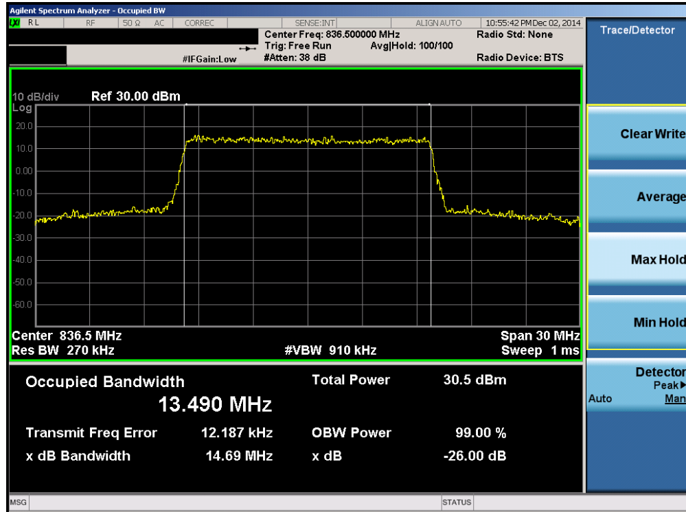
Plot 6-1. Occupied Bandwidth Plot (Band 26 – 15.0MHz QPSK – RB Size 75)
