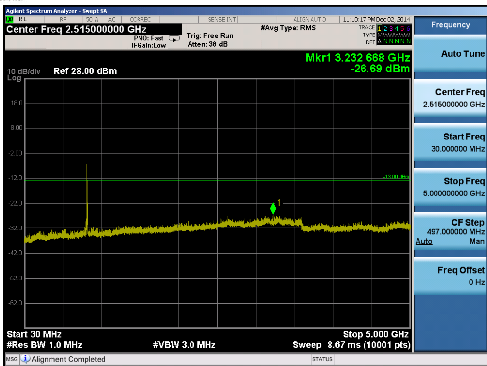
Plot 6-7. Conducted Spurious Plot (Band 26 – 15.0MHz QPSK – RB Size 1, RB Offset 0 – High Channel)
