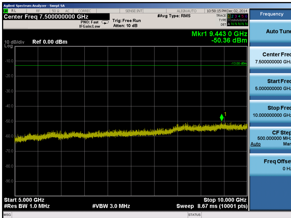
Plot 6-6. Conducted Spurious Plot (Band 26 – 15.0MHz QPSK – RB Size 1, RB Offset 0 – Mid Channel)
