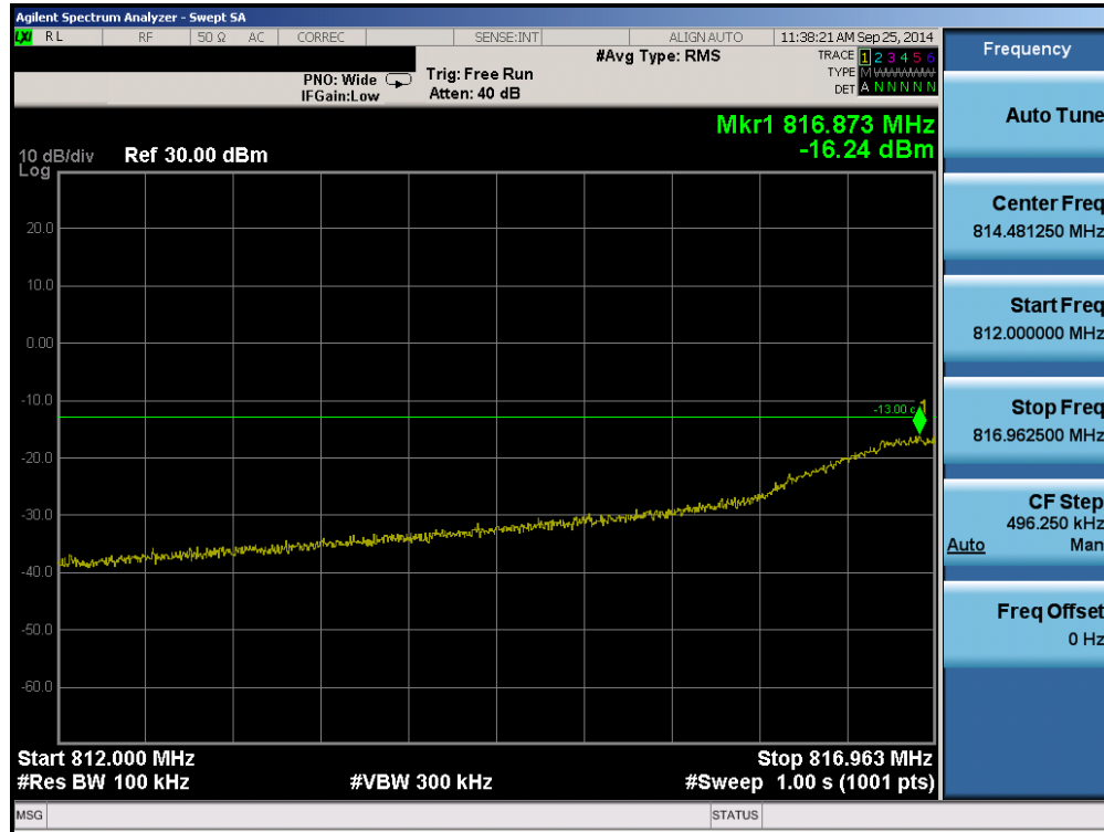
Plot 7-5. Outer Extended Band Edge Plot (Ch. 476)
