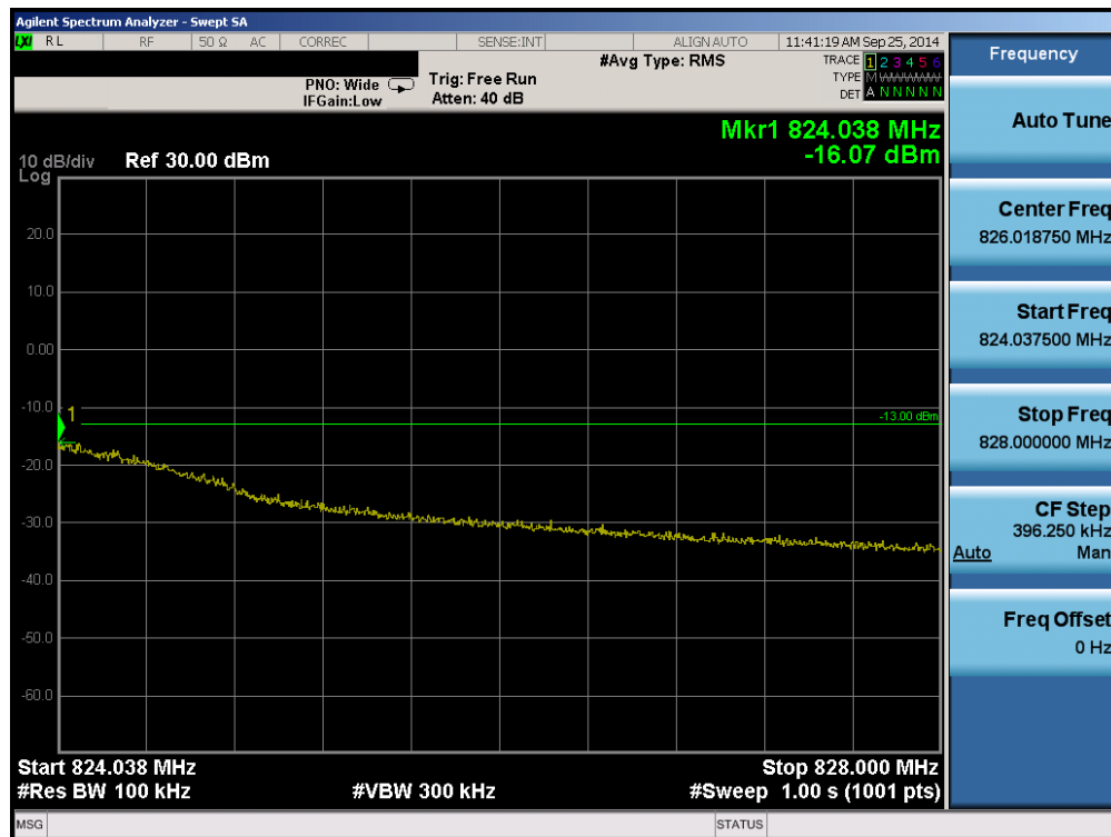
Plot 7-10. Outer Extended Band Edge Plot (Ch. 684)
