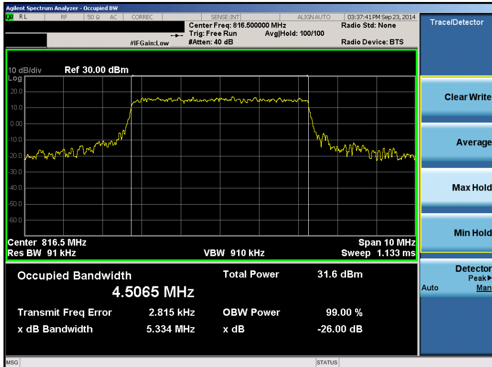
Plot 8-18. Occupied Bandwidth Plot (5MHz 16QAM – RB Size 25– Low Channel)
