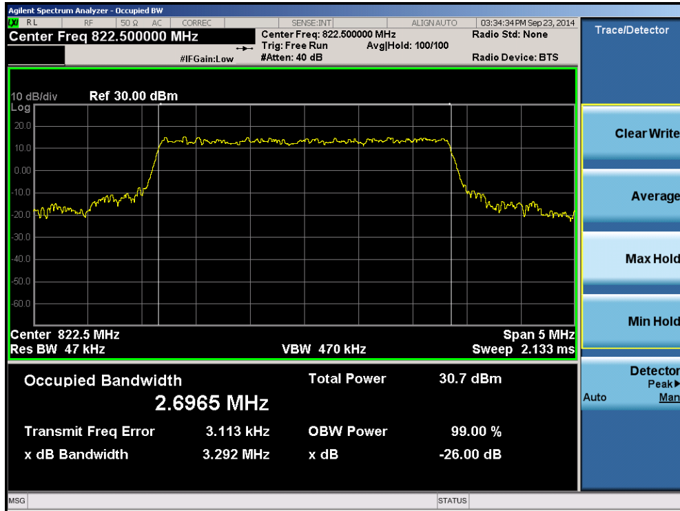
Plot 8-15. Occupied Bandwidth Plot (3MHz 16QAM – RB Size 15– High Channel)
