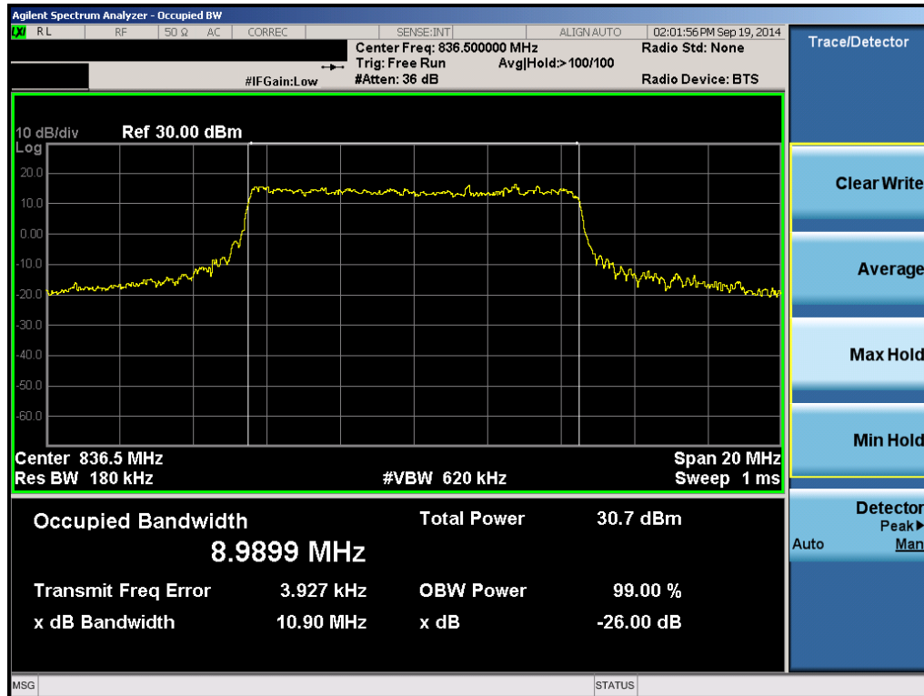
Plot 8-24. Occupied Bandwidth Plot (10MHz 16QAM – RB Size 50)
