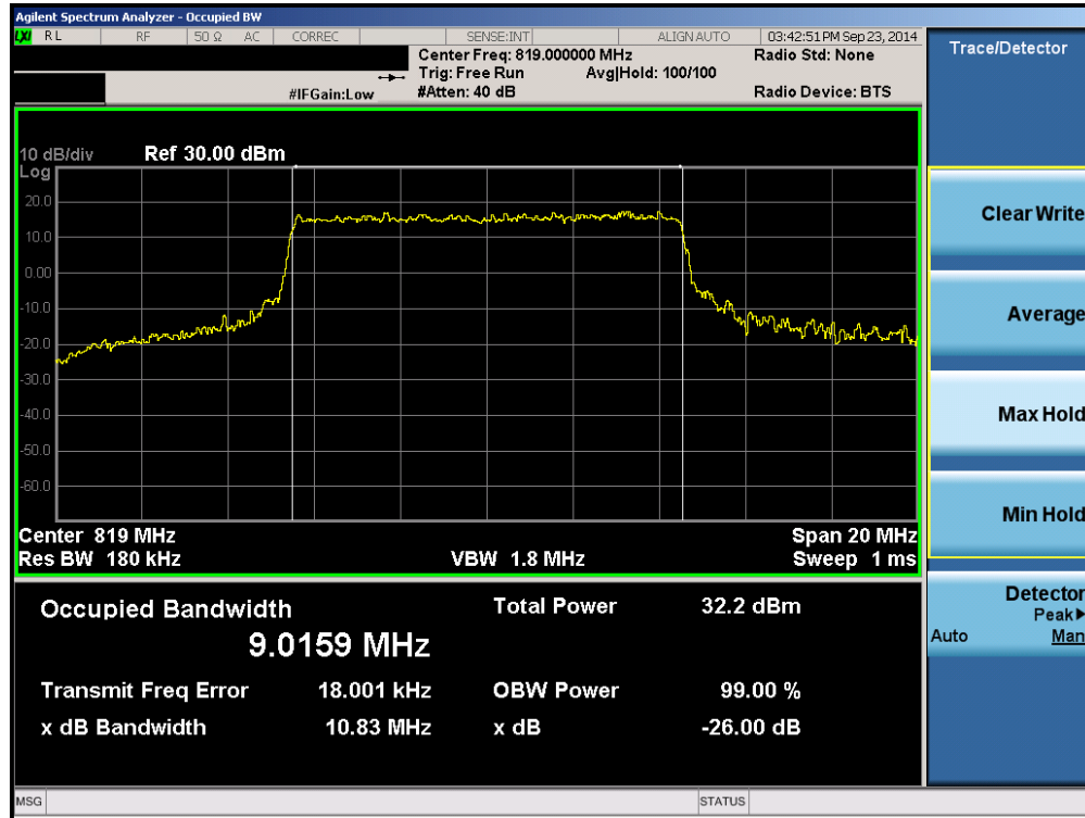
Plot 8-23. Occupied Bandwidth Plot (10MHz QPSK – RB Size 50)
