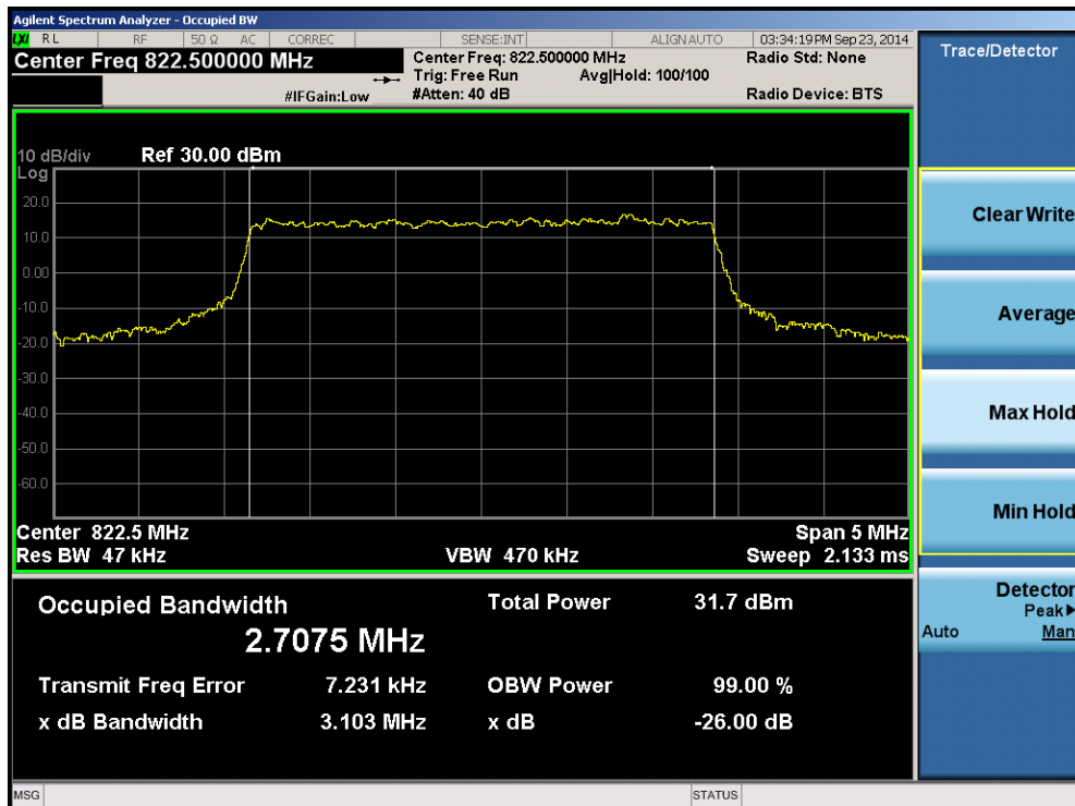
Plot 8-14. Occupied Bandwidth Plot (3MHz QPSK – RB Size 15– High Channel)
