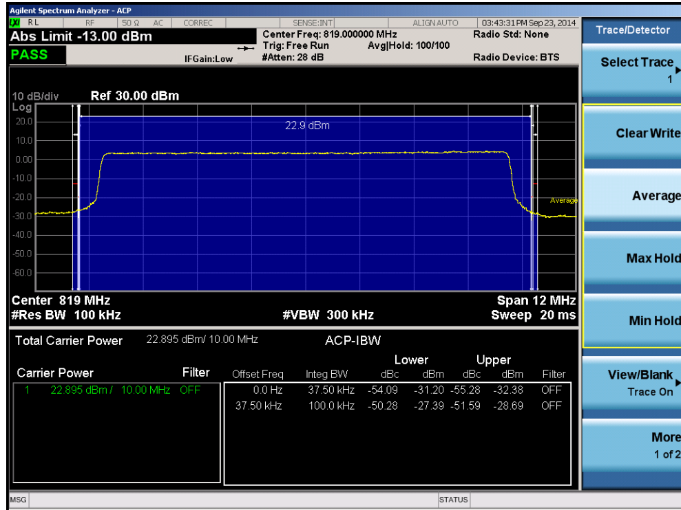
Plot 8-25. Adjacent Channel Plot (10MHz QPSK – RB Size 50)
