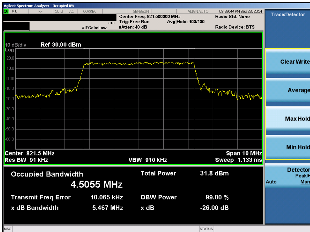
Plot 8-20. Occupied Bandwidth Plot (5MHz QPSK – RB Size 25 – High Channel)
