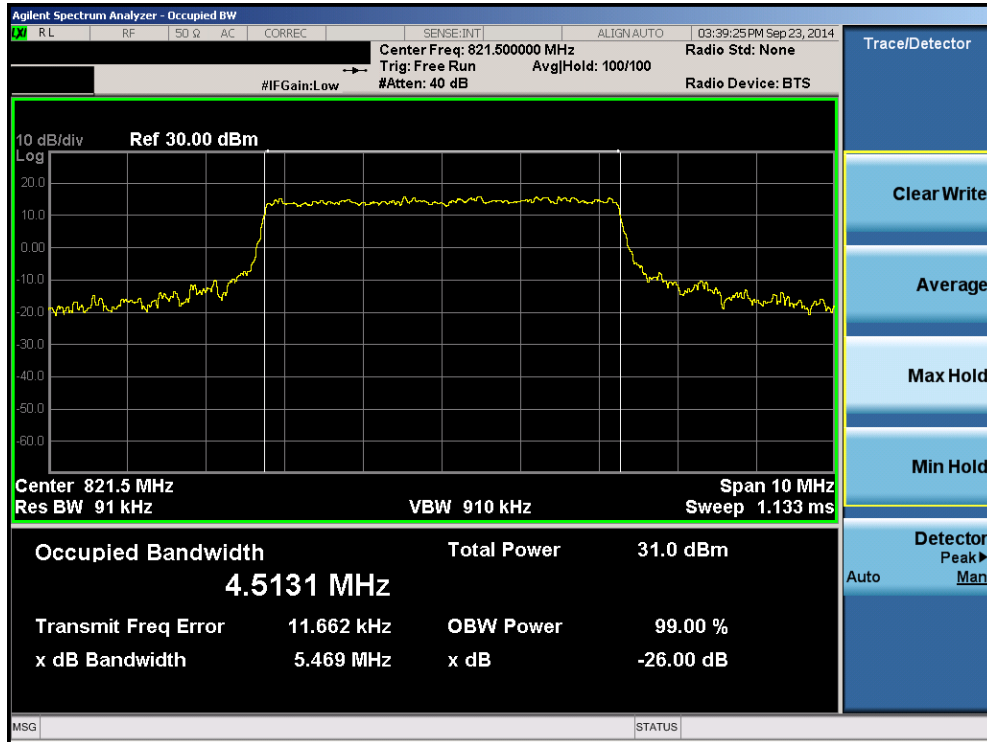
Plot 8-21. Occupied Bandwidth Plot (5MHz 16QAM – RB Size 25 – High Channel)
