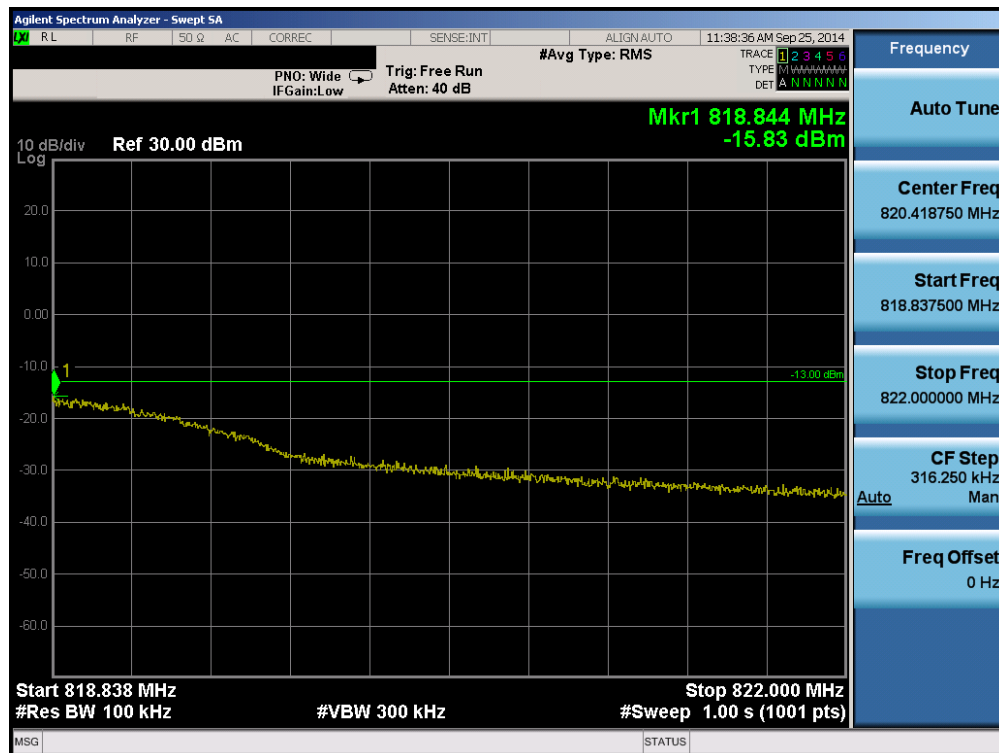
Plot 7-4. Inner Extended Band Edge Plot (Ch. 476)
