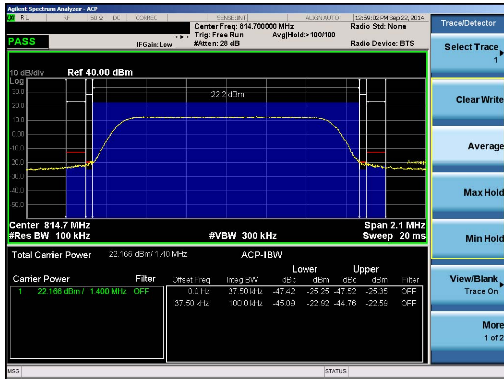
Plot 8-3. Adjacent Channel Plot (1.4MHz QPSK – RB Size 6, RB Offset 0 – Low Channel)
