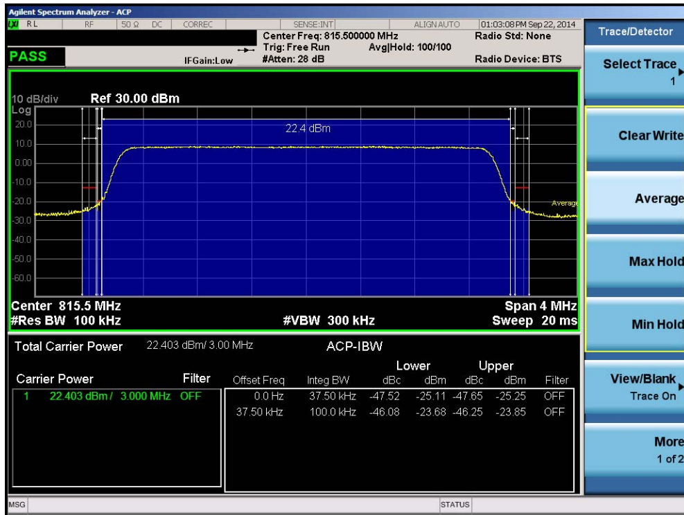
Plot 8-13. Adjacent Channel Plot (3MHz QPSK – RB Size 15– Low Channel)
