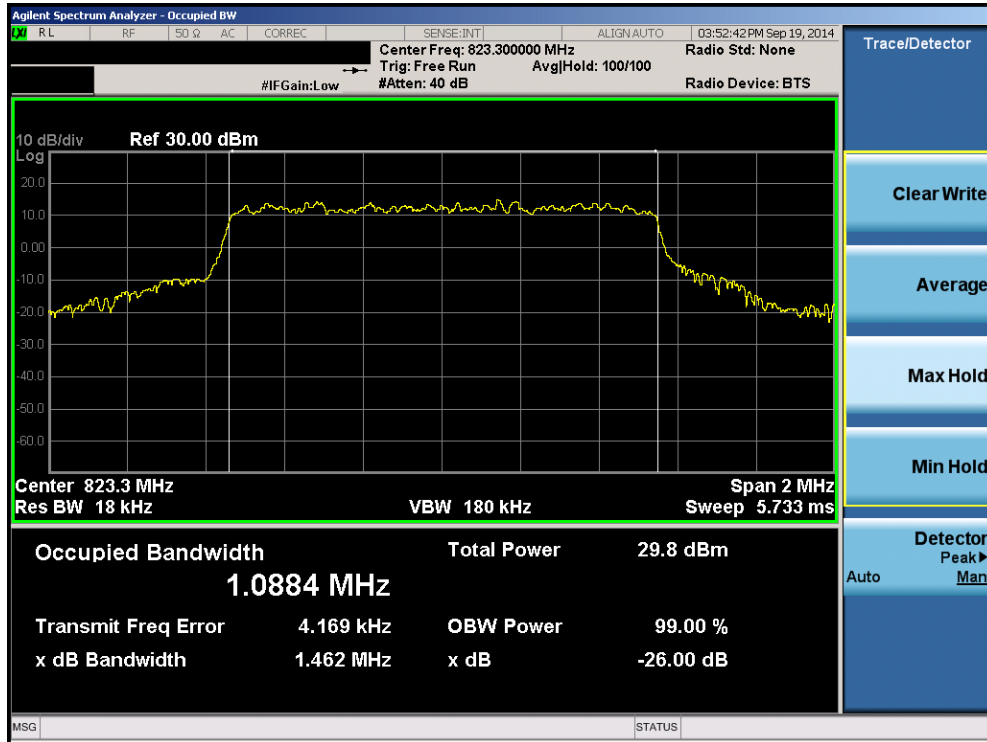
Plot 8-9. Occupied Bandwidth Plot (1.4MHz 16QAM – RB Size 6, RB Offset 0 – High Channel)
