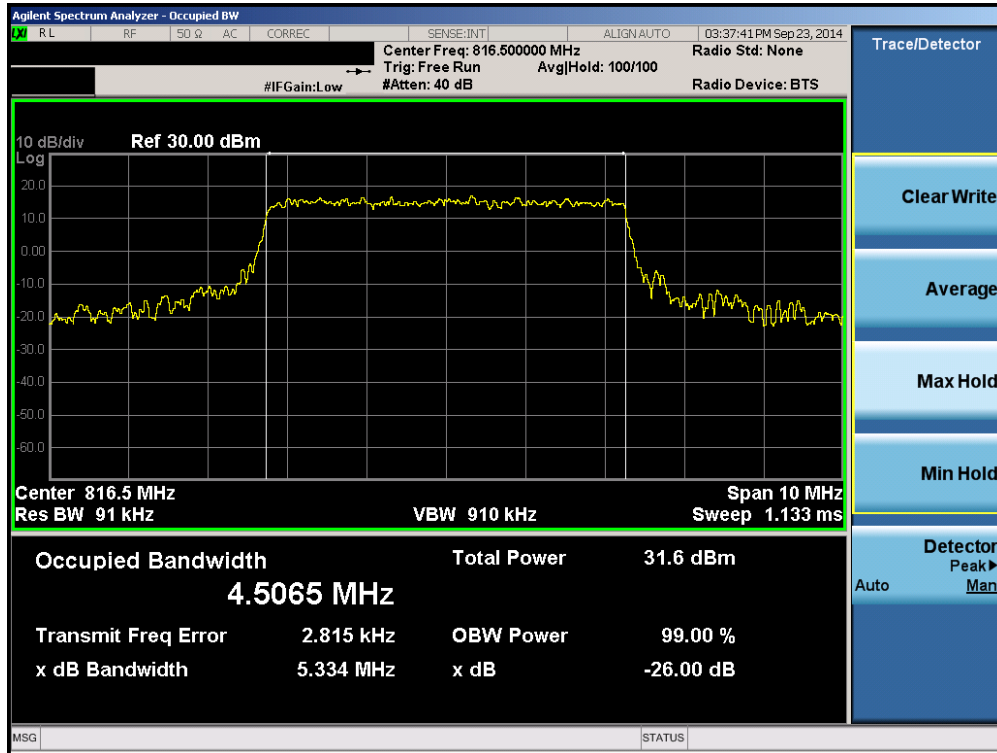
Plot 8-17. Occupied Bandwidth Plot (5MHz QPSK – RB Size 25– Low Channel)
