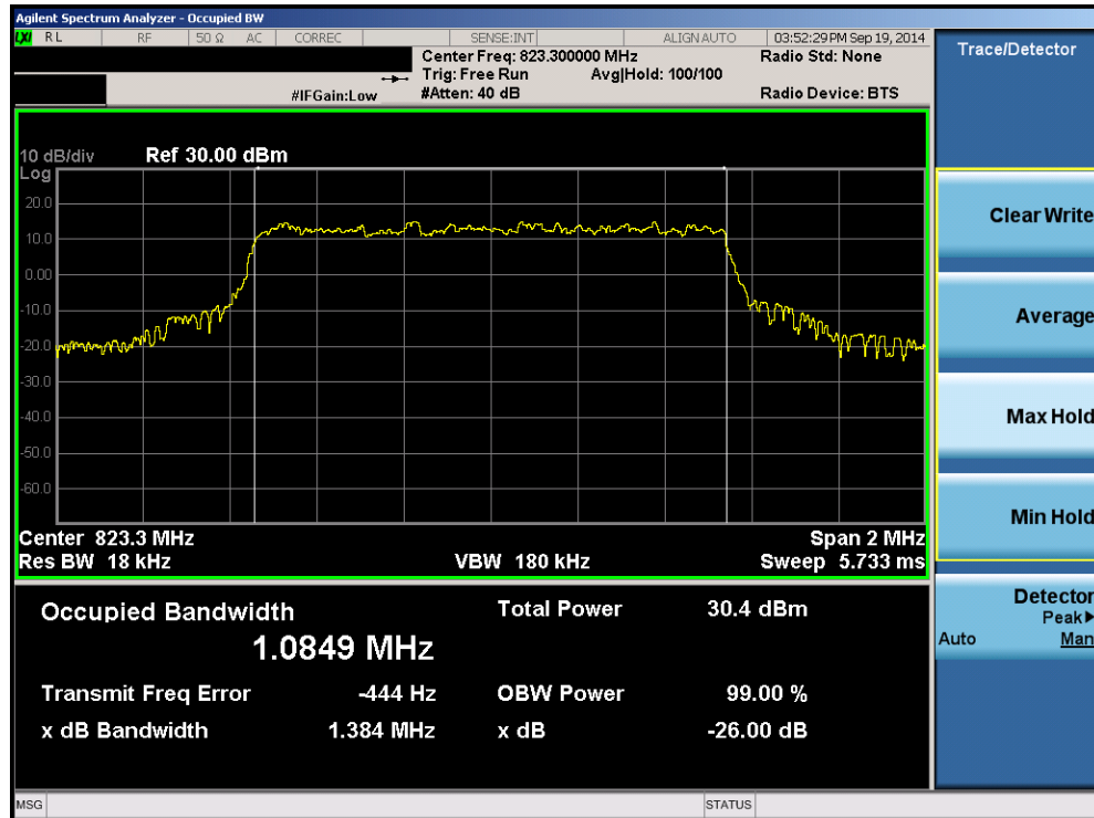
Plot 8-8. Occupied Bandwidth Plot (1.4MHz QPSK – RB Size 6, RB Offset 0 – High Channel)
