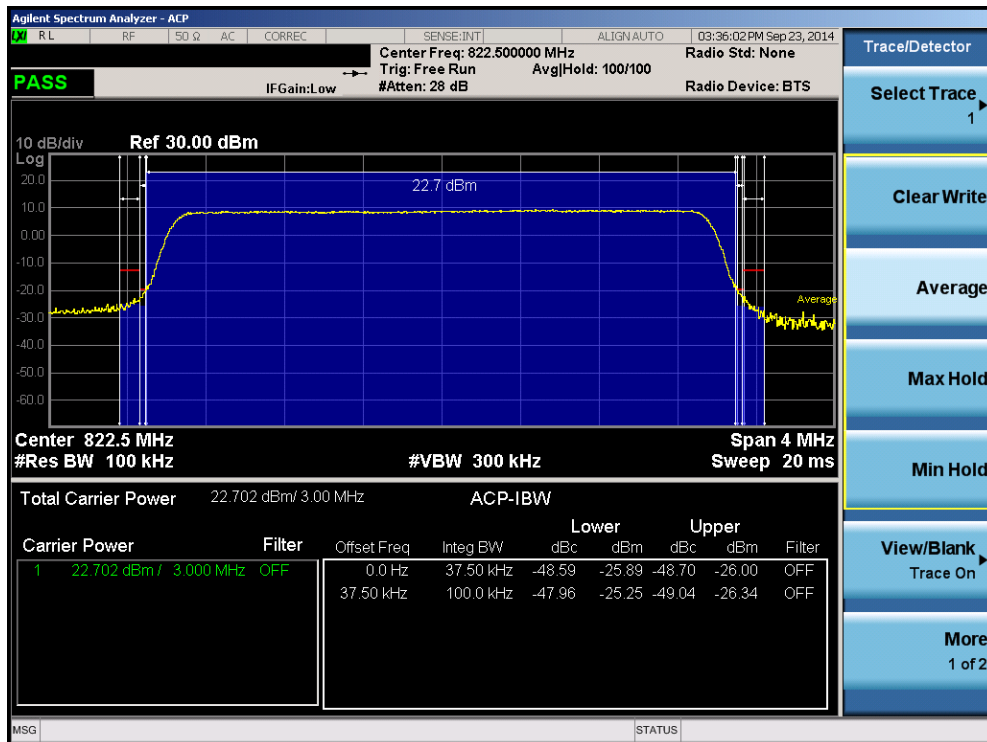
Plot 8-16. Adjacent Channel Plot (3MHz QPSK – RB Size 15– High Channel)
