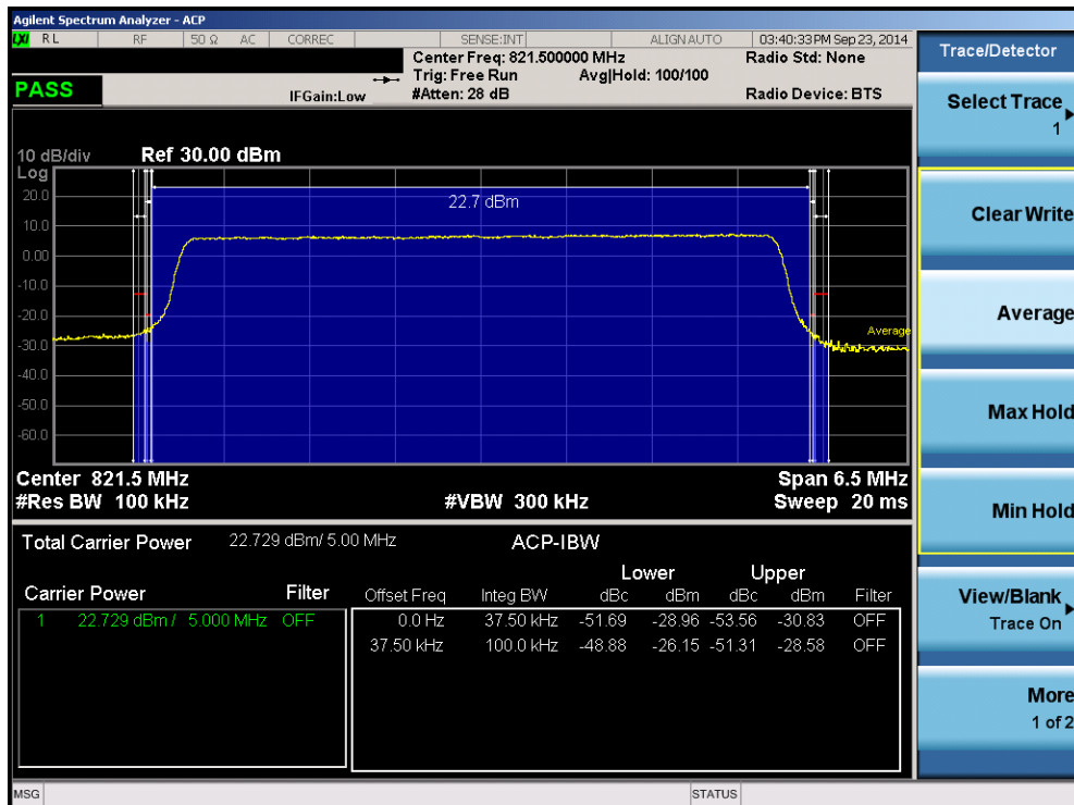
Plot 8-22. Adjacent Channel Plot (5MHz QPSK – RB Size 25 – High Channel)
