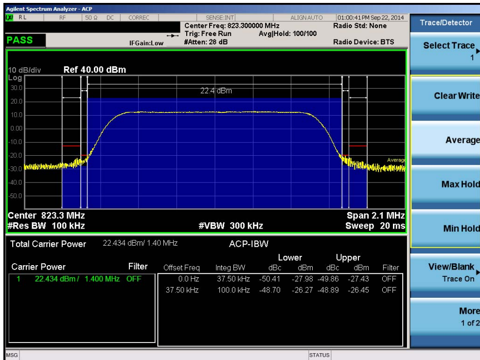
Plot 8-10. Adjacent Channel Plot (1.4MHz QPSK – RB Size 6, RB Offset 0 – High Channel)
