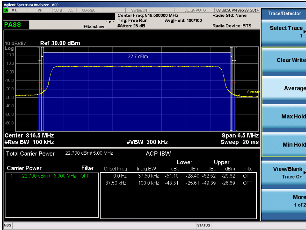
Plot 8-19. Adjacent Channel Plot (5MHz QPSK – RB Size 25– Low Channel)
