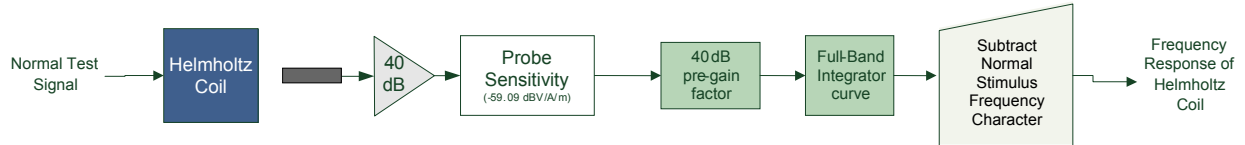
Figure 5-12 Frequency Response Block Diagram
