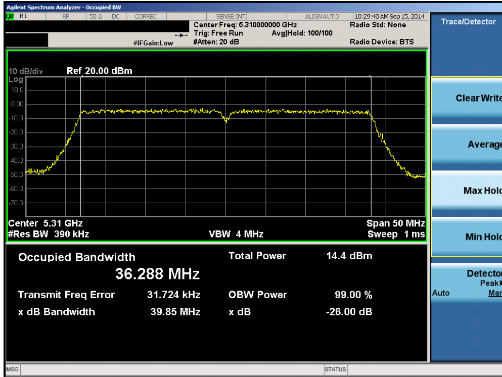
Plot 6-53. 26dB Bandwidth Plot (40MHz BW 802.11n (UNII Band 2A) – Ch. 62)
