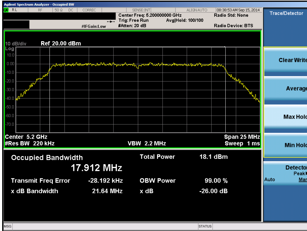
Plot 6-41. 26dB Bandwidth Plot (20MHz BW 802.11n (UNII Band 1) – Ch. 40)
