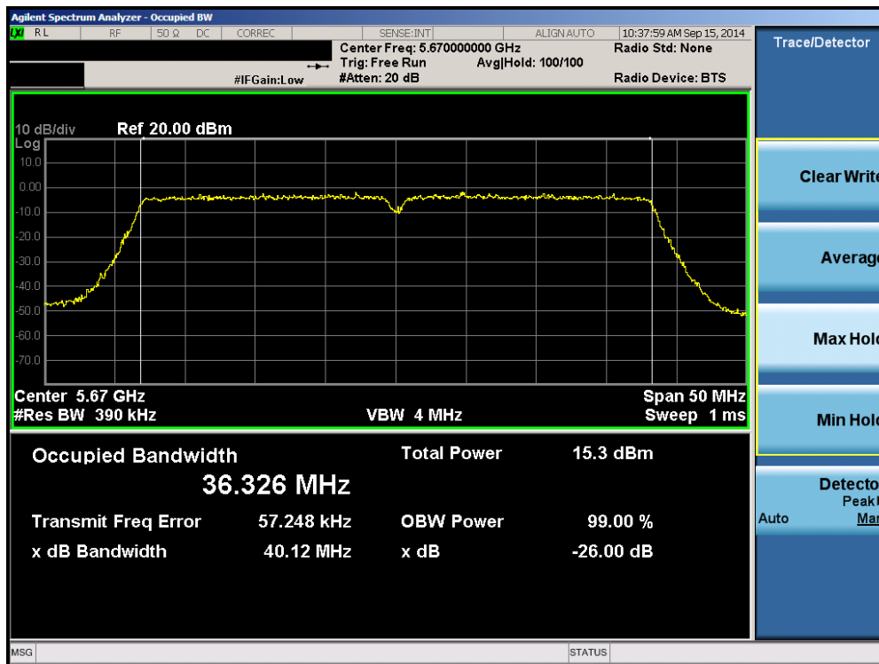
Plot 6-63. 26dB Bandwidth Plot (40MHz BW 802.11n (UNII Band 2C) – Ch. 134)
