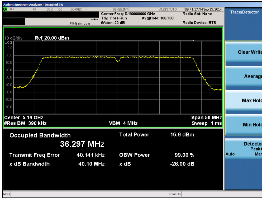
Plot 6-43. 26dB Bandwidth Plot (40MHz BW 802.11n (UNII Band 1) – Ch. 38)
