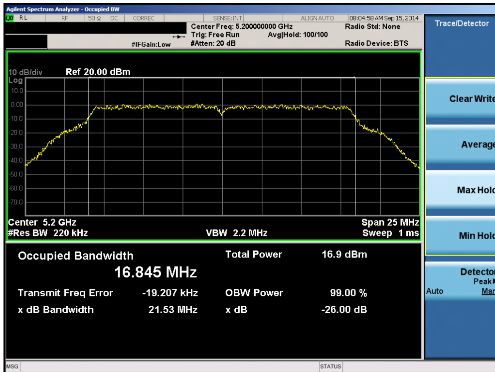
Plot 6-38. 26dB Bandwidth Plot (802.11a (UNII Band 1) – Ch. 40)
