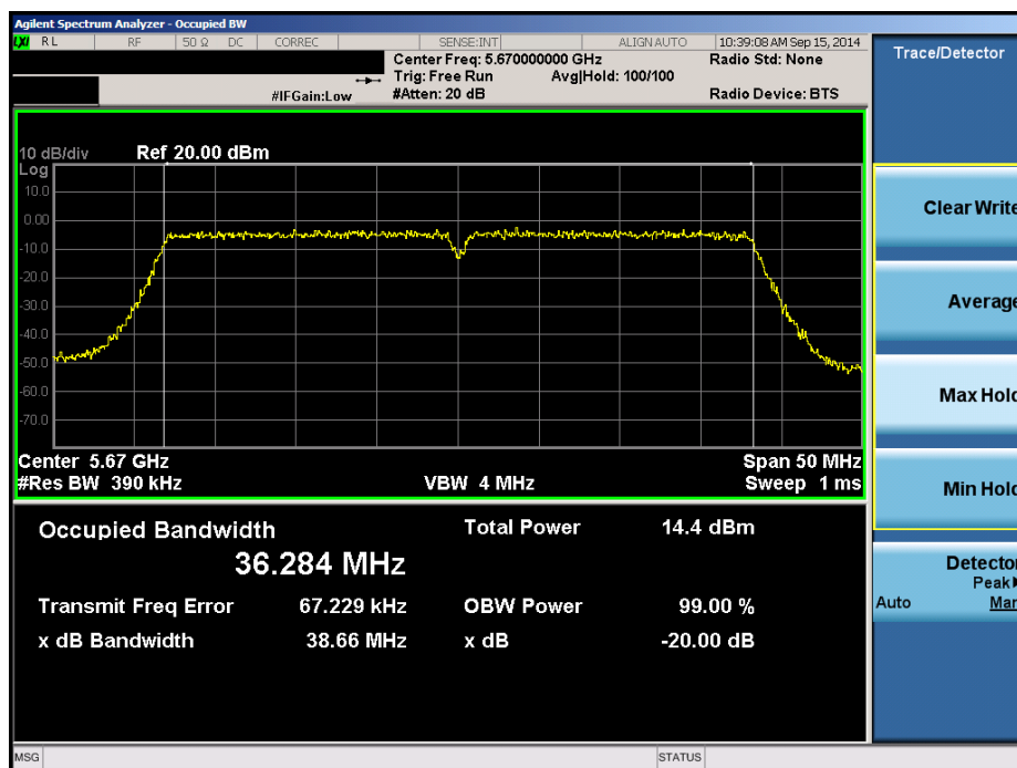
Plot 6-68. 20dB Bandwidth Plot (40MHz BW 802.11n (UNII Band 2C) – Ch. 134)
