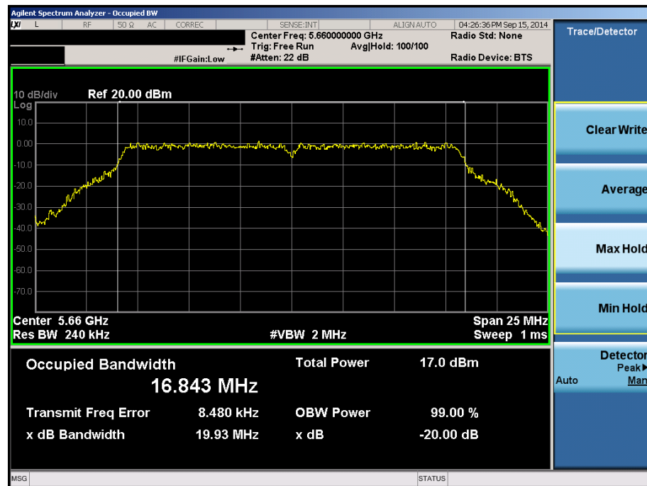
Plot 6-70. 20dB Bandwidth (20MHz BW 802.11n (UNII Band 2C) – Ch. 132)
