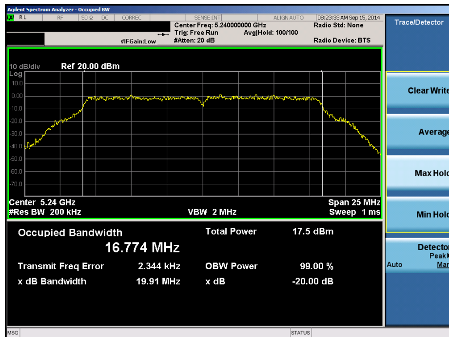
Plot 6-65. 20dB Bandwidth Plot (20MHz BW 802.11a (UNII Band 1) – Ch. 48)
