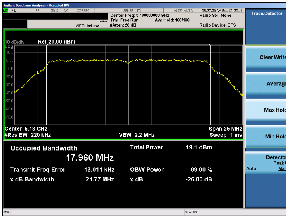
Plot 6-40. 26dB Bandwidth Plot (20MHz BW 802.11n (UNII Band 1) – Ch. 36)
