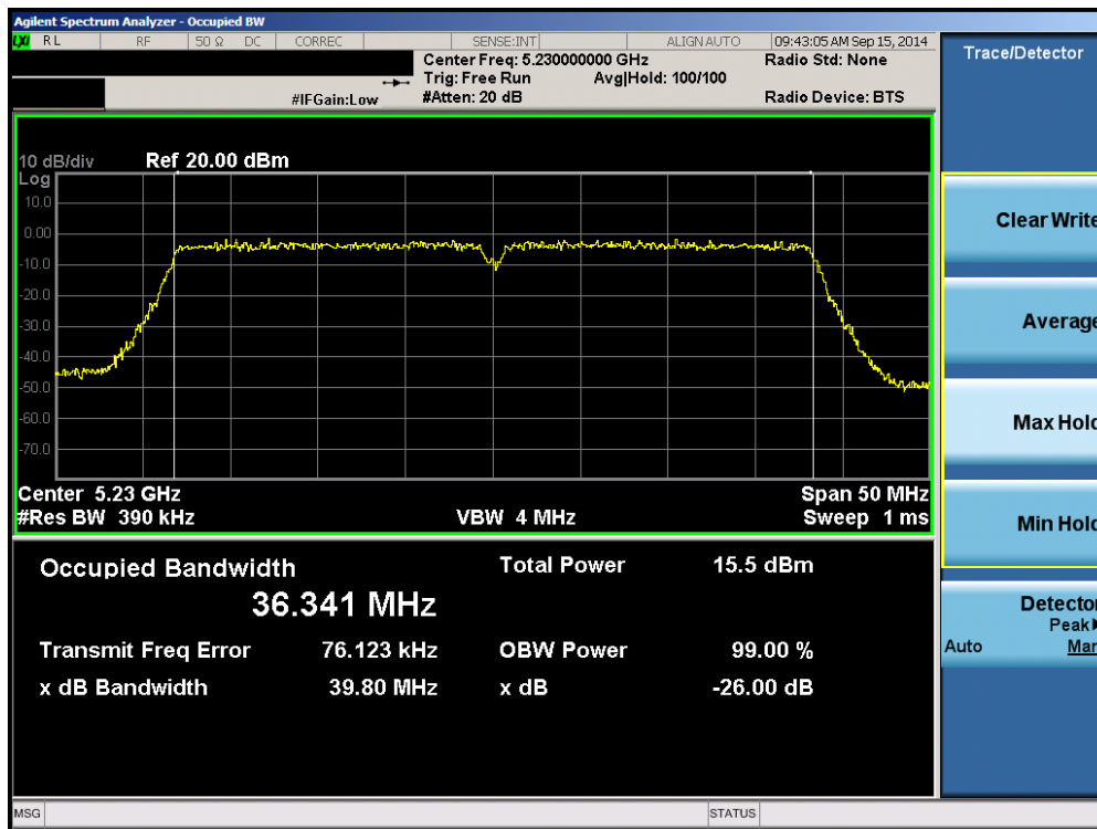
Plot 6-44. 26dB Bandwidth Plot (40MHz BW 802.11n (UNII Band 1) – Ch. 46)
