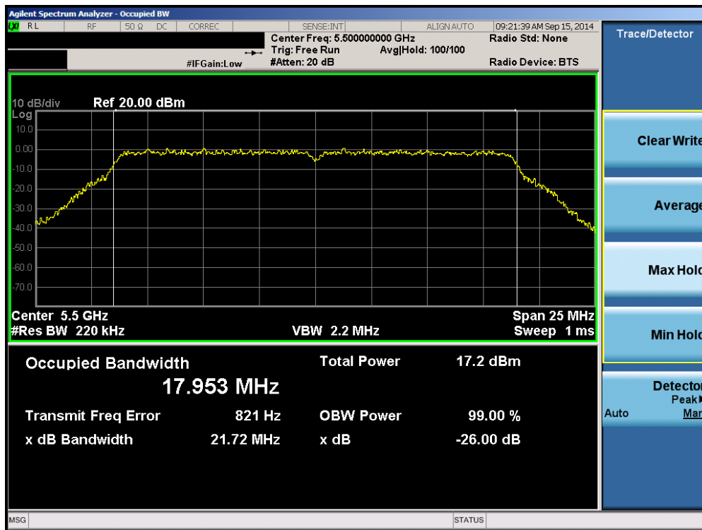
Plot 6-58. 26dB Bandwidth Plot (20MHz BW 802.11n (UNII Band 2C) – Ch. 100)
