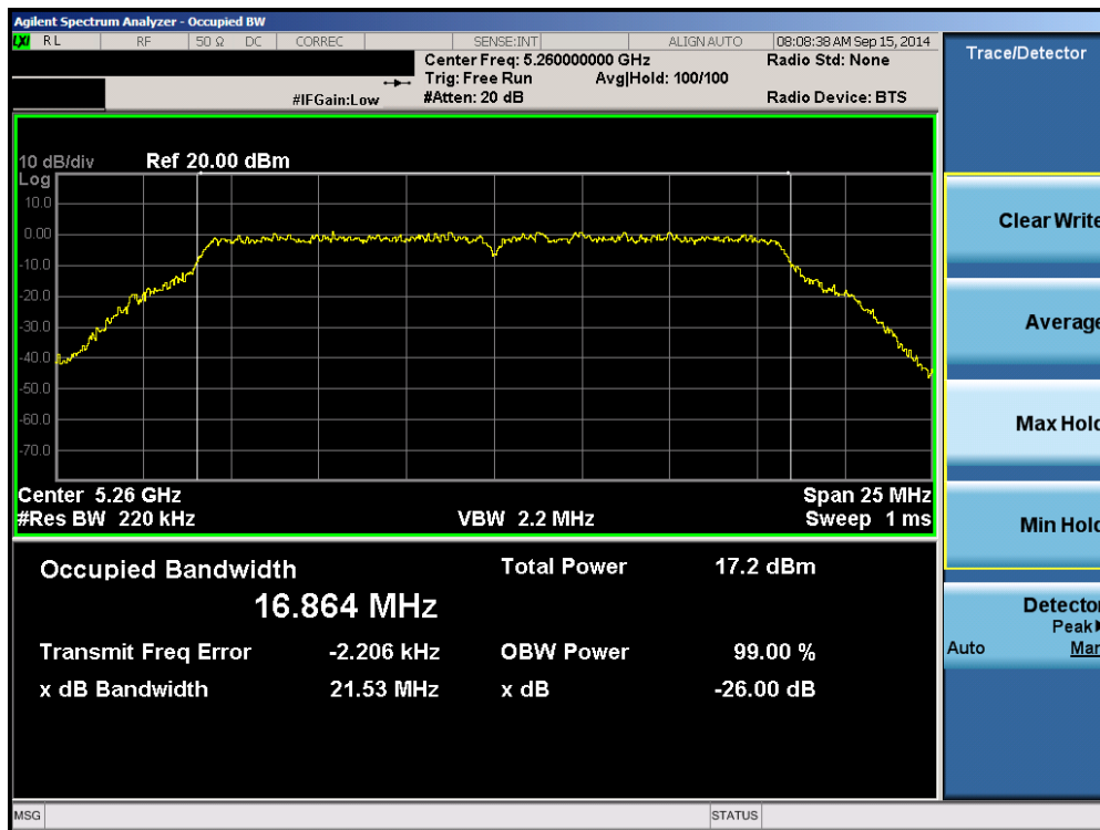
Plot 6-46. 26dB Bandwidth Plot (802.11a (UNII Band 2A) – Ch. 52)
