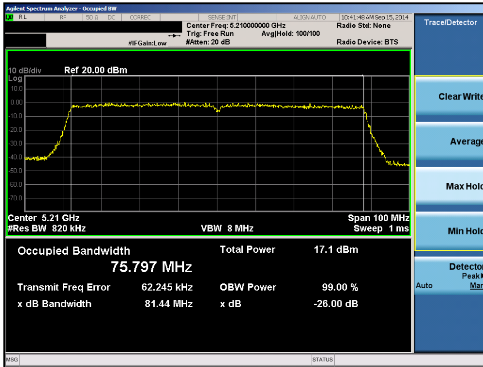
Plot 6-45. 26dB Bandwidth Plot (80MHz BW 802.11ac (UNII Band 1) – Ch. 42)
