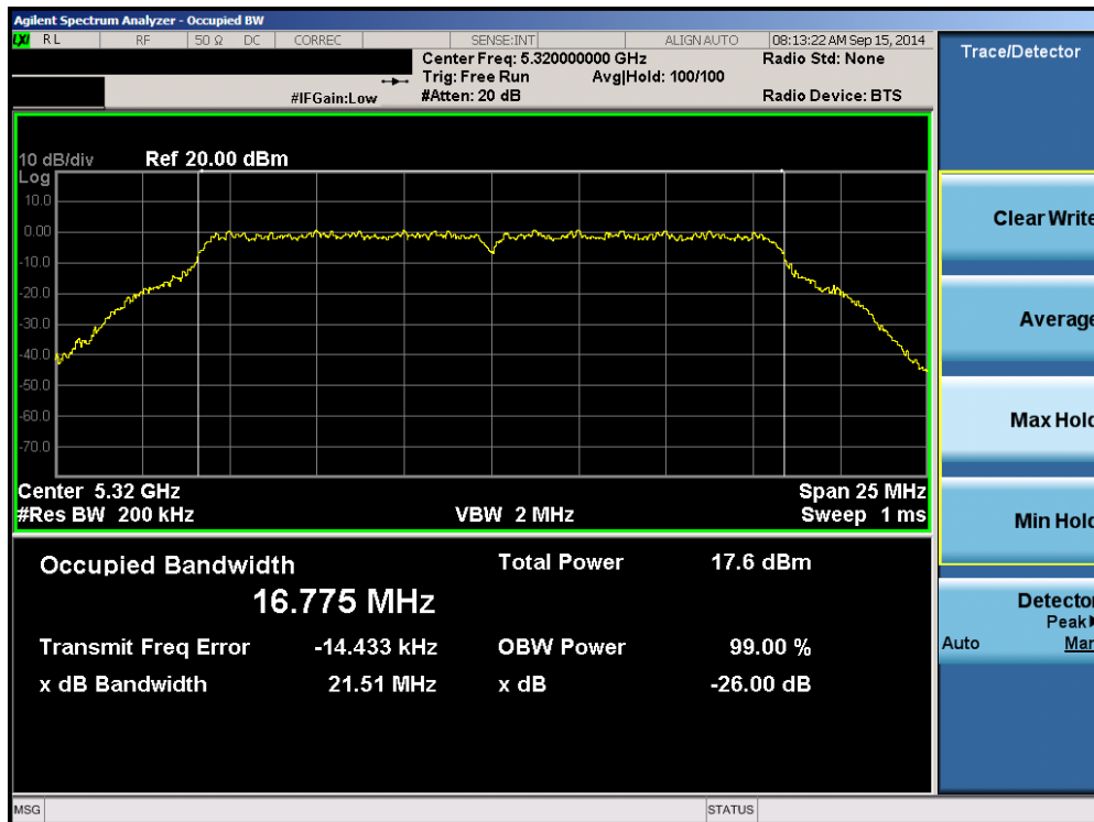
Plot 6-48. 26dB Bandwidth Plot (802.11a (UNII Band 2A) – Ch. 64)
