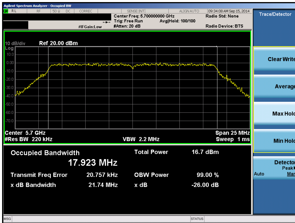
Plot 6-60. 26dB Bandwidth Plot (20MHz BW 802.11n (UNII Band 2C) – Ch. 140)
