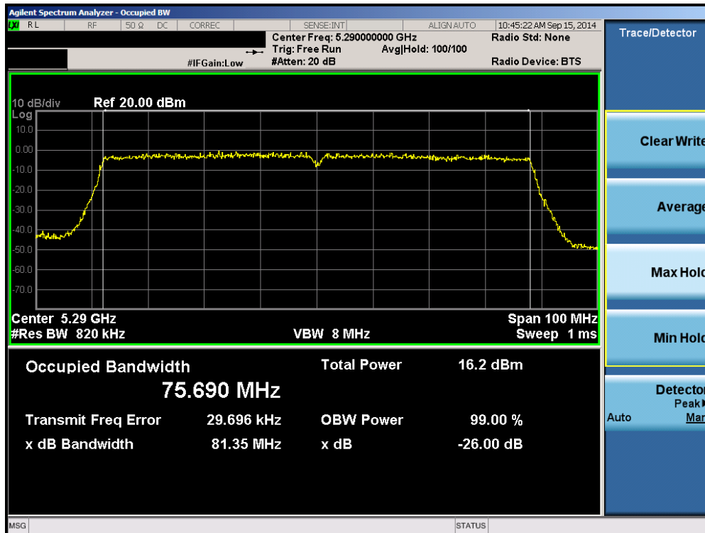
Plot 6-54. 26dB Bandwidth Plot (80MHz BW 802.11ac (UNII Band 2A) – Ch. 58)
