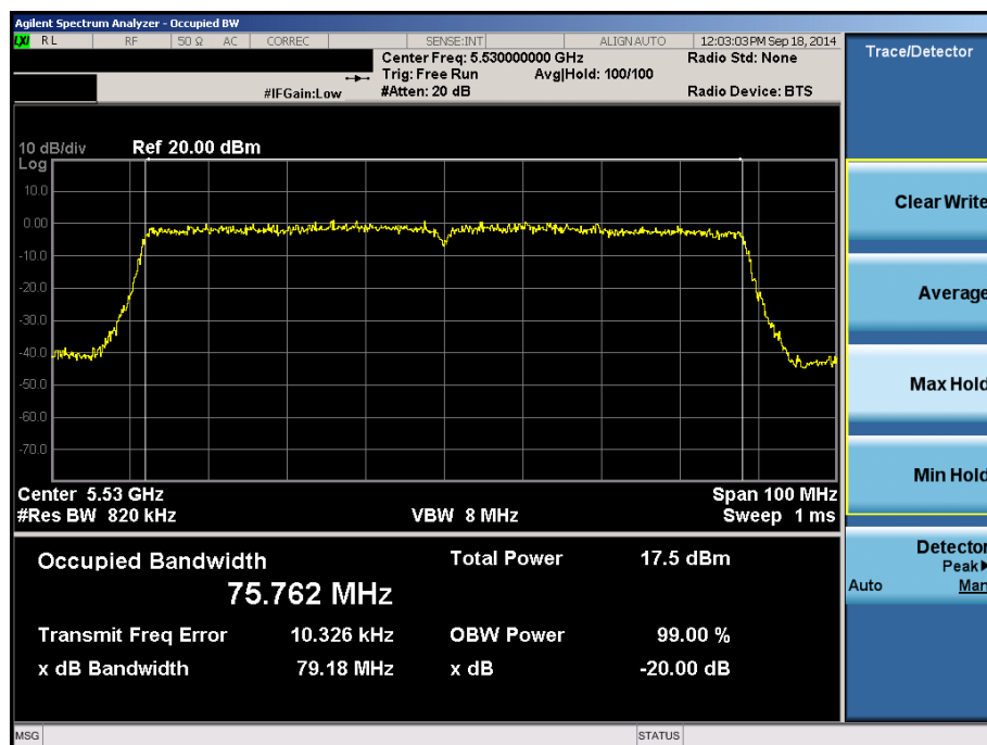
Plot 6-36. 20dB Bandwidth Plot (80MHz BW 802.11ac (UNII Band 2C) – Ch. 106
