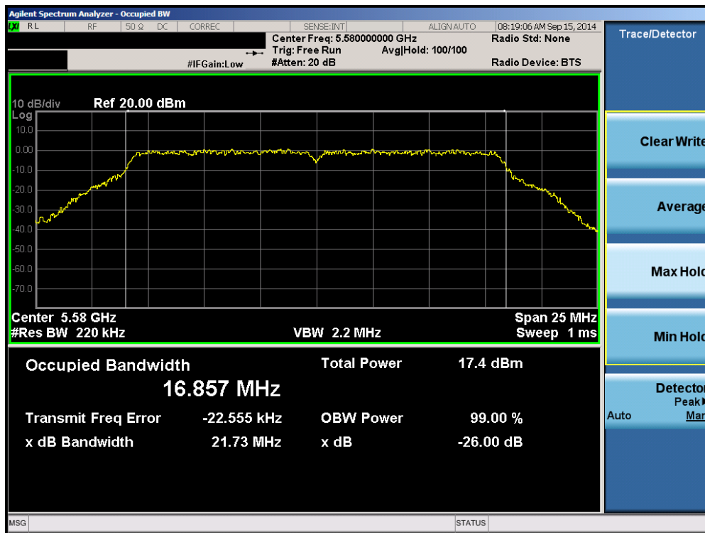
Plot 6-56. 26dB Bandwidth Plot (802.11a (UNII Band 2C) – Ch. 116)
