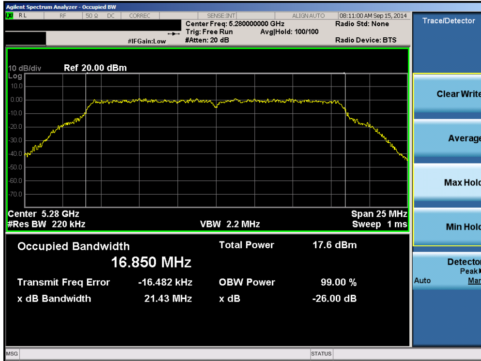
Plot 6-47. 26dB Bandwidth Plot (802.11a (UNII Band 2A) – Ch. 56)
