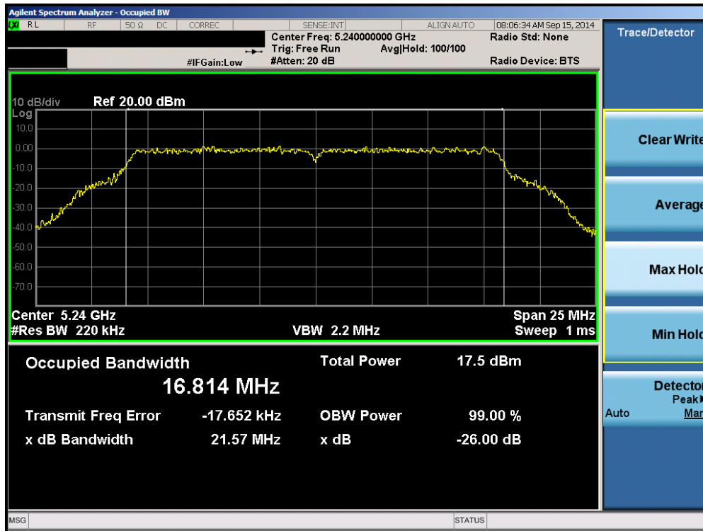
Plot 6-39. 26dB Bandwidth Plot (802.11a (UNII Band 1) – Ch. 48)
