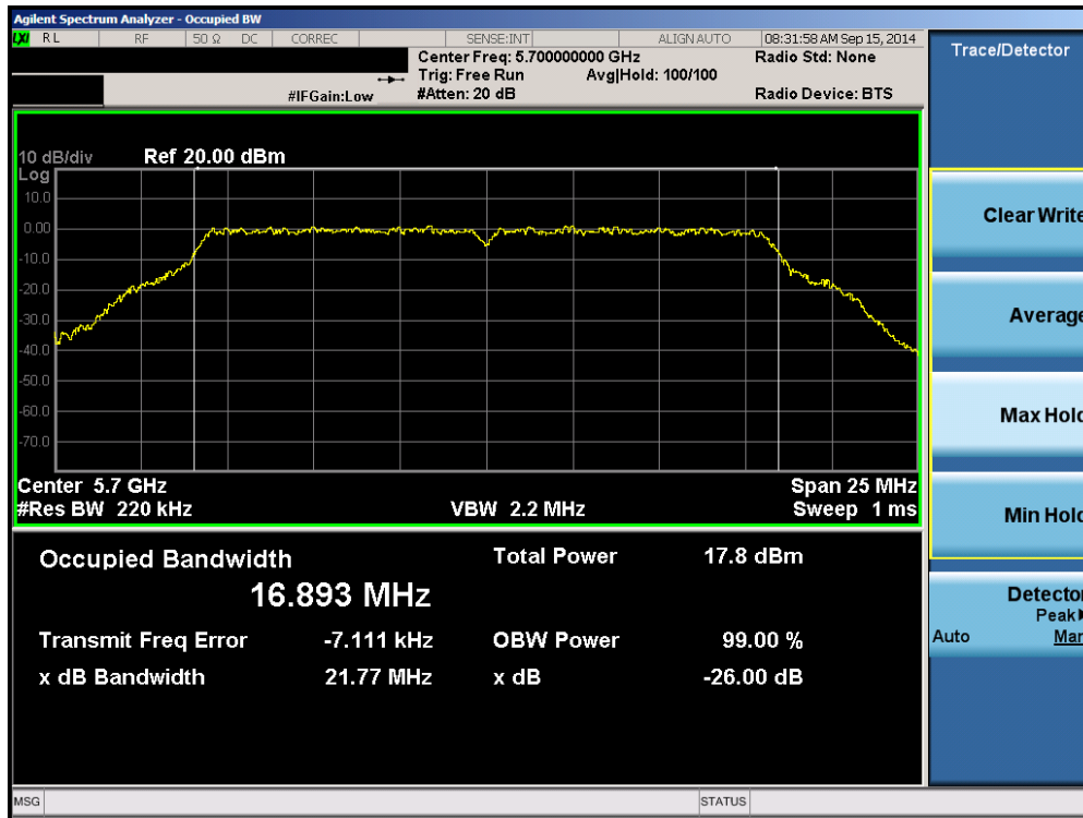
Plot 6-57. 26dB Bandwidth Plot (802.11a (UNII Band 2C) – Ch. 140)
