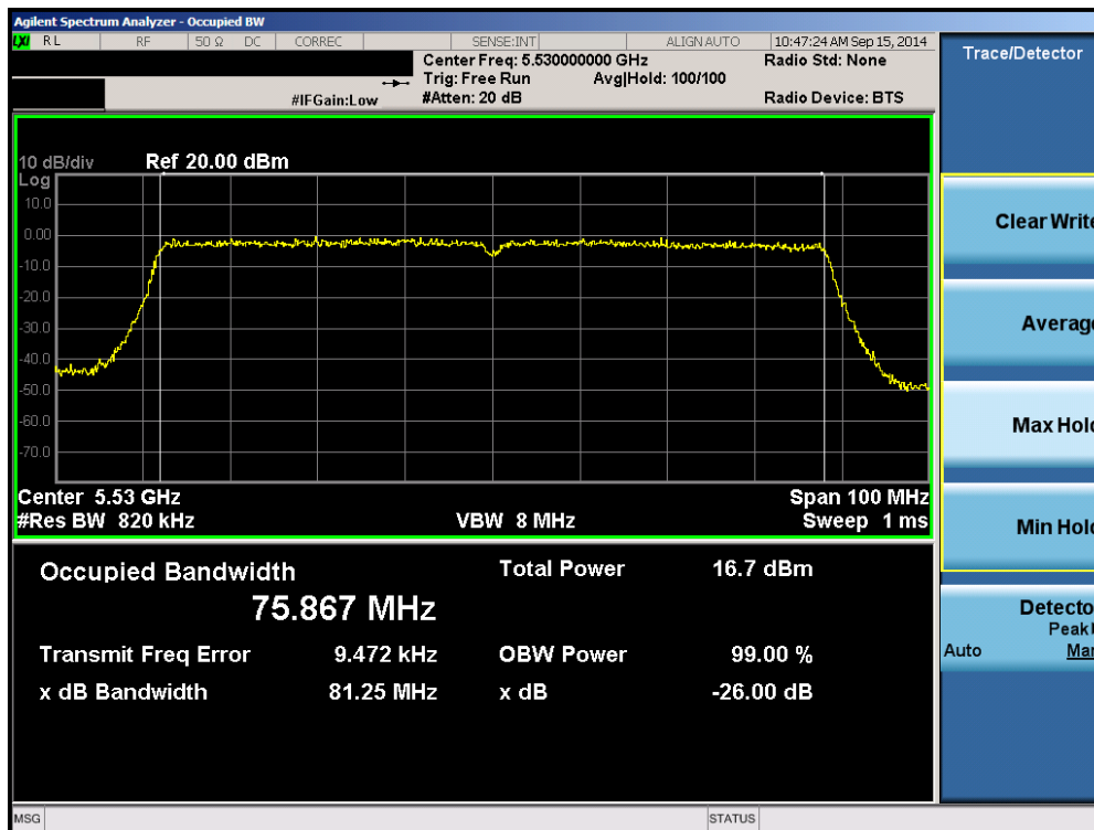
Plot 6-64. 26dB Bandwidth Plot (80MHz BW 802.11ac (UNII Band 2C) – Ch. 106)
