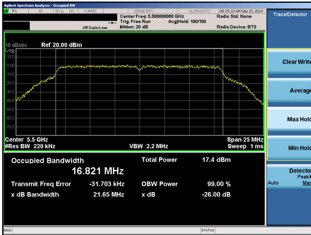
Plot 6-55. 26dB Bandwidth Plot (802.11a (UNII Band 2C) – Ch. 100)
