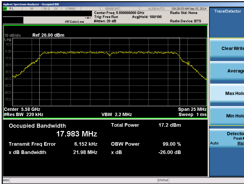
Plot 6-59. 26dB Bandwidth Plot (20MHz BW 802.11n (UNII Band 2C) – Ch. 116)
