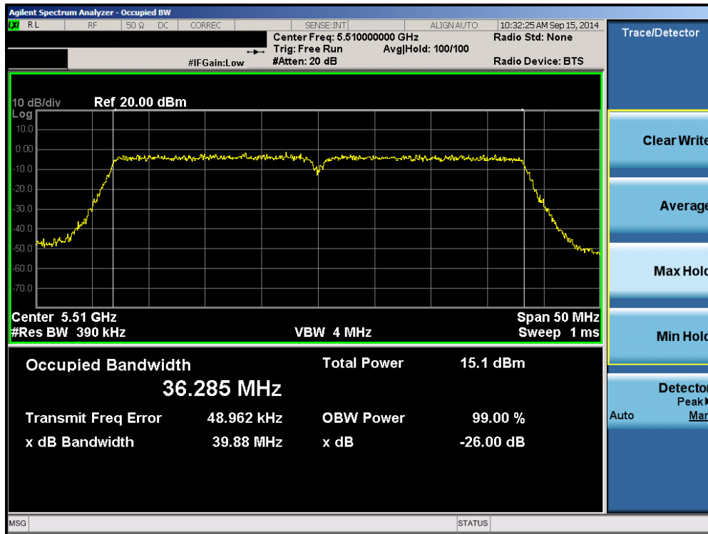
Plot 6-61. 26dB Bandwidth Plot (40MHz BW 802.11n (UNII Band 2C) – Ch. 102)
