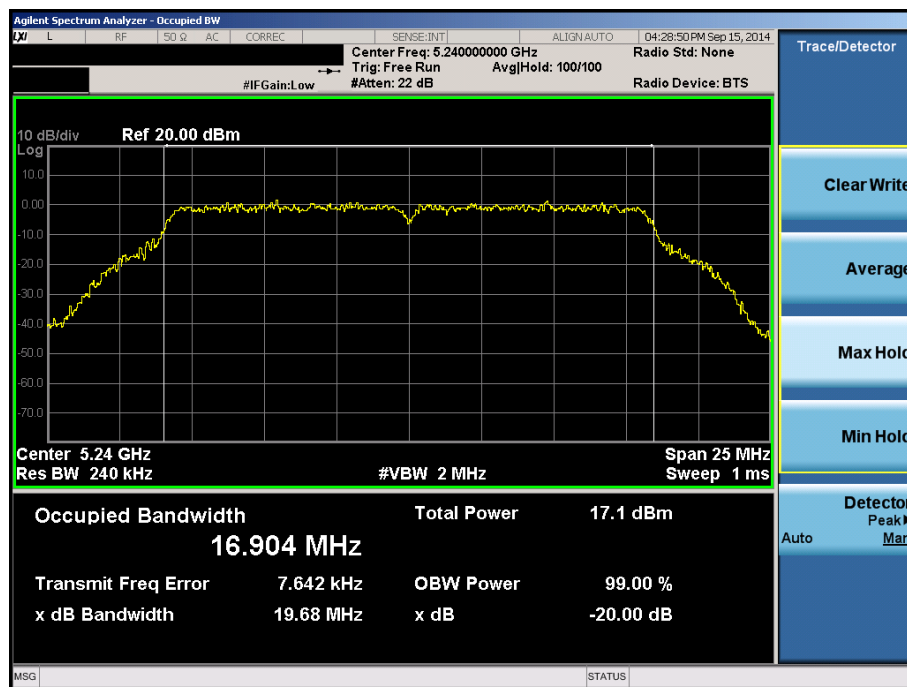
Plot 6-66. 20dB Bandwidth Plot (20MHz BW 802.11n (UNII Band 1) – Ch. 48)
