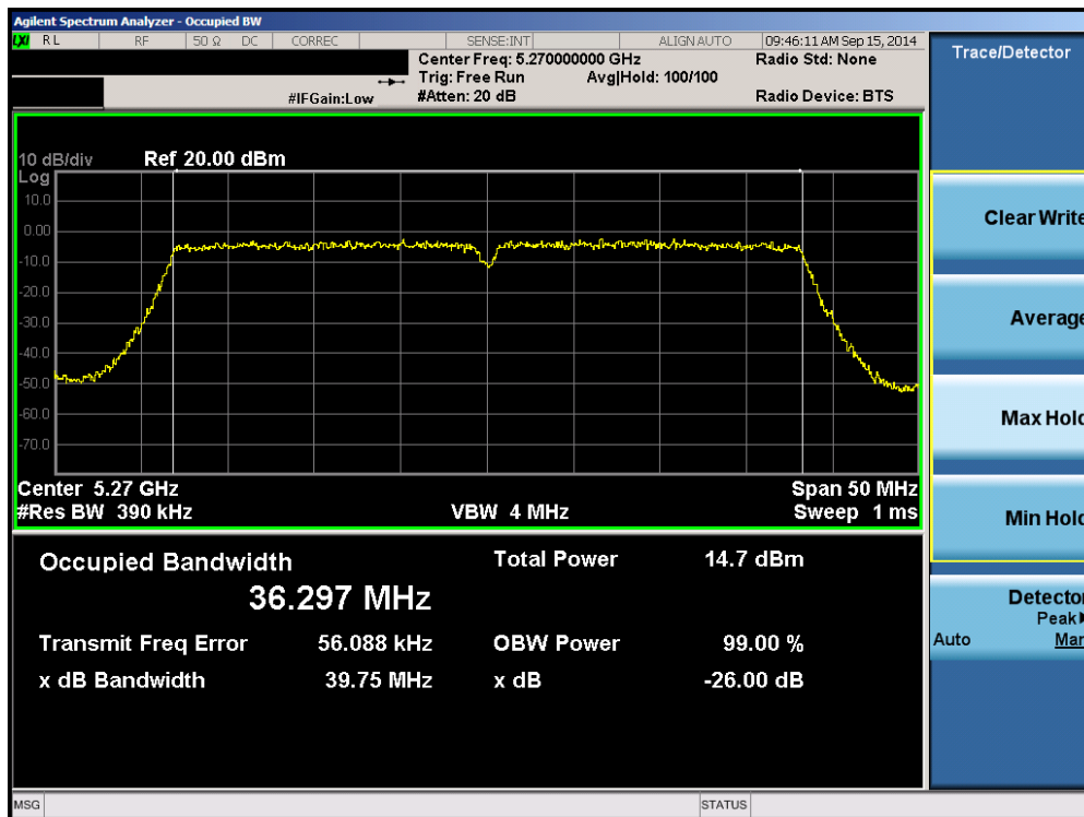
Plot 6-52. 26dB Bandwidth Plot (40MHz BW 802.11n (UNII Band 2A) – Ch. 54)
