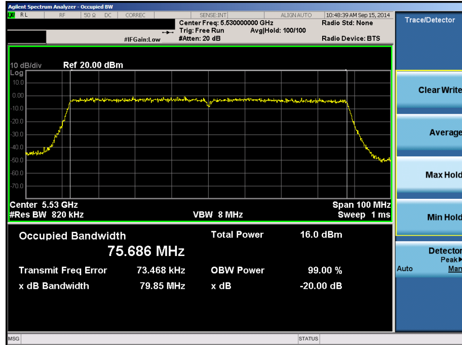
Plot 6-71. 20dB Bandwidth (80MHz BW 802.11ac (UNII Band 2C) – Ch. 106)
