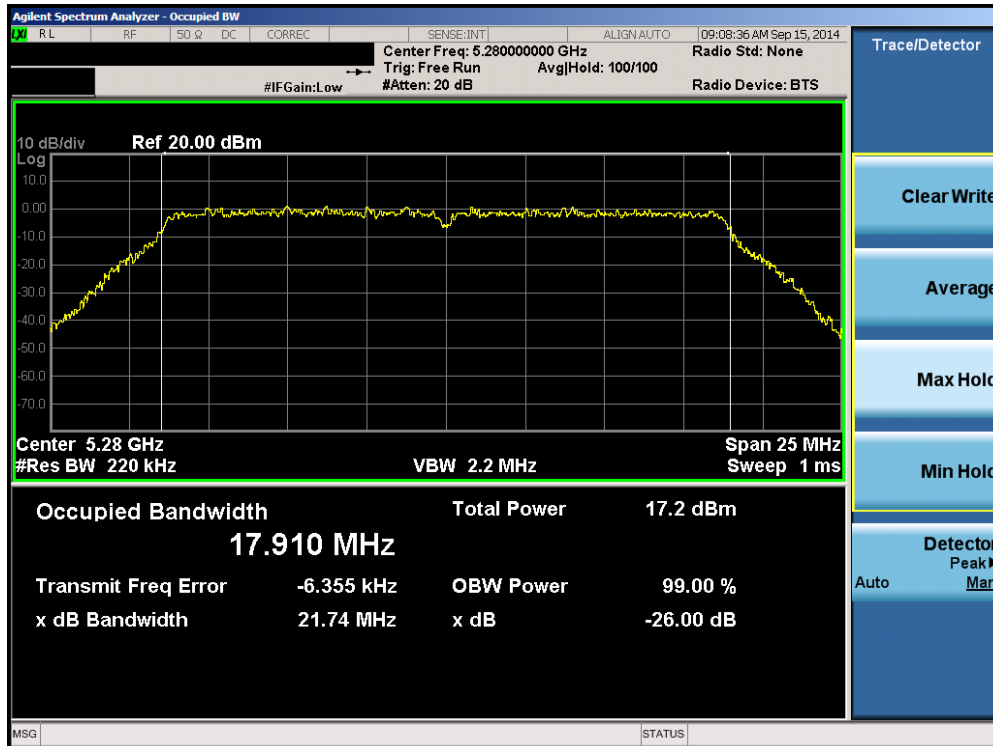
Plot 6-50. 26dB Bandwidth Plot (20MHz BW 802.11n (UNII Band 2A) – Ch. 56)
