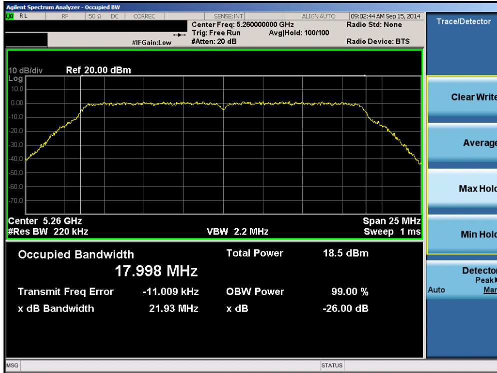
Plot 6-49. 26dB Bandwidth Plot (20MHz BW 802.11n (UNII Band 2A) – Ch. 52)
