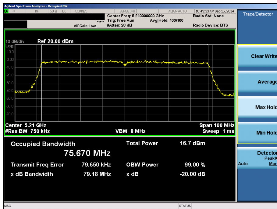
Plot 6-67. 20dB BW Plot (80MHz BW 802.11ac (UNII Band 1) – Ch. 42
