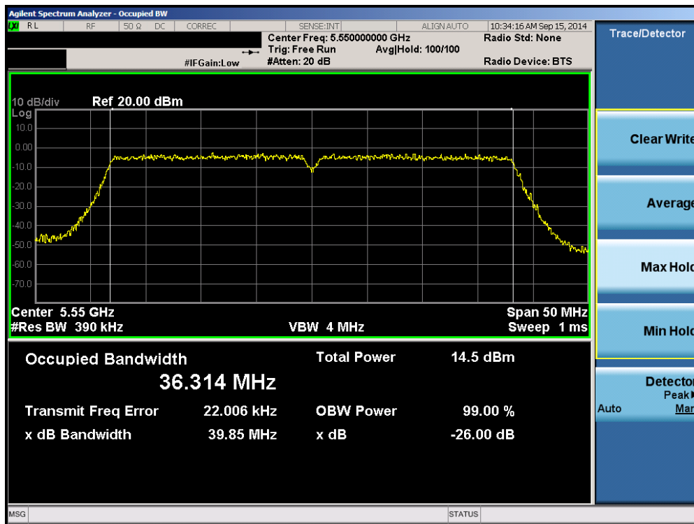
Plot 6-62. 26dB Bandwidth Plot (40MHz BW 802.11n (UNII Band 2C) – Ch. 110)
