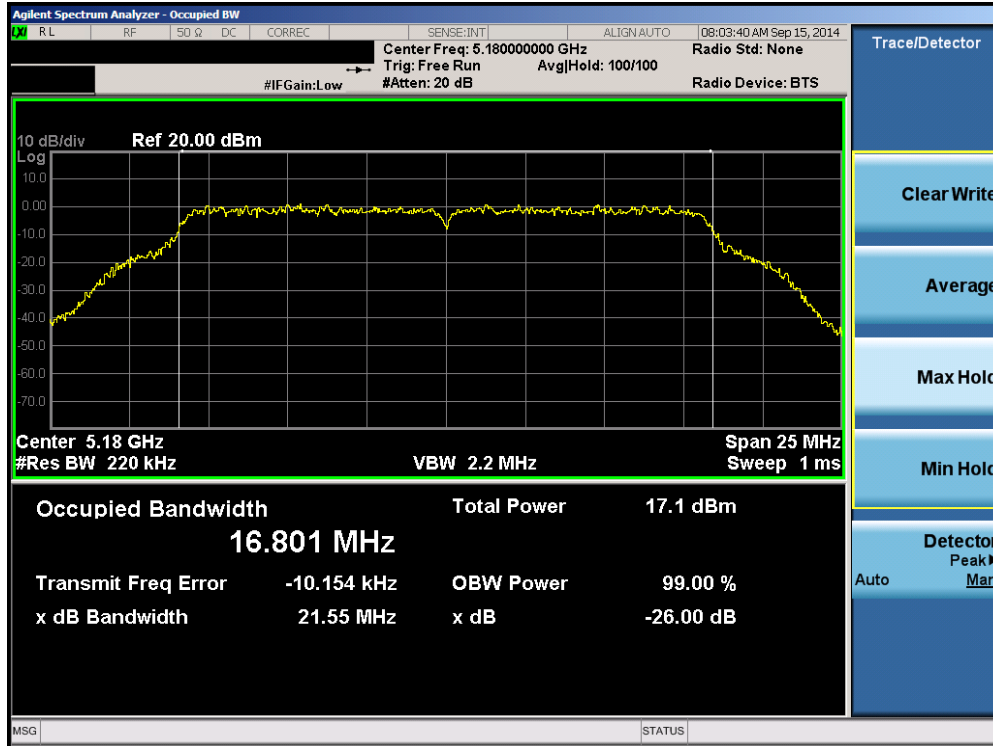
Plot 6-37. 26dB Bandwidth Plot (802.11a (UNII Band 1) – Ch. 36)
