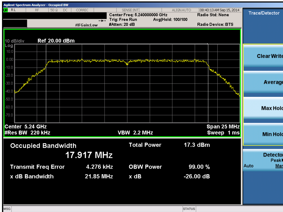
Plot 6-42. 26dB Bandwidth Plot (20MHz BW 802.11n (UNII Band 1) – Ch. 48)
