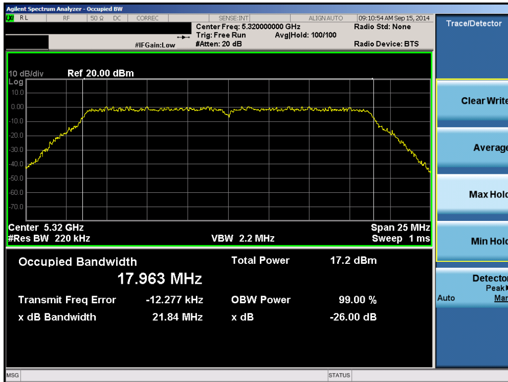
Plot 6-51. 26dB Bandwidth Plot (20MHz BW 802.11n (UNII Band 2A) – Ch. 64)
