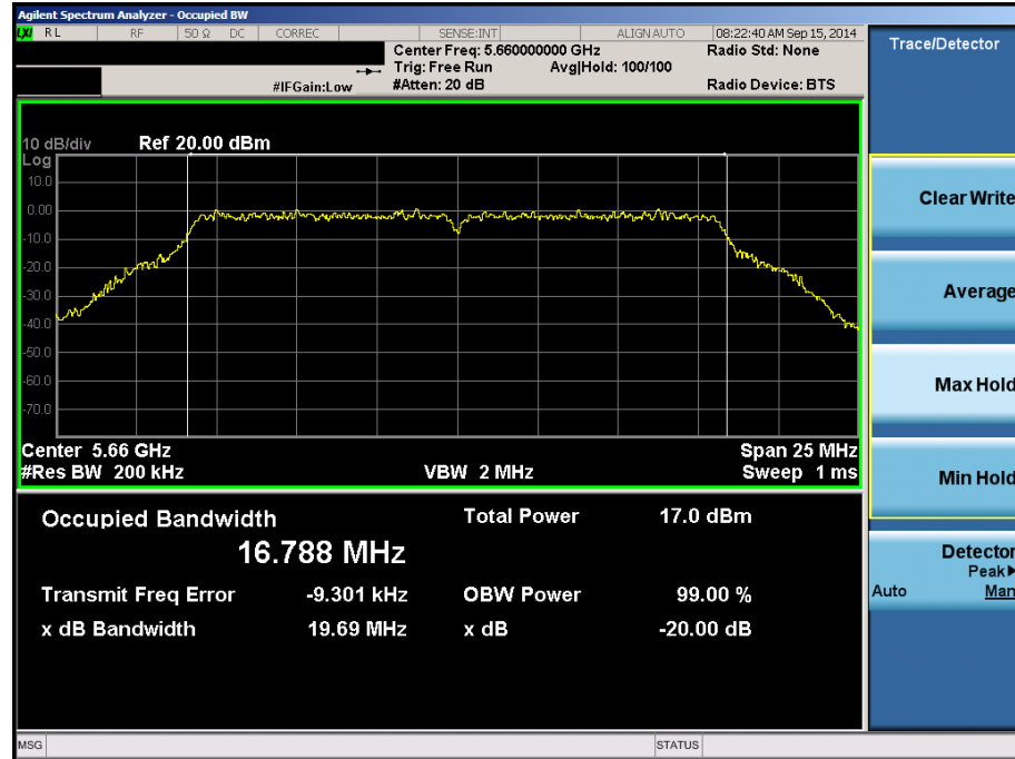
Plot 6-69. 20dB Bandwidth (20MHz BW 802.11a (UNII Band 2C) – Ch. 132)
