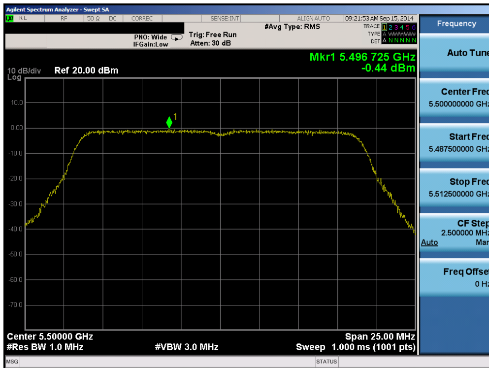
Plot 6-121. Peak Power Spectral Density Plot (20MHz BW 802.11n (UNII Band 2C) – Ch. 100)
