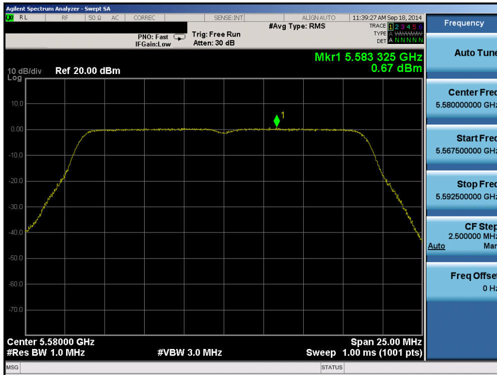
Plot 6-94. Peak Power Spectral Density Plot (20MHz BW 802.11n (UNII Band 2C) – Ch. 116)
