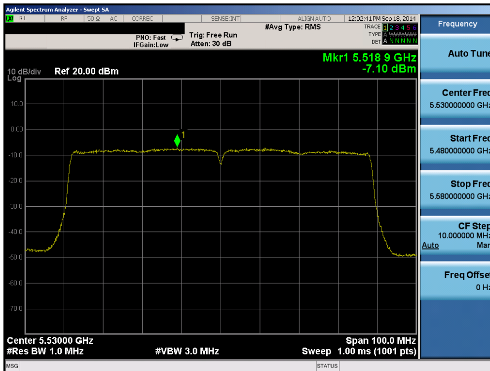
Plot 6-99. Peak Power Spectral Density Plot (80MHz BW 802.11ac (UNII Band 2C) – Ch. 106)
