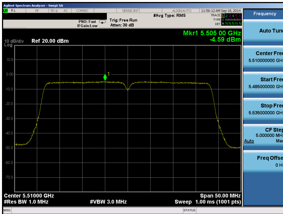
Plot 6-96. Peak Power Spectral Density Plot (40MHz BW 802.11n (UNII Band 2C) – Ch. 102)
