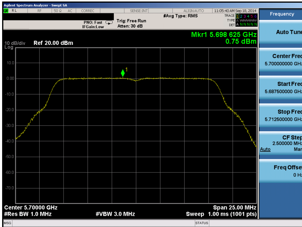
Plot 6-92. Peak Power Spectral Density Plot (802.11a (UNII Band 2C) – Ch. 140)
