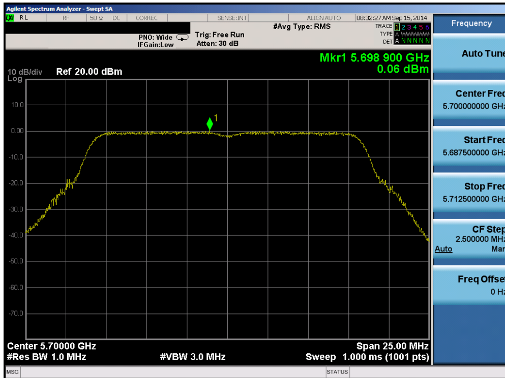
Plot 6-120. Peak Power Spectral Density Plot (802.11a (UNII Band 2C) – Ch. 140)
