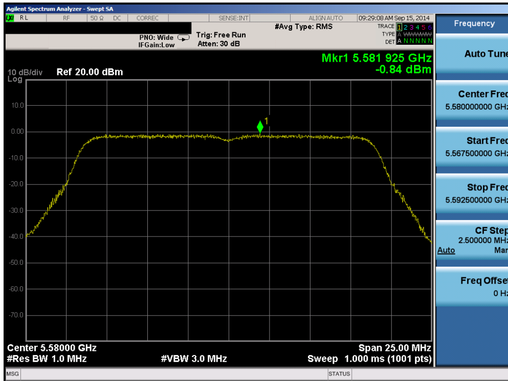
Plot 6-122. Peak Power Spectral Density Plot (20MHz BW 802.11n (UNII Band 2C) – Ch. 116)
