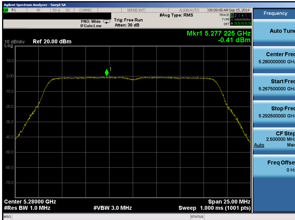
Plot 6-113. Peak Power Spectral Density Plot (20MHz BW 802.11n (UNII Band 2A) – Ch. 56)
