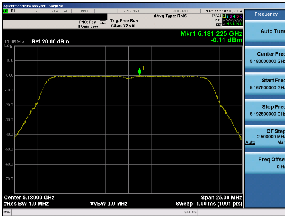
Plot 6-75. Peak Power Spectral Density Plot (20MHz BW 802.11n (UNII Band 1) – Ch. 36)
