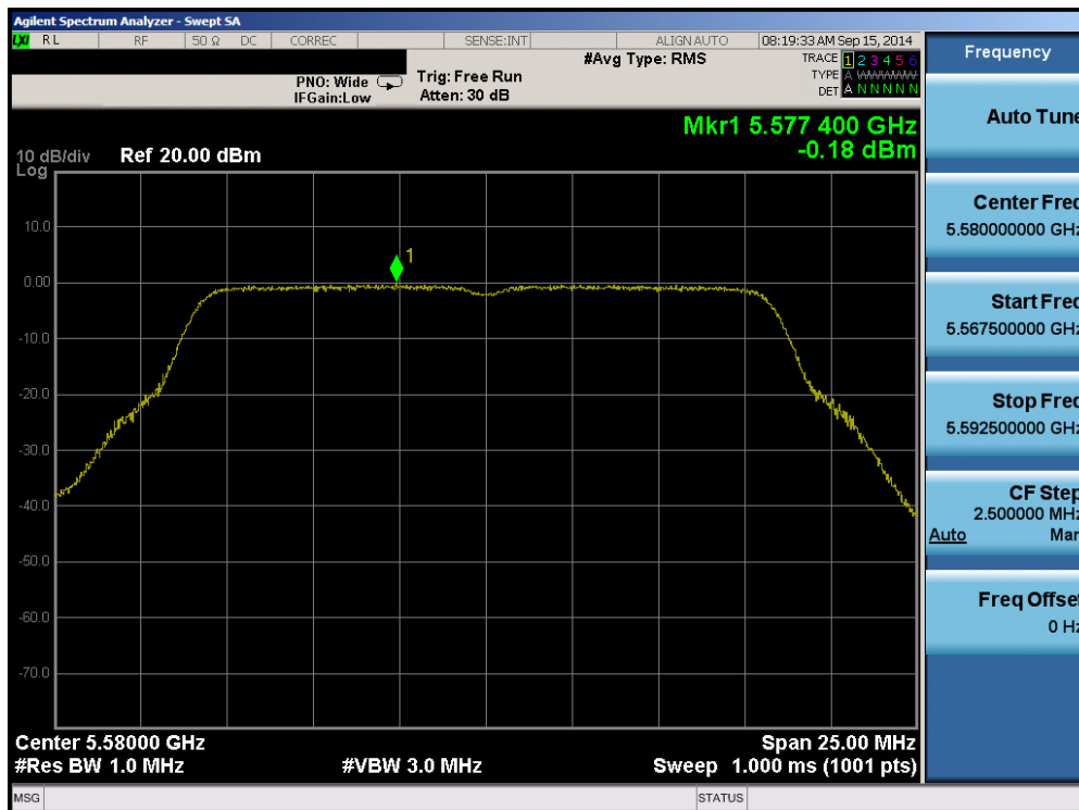
Plot 6-119. Peak Power Spectral Density Plot (802.11a (UNII Band 2C) – Ch. 116)
