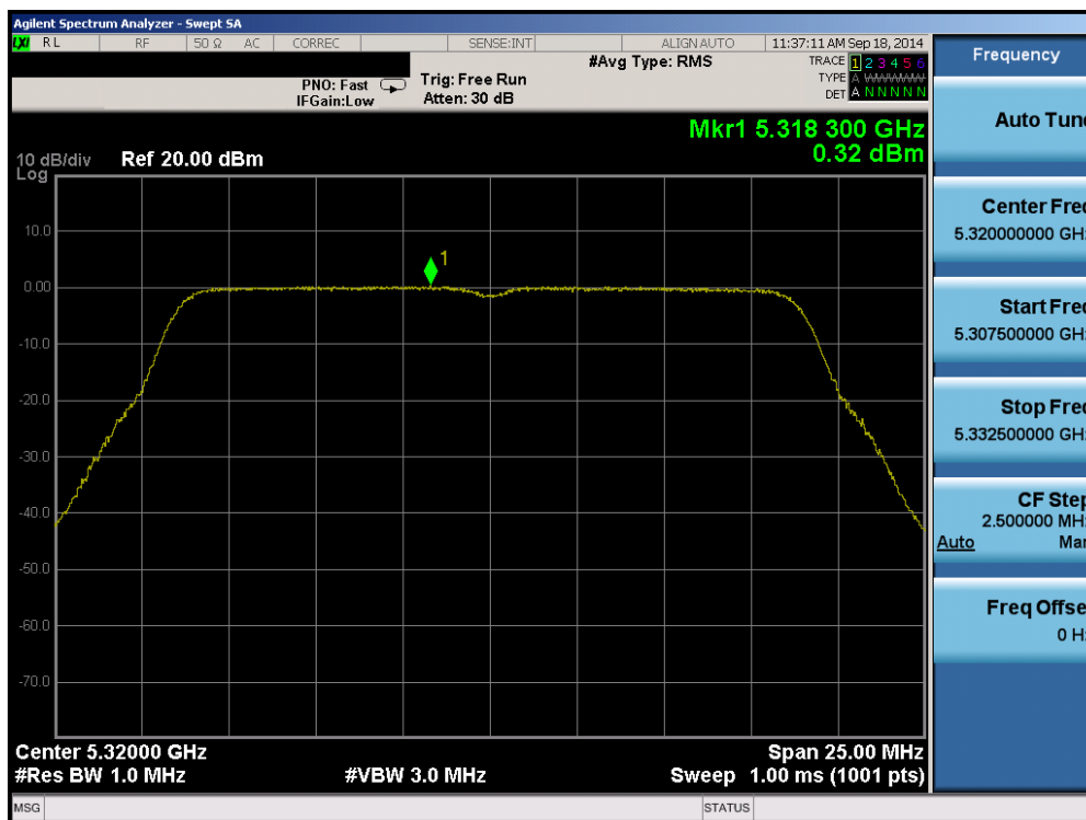
Plot 6-86. Peak Power Spectral Density Plot (20MHz BW 802.11n (UNII Band 2A) – Ch. 64)
