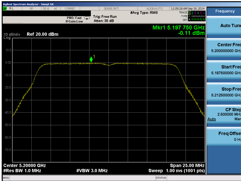
Plot 6-76. Peak Power Spectral Density Plot (20MHz BW 802.11n (UNII Band 1) – Ch. 40)
