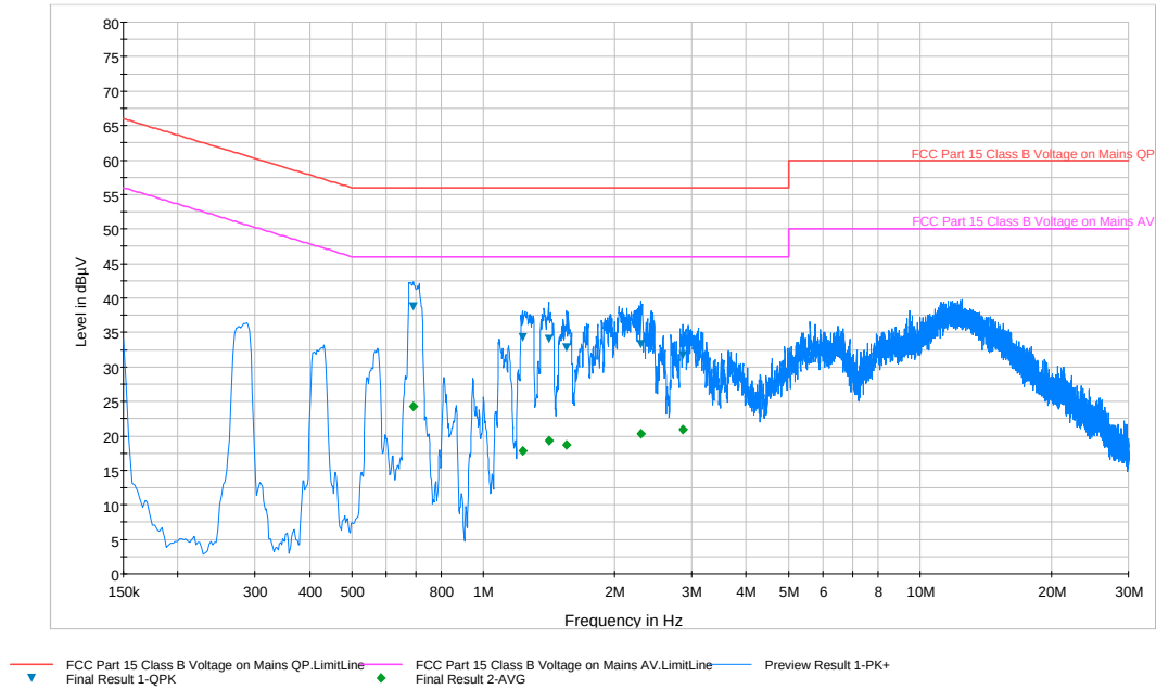
Plot 6-198. Line Conducted Plot with 802.11a UNII Band 2A (L1)
