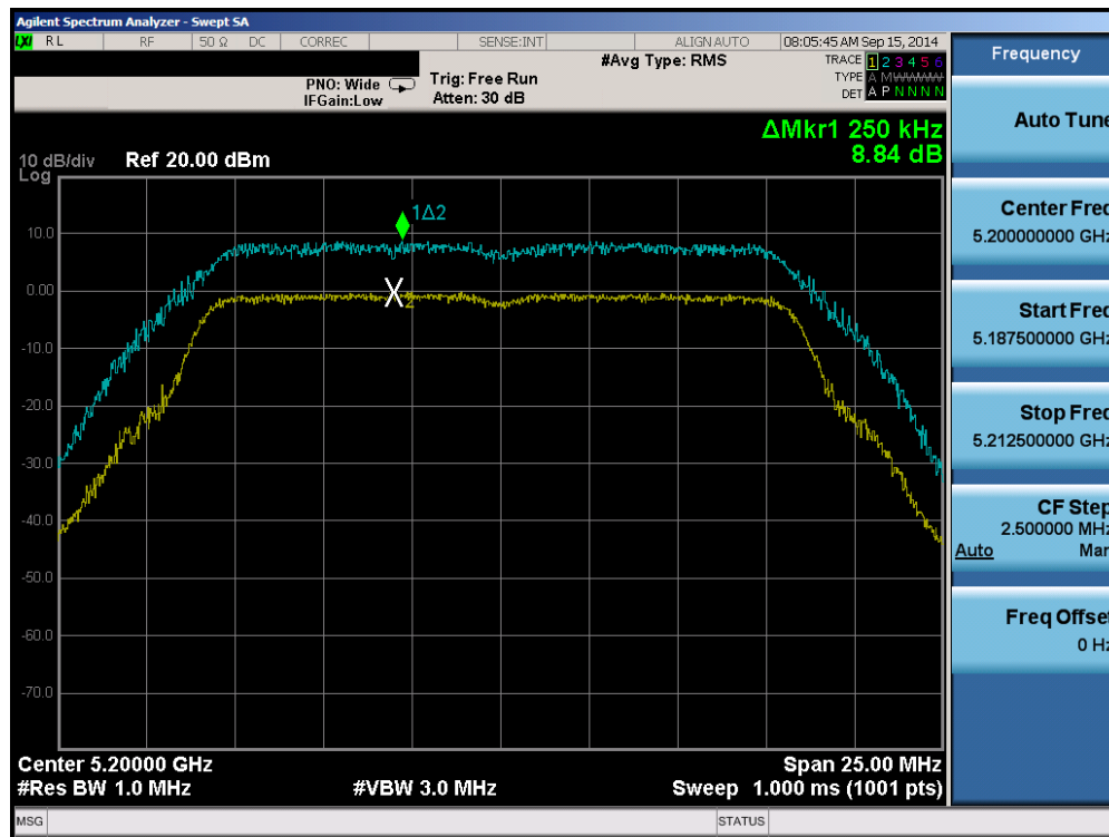
Plot 6-132. Peak Excursion Ratio Plot (802.11a (UNII Band 1) – Ch. 40)
