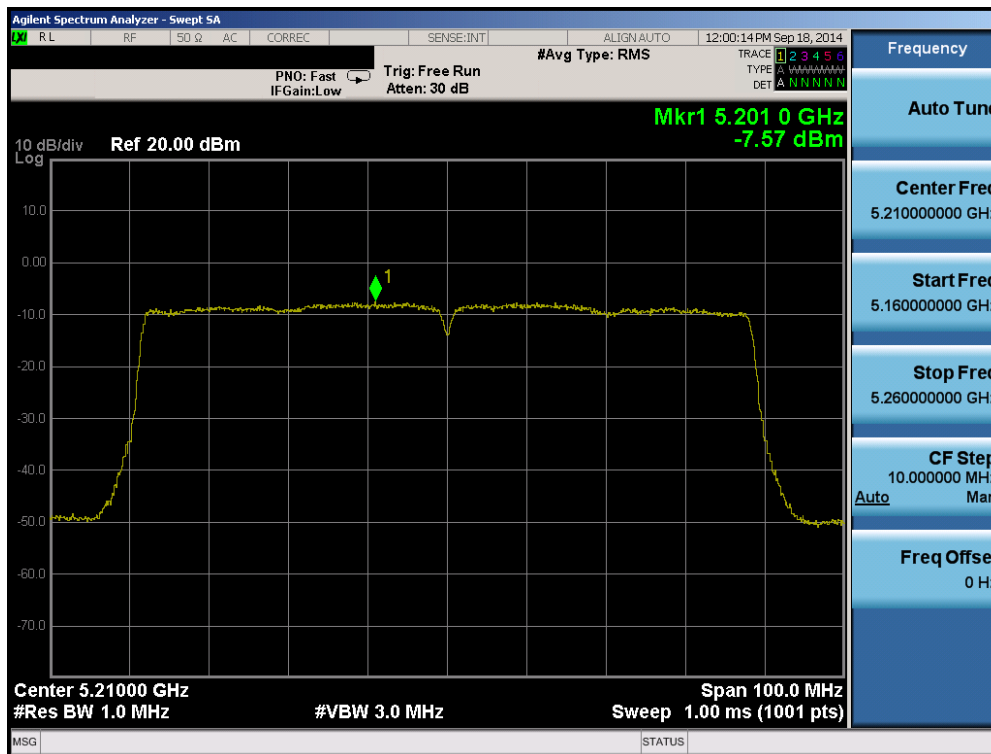
Plot 6-80. Peak Power Spectral Density Plot (80MHz BW 802.11ac (UNII Band 1) – Ch. 42)
