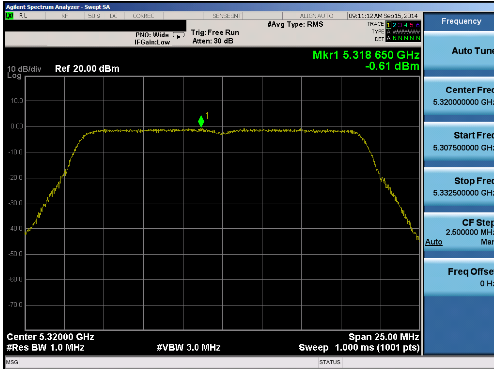
Plot 6-114. Peak Power Spectral Density Plot (20MHz BW 802.11n (UNII Band 2A) – Ch. 64)
