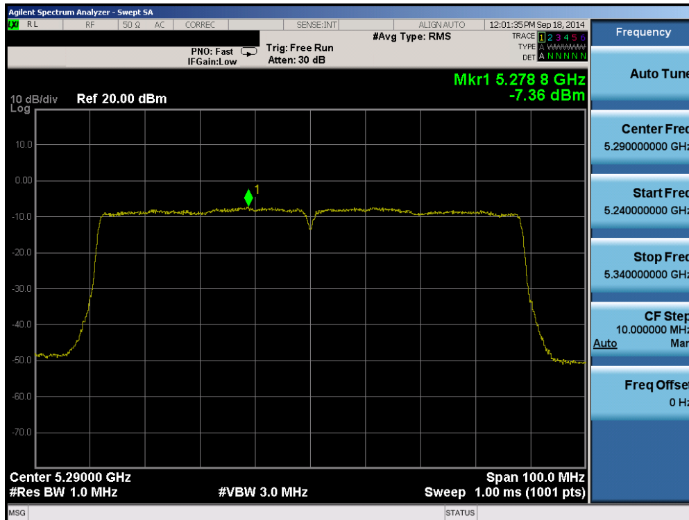
Plot 6-89. Peak Power Spectral Density Plot (80MHz BW 802.11ac (UNII Band 2A) – Ch. 58)
