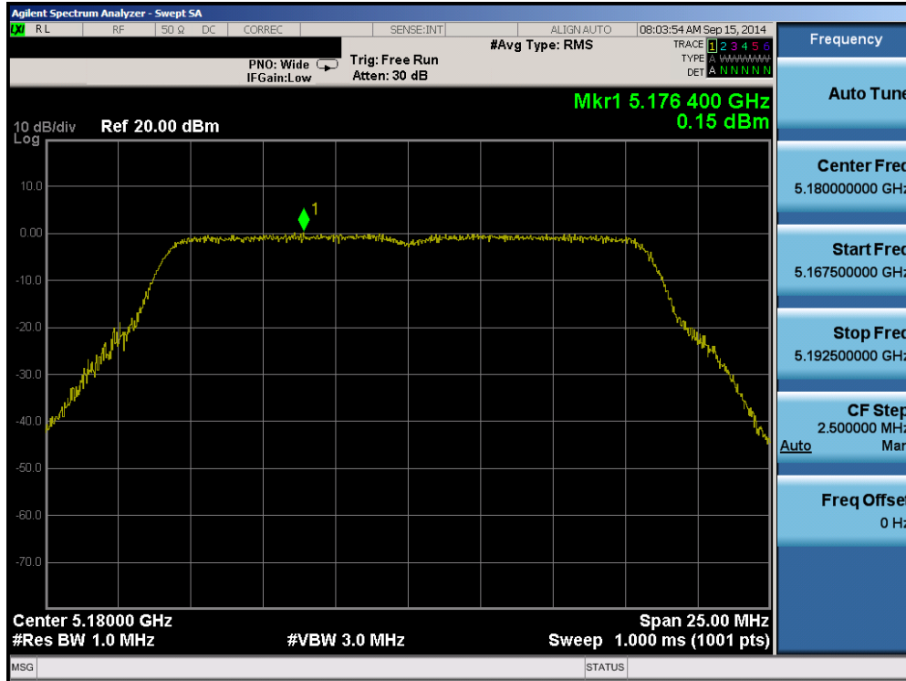
Plot 6-100. Peak Power Spectral Density Plot (802.11a (UNII Band 1) – Ch. 36)
