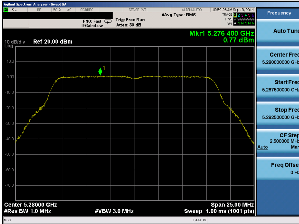
Plot 6-82. Peak Power Spectral Density Plot (802.11a (UNII Band 2A) – Ch. 56)
