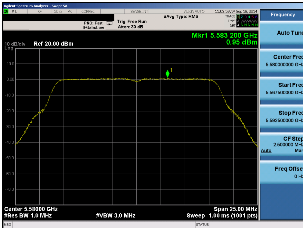
Plot 6-91. Peak Power Spectral Density Plot (802.11a (UNII Band 2C) – Ch. 116)
