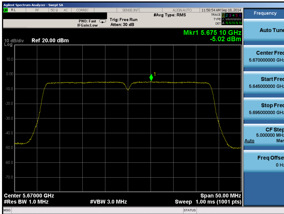
Plot 6-98. Peak Power Spectral Density Plot (40MHz BW 802.11n (UNII Band 2C) – Ch. 134)
