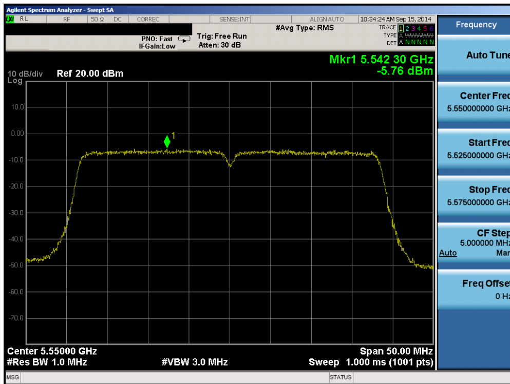
Plot 6-125. Peak Power Spectral Density Plot (40MHz BW 802.11n (UNII Band 2C) – Ch. 110)
