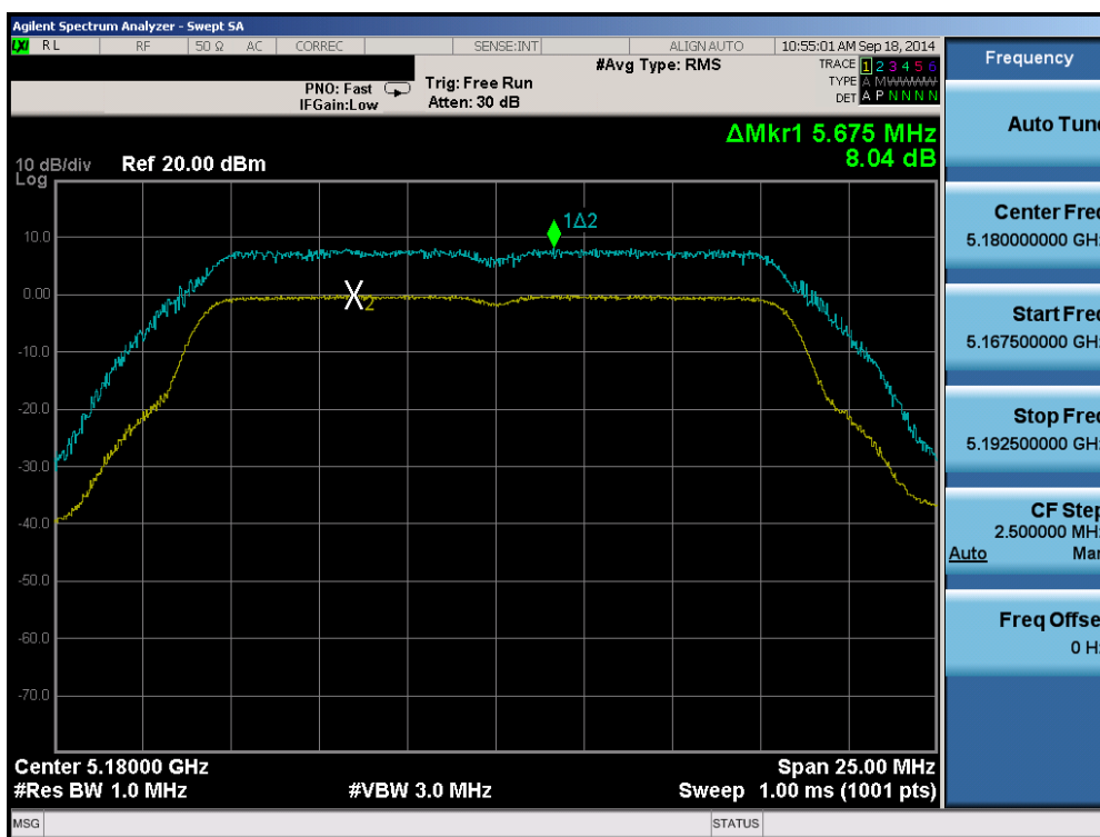
Plot 6-128. Peak Excursion Ratio Plot (802.11a (UNII Band 1) – Ch. 36)
