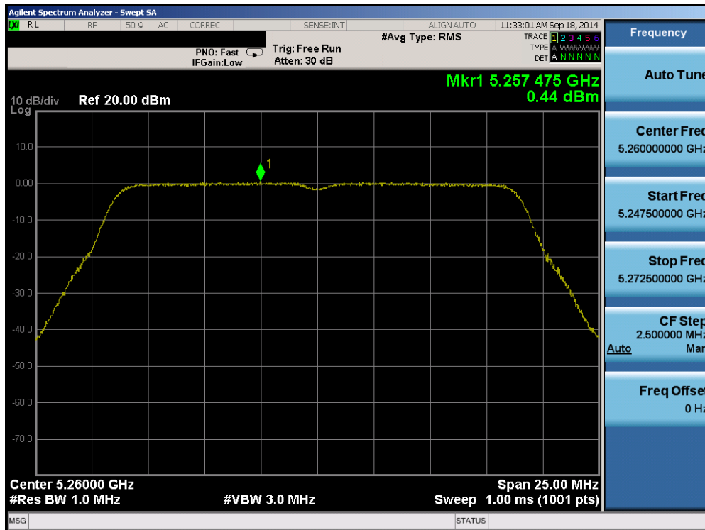
Plot 6-84. Peak Power Spectral Density Plot (20MHz BW 802.11n (UNII Band 2A) – Ch. 52)
