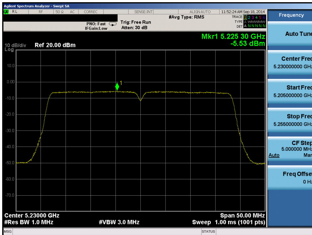
Plot 6-79. Peak Power Spectral Density Plot (40MHz BW 802.11n (UNII Band 1) – Ch. 46)
