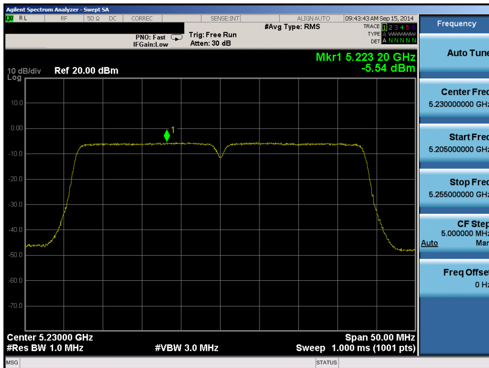
Plot 6-107. Peak Power Spectral Density Plot (40MHz BW 802.11n (UNII Band 1) – Ch. 46)
