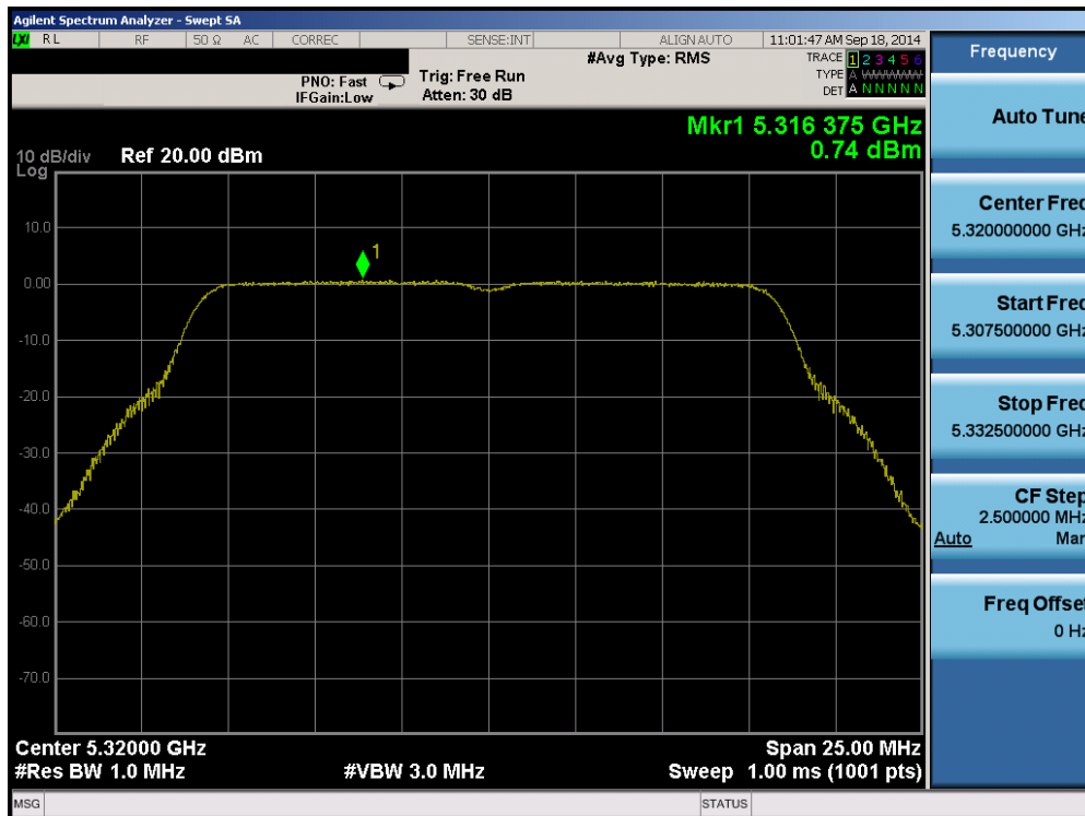
Plot 6-83. Peak Power Spectral Density Plot (802.11a (UNII Band 2A) – Ch. 64)
