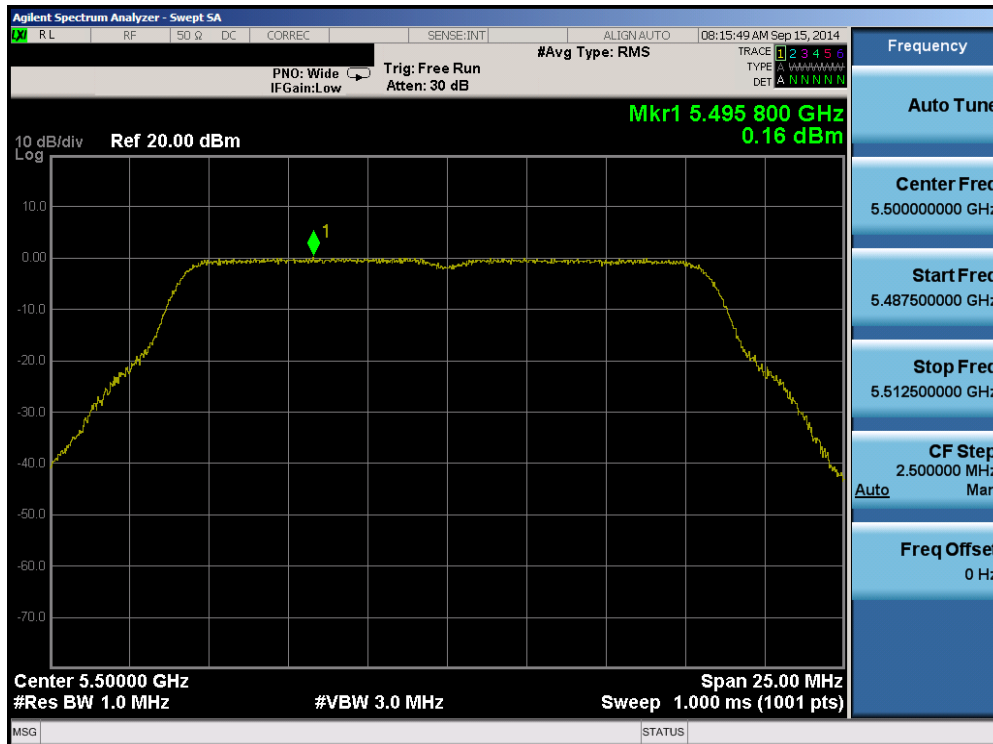
Plot 6-118. Peak Power Spectral Density Plot (802.11a (UNII Band 2C) – Ch. 100)
