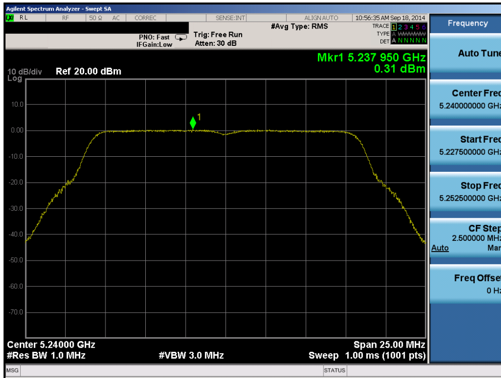
Plot 6-74. Peak Power Spectral Density Plot (802.11a (UNII Band 1) – Ch. 48)
