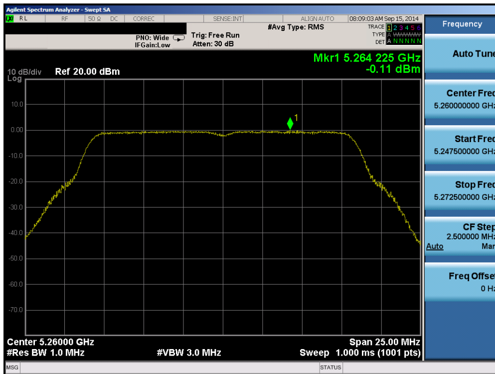
Plot 6-109. Peak Power Spectral Density Plot (802.11a (UNII Band 2A) – Ch. 52)
