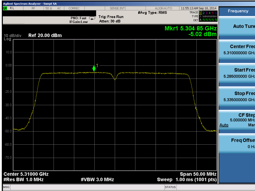
Plot 6-88. Peak Power Spectral Density Plot (40MHz BW 802.11n (UNII Band 2A) – Ch. 62)
