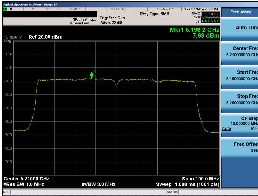
Plot 6-108. Peak Power Spectral Density Plot (80MHz BW 802.11ac (UNII Band 1) – Ch. 42)
