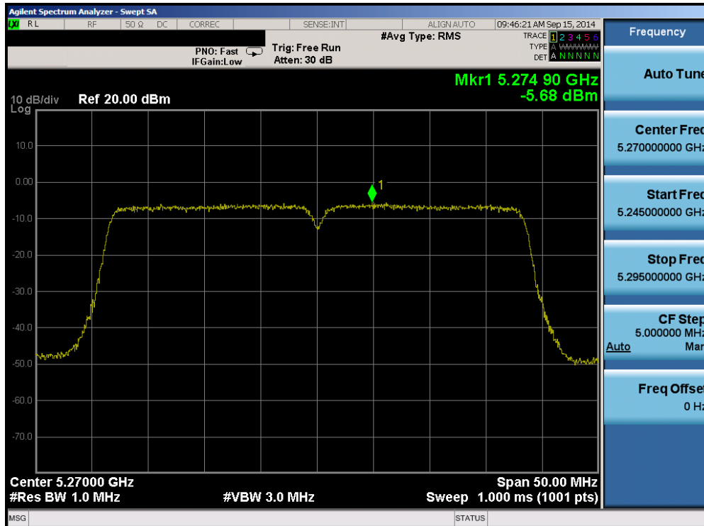
Plot 6-115. Peak Power Spectral Density Plot (40MHz BW 802.11n (UNII Band 2A) – Ch. 54)
