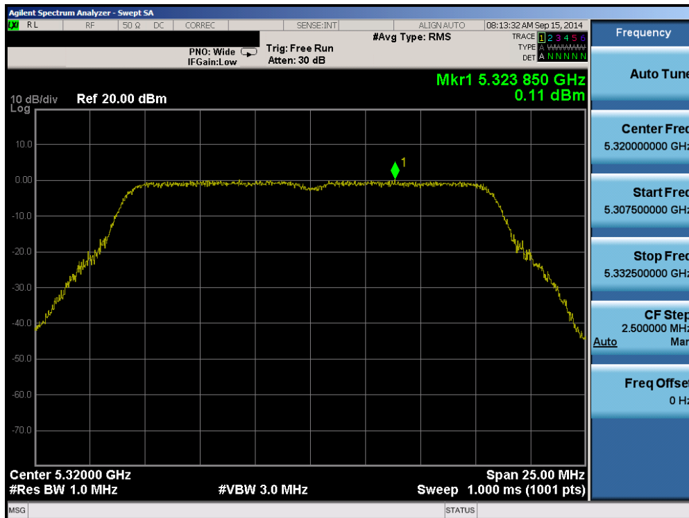
Plot 6-111. Peak Power Spectral Density Plot (802.11a (UNII Band 2A) – Ch. 64)
