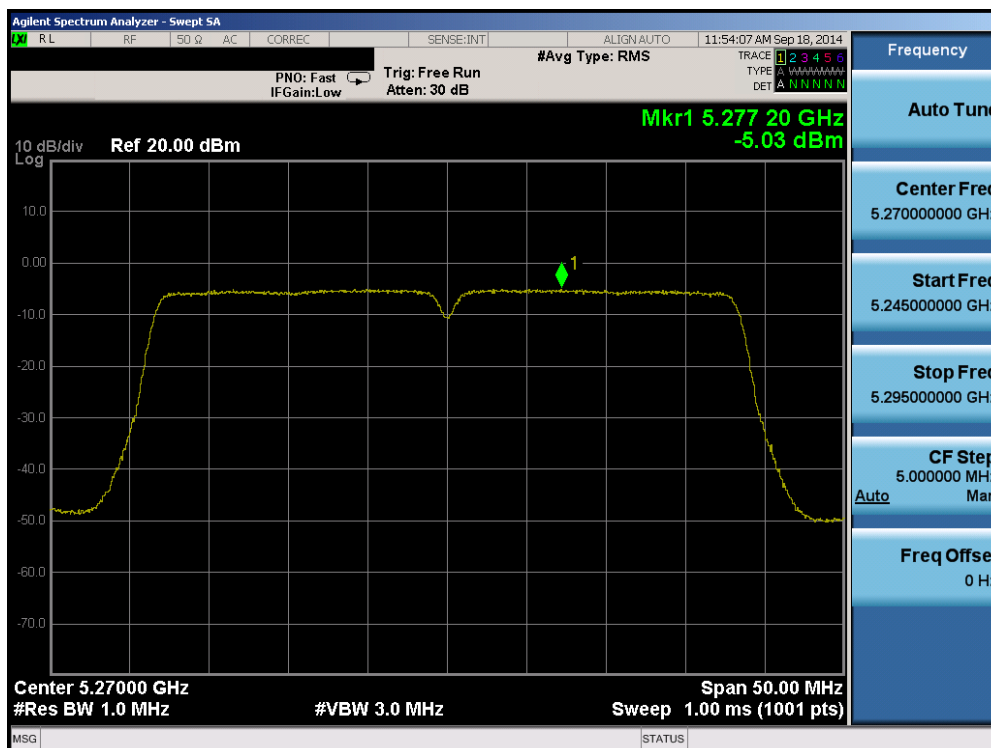
Plot 6-87. Peak Power Spectral Density Plot (40MHz BW 802.11n (UNII Band 2A) – Ch. 54)
