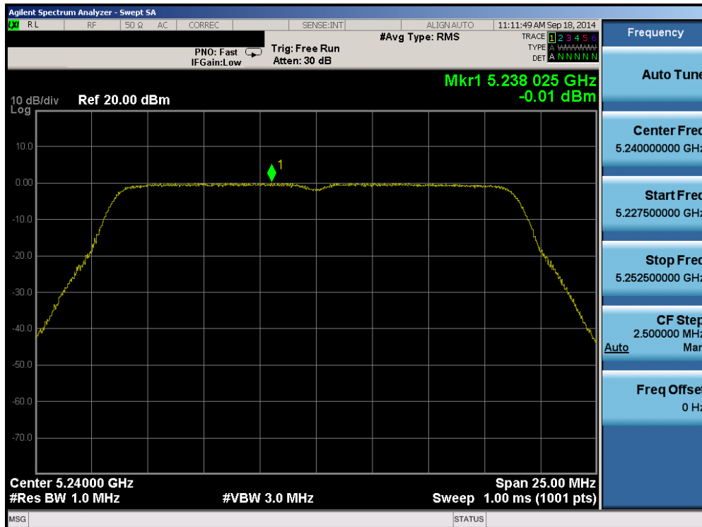
Plot 6-77. Peak Power Spectral Density Plot (20MHz BW 802.11n (UNII Band 1) – Ch. 48)
