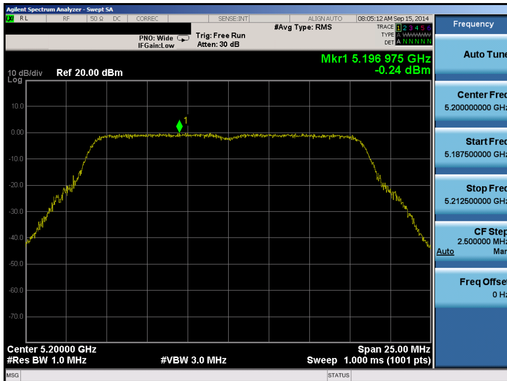
Plot 6-101. Peak Power Spectral Density Plot (802.11a (UNII Band 1) – Ch. 40)
