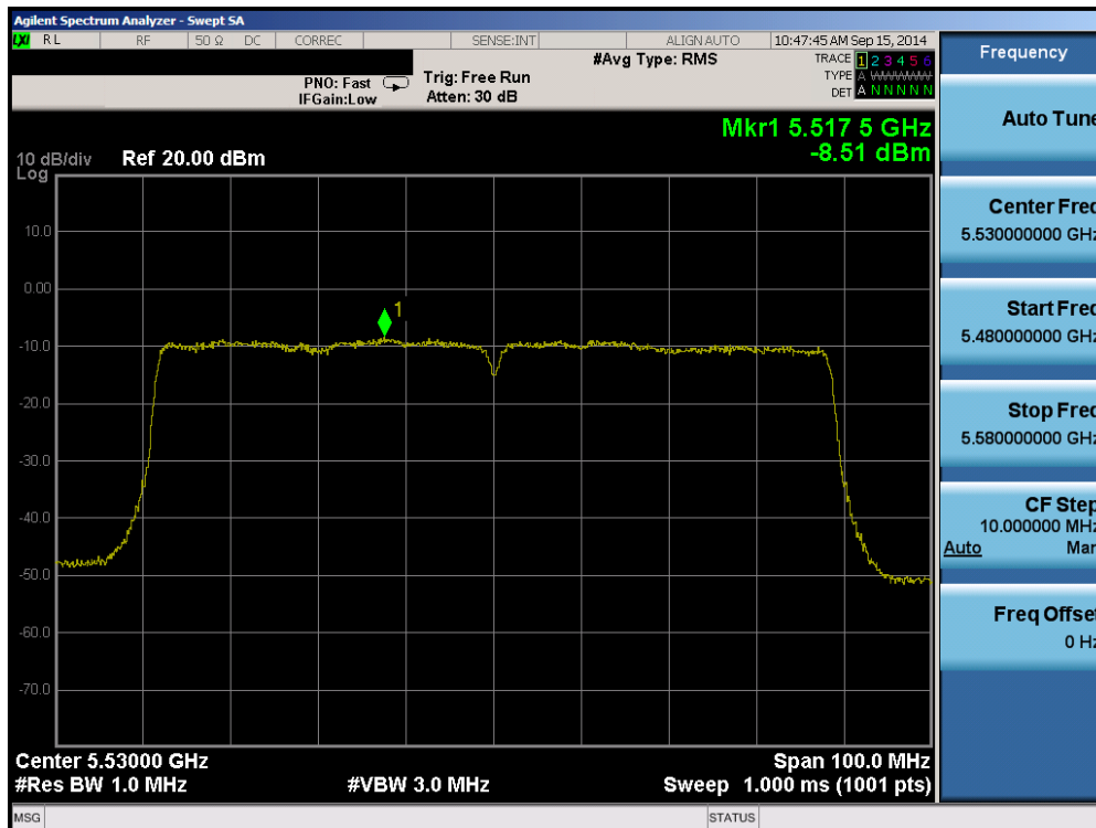
Plot 6-127. Peak Power Spectral Density Plot (80MHz BW 802.11ac (UNII Band 2C) – Ch. 106)
