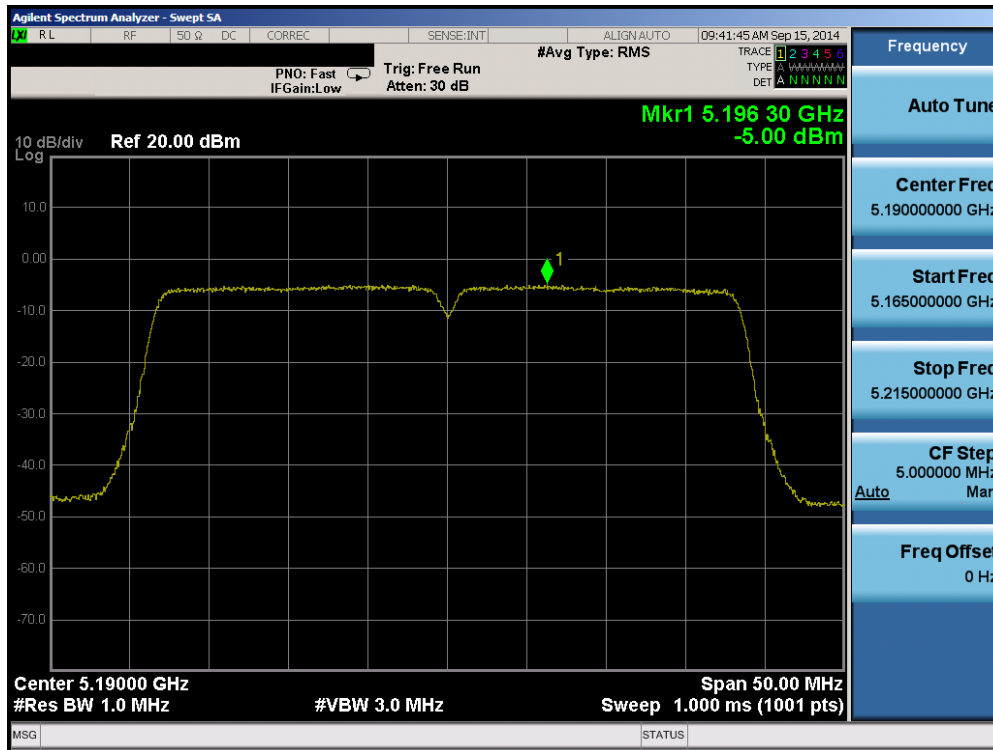
Plot 6-106. Peak Power Spectral Density Plot (40MHz BW 802.11n (UNII Band 1) – Ch. 38)
