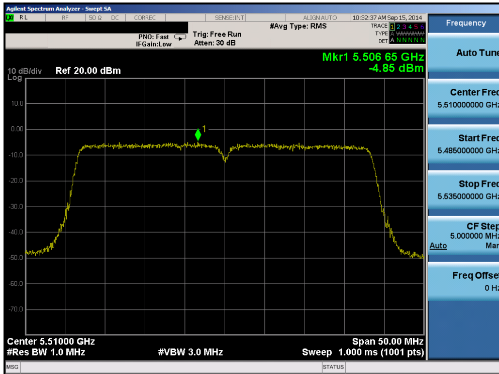
Plot 6-124. Peak Power Spectral Density Plot (40MHz BW 802.11n (UNII Band 2C) – Ch. 102)
