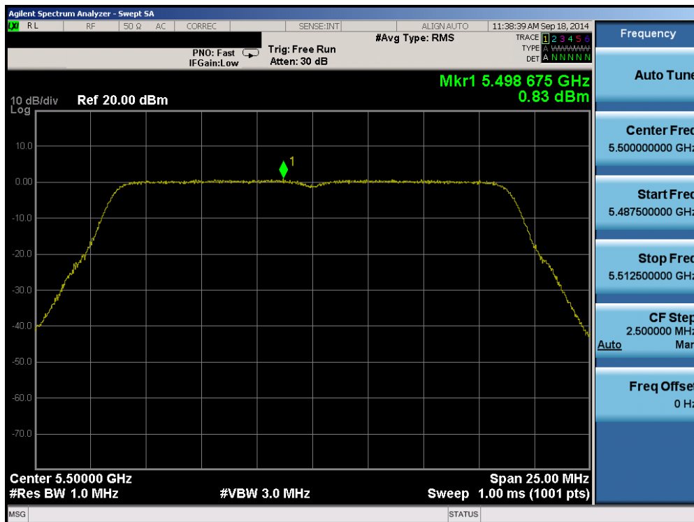
Plot 6-93. Peak Power Spectral Density Plot (20MHz BW 802.11n (UNII Band 2C) – Ch. 100)
