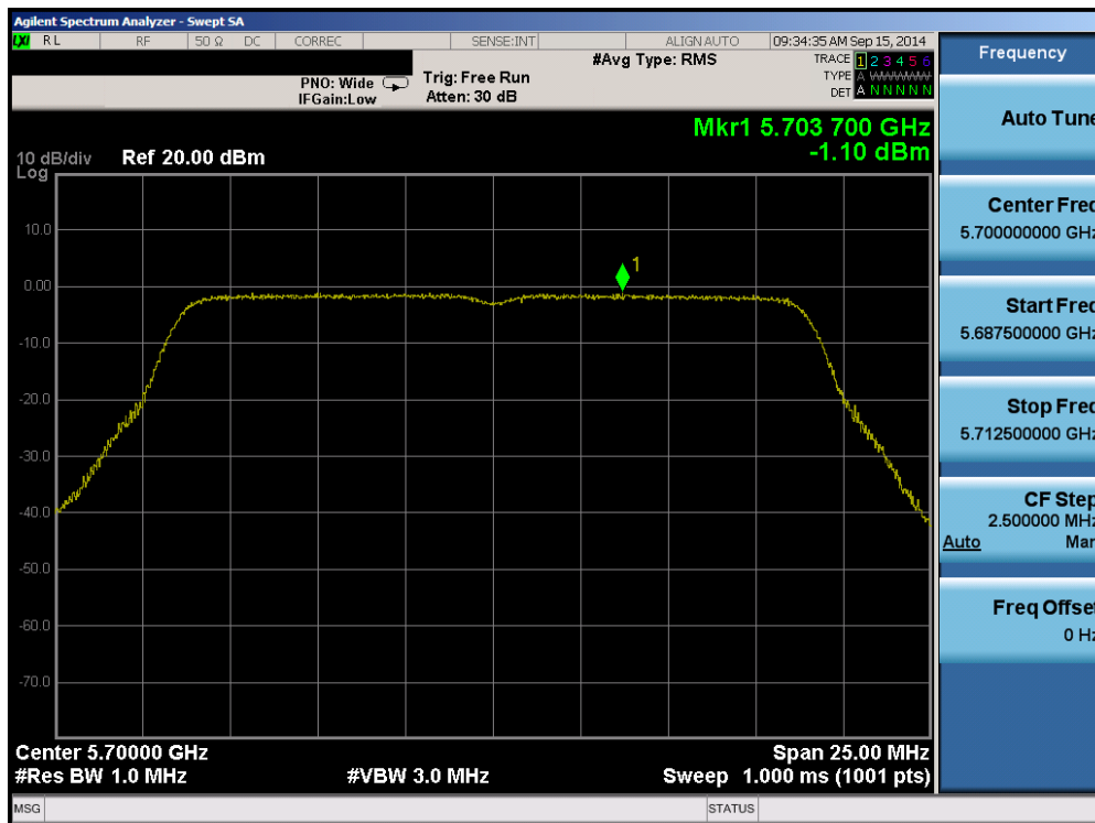
Plot 6-123. Peak Power Spectral Density Plot (20MHz BW 802.11n (UNII Band 2C) – Ch. 140)
