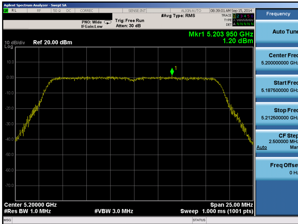
Plot 6-104. Peak Power Spectral Density Plot (20MHz BW 802.11n (UNII Band 1) – Ch. 40)
