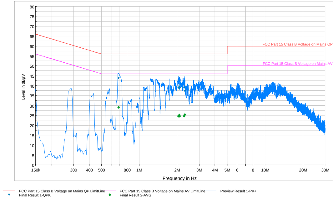
Plot 6-197. Line Conducted Plot with 802.11a UNII Band 1 (N)
