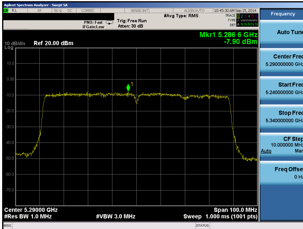
Plot 6-117. Peak Power Spectral Density Plot (80MHz BW 802.11ac (UNII Band 2A) – Ch. 58)
