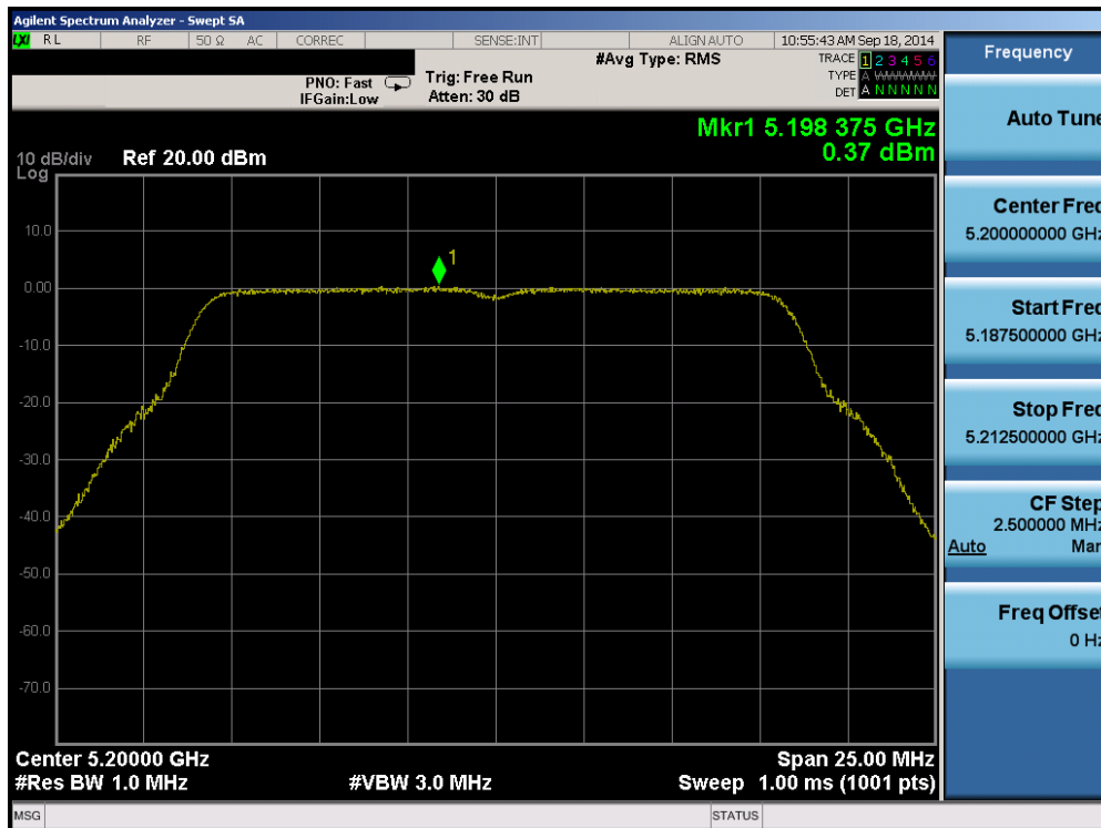
Plot 6-73. Peak Power Spectral Density Plot (802.11a (UNII Band 1) – Ch. 40)
