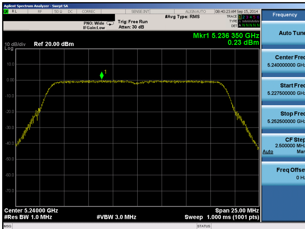
Plot 6-105. Peak Power Spectral Density Plot (20MHz BW 802.11n (UNII Band 1) – Ch. 48)
