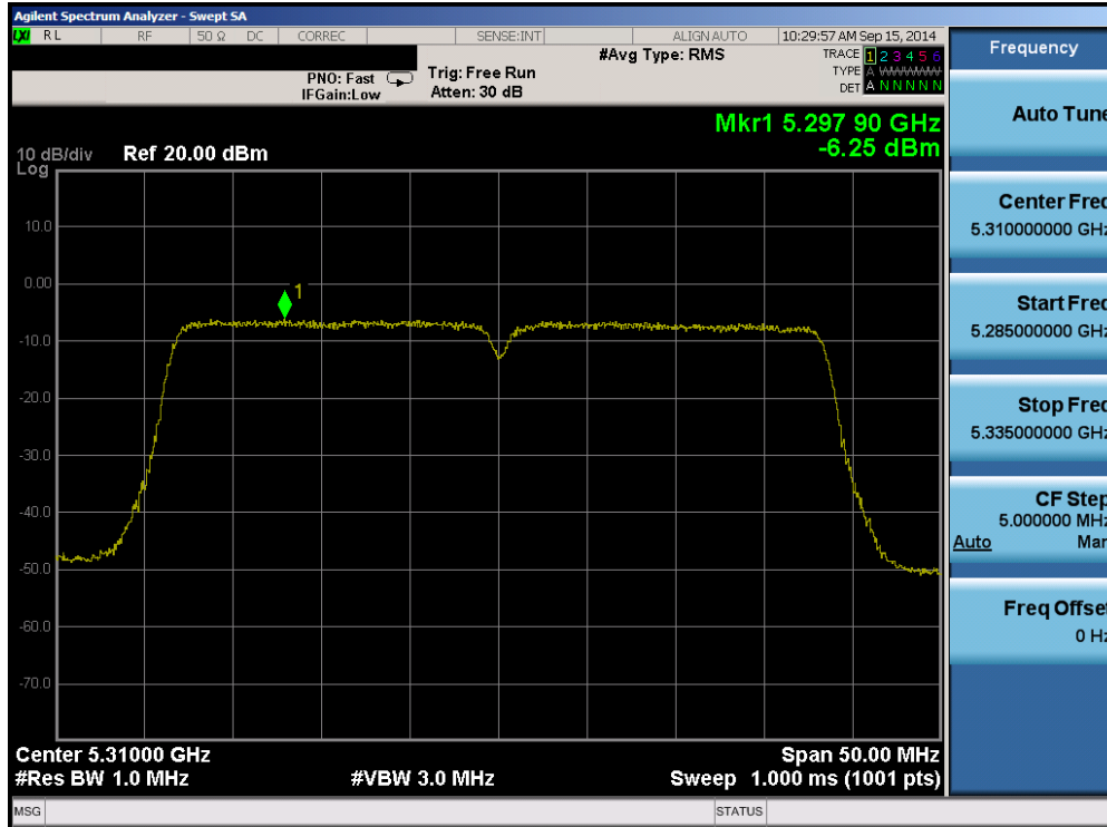
Plot 6-116. Peak Power Spectral Density Plot (40MHz BW 802.11n (UNII Band 2A) – Ch. 62)
