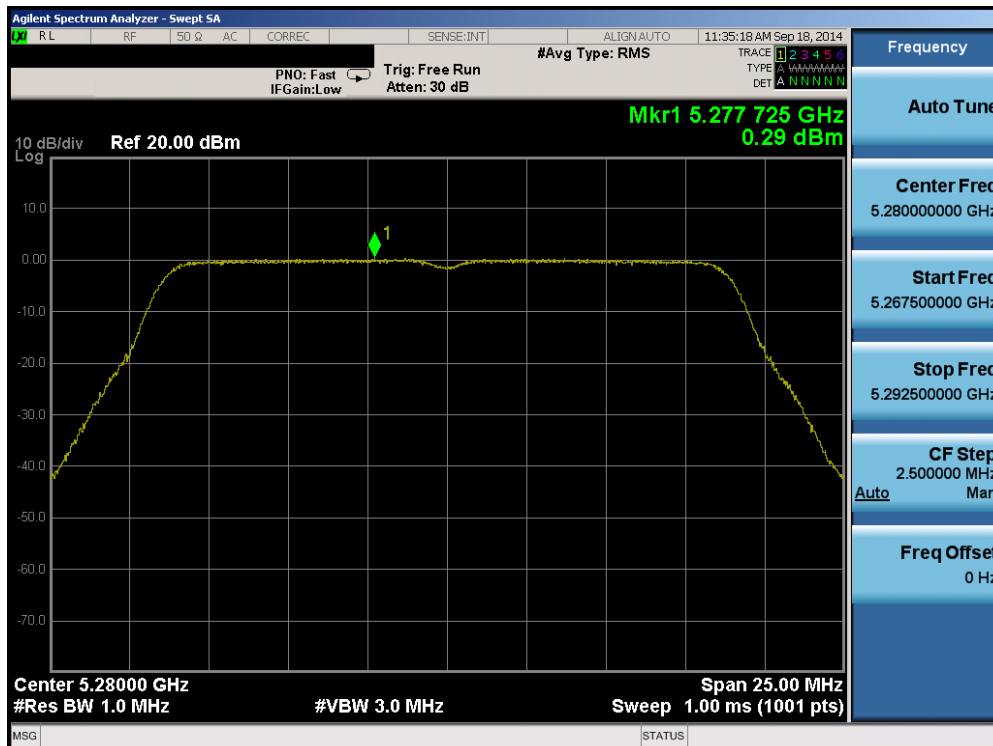
Plot 6-85. Peak Power Spectral Density Plot (20MHz BW 802.11n (UNII Band 2A) – Ch. 56)
