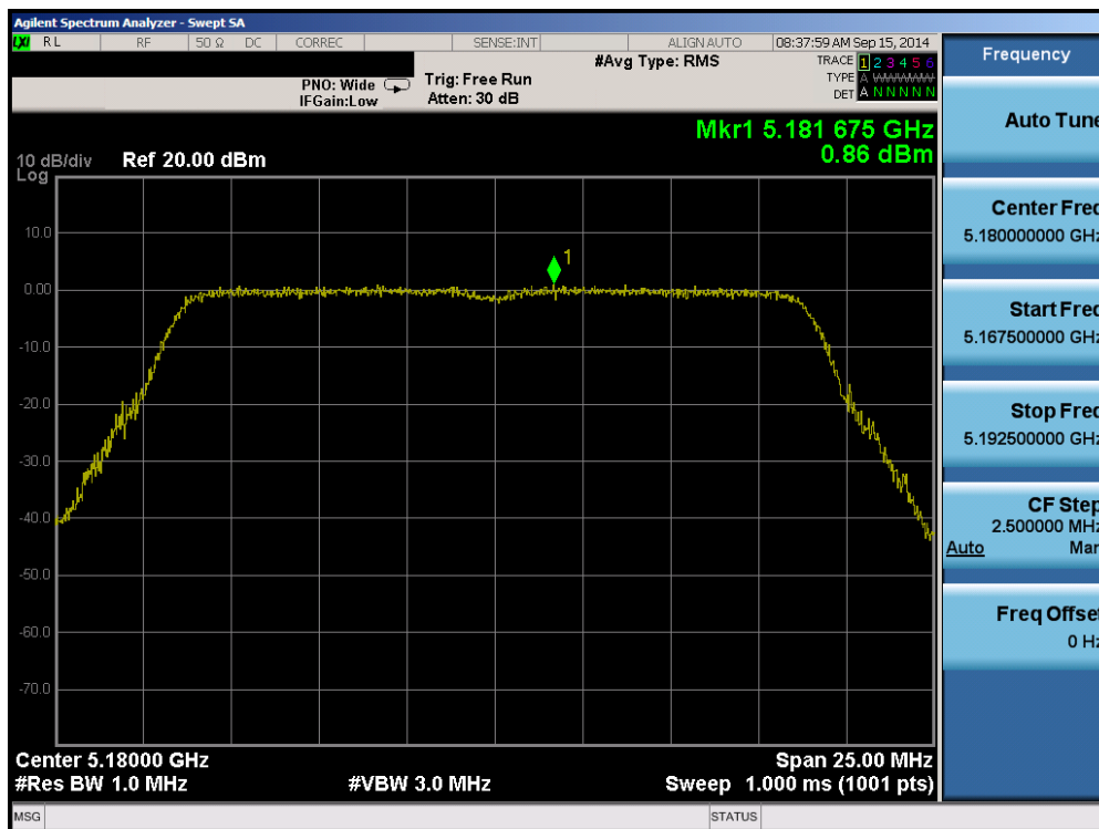
Plot 6-103. Peak Power Spectral Density Plot (20MHz BW 802.11n (UNII Band 1) – Ch. 36)
