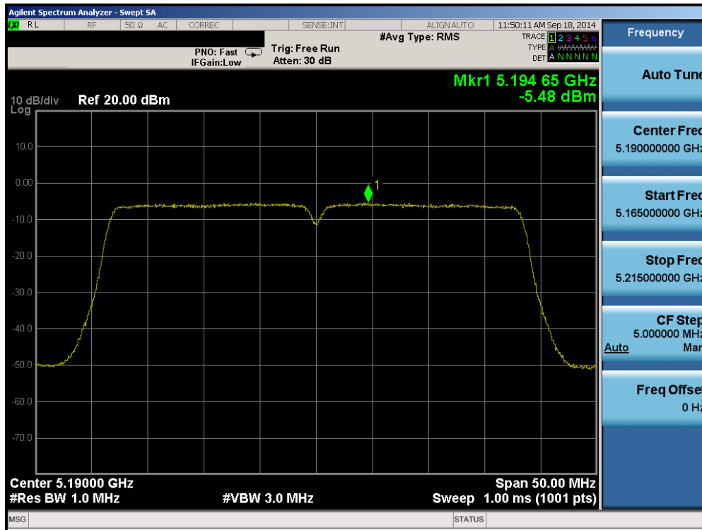
Plot 6-78. Peak Power Spectral Density Plot (40MHz BW 802.11n (UNII Band 1) – Ch. 38)
