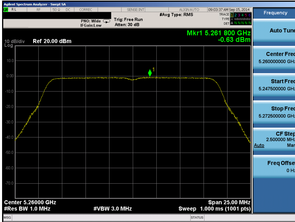
Plot 6-112. Peak Power Spectral Density Plot (20MHz BW 802.11n (UNII Band 2A) – Ch. 52)
