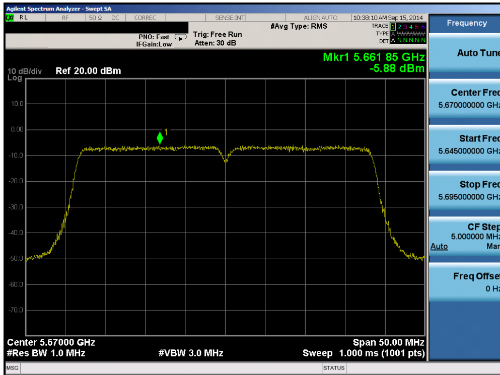
Plot 6-126. Peak Power Spectral Density Plot (40MHz BW 802.11n (UNII Band 2C) – Ch. 134)
