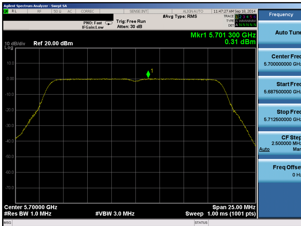
Plot 6-95. Peak Power Spectral Density Plot (20MHz BW 802.11n (UNII Band 2C) – Ch. 140)
