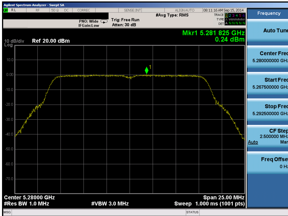
Plot 6-110. Peak Power Spectral Density Plot (802.11a (UNII Band 2A) – Ch. 56)
