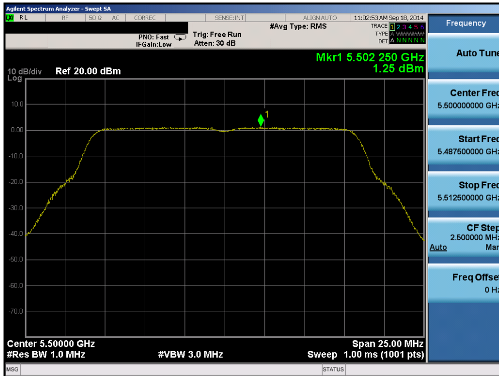
Plot 6-90. Peak Power Spectral Density Plot (802.11a (UNII Band 2C) – Ch. 100)
