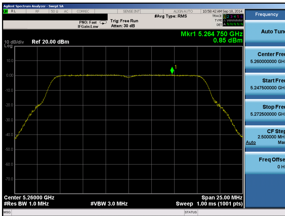
Plot 6-81. Peak Power Spectral Density Plot (802.11a (UNII Band 2A) – Ch. 52)
