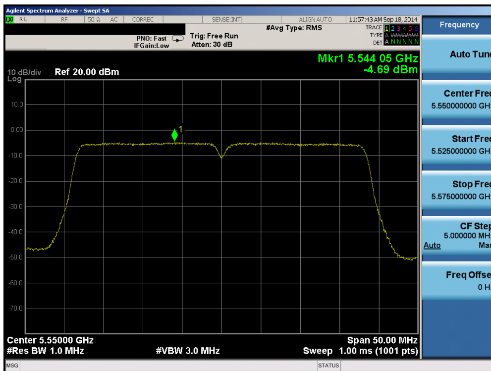
Plot 6-97. Peak Power Spectral Density Plot (40MHz BW 802.11n (UNII Band 2C) – Ch. 110)
