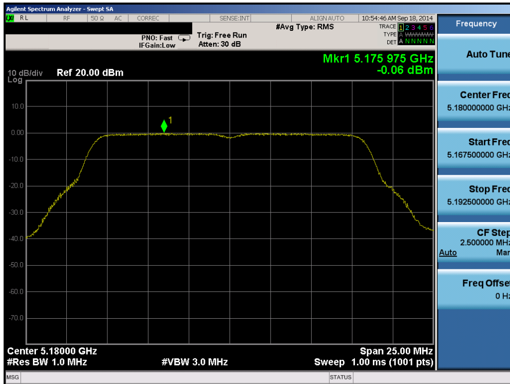
Plot 6-72. Peak Power Spectral Density Plot (802.11a (UNII Band 1) – Ch. 36)
