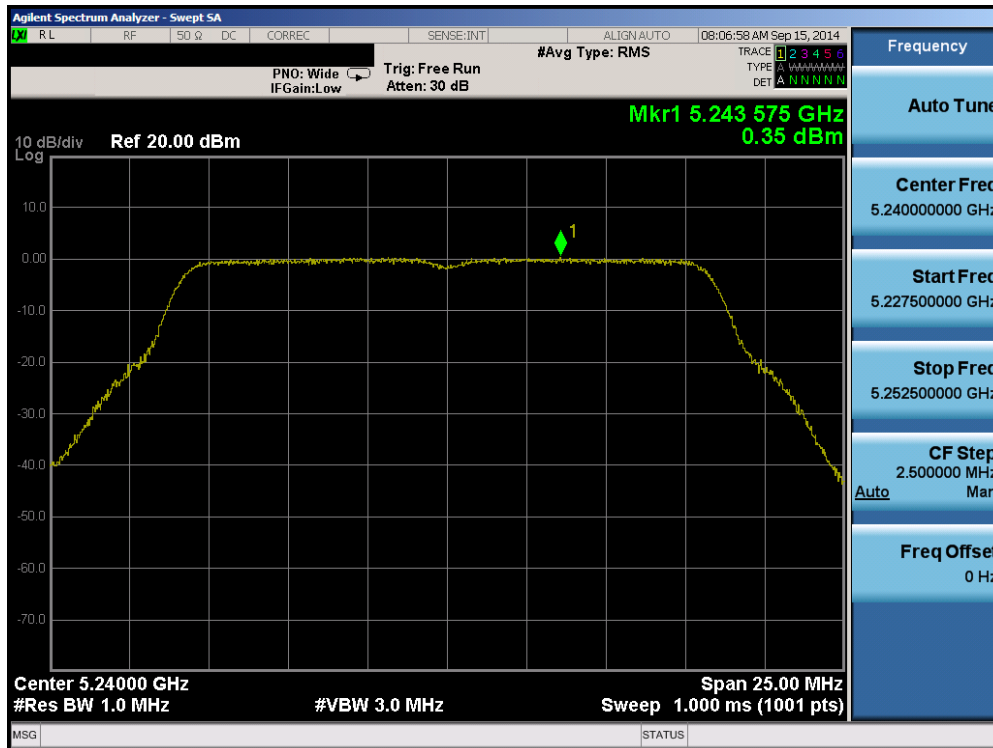
Plot 6-102. Peak Power Spectral Density Plot (802.11a (UNII Band 1) – Ch. 48)
