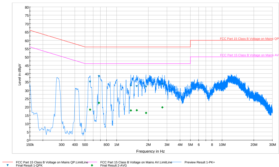
Plot 6-196. Line Conducted Plot with 802.11a UNII Band 1 (L1)
