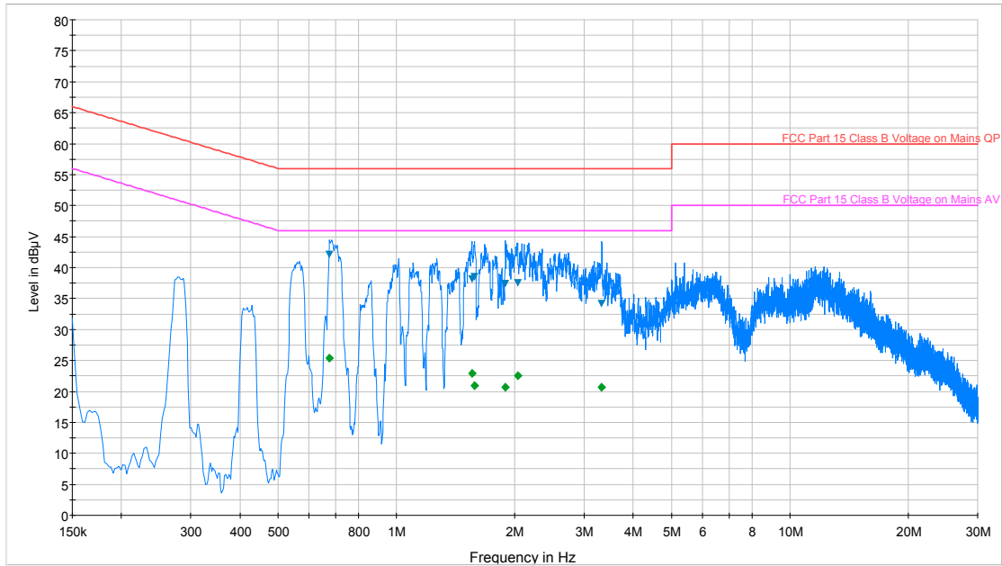
Plot 6-140. Line Conducted Plot with 802.11a (N)
