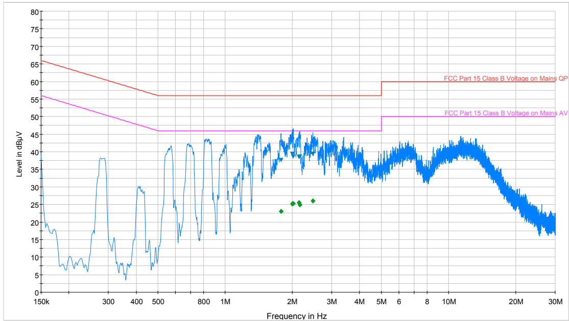
Plot 6-138. Line Conducted Plot with 802.11b (N)
