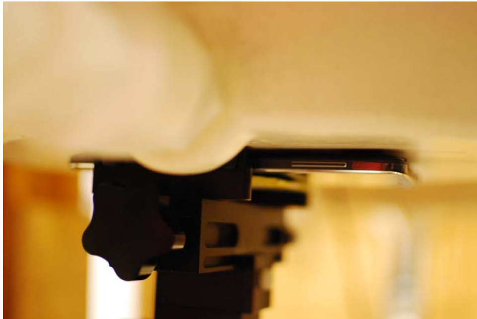
SAR Test Setup Photo 12 – Back Side at 0.0 cm, Standard Cover
