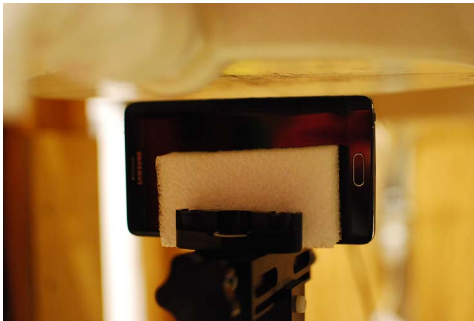
SAR Test Setup Photo 23 – Right Edge at 1.0 cm, Standard Cover
