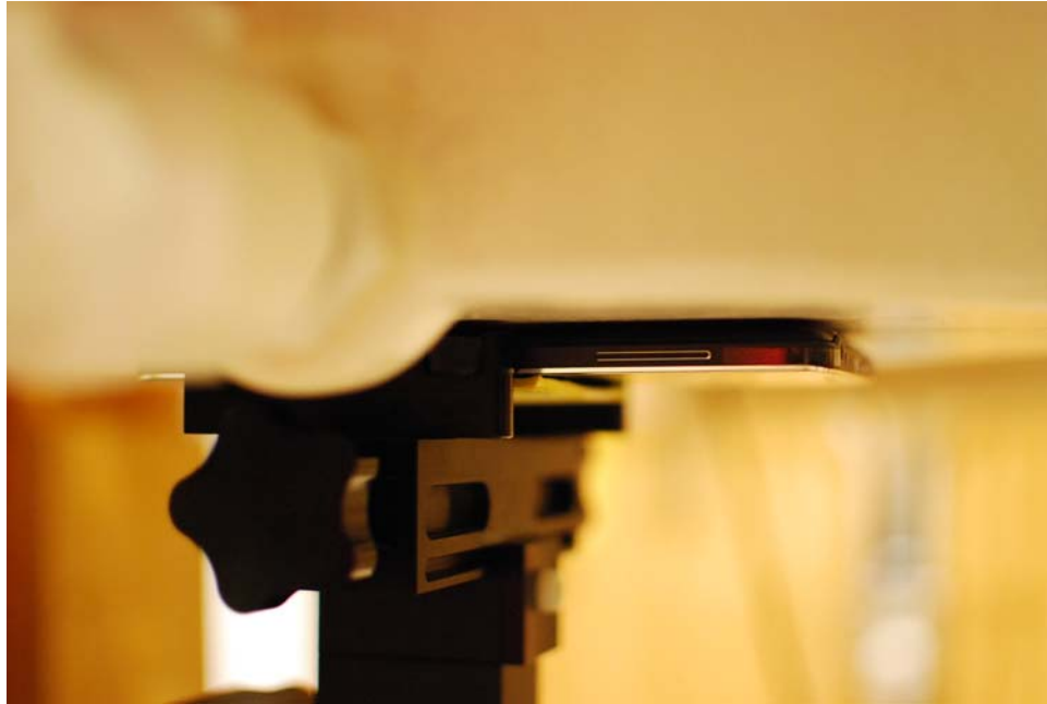
SAR Test Setup Photo 13- Back Edge at 0mm, Wireless Charging Cover
