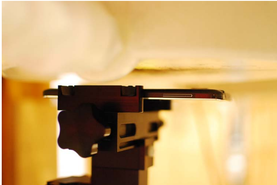
SAR Test Setup Photo 8 – Back Side at 1.5 cm, Standard Cover
