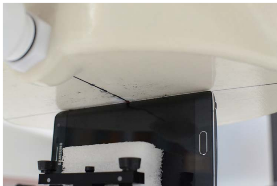
SAR Test Setup Photo 24 – Right Edge at 0.0 cm, Standard Cover
