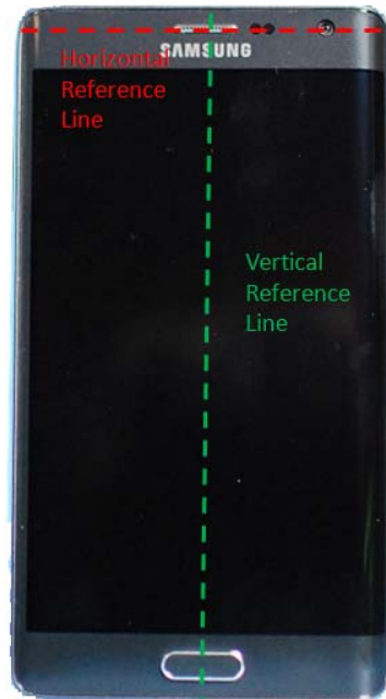
SAR Test Setup Photo 27 – Horizontal and Vertical Reference Lines
