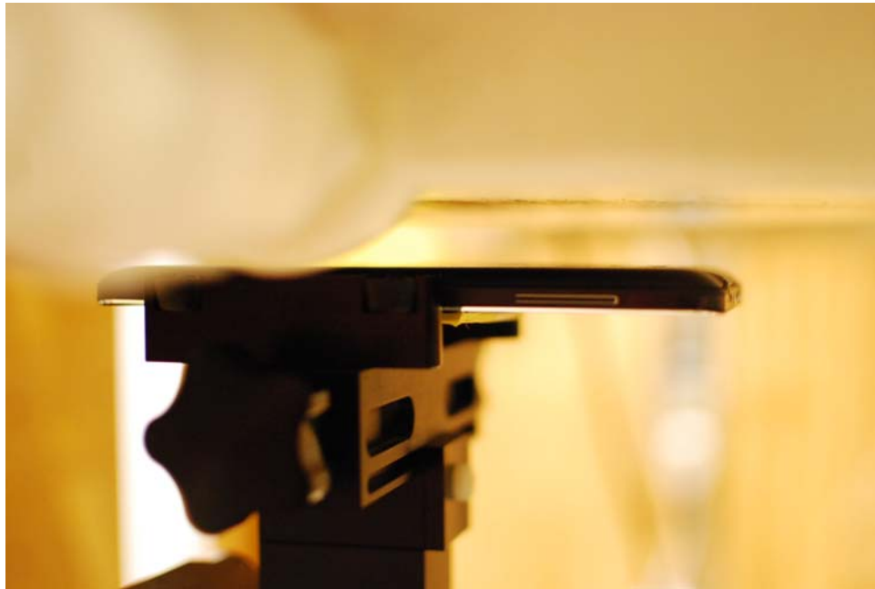
SAR Test Setup Photo 9- Back Side at 1.5 cm, Wireless Charging Cover
