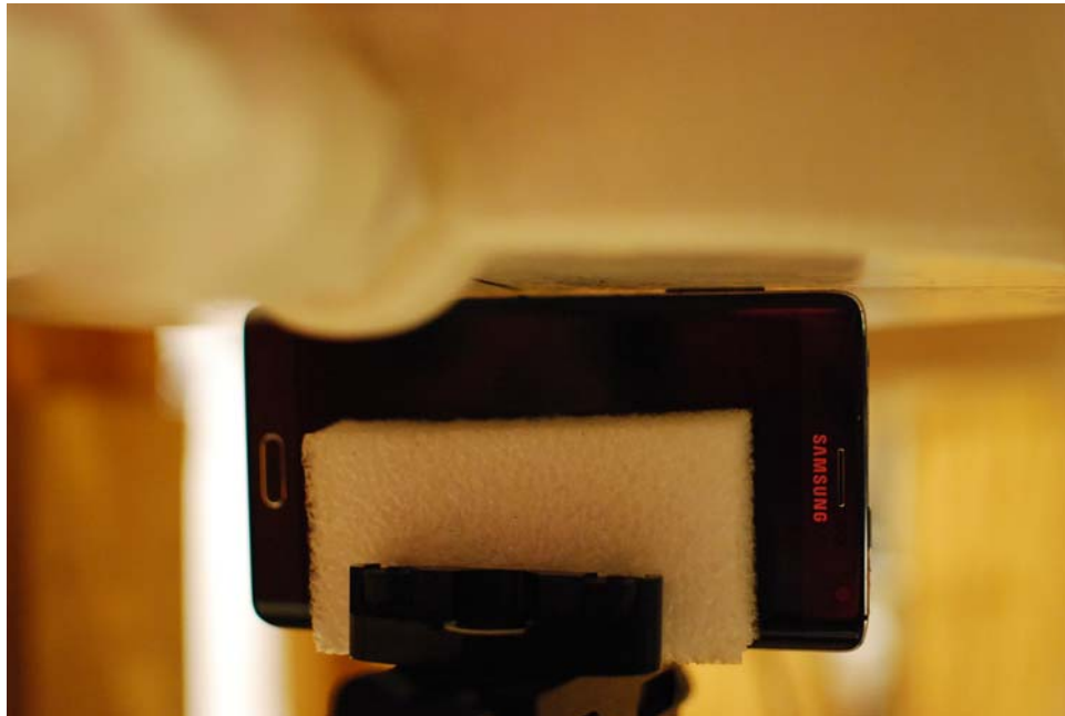
SAR Test Setup Photo 26 – Left Edge at 0.0 cm, Standard Cover
