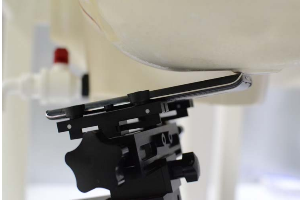
SAR Test Setup Photo 7 – Left Tilt, Wireless Charging Cover
