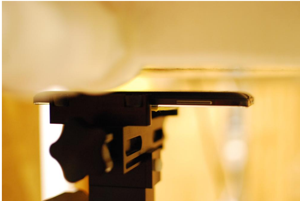
SAR Test Setup Photo 7 - Back Side at 1.5 cm, Wireless Charging Cover
