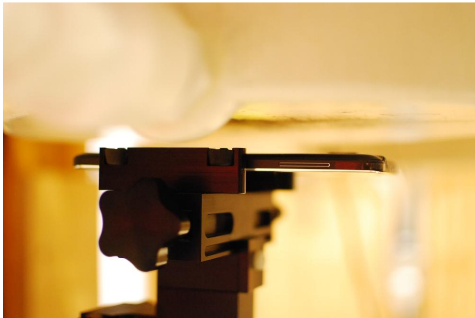
SAR Test Setup Photo 6 – Back Side at 1.5 cm, Standard Cover
