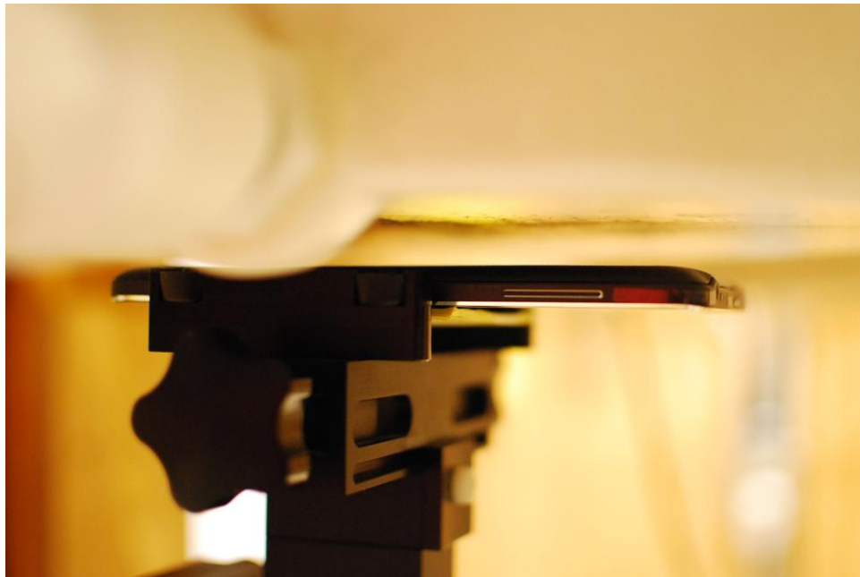
SAR Test Setup Photo 8 – Back Side at 1.0 cm, Standard Cover
