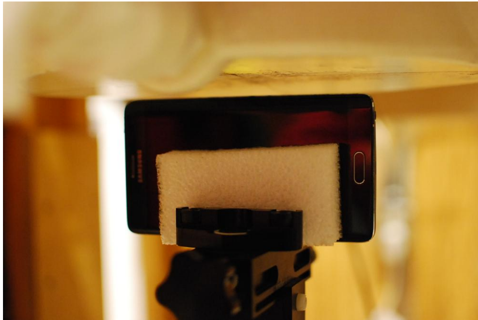
SAR Test Setup Photo 12 – Right Edge at 1.0 cm, Standard Cover
