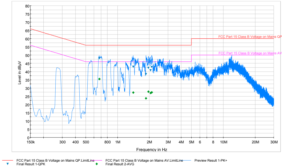
Plot 6-45. Line-Conducted Test Plot (N)
