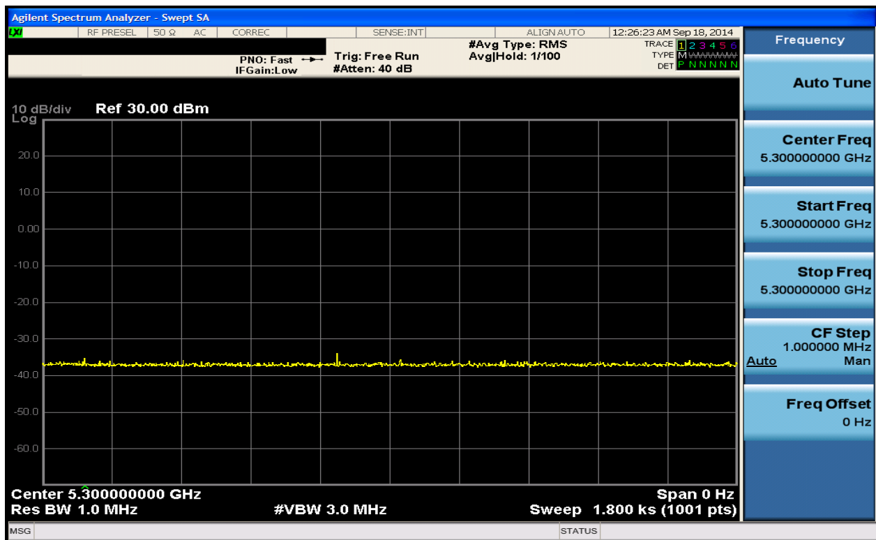
Figure 5-3. Band 2A Non-occupancy Period - Monitoring live spectrum - Elapse time 30 minutes
