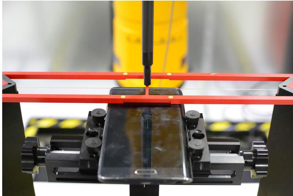
Figure 18-1 Ear Reference Point HAC Phantom Alignment
