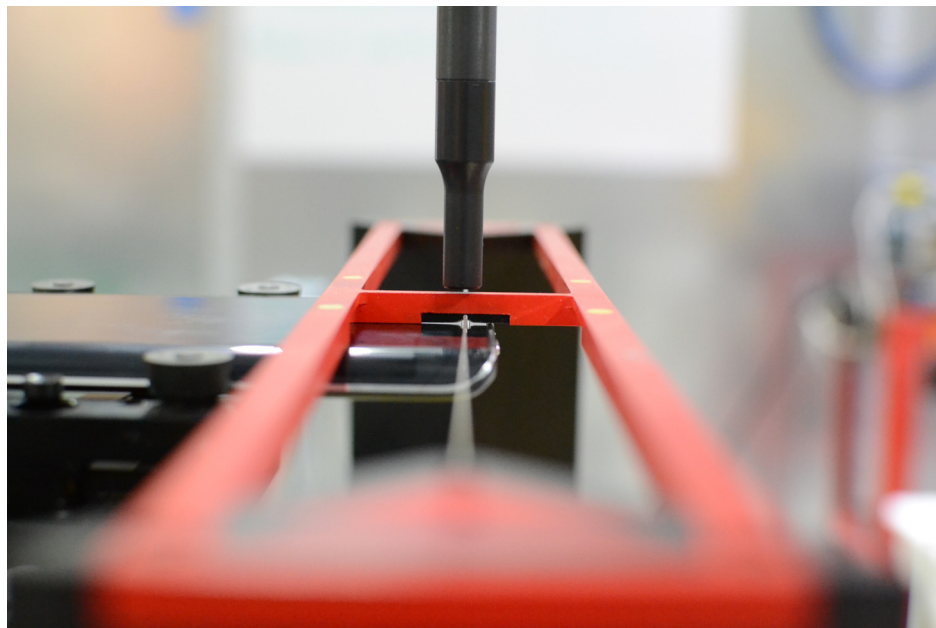
Figure 18-2 HAC Phantom Plane Alignment
