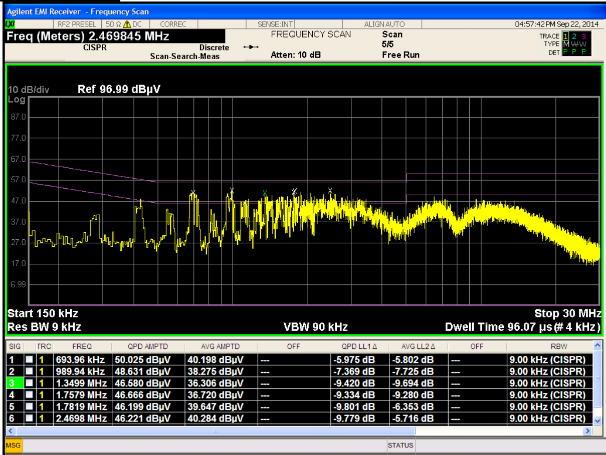
Plot 6-22. Line Conducted Plot with Bluetooth LE (L1)
