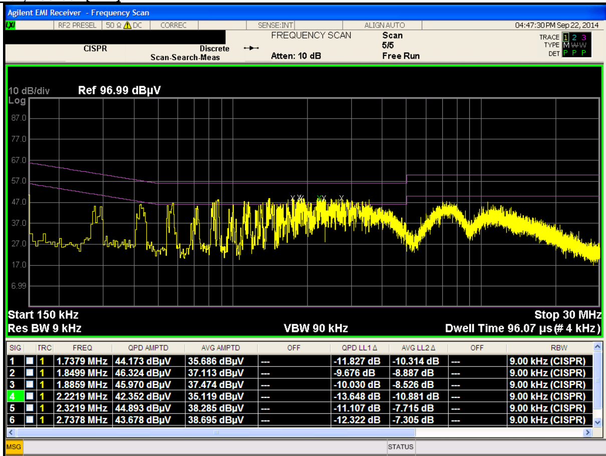
Plot 6-23. Line Conducted Plot with Bluetooth LE (N)
