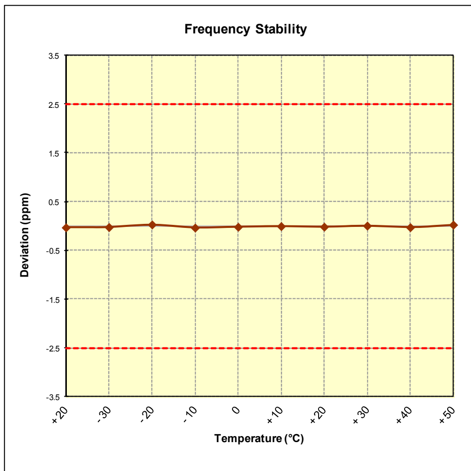
Figure 6-7. Frequency Stability Graph (Band 12)
