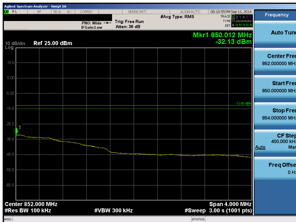
Plot 6-86. Upper Extended Band Edge Plot (Band 5 - Band 5 - 3.0MHz QPSK - RB Size 15)
