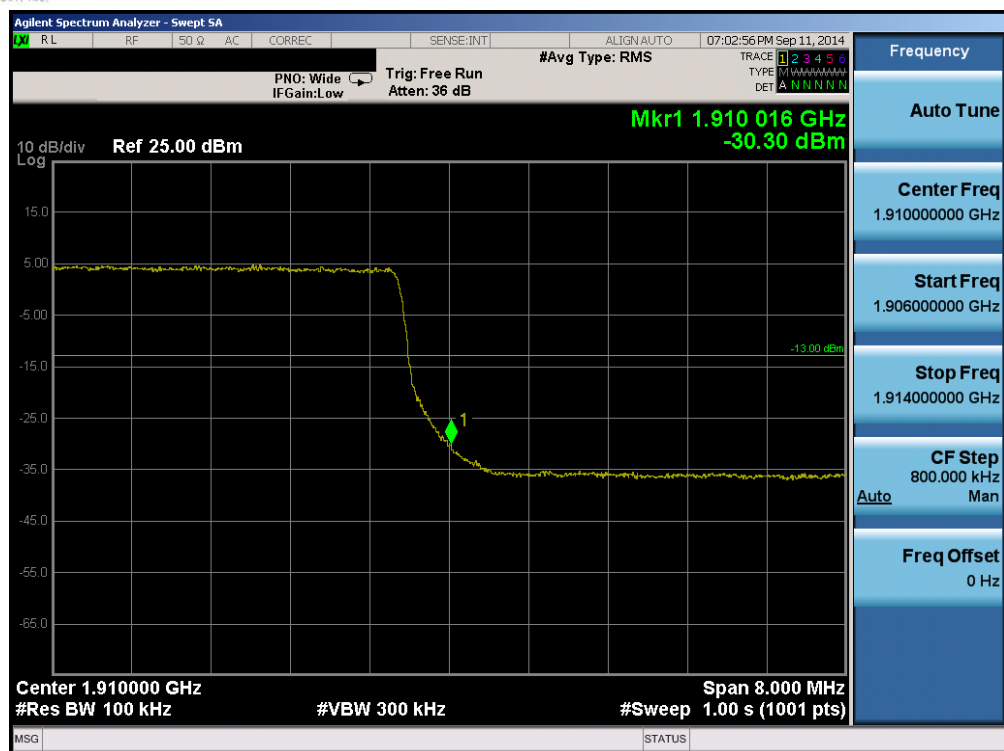
Plot 6-131. Upper Band Edge Plot (Band 2 – 10.0MHz QPSK – RB Size 50)
