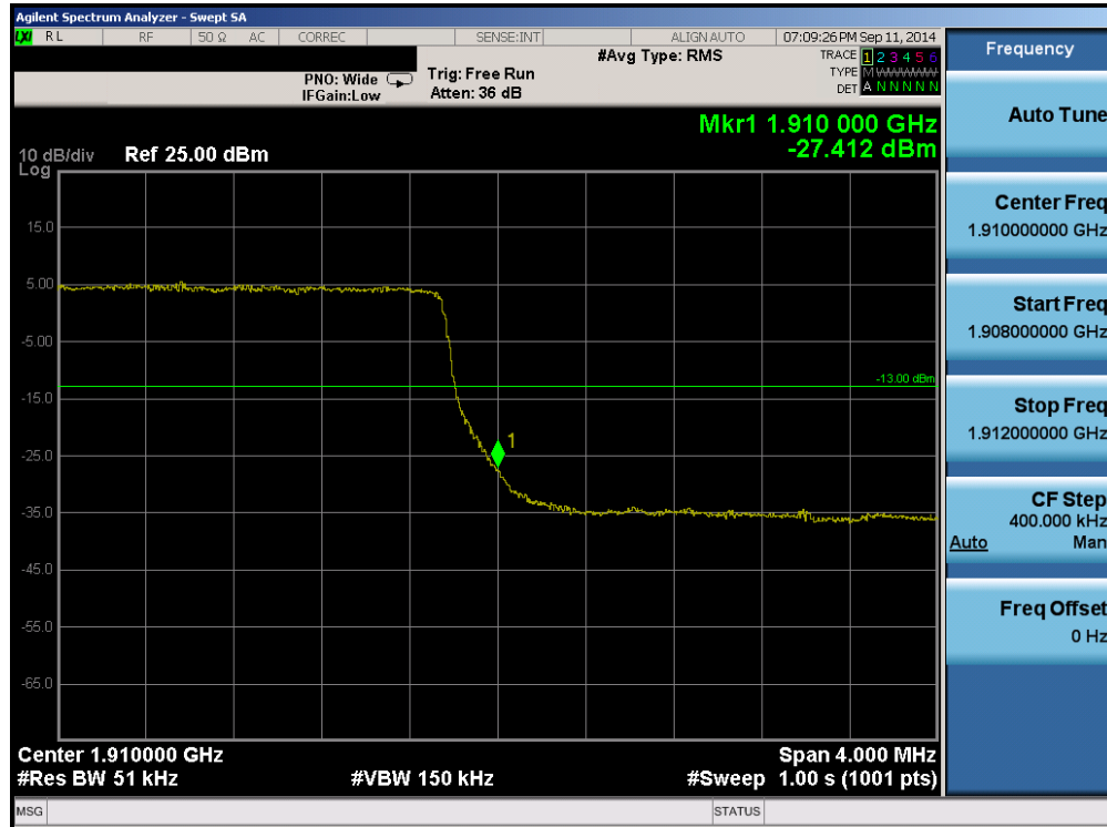
Plot 6-127. Upper Band Edge Plot (Band 2 – 5.0MHz QPSK – RB Size 25)
