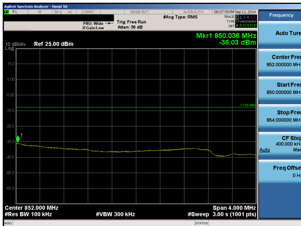
Plot 6-90. Upper Extended Band Edge Plot (Band 5 – 5.0MHz QPSK – RB Size 25)
