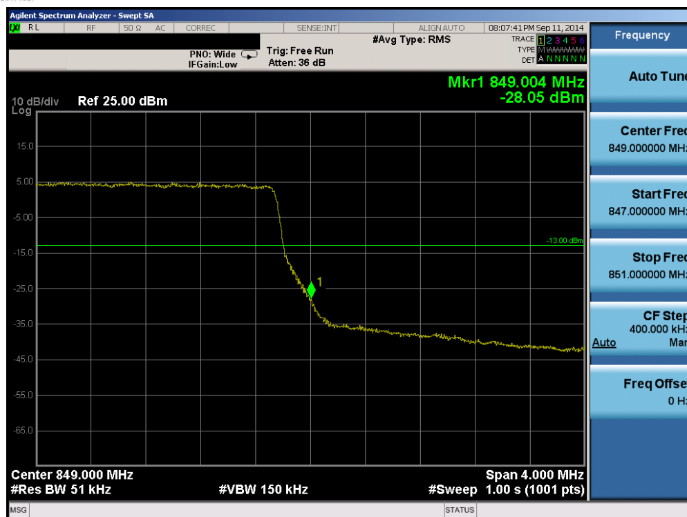
Plot 6-89. Upper Band Edge Plot (Band 5 – 5.0MHz QPSK – RB Size 25)
