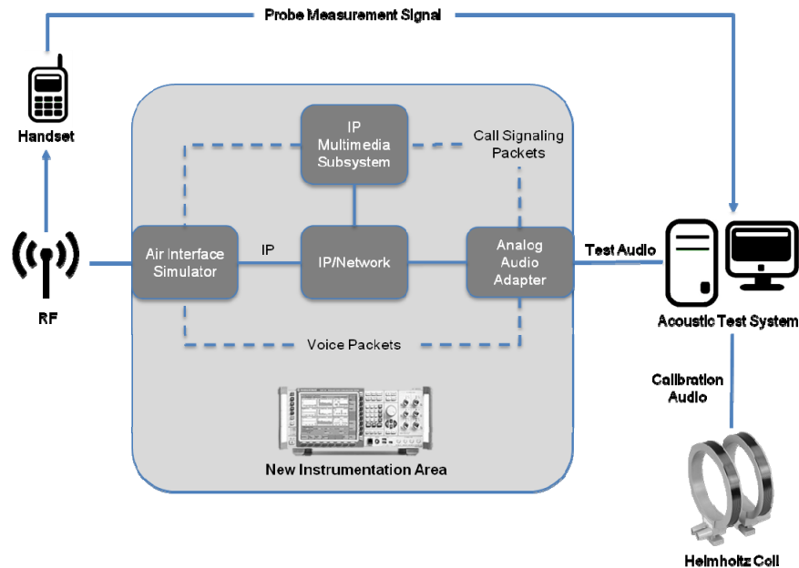
Figure 6-1 Test Setup for VoLTE T-Coil Measurements
