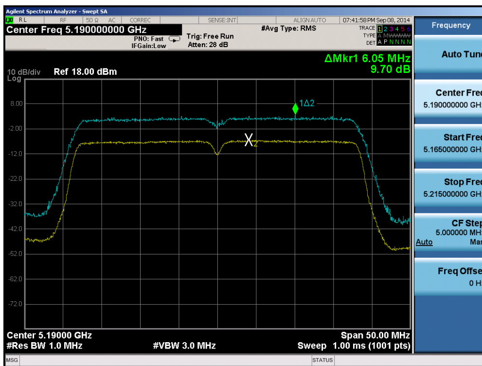
Plot 6-129. Peak Excursion Ratio Plot (40MHz BW 802.11n (UNII Band 1) – Ch. 38)
