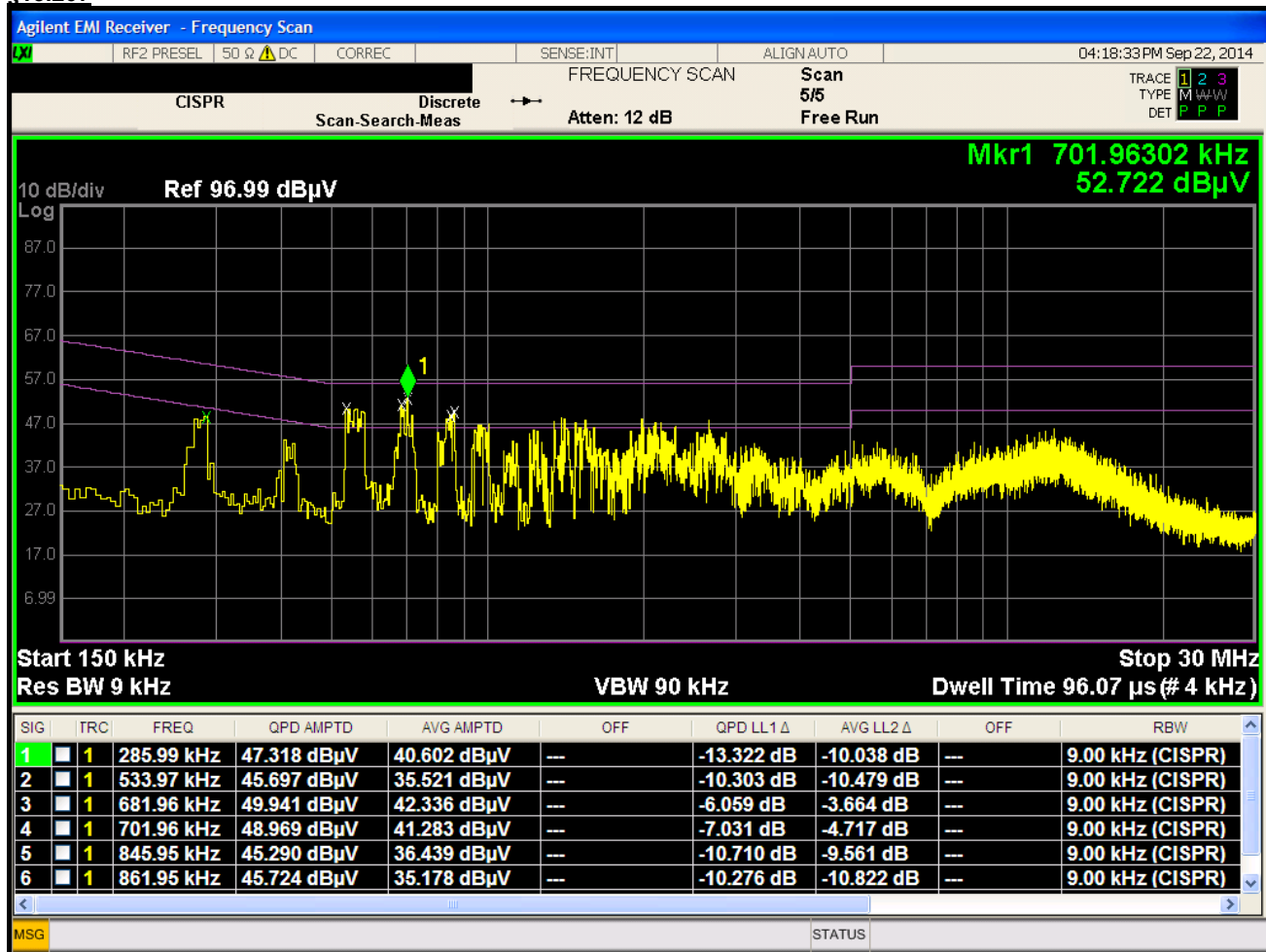
Plot 6-145. Line Conducted Plot with 802.11a (L1)
