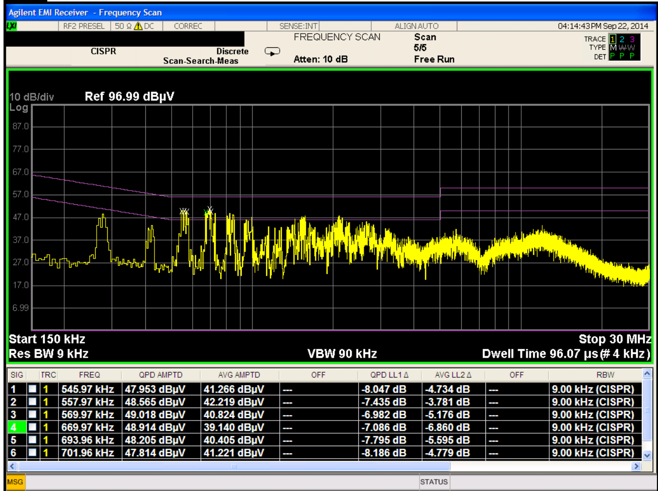
Plot 6-146. Line Conducted Plot with 802.11a (N)
