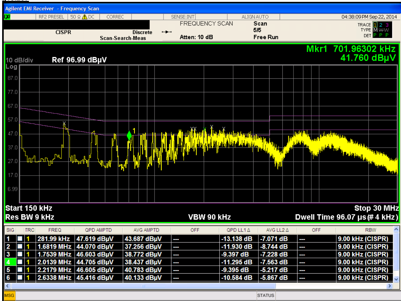
Plot 6-143. Line Conducted Plot with 802.11b (L1)
