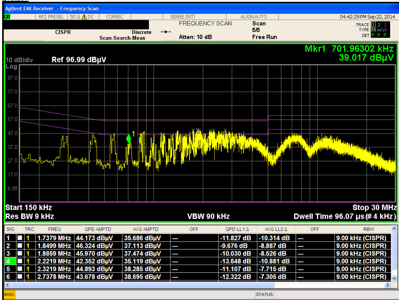
Plot 6-144. Line Conducted Plot with 802.11b (N)
