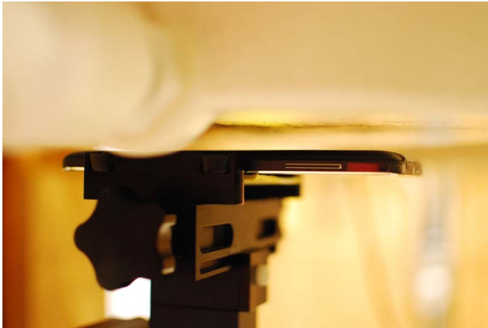
SAR Test Setup Photo 10: Back Side at 10mm, Wireless Charging Cover
