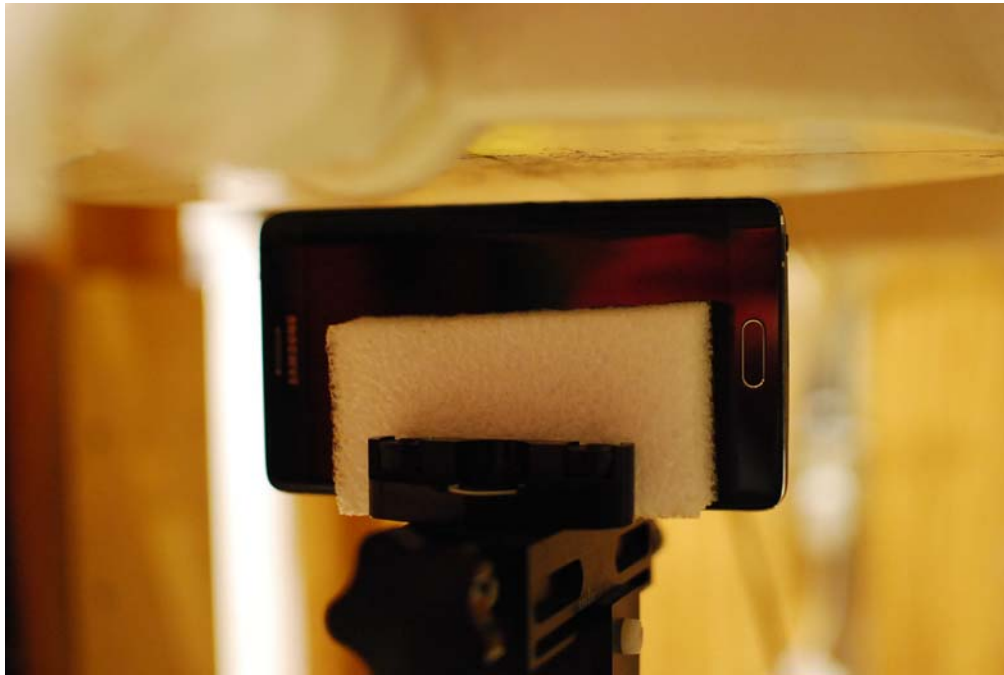
SAR Test Setup Photo 16: Right Edge at 10mm, Standard Back Cover
