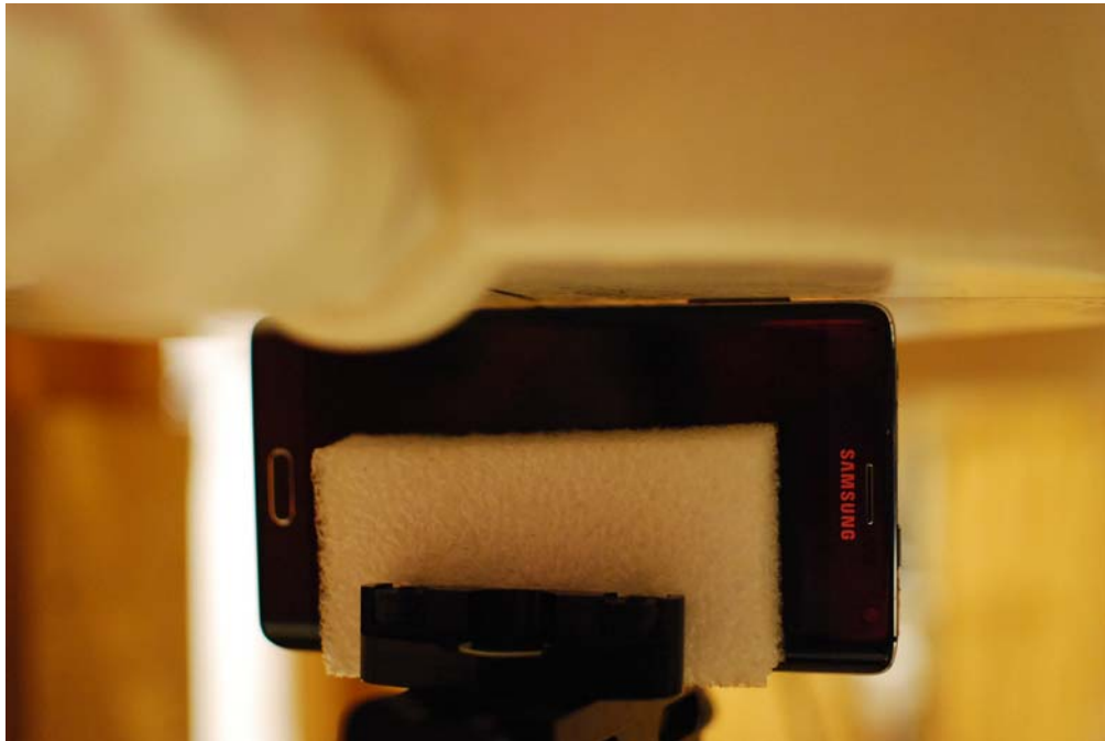
SAR Test Setup Photo 24: Left Edge at 0mm, Standard Back Cover
