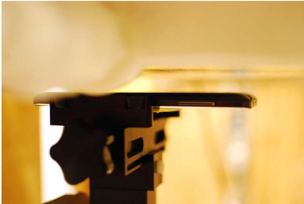
SAR Test Setup Photo 8: Back Side at 15mm, Wireless Charging Cover
