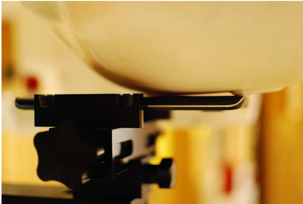
SAR Test Setup Photo 4: Left Cheek, Standard Back Cover
