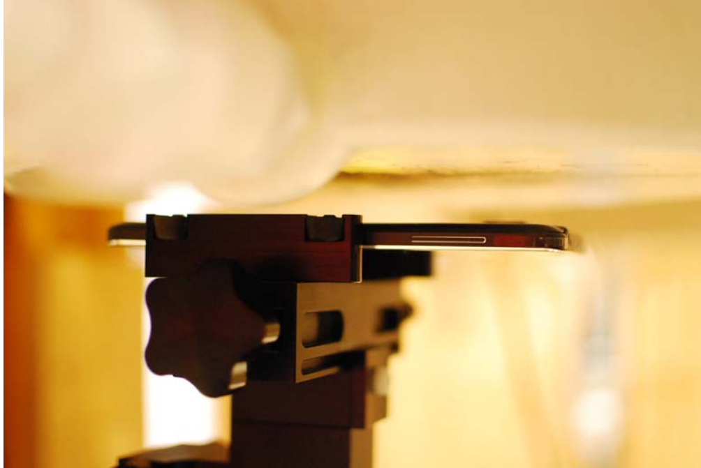
SAR Test Setup Photo 7: Back Side at 15mm, Standard Back Cover
