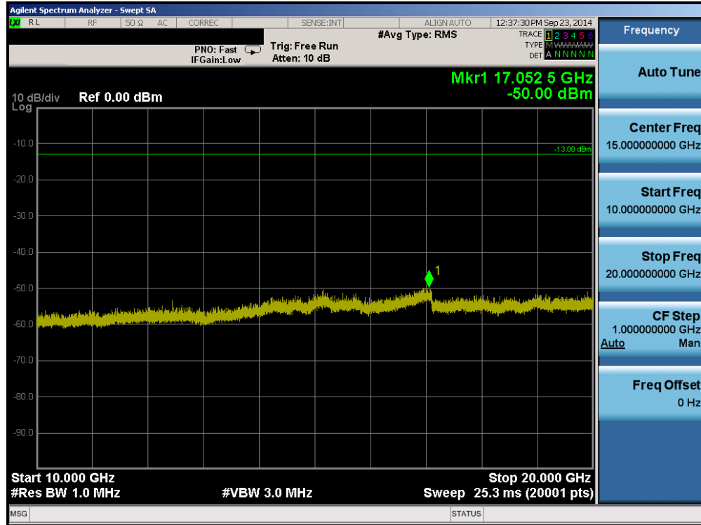
Plot 6-47. Conducted Spurious Plot (PCS WCDMA Mode – Ch. 9538)
