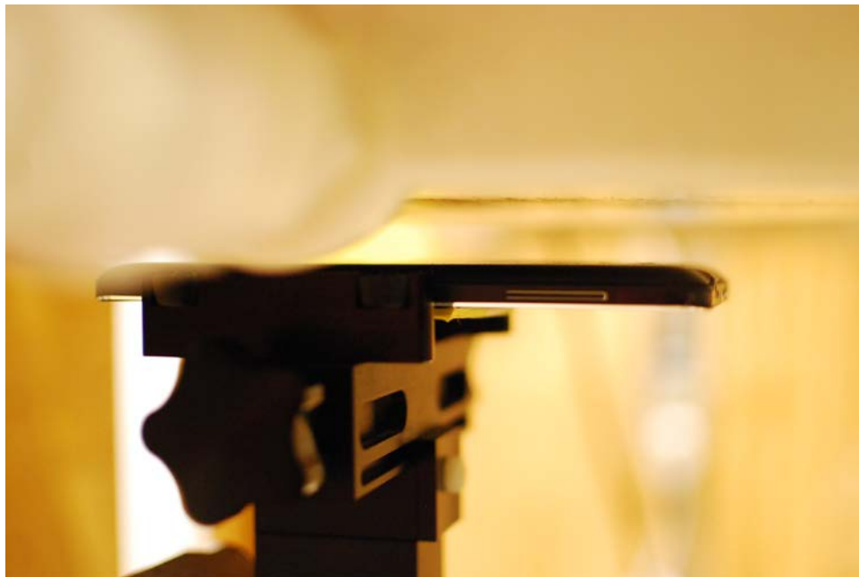
SAR Test Setup Photo 10 – Back Side at 1.5 cm with Wireless Charging Cover
