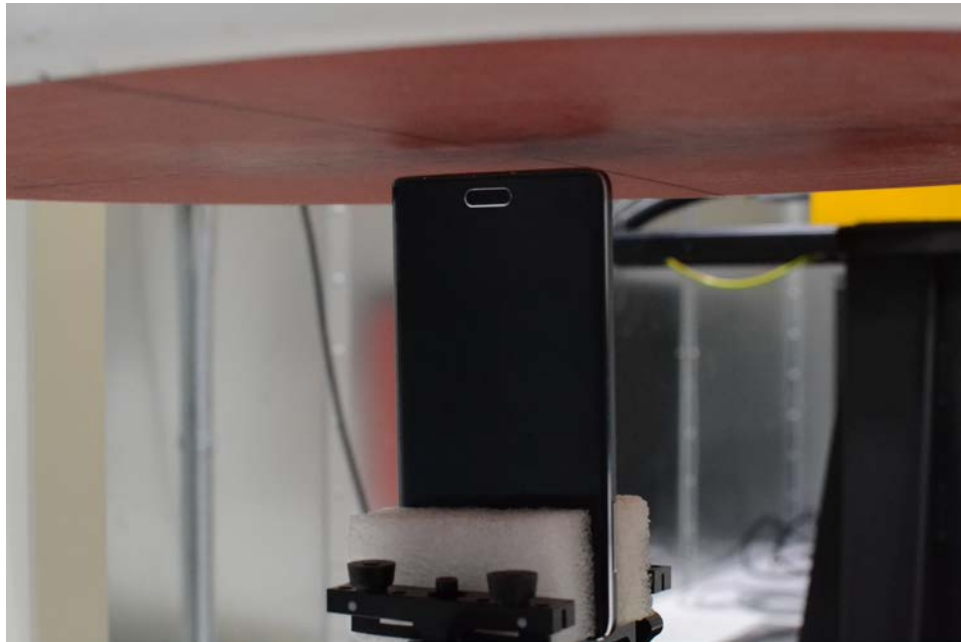
SAR Test Setup Photo 22 – Bottom Edge at 0.6 cm
