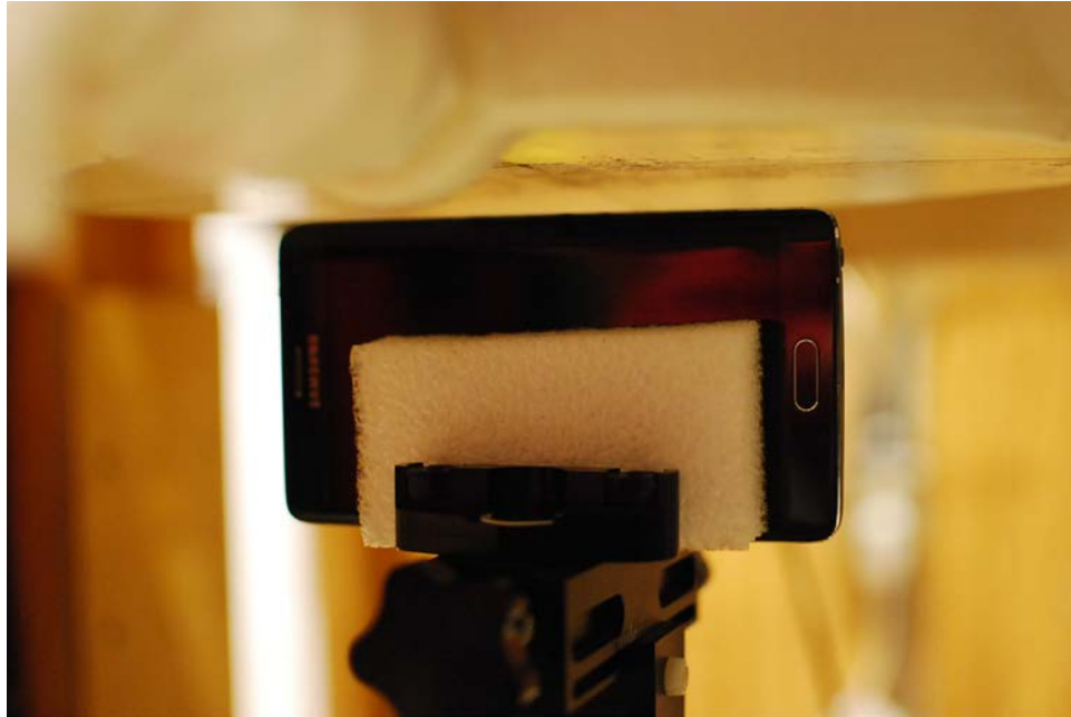
SAR Test Setup Photo 25 – Right Edge at 1.0 cm
