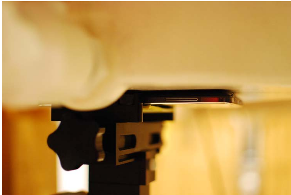
SAR Test Setup Photo 12 – Back Side at 0.0 cm with Wireless Charging Cover
