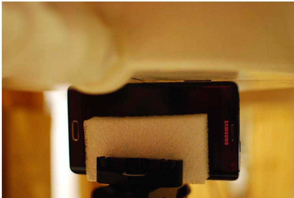
SAR Test Setup Photo 28 – Left Edge at 0.0 cm
