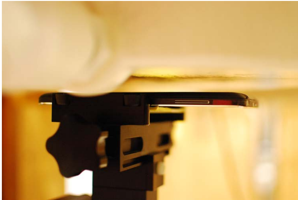
SAR Test Setup Photo 8 – Back Side at 1.0 cm with Wireless Charging Cover
