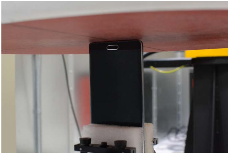
SAR Test Setup Photo 24 – Bottom Edge at 0.0 cm with Wireless Charging
