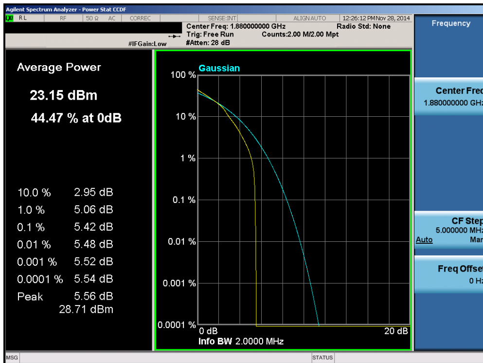
Plot 6-142. PAR Plot (Band 2 – 1.4MHz 16-QAM – RB Size 6)
