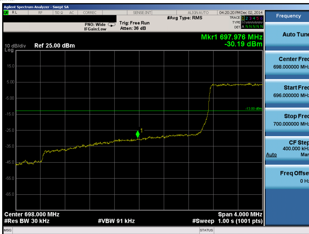
Plot 6-69. Lower Band Edge Plot (Band 12 – 3.0MHz QPSK – RB Size 15)
