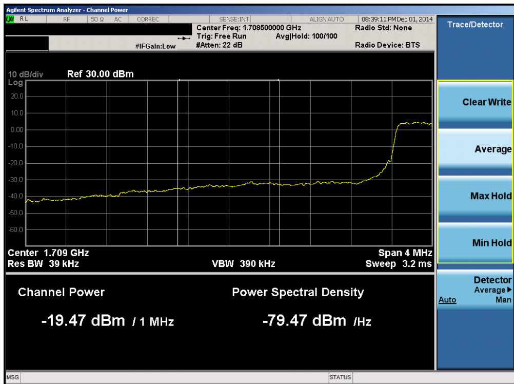
Plot 6-98. Lower Extended Band Edge Plot (Band 4 – 3.0MHz QPSK – RB Size 15)
