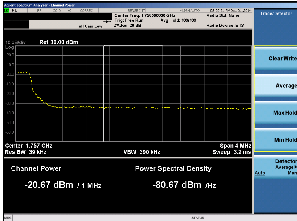
Plot 6-104. Upper Extended Band Edge Plot (Band 4 – 5.0MHz QPSK – RB Size 25)
