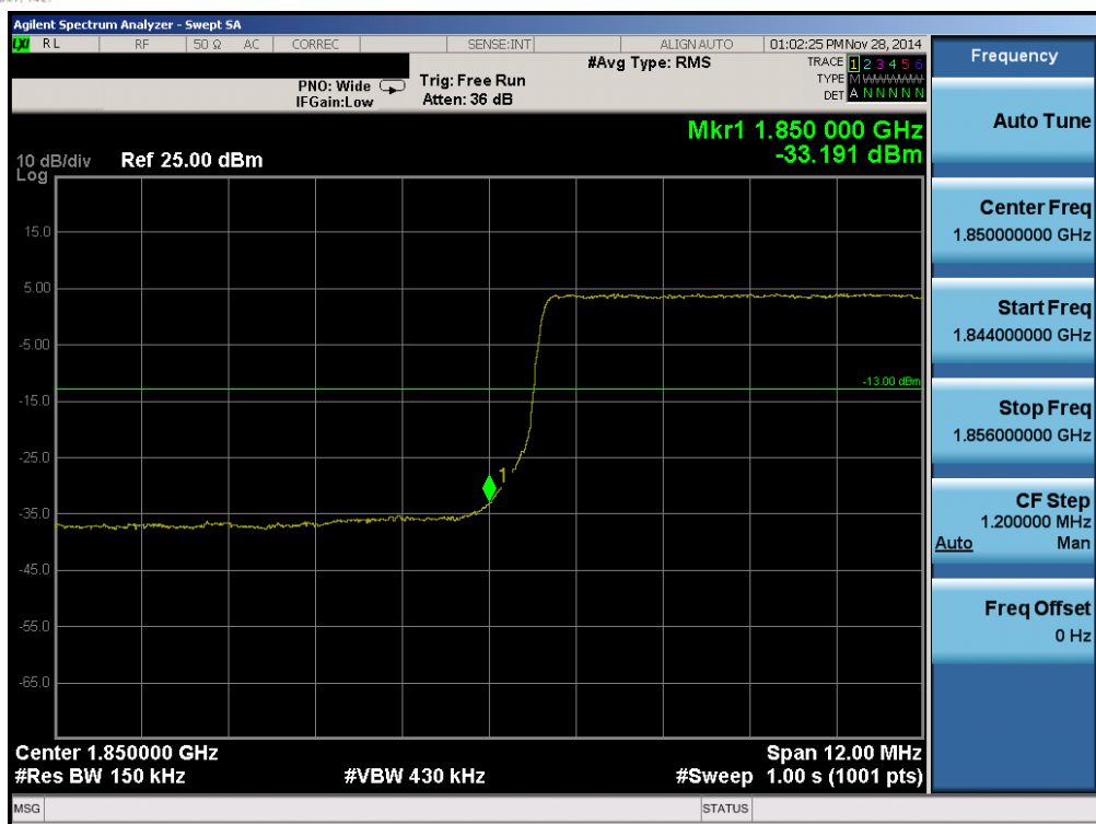
Plot 6-133. Lower Band Edge Plot (Band 2 – 15.0MHz QPSK – RB Size 75)
