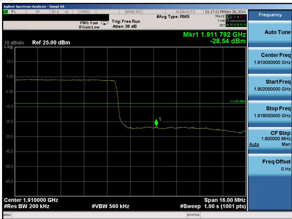
Plot 6-139. Upper Band Edge Plot (Band 2 – 20.0MHz QPSK – RB Size 100)
