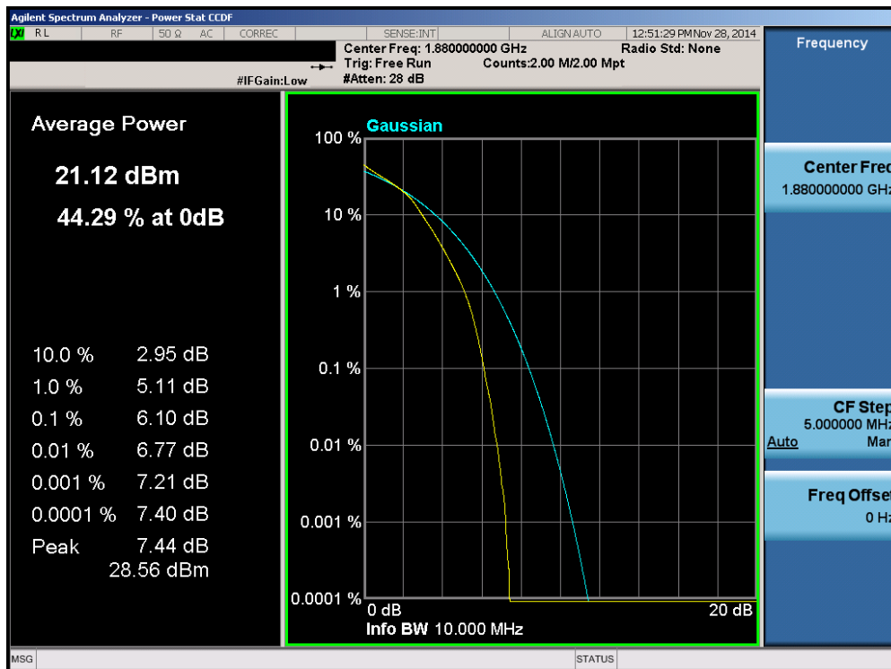
Plot 6-148. PAR Plot (Band 2 – 10.0MHz 16-QAM – RB Size 50)
