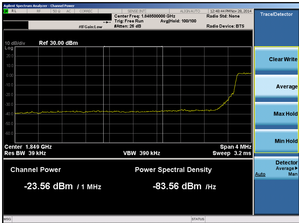
Plot 6-126. Lower Extended Band Edge Plot (Band 2 – 5.0MHz QPSK – RB Size 25)
