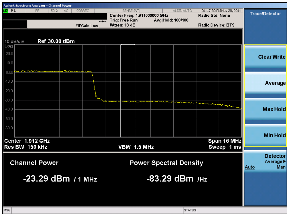
Plot 6-140. Upper Extended Band Edge Plot (Band 2 – 20.0MHz QPSK – RB Size 100)
