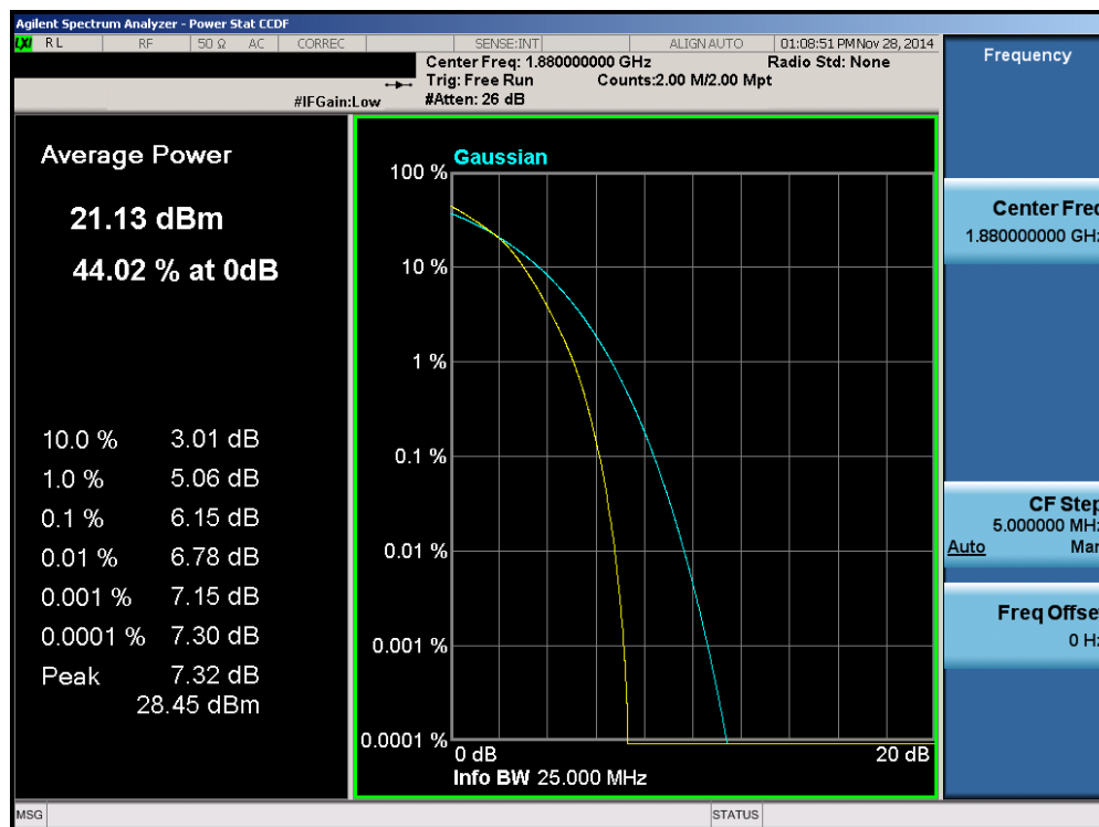
Plot 6-152. PAR Plot (Band 2 – 20.0MHz 16-QAM – RB Size 100)
