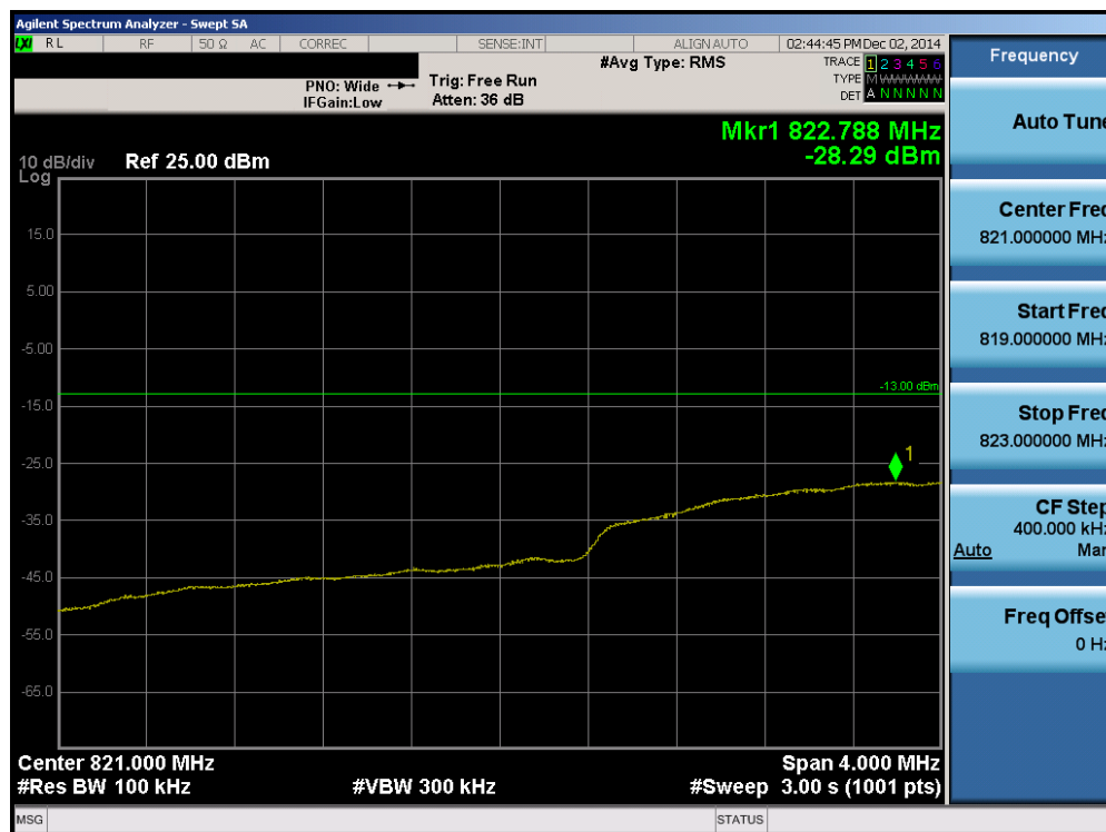
Plot 6-84. Lower Extended Band Edge Plot (Band 5 – 3.0MHz QPSK – RB Size 15)
