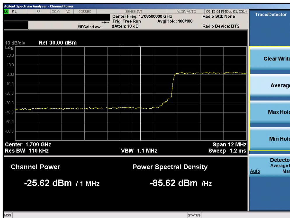
Plot 6-110. Lower Extended Band Edge Plot (Band 4 – 15.0MHz QPSK – RB Size 75)
