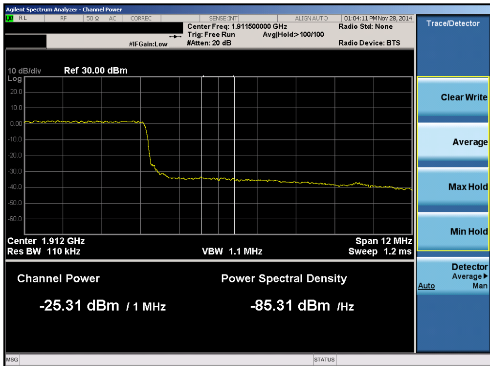
Plot 6-136. Upper Extended Band Edge Plot (Band 2 – 15.0MHz QPSK – RB Size 75)
