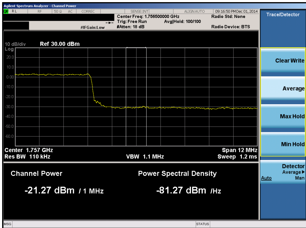
Plot 6-112. Upper Extended Band Edge Plot (Band 4 – 15.0MHz QPSK – RB Size 75)
