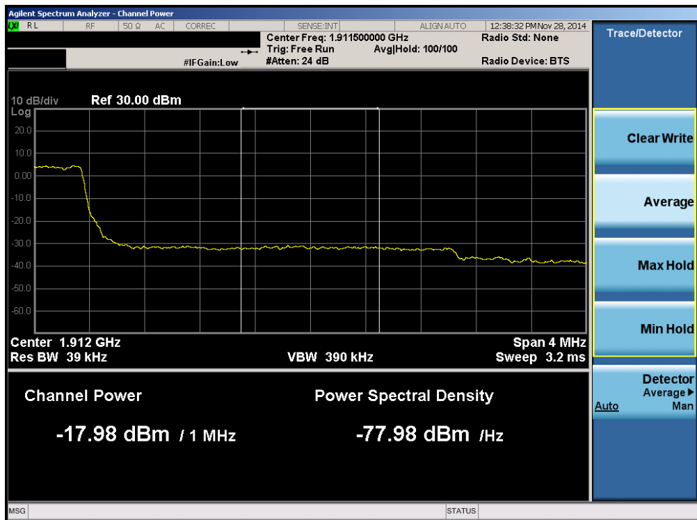
Plot 6-124. Upper Extended Band Edge Plot (Band 2 – 3.0MHz QPSK – RB Size 15)
