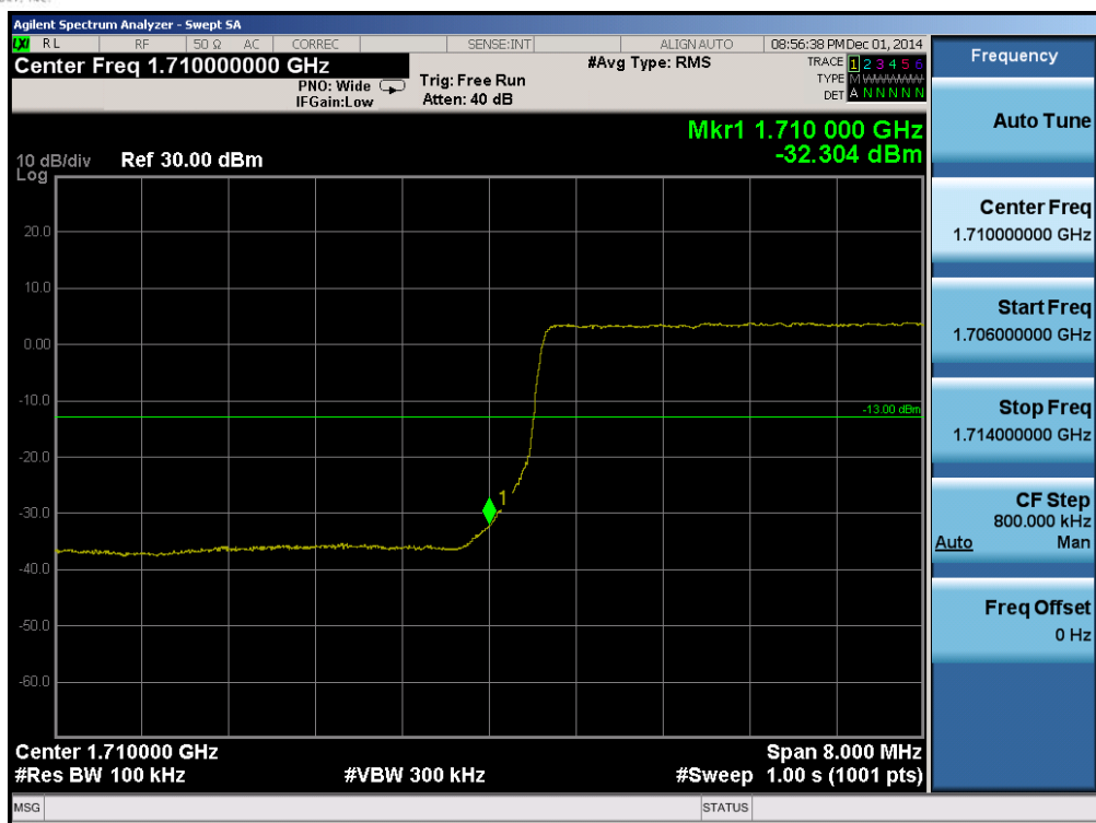
Plot 6-105. Lower Band Edge Plot (Band 4 – 10.0MHz QPSK – RB Size 50)
