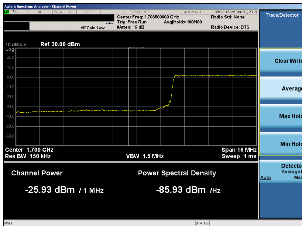
Plot 6-114. Lower Extended Band Edge Plot (Band 4 – 20.0MHz QPSK – RB Size 100)
