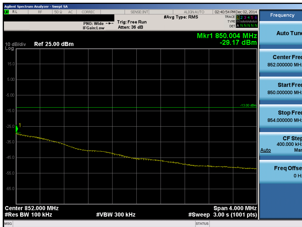
Plot 6-82. Upper Extended Band Edge Plot (Band 5 - 1.4MHz QPSK - RB Size 6)
