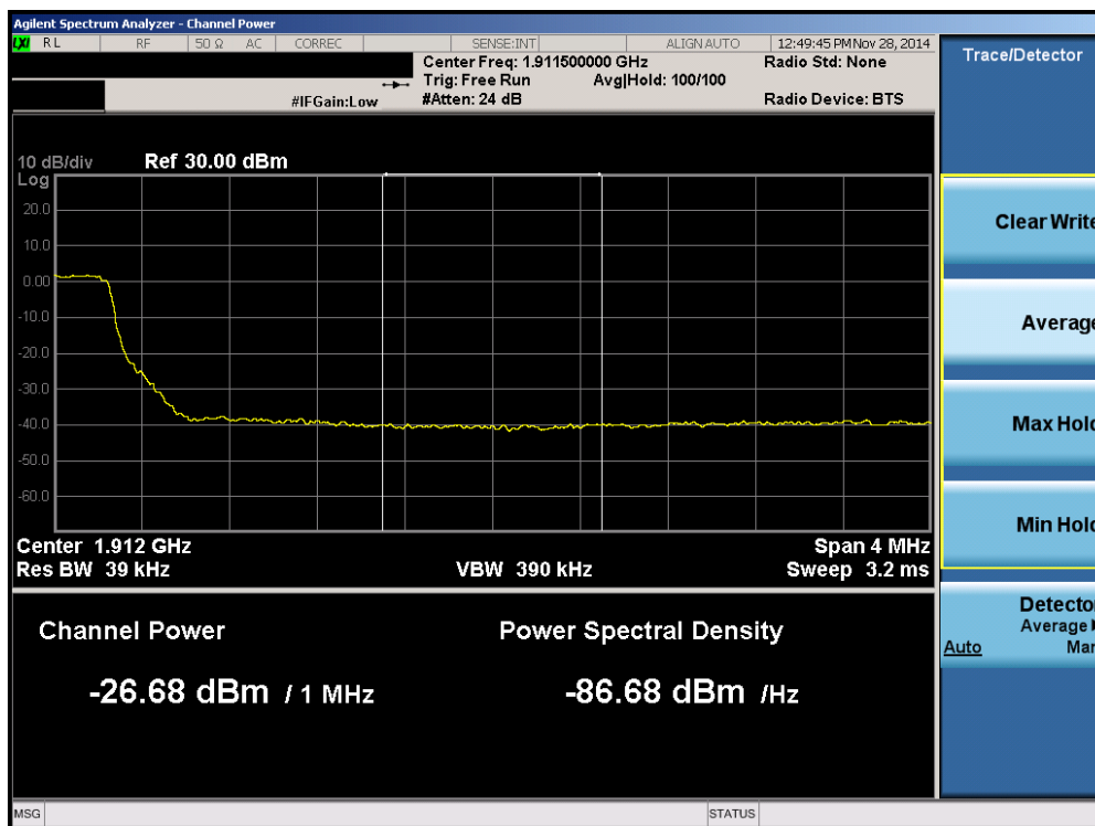
Plot 6-128. Upper Extended Band Edge Plot (Band 2 – 5.0MHz QPSK – RB Size 25)
