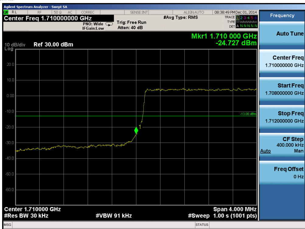
Plot 6-97. Lower Band Edge Plot (Band 4 – 3.0MHz QPSK – RB Size 15)
