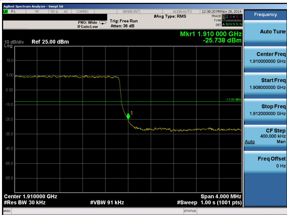
Plot 6-123. Upper Band Edge Plot (Band 2 – 3.0MHz QPSK – RB Size 15)
