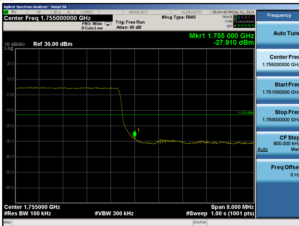
Plot 6-107. Upper Band Edge Plot (Band 4 – 10.0MHz QPSK – RB Size 50)
