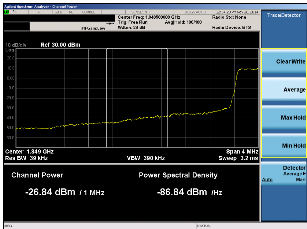
Plot 6-118. Lower Extended Band Edge Plot (Band 2 – 1.4MHz QPSK – RB Size 6)
