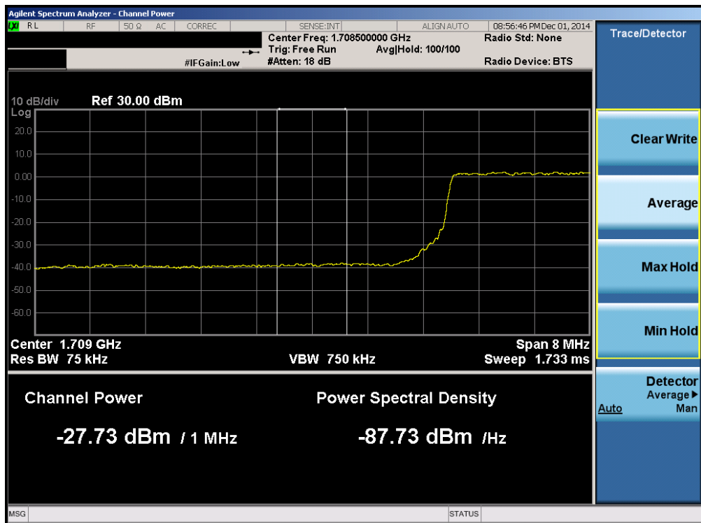
Plot 6-106. Lower Extended Band Edge Plot (Band 4 – 10.0MHz QPSK – RB Size 50)
