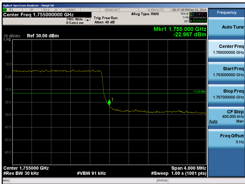
Plot 6-99. Upper Band Edge Plot (Band 4 – 3.0MHz QPSK – RB Size 15)
