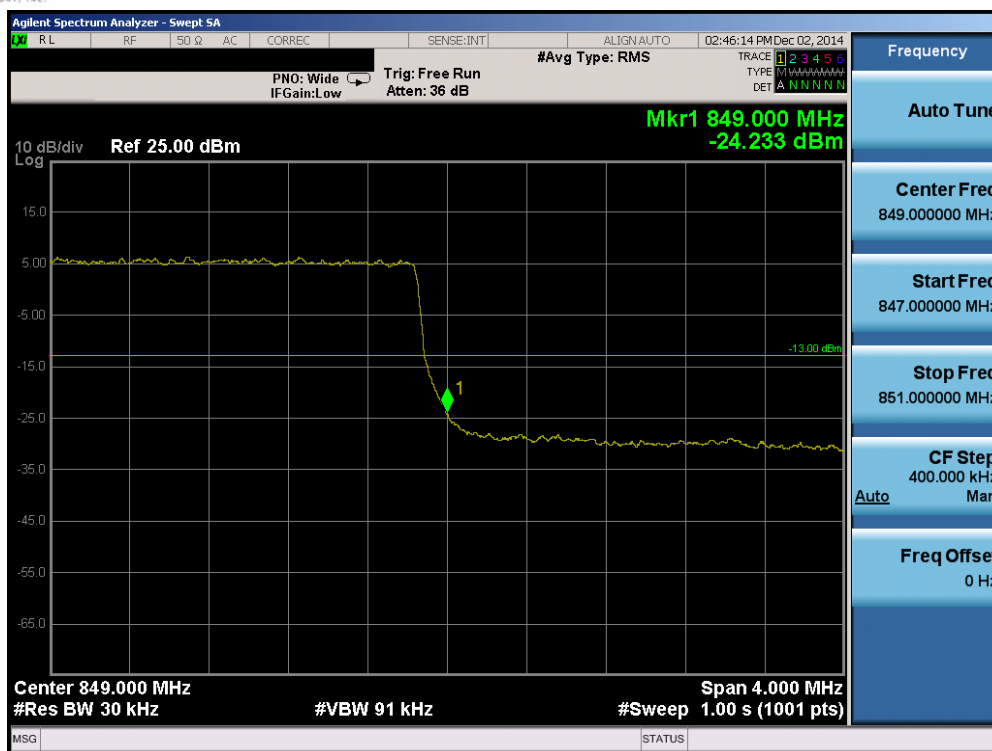
Plot 6-85. Upper Band Edge Plot (Band 5 – 3.0MHz QPSK – RB Size 15)
