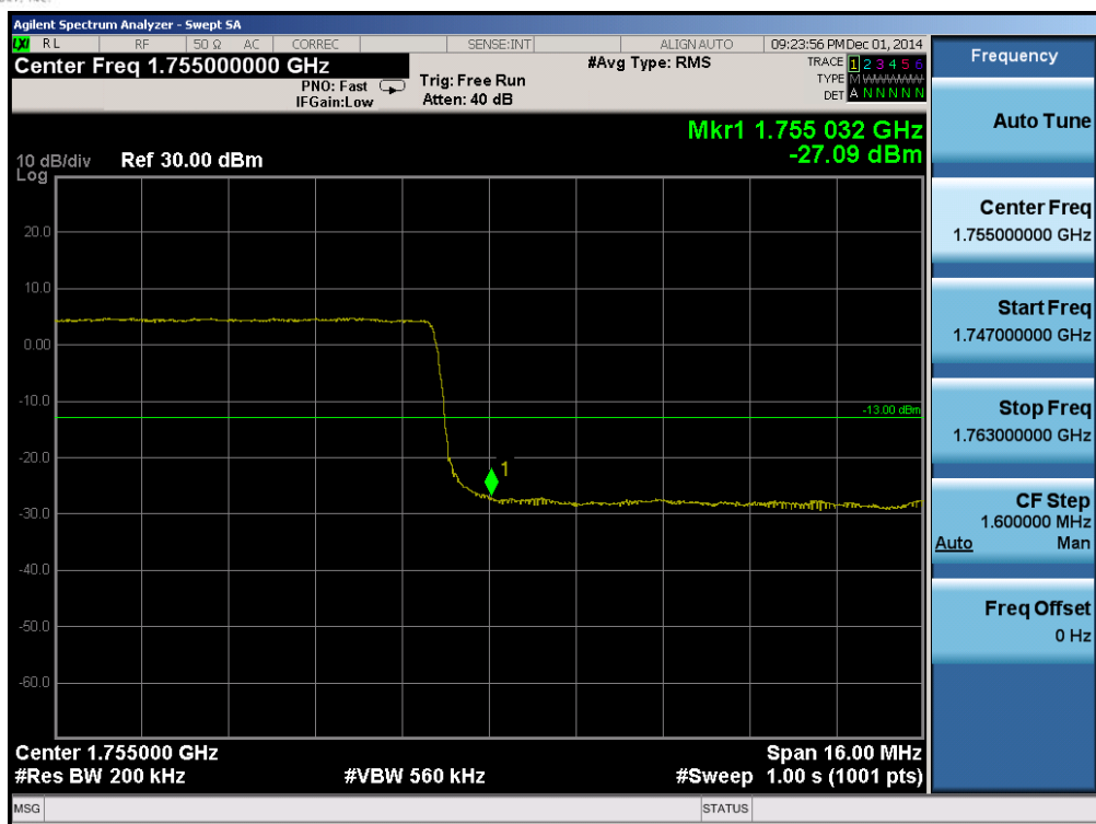
Plot 6-115. Upper Band Edge Plot (Band 4 – 20.0MHz QPSK – RB Size 100)
