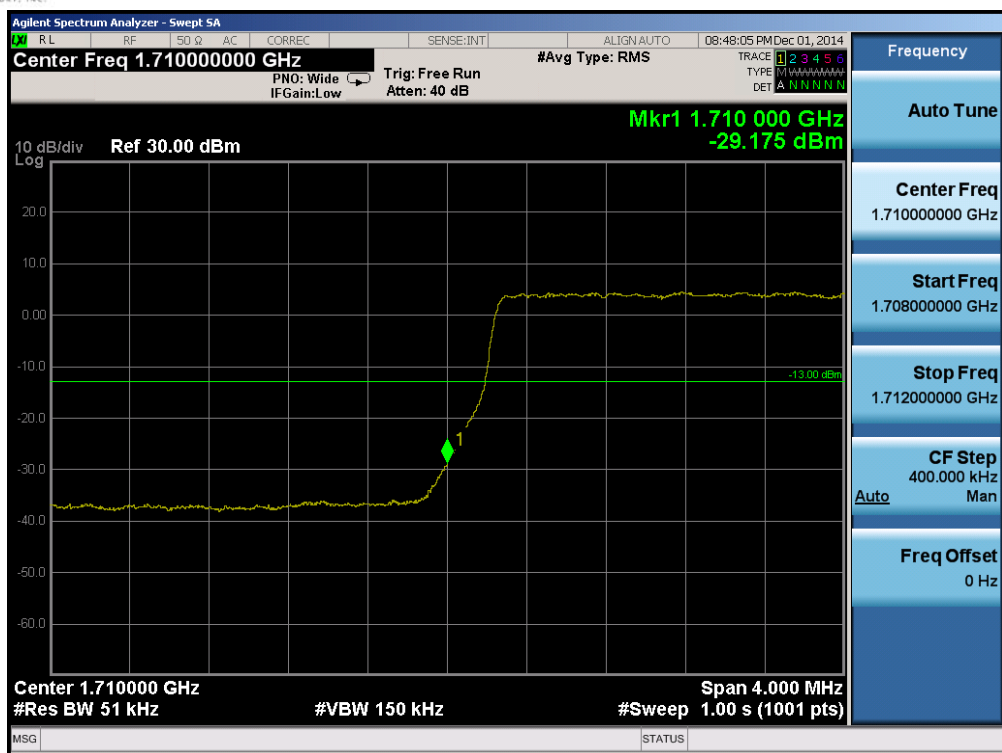
Plot 6-101. Lower Band Edge Plot (Band 4 – 5.0MHz QPSK – RB Size 25)
