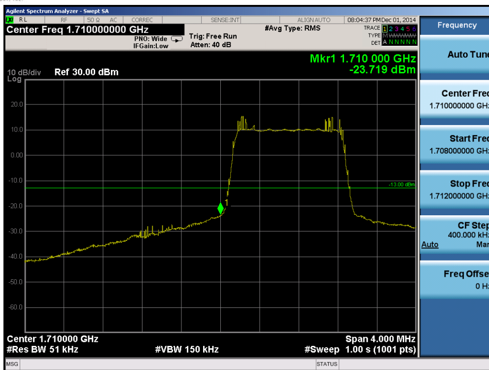
Plot 6-93. Lower Band Edge Plot (Band 4 – 1.4MHz QPSK – RB Size 6)
