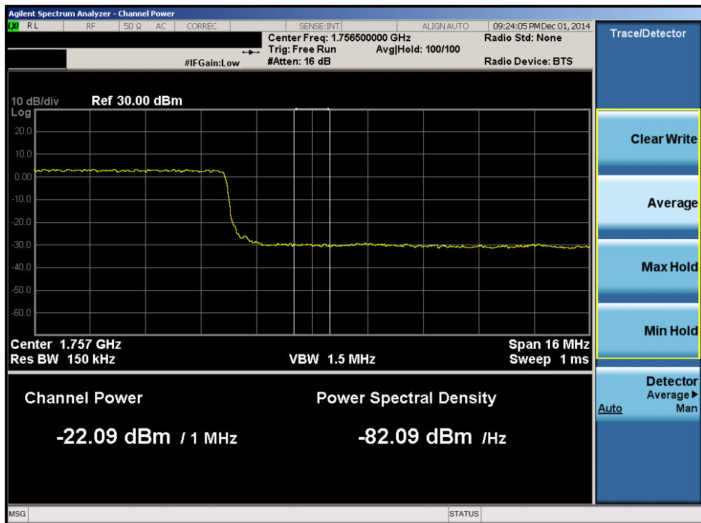
Plot 6-116. Upper Extended Band Edge Plot (Band 4 – 20.0MHz QPSK – RB Size 100)
