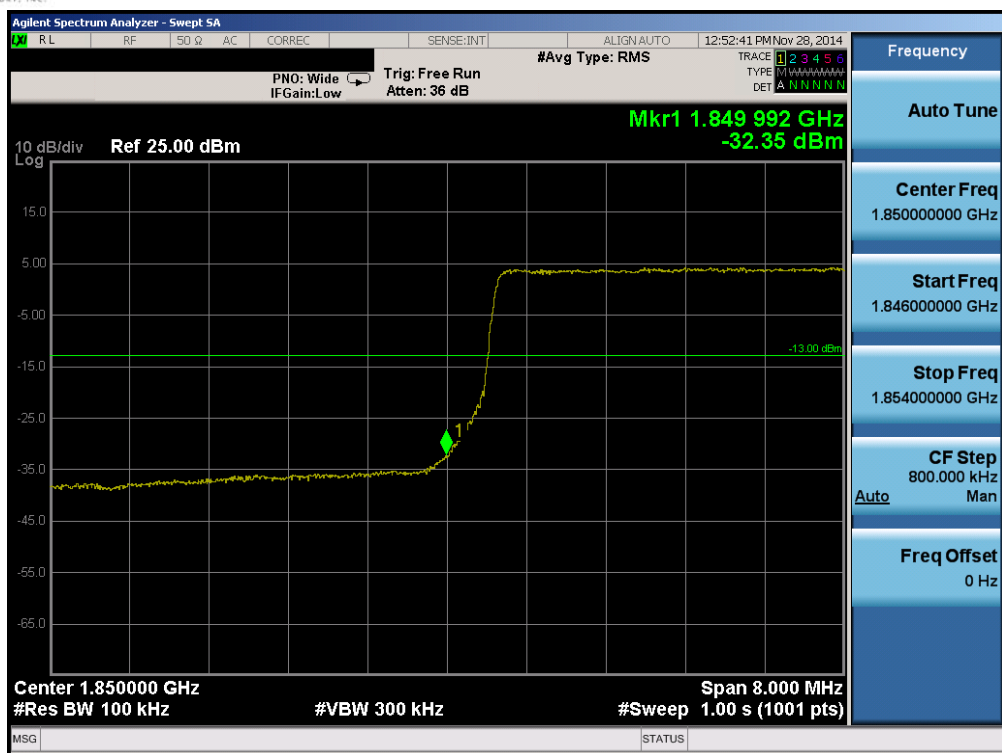
Plot 6-129. Lower Band Edge Plot (Band 2 – 10.0MHz QPSK – RB Size 50)
