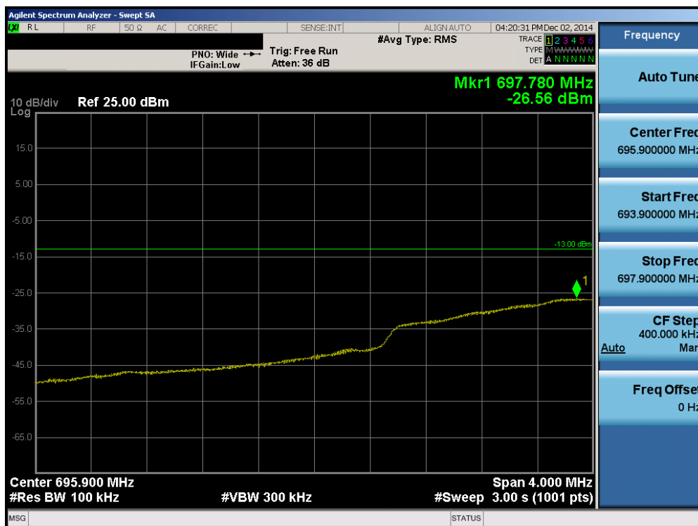
Plot 6-70. Lower Extended Band Edge Plot (Band 12 – 3.0MHz QPSK – RB Size 15)
