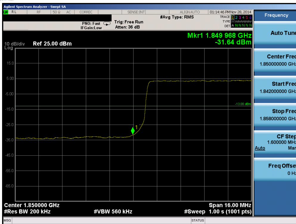
Plot 6-137. Lower Band Edge Plot (Band 2 – 20.0MHz QPSK – RB Size 100)
