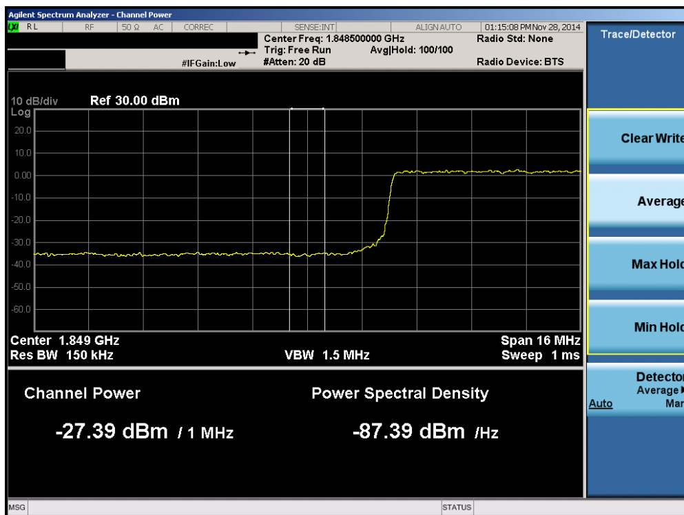
Plot 6-138. Lower Extended Band Edge Plot (Band 2 – 20.0MHz QPSK – RB Size 100)
