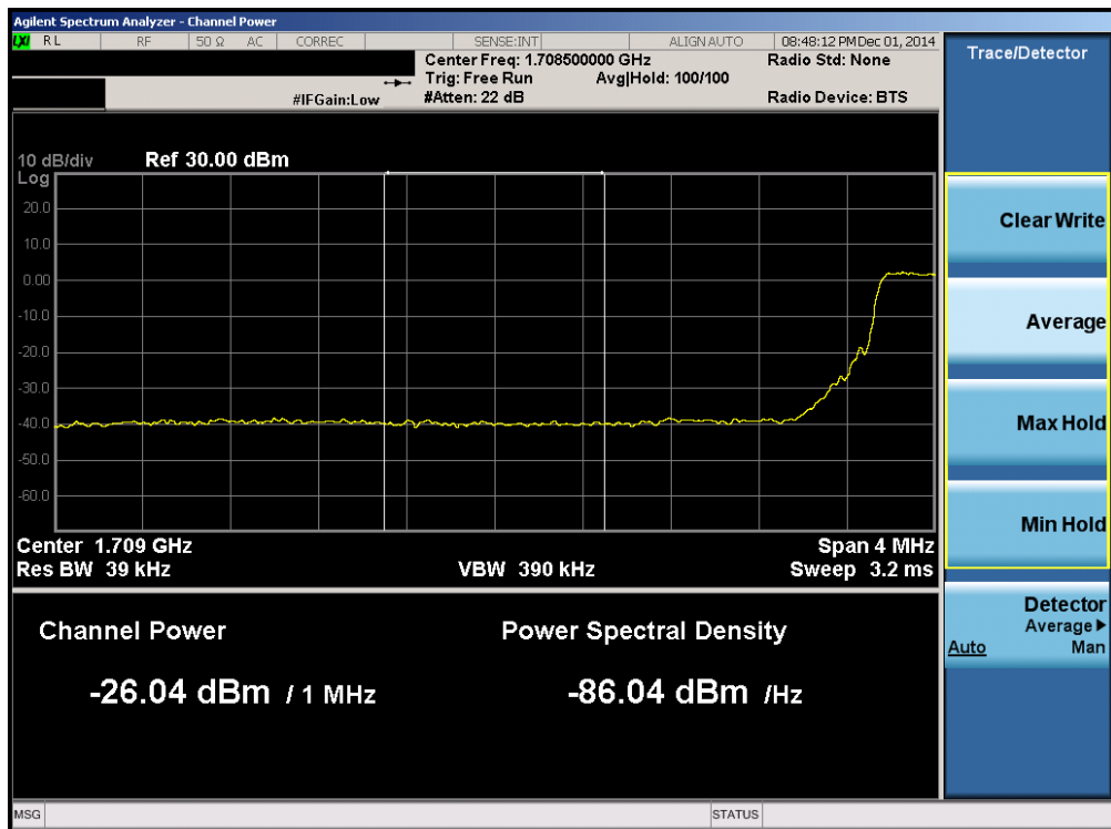
Plot 6-102. Lower Extended Band Edge Plot (Band 4 – 5.0MHz QPSK – RB Size 25)
