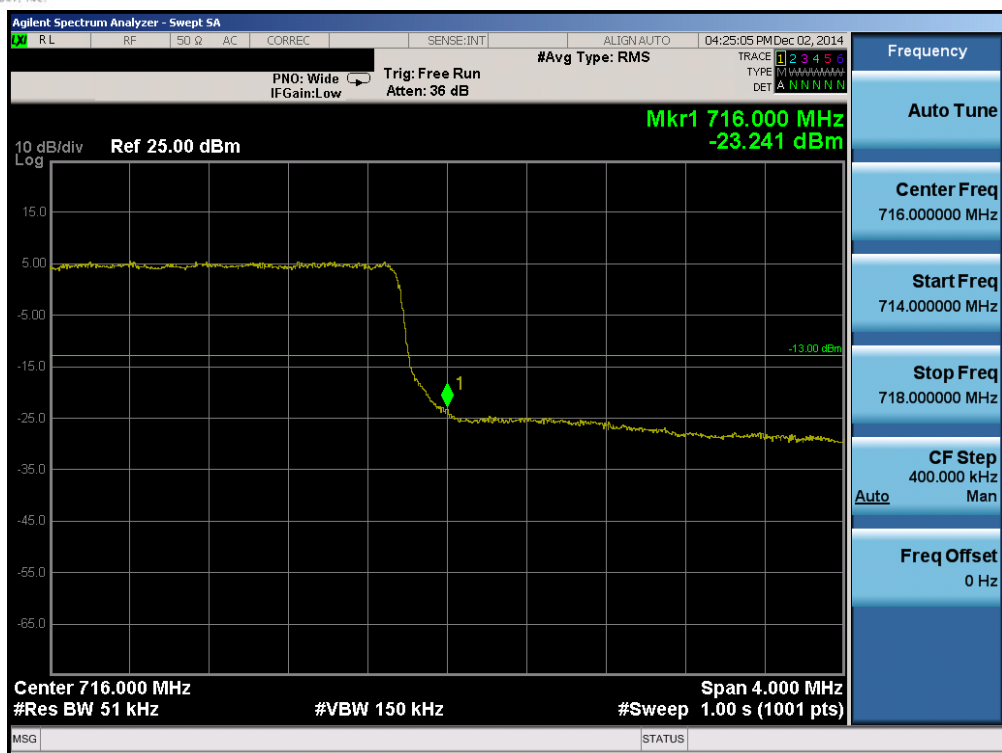
Plot 6-75. Upper Band Edge Plot (Band 12/17 – 5.0MHz QPSK – RB Size 25)
