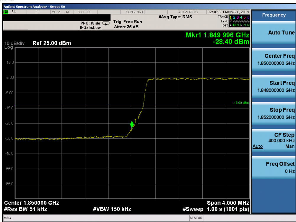
Plot 6-125. Lower Band Edge Plot (Band 2 – 5.0MHz QPSK – RB Size 25)
