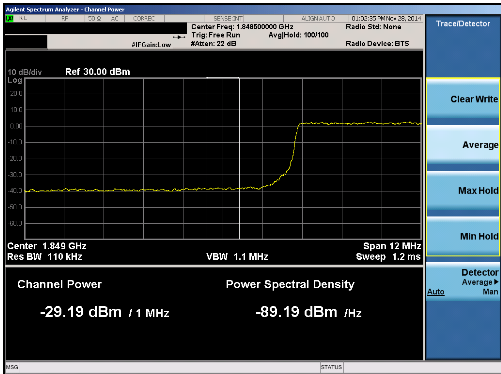
Plot 6-134. Lower Extended Band Edge Plot (Band 2 – 15.0MHz QPSK – RB Size 75)
