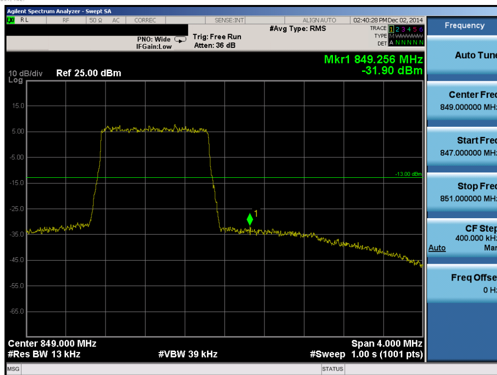
Plot 6-81. Upper Band Edge Plot (Band 5 - 1.4MHz QPSK - RB Size 6)
