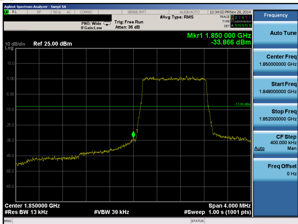
Plot 6-117. Lower Band Edge Plot (Band 2 – 1.4MHz QPSK – RB Size 6)
