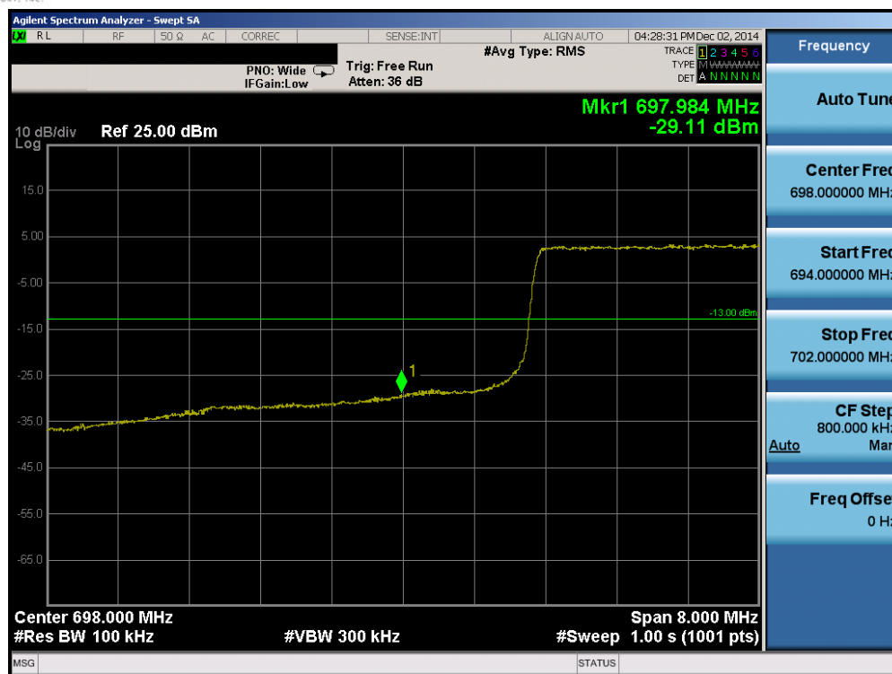
Plot 6-77. Lower Band Edge Plot (Band 12/17 – 10.0MHz QPSK – RB Size 50)
