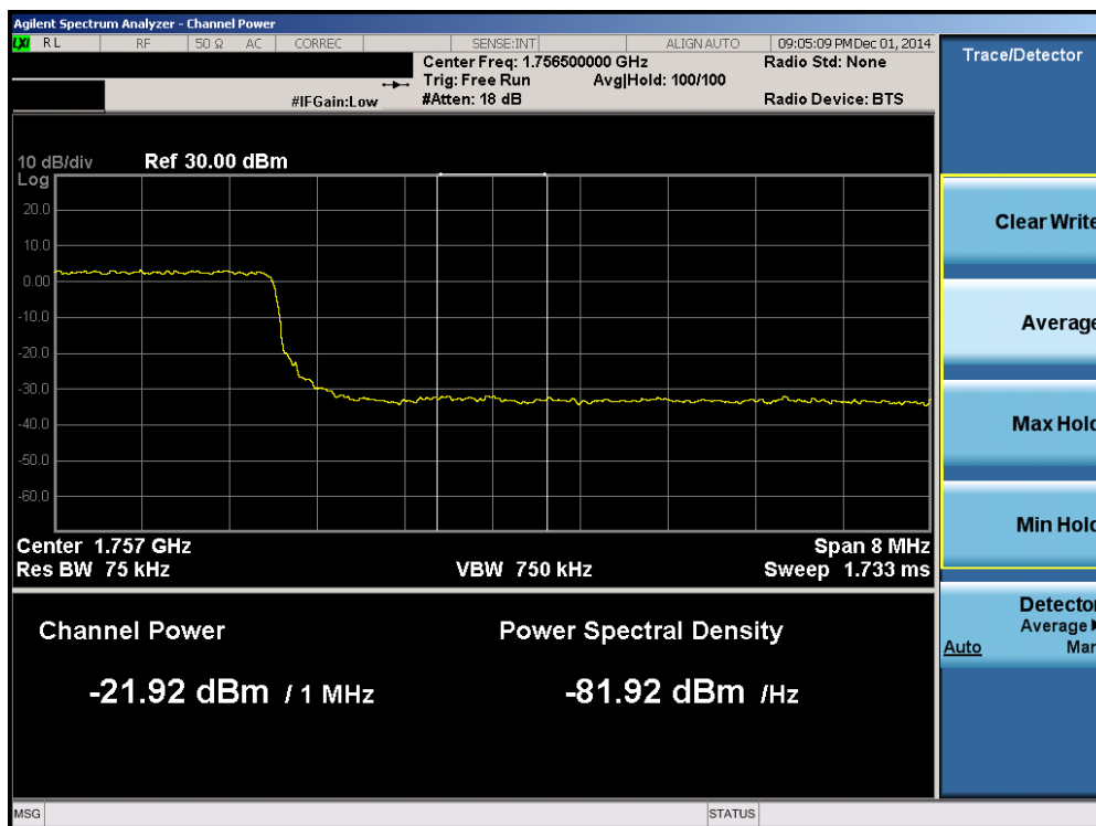
Plot 6-108. Upper Extended Band Edge Plot (Band 4 – 10.0MHz QPSK – RB Size 50)
