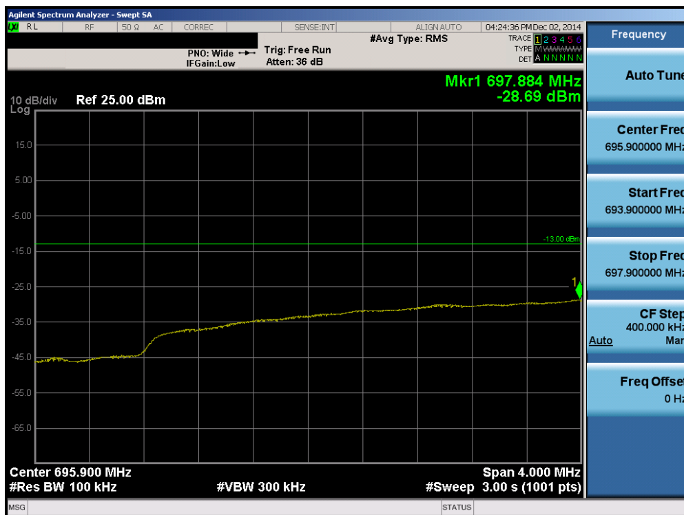
Plot 6-74. Lower Extended Band Edge Plot (Band 12/17 – 5.0MHz QPSK – RB Size 25)
