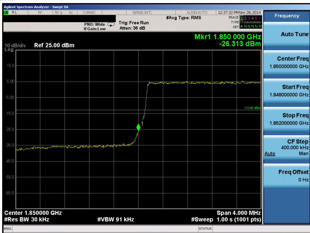
Plot 6-121. Lower Band Edge Plot (Band 2 – 3.0MHz QPSK – RB Size 15)
