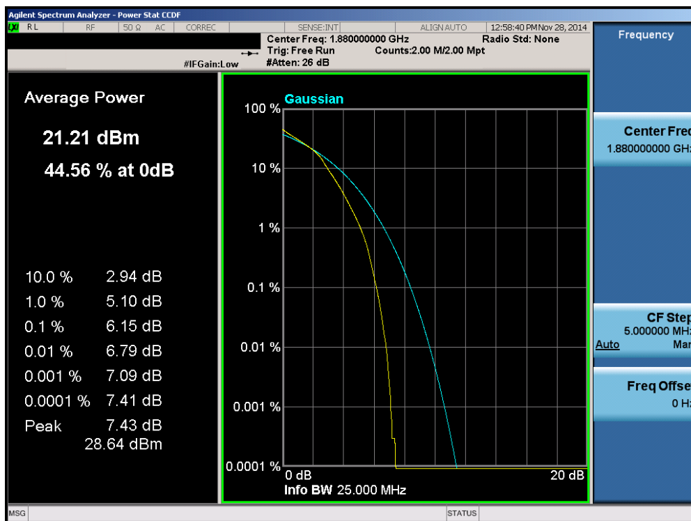
Plot 6-150. PAR Plot (Band 2 – 15.0MHz 16-QAM – RB Size 75)
