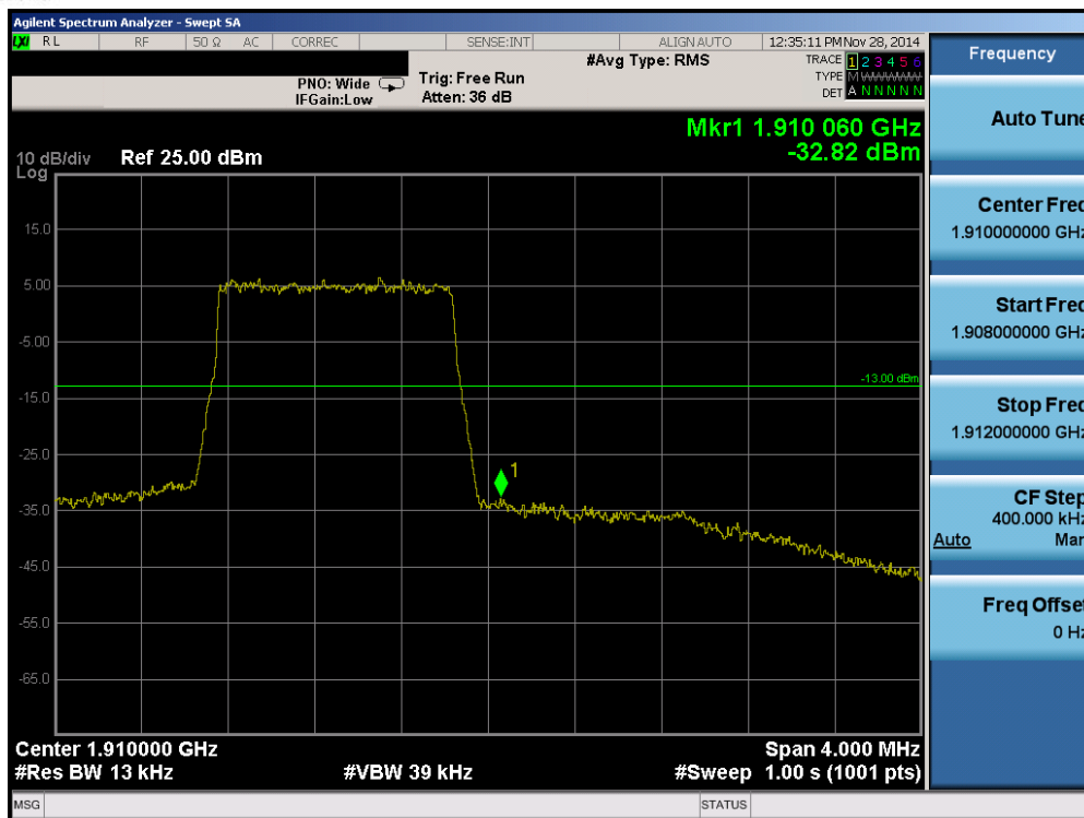
Plot 6-119. Upper Band Edge Plot (Band 2 – 1.4MHz QPSK – RB Size 6)
