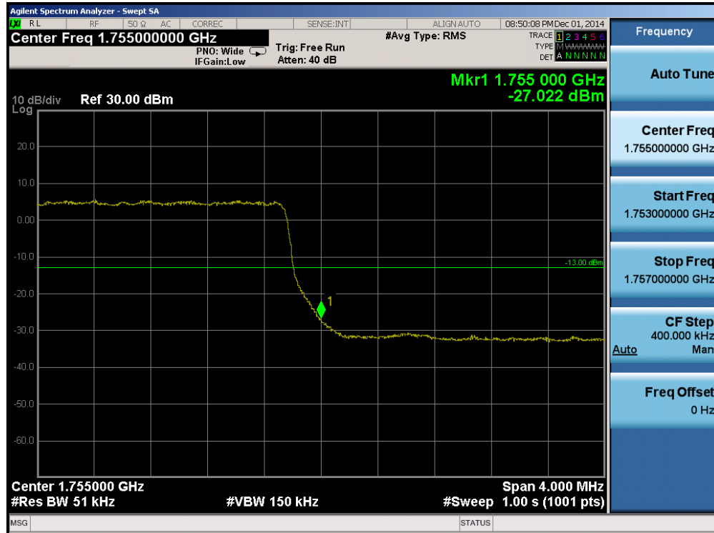
Plot 6-103. Upper Band Edge Plot (Band 4 – 5.0MHz QPSK – RB Size 25)
