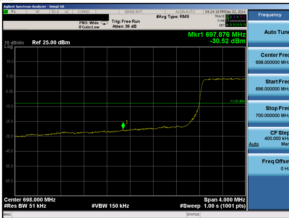
Plot 6-73. Lower Band Edge Plot (Band 12/17 – 5.0MHz QPSK – RB Size 25)
