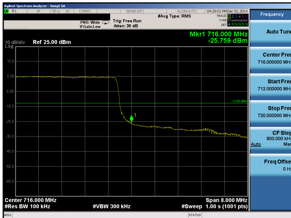
Plot 6-78. Upper Band Edge Plot (Band 12/17 – 10.0MHz QPSK – RB Size 50)
