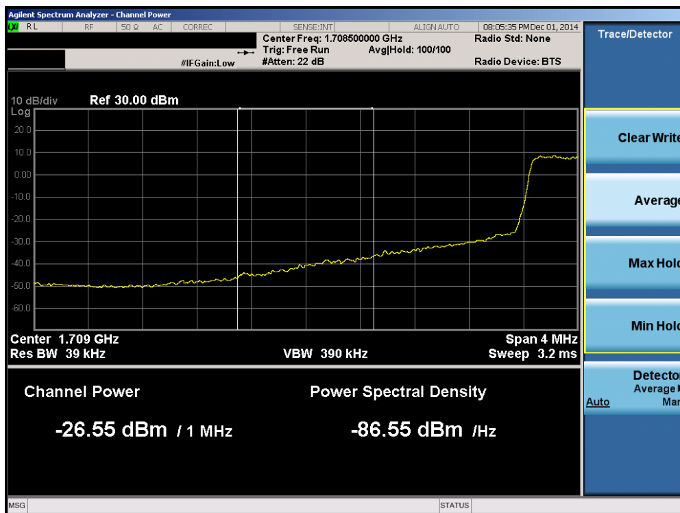
Plot 6-94. Lower Extended Band Edge Plot (Band 4 – 1.4MHz QPSK – RB Size 6)
