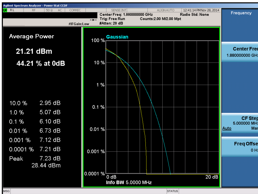
Plot 6-146. PAR Plot (Band 2 – 5.0MHz 16-QAM – RB Size 25)
