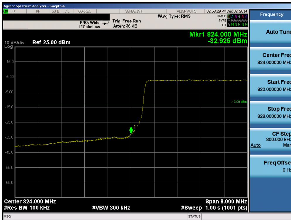
Plot 6-91. Lower Band Edge Plot (Band 5 – 10.0MHz QPSK – RB Size 50)
