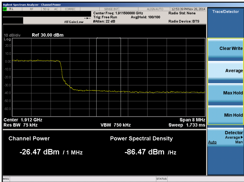
Plot 6-132. Upper Extended Band Edge Plot (Band 2 – 10.0MHz QPSK – RB Size 50)
