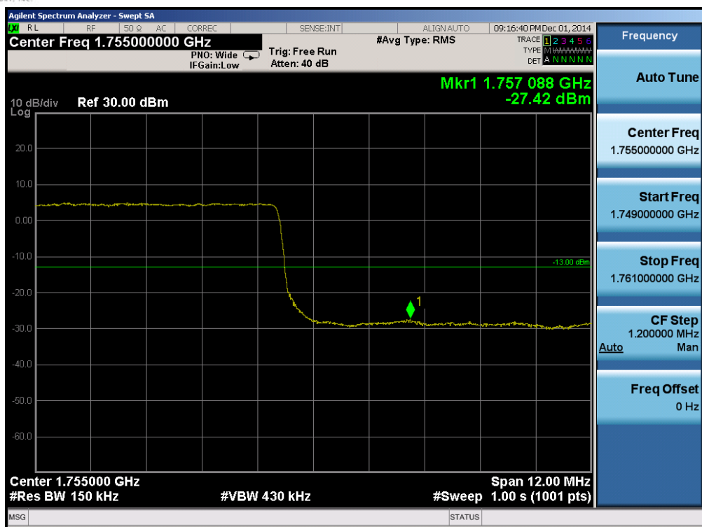
Plot 6-111. Upper Band Edge Plot (Band 4 – 15.0MHz QPSK – RB Size 75)
