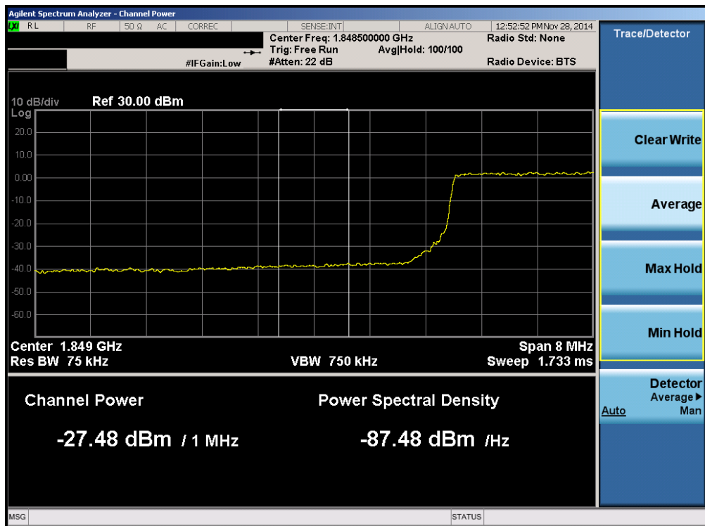
Plot 6-130. Lower Extended Band Edge Plot (Band 2 – 10.0MHz QPSK – RB Size 50)
