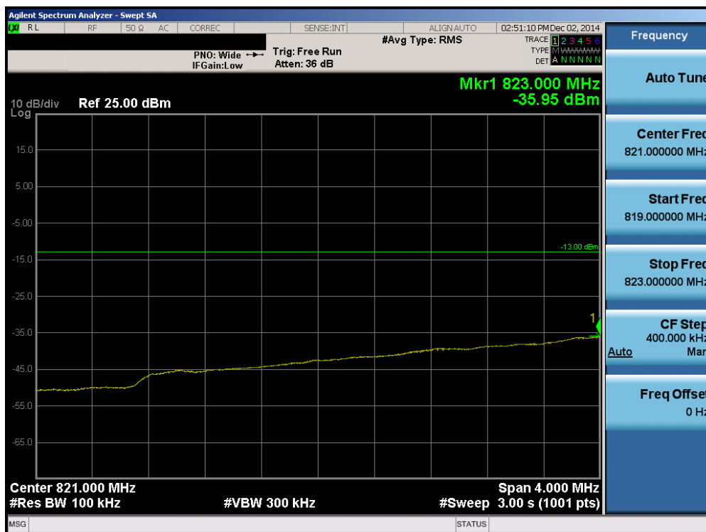
Plot 6-88. Lower Extended Band Edge Plot (Band 5 – 5.0MHz QPSK – RB Size 25)
