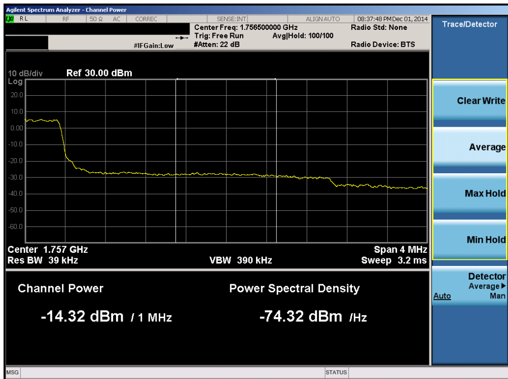
Plot 6-100. Upper Extended Band Edge Plot (Band 4 – 3.0MHz QPSK – RB Size 15)
