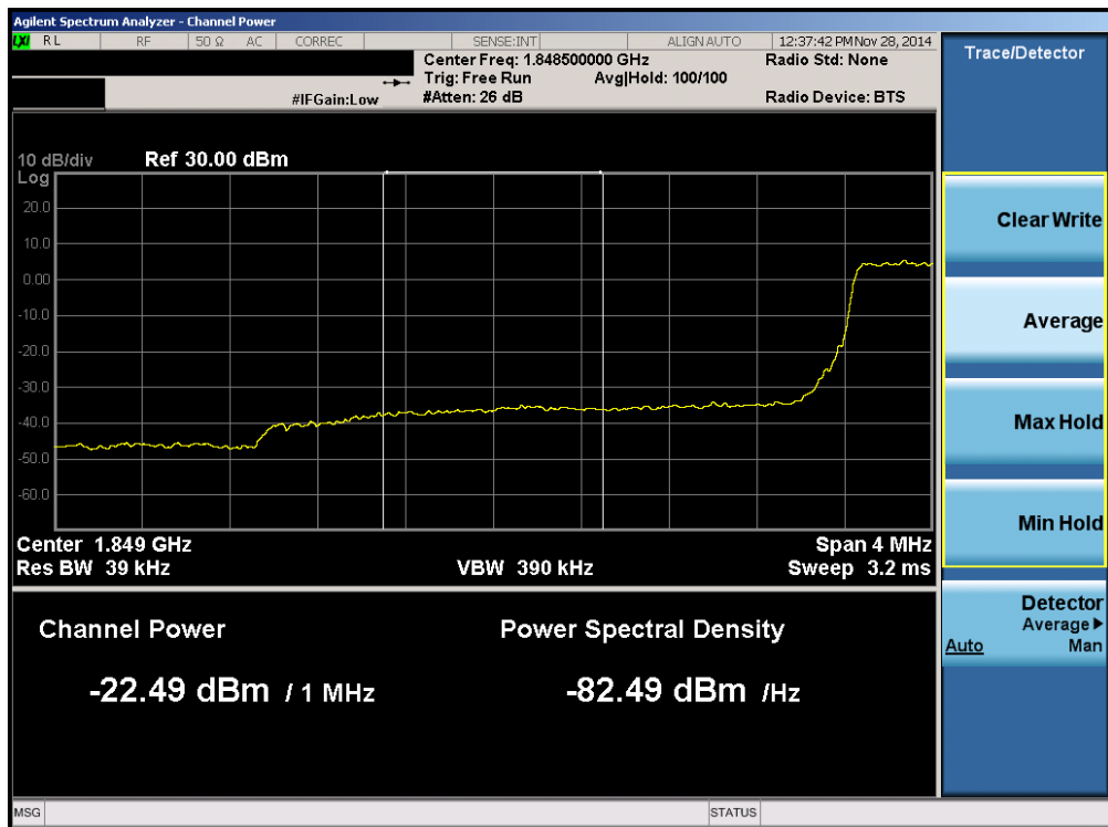
Plot 6-122. Lower Extended Band Edge Plot (Band 2 – 3.0MHz QPSK – RB Size 15)
