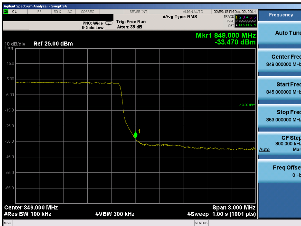
Plot 6-92. Upper Band Edge Plot (Band 5 – 10.0MHz QPSK – RB Size 50)
