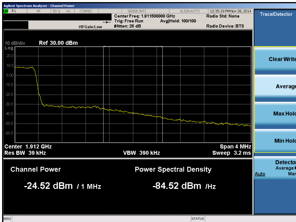
Plot 6-120. Upper Extended Band Edge Plot (Band 2 – 1.4MHz QPSK – RB Size 6)
