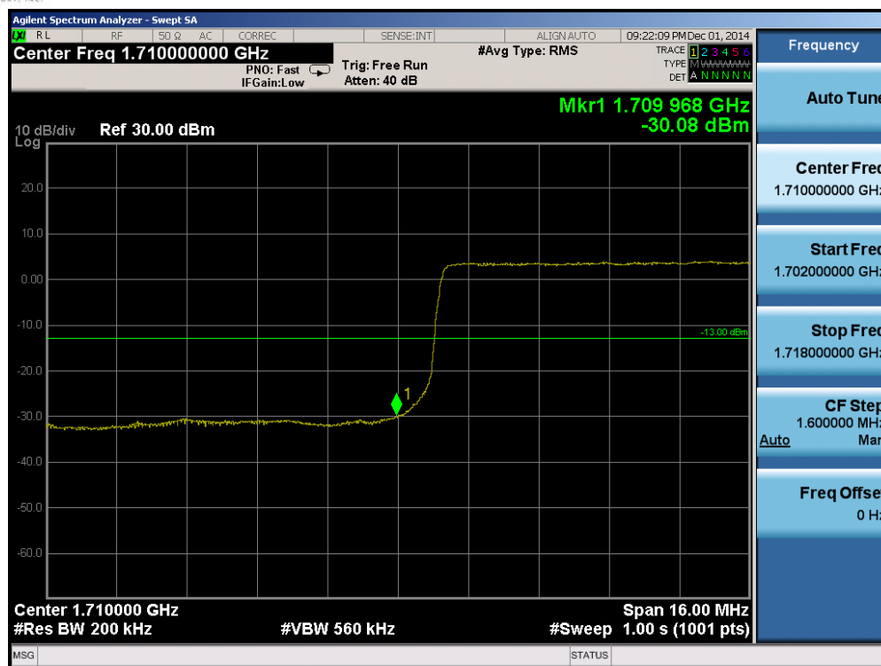
Plot 6-113. Lower Band Edge Plot (Band 4 – 20.0MHz QPSK – RB Size 100)
