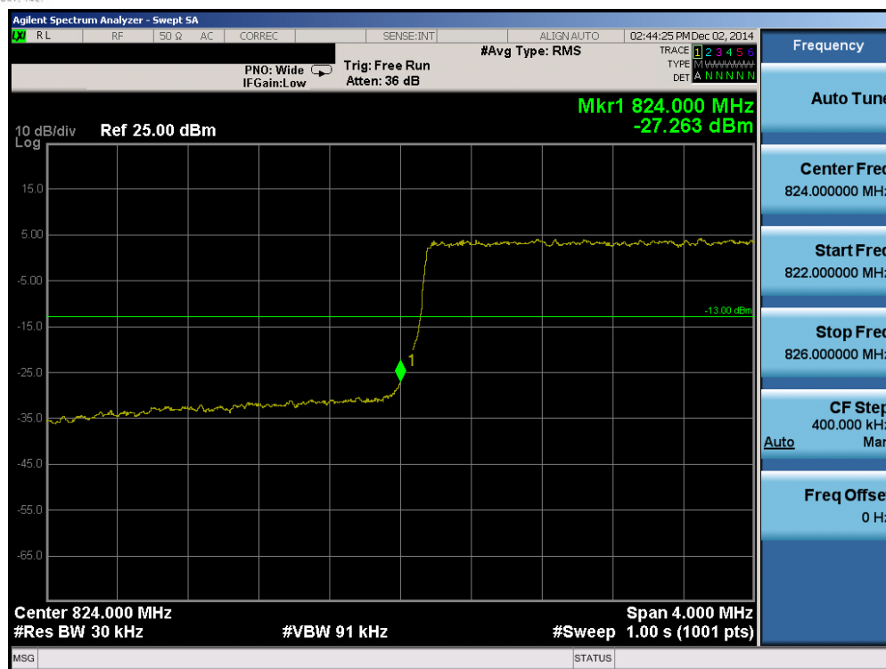
Plot 6-83. Lower Band Edge Plot (Band 5 – 3.0MHz QPSK – RB Size 15)
