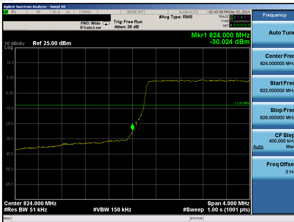
Plot 6-87. Lower Band Edge Plot (Band 5 – 5.0MHz QPSK – RB Size 25)
