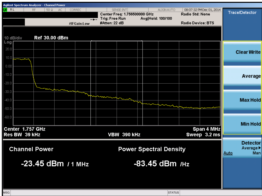
Plot 6-96. Upper Extended Band Edge Plot (Band 4 – 1.4MHz QPSK – RB Size 6)
