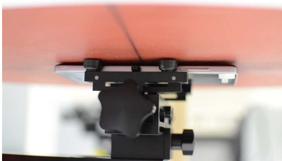
SAR Test Setup Photo 6 – Back at 0.0 cm
