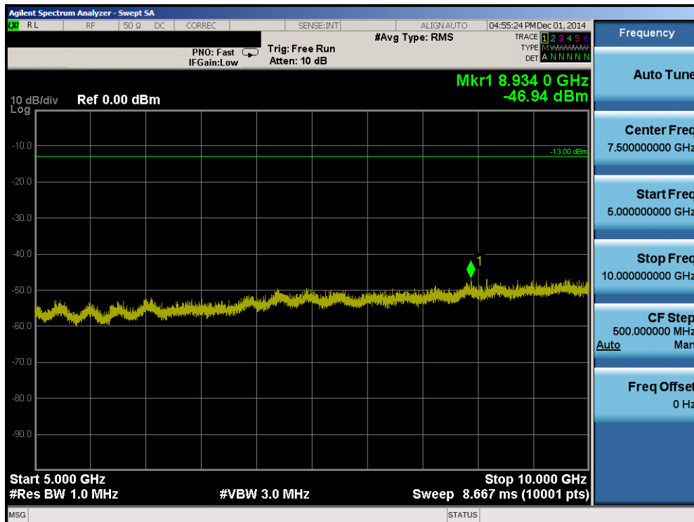
Plot 6-18. Conducted Spurious Plot (Band 17 – 10.0MHz QPSK – RB Size 1, RB Offset 0 – High Channel)
