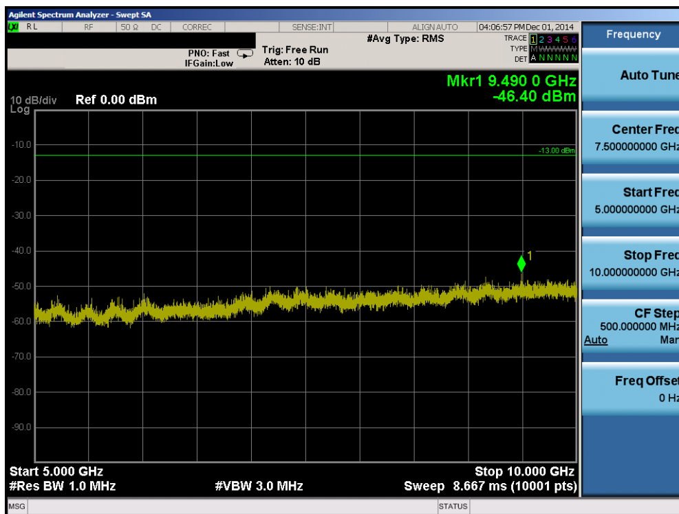
Plot 6-20. Conducted Spurious Plot (Band 5 – 10.0MHz QPSK – RB Size 1, RB Offset 0 – Low Channel)
