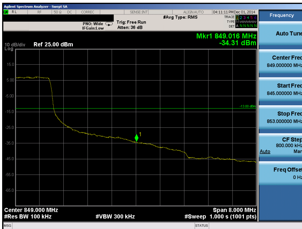
Plot 6-44. Upper Band Edge Plot (Band 5 – 10.0MHz QPSK – RB Size 50)
