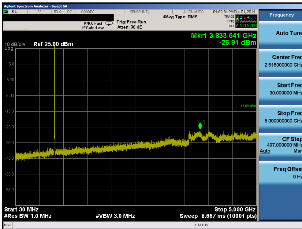
Plot 6-23. Conducted Spurious Plot (Band 5 – 10.0MHz QPSK – RB Size 1, RB Offset 0 – High Channel)
