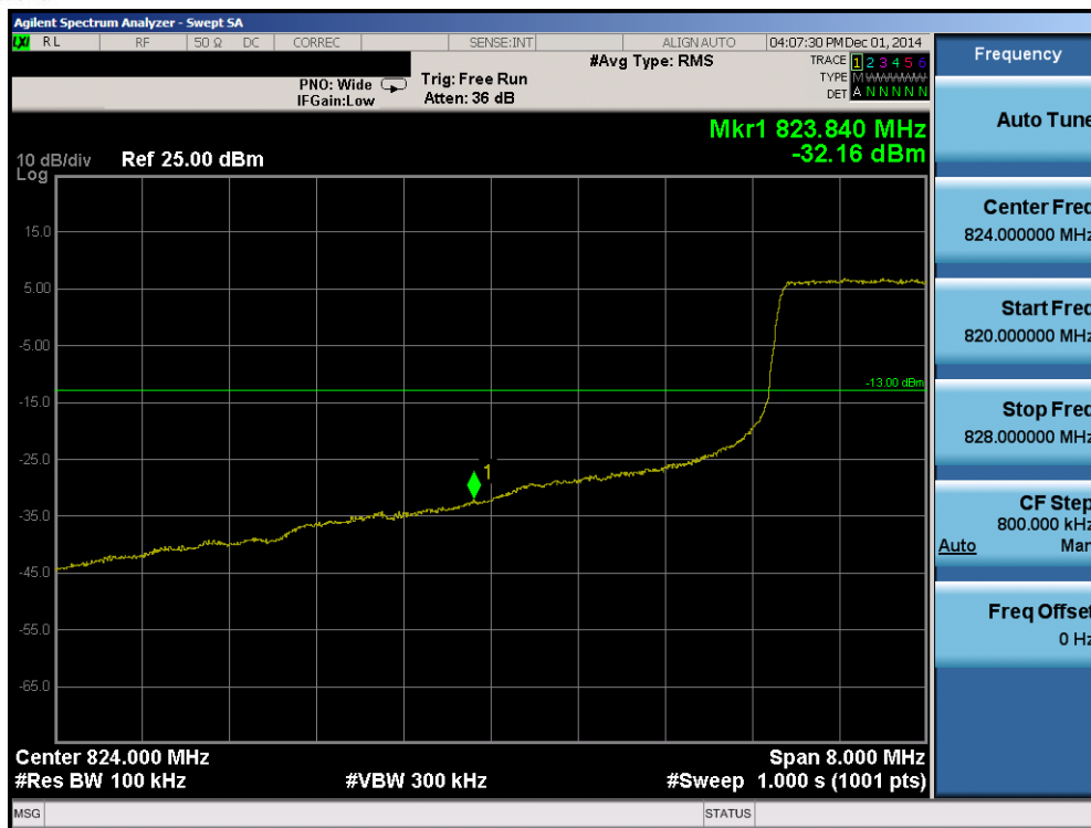
Plot 6-43. Lower Band Edge Plot (Band 5 – 10.0MHz QPSK – RB Size 50)
