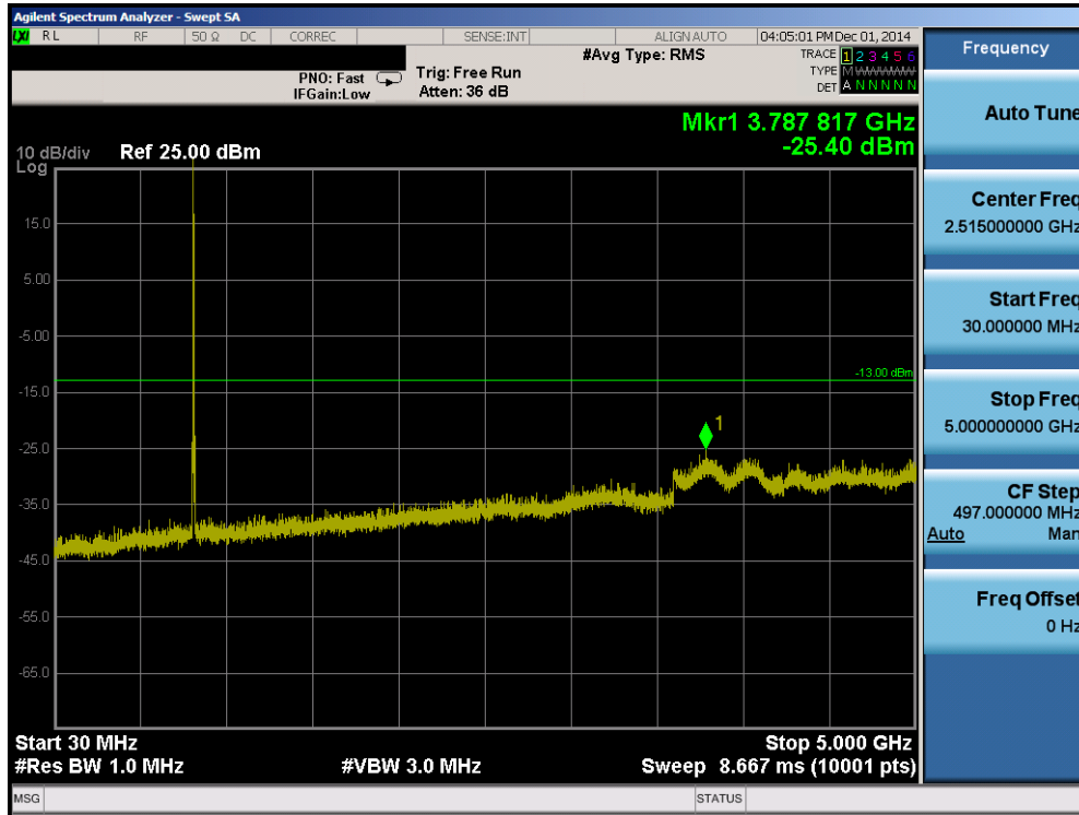
Plot 6-21. Conducted Spurious Plot (Band 5 – 10.0MHz QPSK – RB Size 1, RB Offset 0 – Mid Channel)
