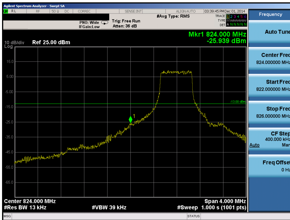
Plot 6-31. Lower Band Edge Plot (Band 5 – 1.4MHz QPSK – RB Size 6)
