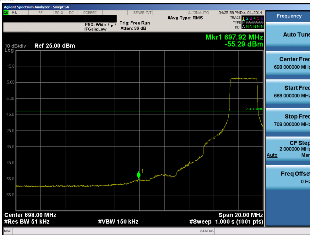
Plot 6-25. Lower Band Edge Plot (Band 17 – 5.0MHz QPSK – RB Size 25)
