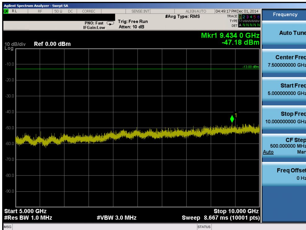
Plot 6-16. Conducted Spurious Plot (Band 17 – 10.0MHz QPSK – RB Size 1, RB Offset 0 – Mid Channel)
