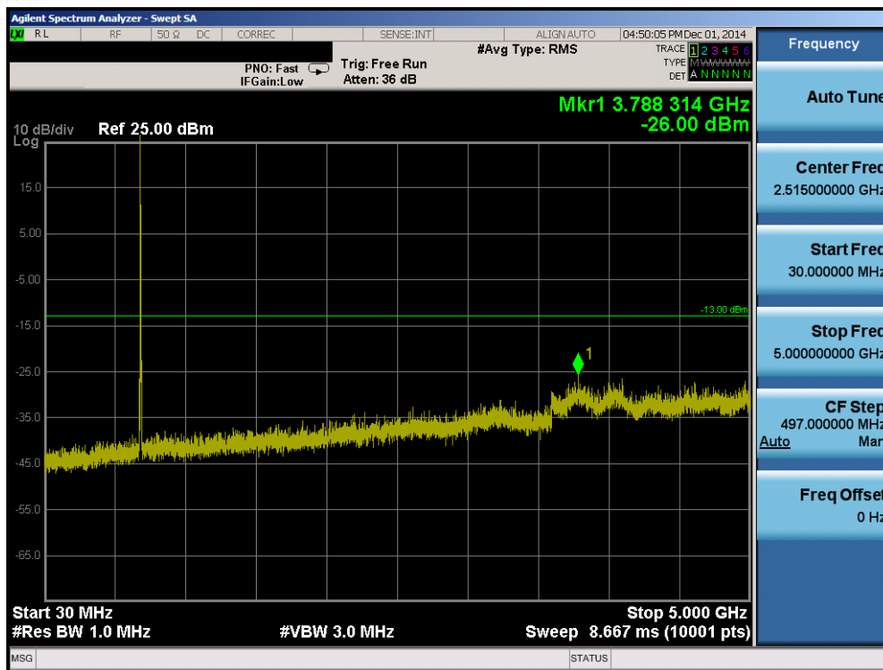
Plot 6-13. Conducted Spurious Plot (Band 17 – 10.0MHz QPSK – RB Size 1, RB Offset 0– Low Channel)
