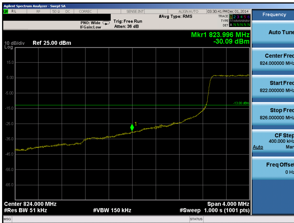
Plot 6-39. Lower Band Edge Plot (Band 5 – 5.0MHz QPSK – RB Size 25)
