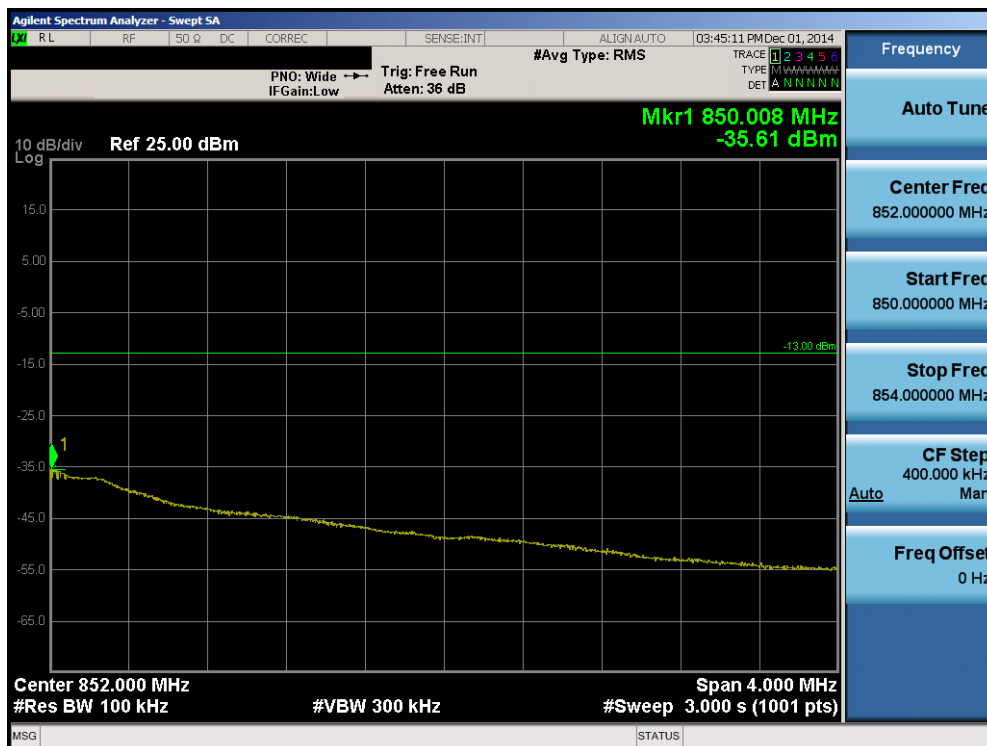
Plot 6-34. Upper Extended Band Edge Plot (Band 5 – 1.4MHz QPSK – RB Size 6)
