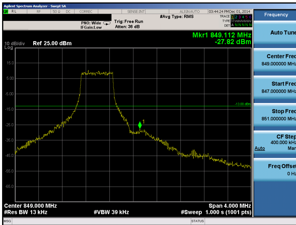
Plot 6-33. Upper Band Edge Plot (Band 5 – 1.4MHz QPSK – RB Size 6)
