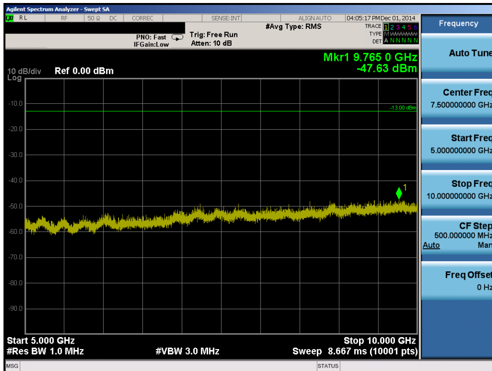
Plot 6-22. Conducted Spurious Plot (Band 5 – 10.0MHz QPSK – RB Size 1, RB Offset 0 – Mid Channel)
