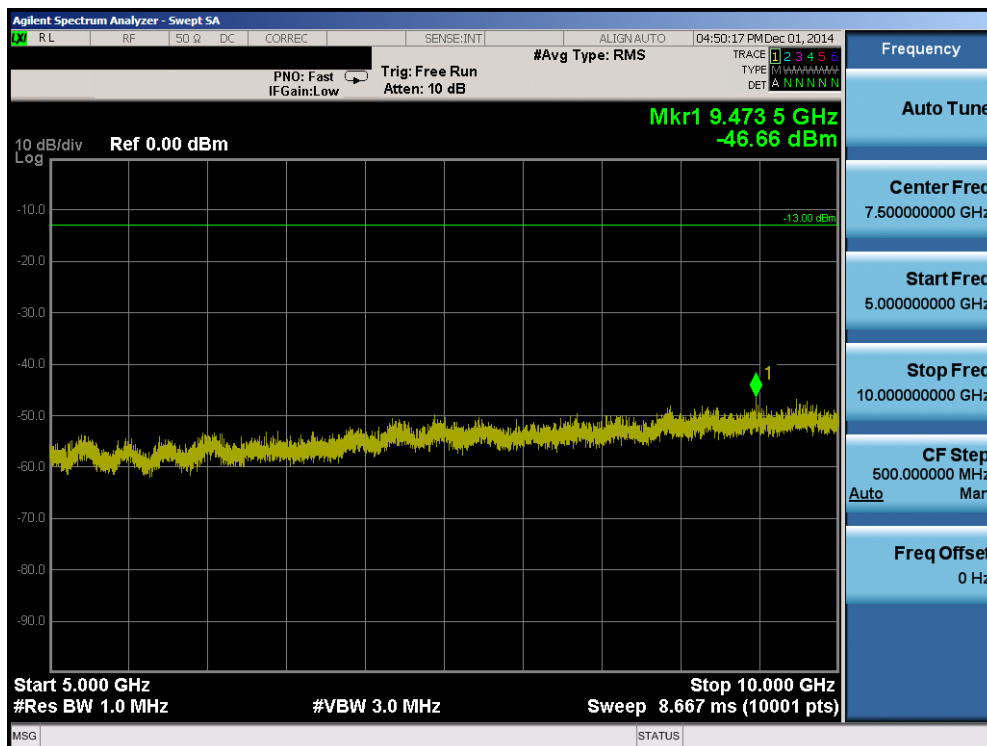
Plot 6-14. Conducted Spurious Plot (Band 17 – 10.0MHz QPSK – RB Size 1, RB Offset 0 – Low Channel)
