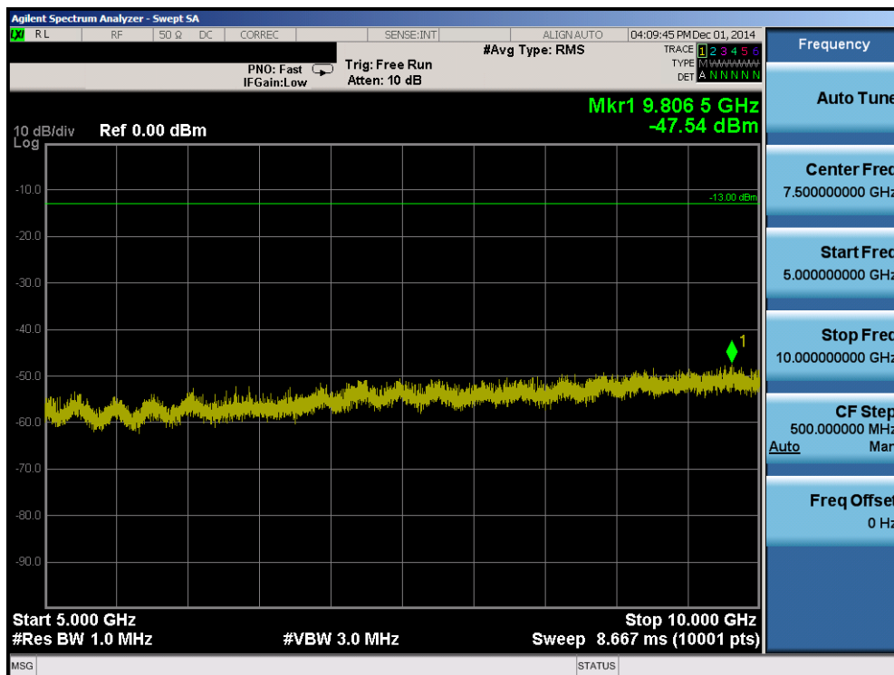
Plot 6-24. Conducted Spurious Plot (Band 5 – 10.0MHz QPSK – RB Size 1, RB Offset 0 – High Channel)
