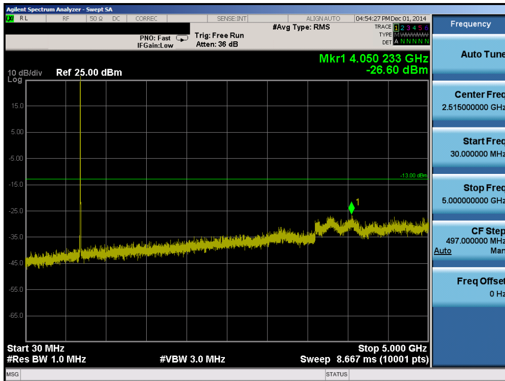
Plot 6-17. Conducted Spurious Plot (Band 17 – 10.0MHz QPSK – RB Size 1, RB Offset 0 – High Channel)
