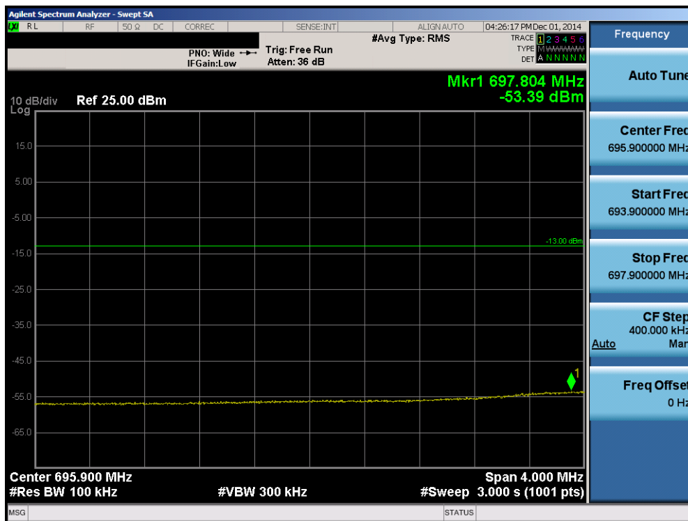
Plot 6-26. Lower Extended Band Edge Plot (Band 17 – 5.0MHz QPSK – RB Size 25)
