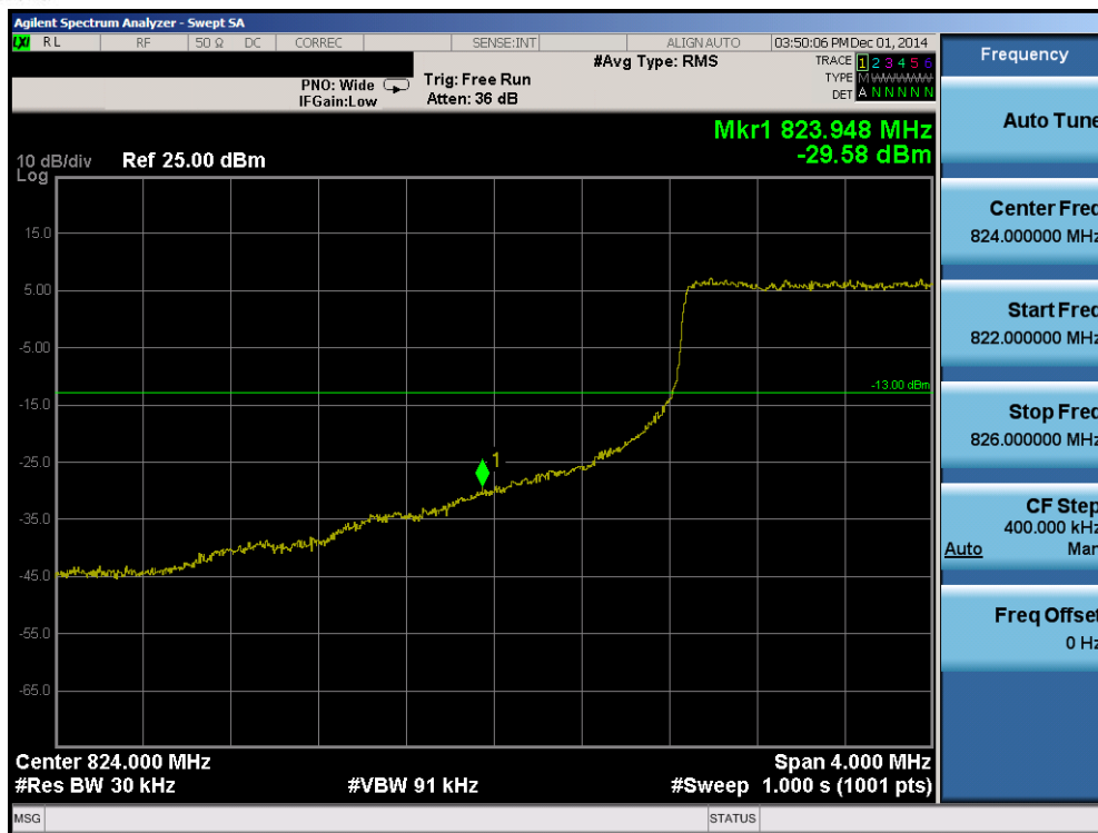
Plot 6-35. Lower Band Edge Plot (Band 5 - 3.0MHz QPSK - RB Size 15)
