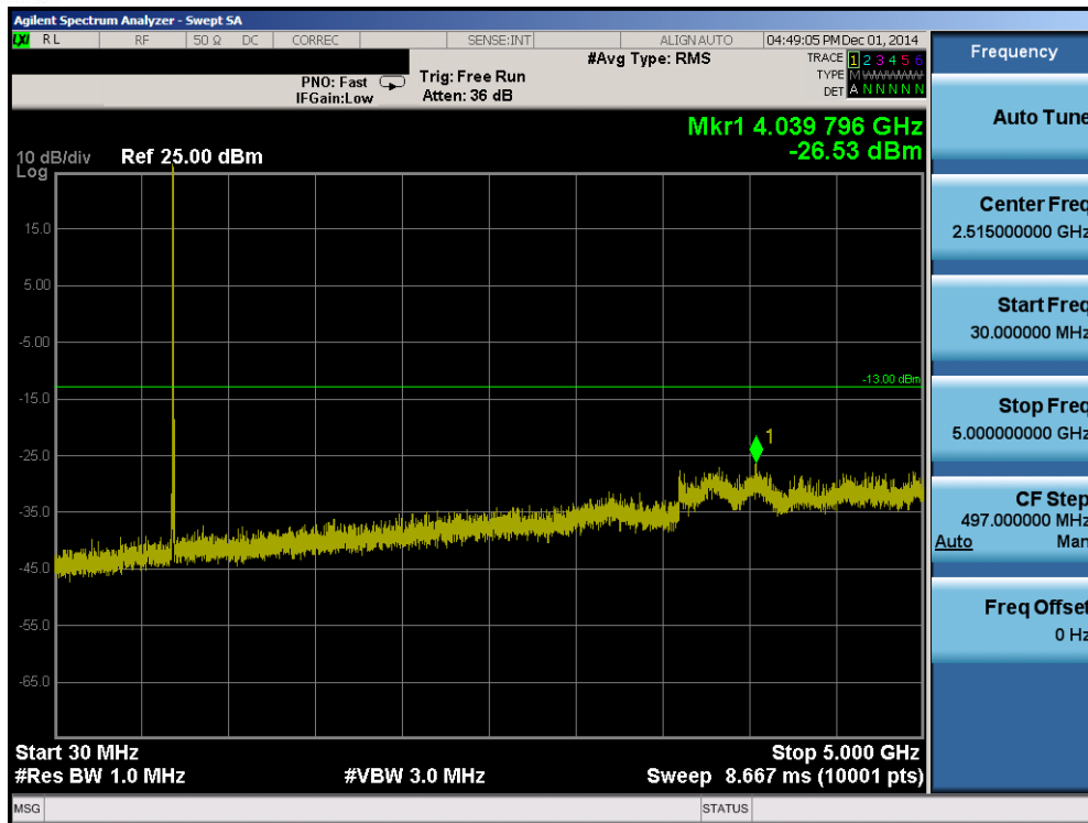
Plot 6-15. Conducted Spurious Plot (Band 17 – 10.0MHz QPSK – RB Size 1, RB Offset 0 – Mid Channel)
