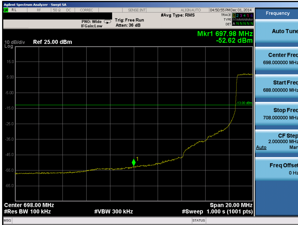
Plot 6-29. Lower Band Edge Plot (Band 17 – 10.0MHz QPSK – RB Size 50)
