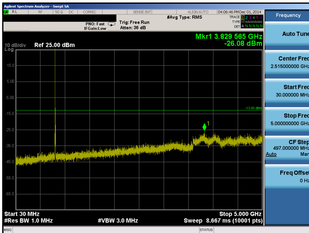
Plot 6-19. Conducted Spurious Plot (Band 5 – 10.0MHz QPSK – RB Size 1, RB Offset 0– Low Channel)
