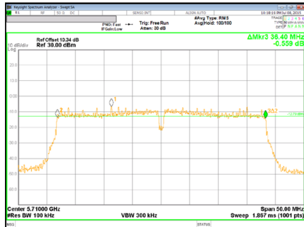
11n HT40 Mode Straddle Channel Chain 1
