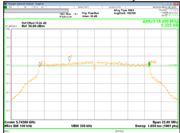
11a Mode Low Channel Secondary
