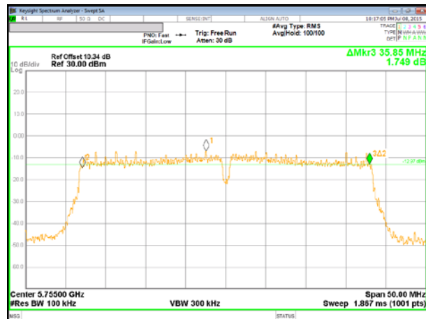
11n HT40 Mode Low Channel Chain 1
