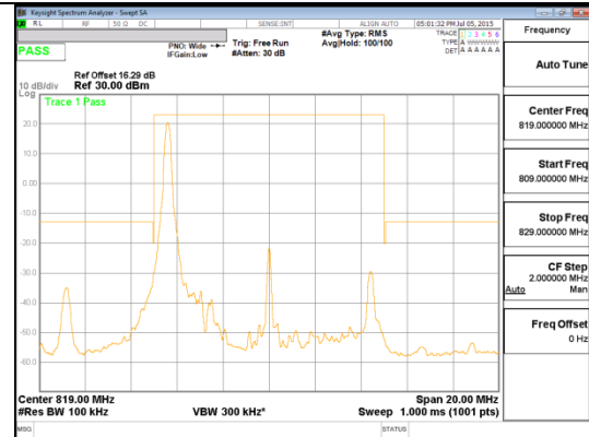
QPSK Mid channel 1RB (Offset 0)
