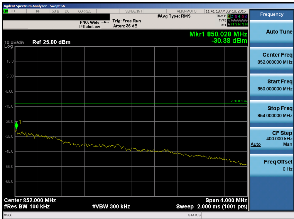
Plot 6-102. Upper Extended Band Edge Plot (Band 5 – 1.4MHz QPSK – RB Size 6)
