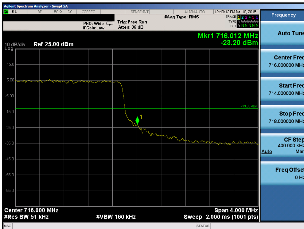
Plot 6-95. Upper Band Edge Plot (Band 12/17 - 5.0MHz QPSK - RB Size 25)
