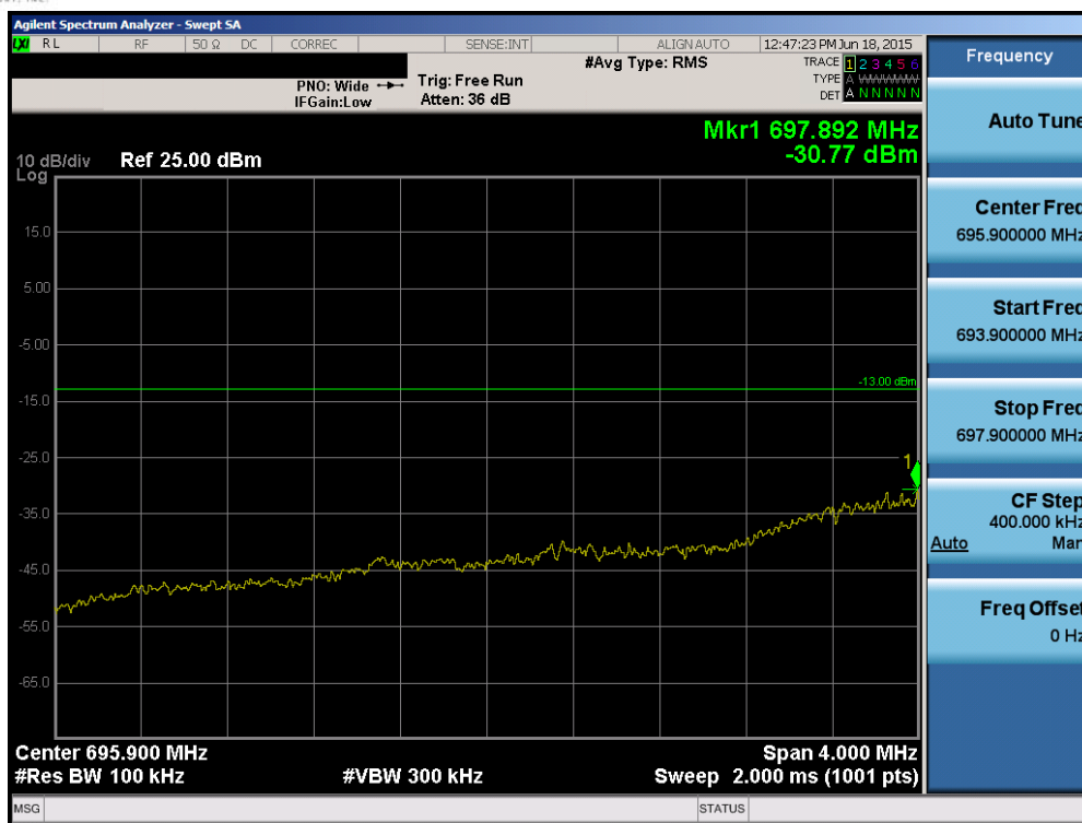
Plot 6-86. Lower Extended Band Edge Plot (Band 17 – 1.4MHz QPSK – RB Size 6)
