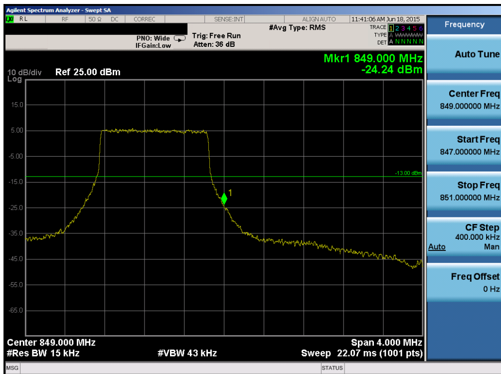
Plot 6-101. Upper Band Edge Plot (Band 5 – 1.4MHz QPSK – RB Size 6)
