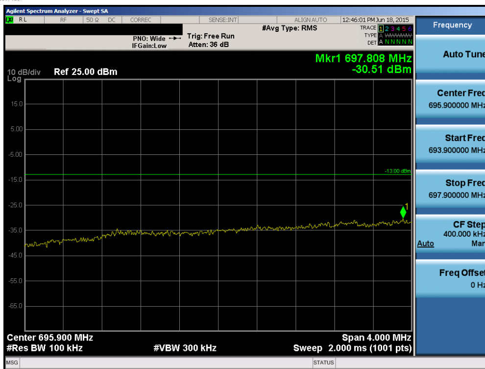
Plot 6-94. Lower Extended Band Edge Plot (Band 12/17 - 5.0MHz QPSK - RB Size 25)
