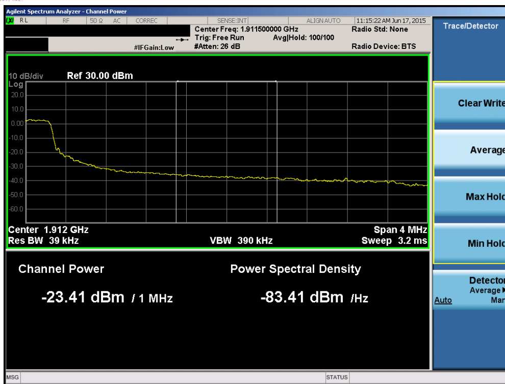
Plot 6-144. Upper Extended Band Edge Plot (Band 2 – 5.0MHz QPSK – RB Size 25)
