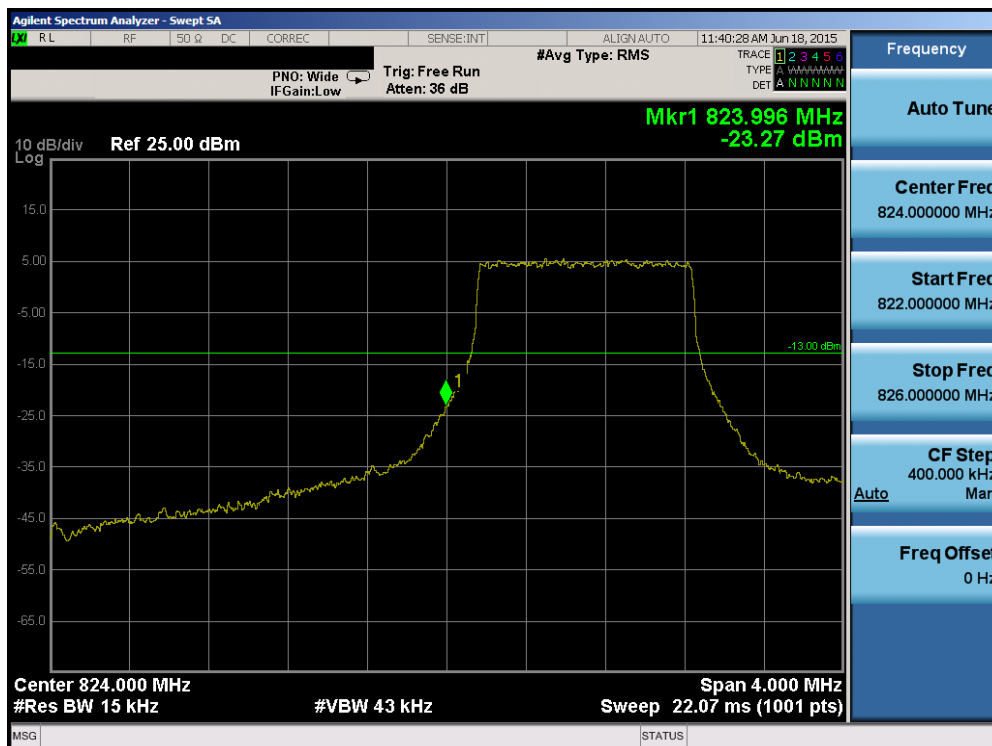
Plot 6-99. Lower Band Edge Plot (Band 5 – 1.4MHz QPSK – RB Size 6)
