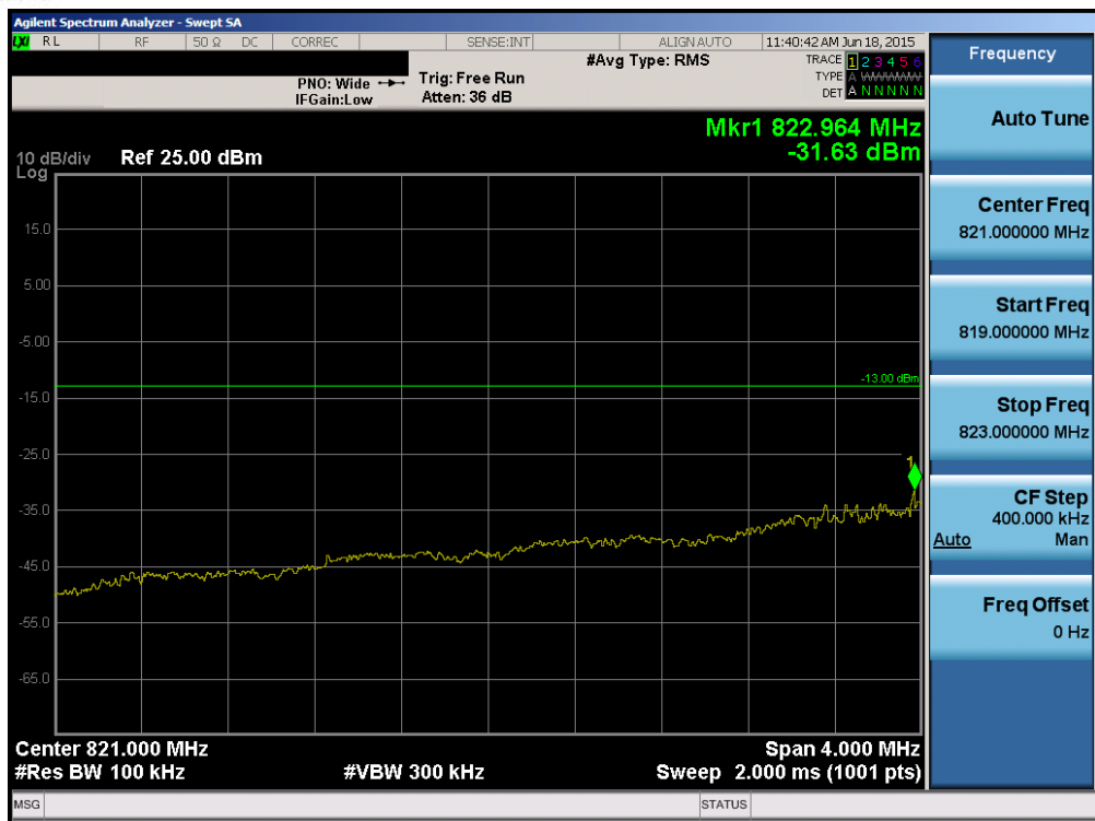
Plot 6-100. Lower Extended Band Edge Plot (Band 5 – 1.4MHz QPSK – RB Size 6)
