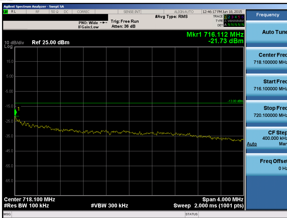
Plot 6-96. Upper Extended Band Edge Plot (Band 12/17 – 5.0MHz QPSK – RB Size 25)
