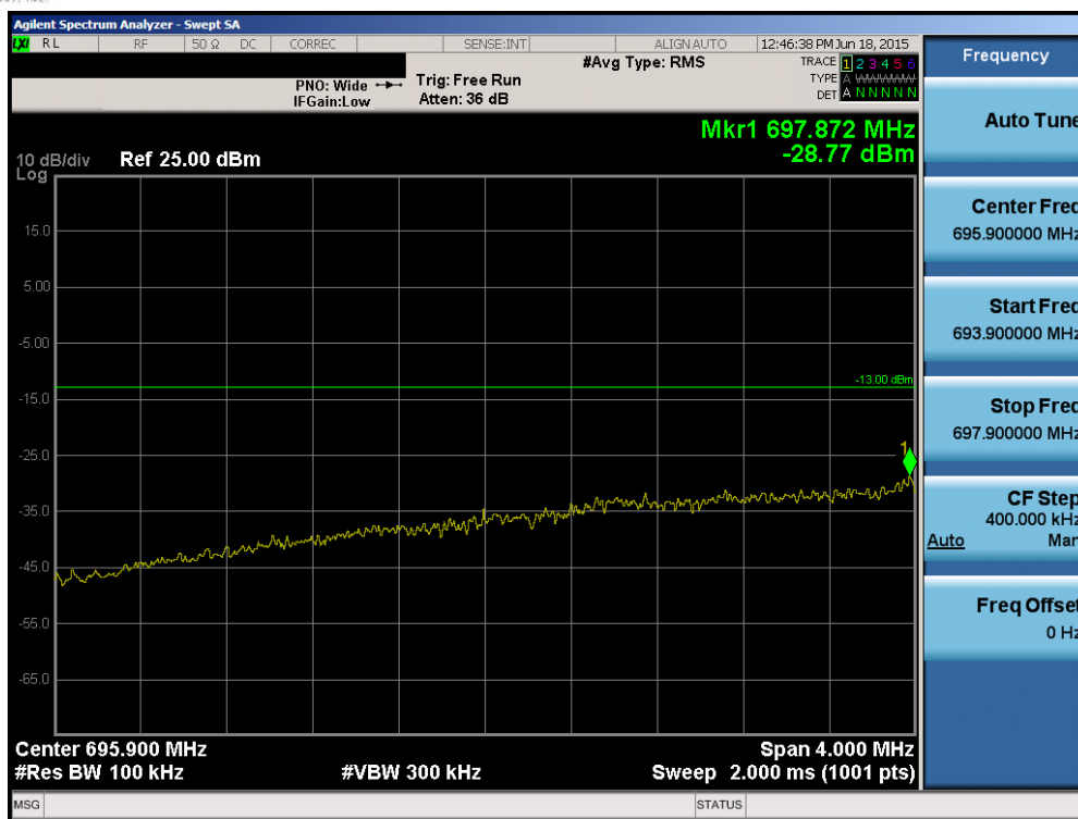
Plot 6-90. Lower Extended Band Edge Plot (Band 17 – 3.0MHz QPSK – RB Size 15)
