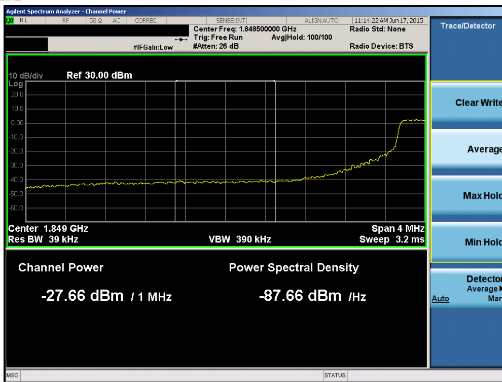
Plot 6-142. Lower Extended Band Edge Plot (Band 2 – 5.0MHz QPSK – RB Size 25)
