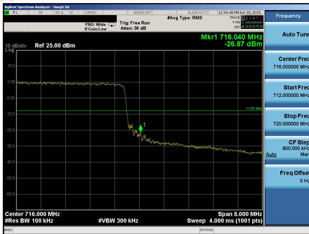
Plot 6-98. Upper Band Edge Plot (Band 12/17 – 10.0MHz QPSK – RB Size 50)
