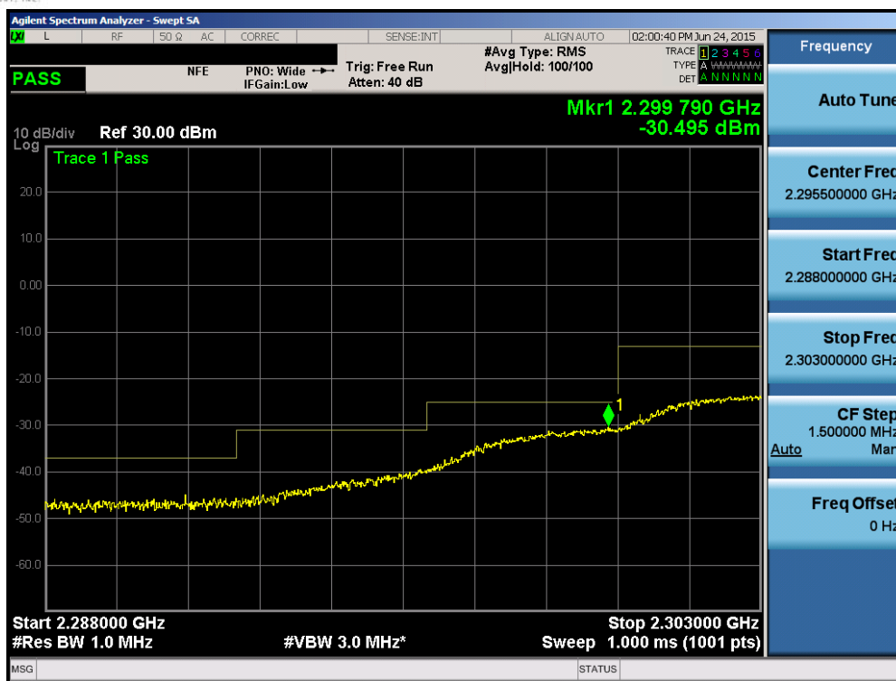
Plot 6-158. Lower Extended Band Edge Plot (Band 30 – 5.0MHz QPSK – RB Size 25)
