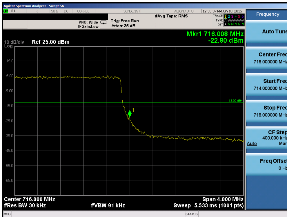
Plot 6-91. Upper Band Edge Plot (Band 17 – 3.0MHz QPSK – RB Size 15)
