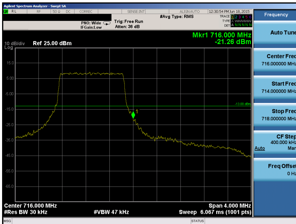
Plot 6-87. Upper Band Edge Plot (Band 17 – 1.4MHz QPSK – RB Size 6)
