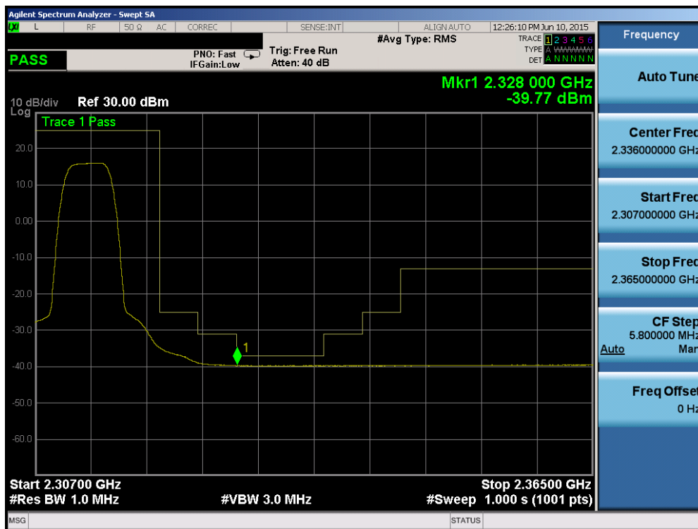
Plot 6-161. Upper Extended Band Edge Plot (Band 30 – 5.0MHz QPSK – RB Size 25)
