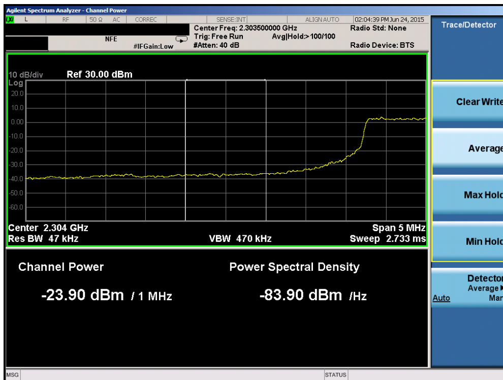
Plot 6-159. Lower Extended Band Edge Plot (Band 30 – 5.0MHz QPSK – RB Size 25)
