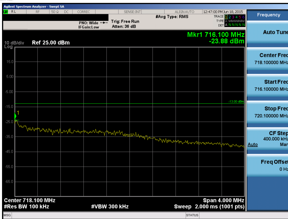
Plot 6-92. Upper Extended Band Edge Plot (Band 17 – 3.0MHz QPSK – RB Size 15)
