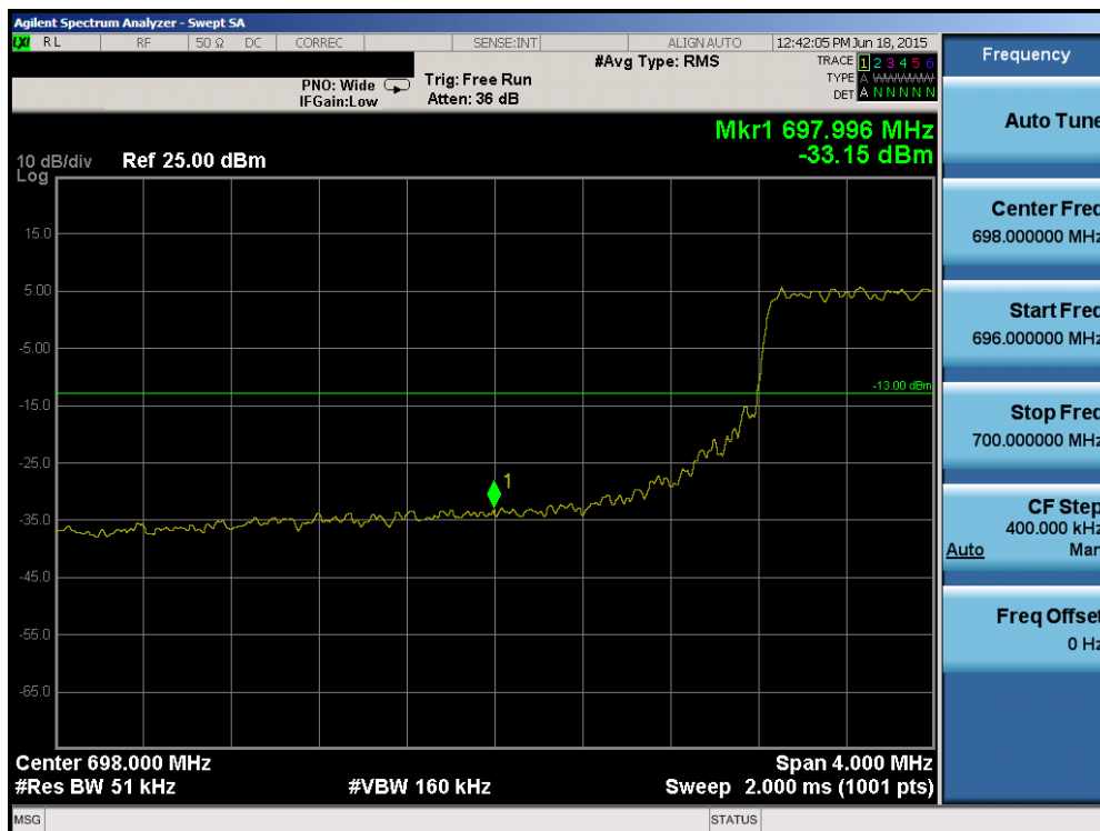
Plot 6-93. Lower Band Edge Plot (Band 12/17 – 5.0MHz QPSK – RB Size 25)
