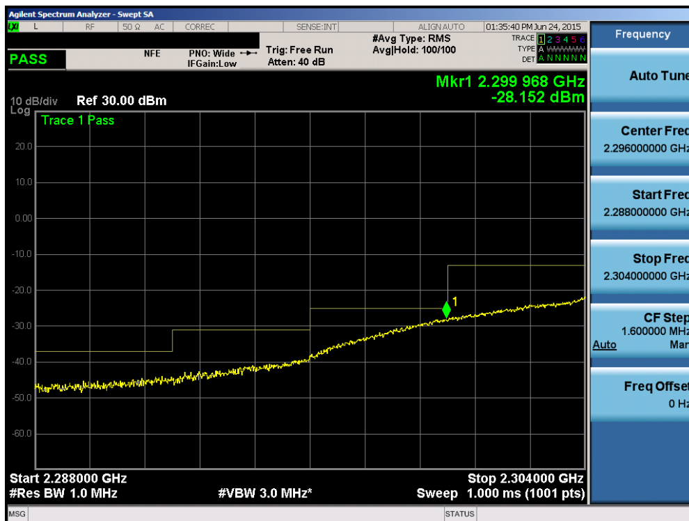
Plot 6-163. Lower Extended Band Edge Plot (Band 30 – 10.0MHz QPSK – RB Size 50)
