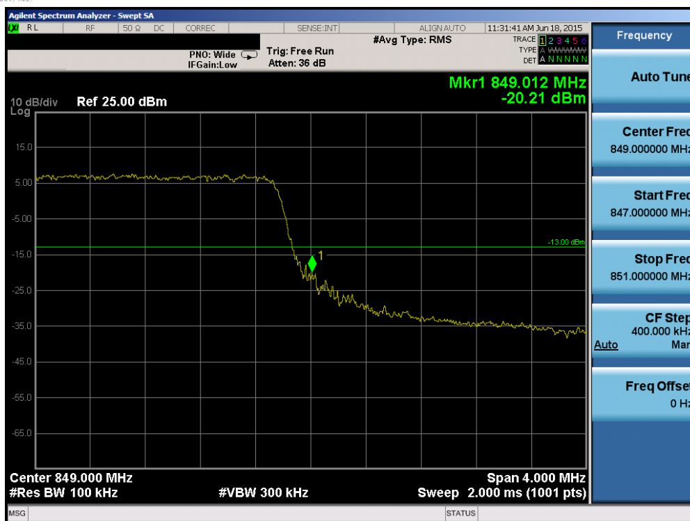
Plot 6-106. Upper Band Edge Plot (Band 5 – 5.0MHz QPSK – RB Size 25)
