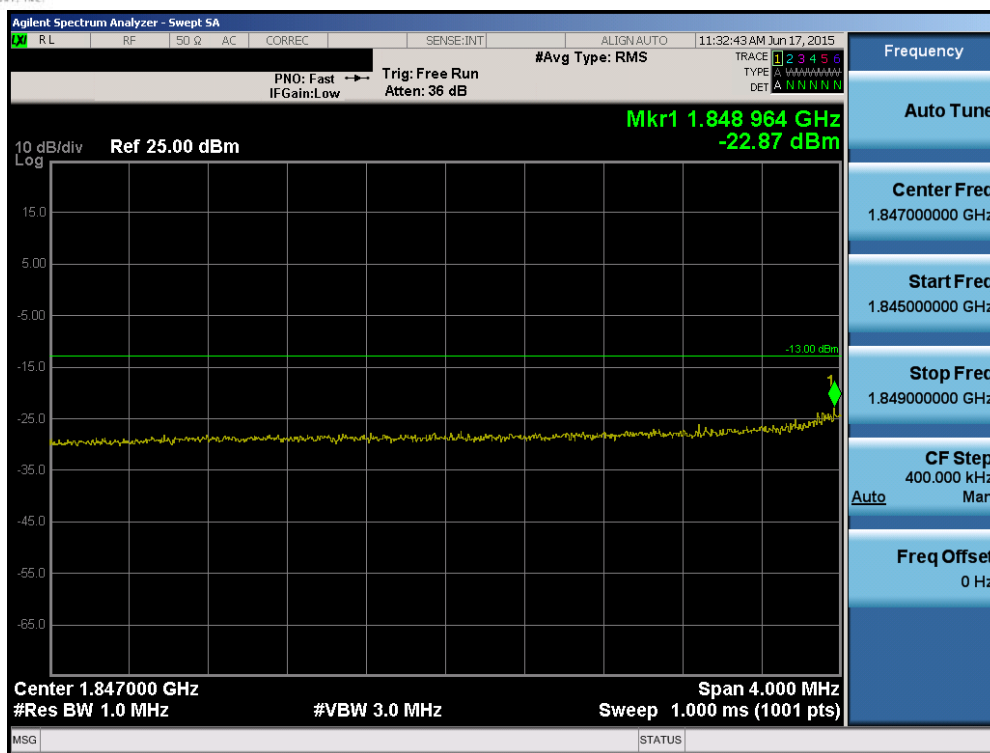
Plot 6-146. Lower Extended Band Edge Plot (Band 2 – 10.0MHz QPSK – RB Size 50)
