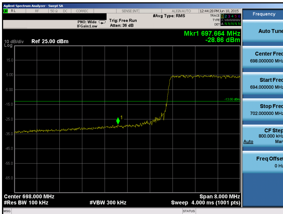
Plot 6-97. Lower Band Edge Plot (Band 12/17 – 10.0MHz QPSK – RB Size 50)
