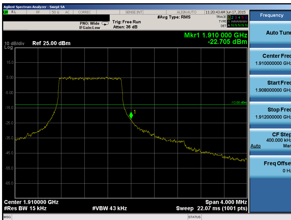
Plot 6-135. Upper Band Edge Plot (Band 2 – 1.4MHz QPSK – RB Size 6)
