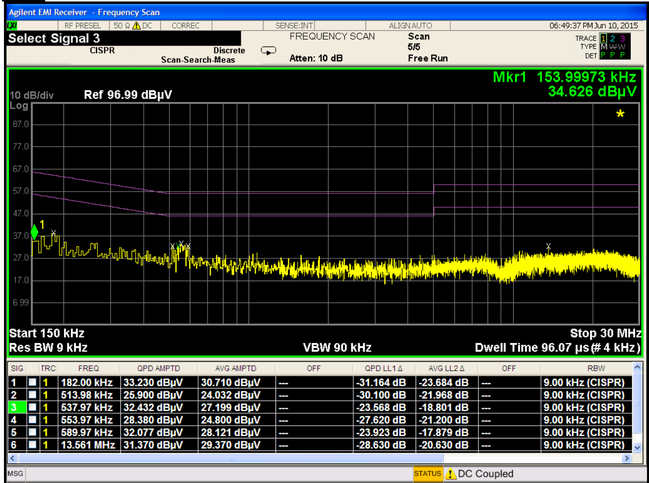
Plot 6-257. Line Conducted Plot with 802.11a UNII Band 2C (N)
