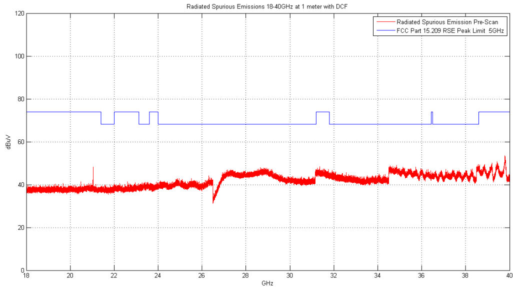
Plot 6-178. Radiated Spurious Plot above 18GHz (Simultaneous Tx 2.4GHz – 5 GHz, Ant. Pol. V)
