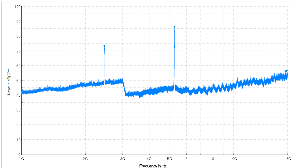
Plot 6-176. Radiated Spurious Plot above 1GHz (Simultaneous Tx 5GHz – 2.4GHz, Ant. Pol. V)
