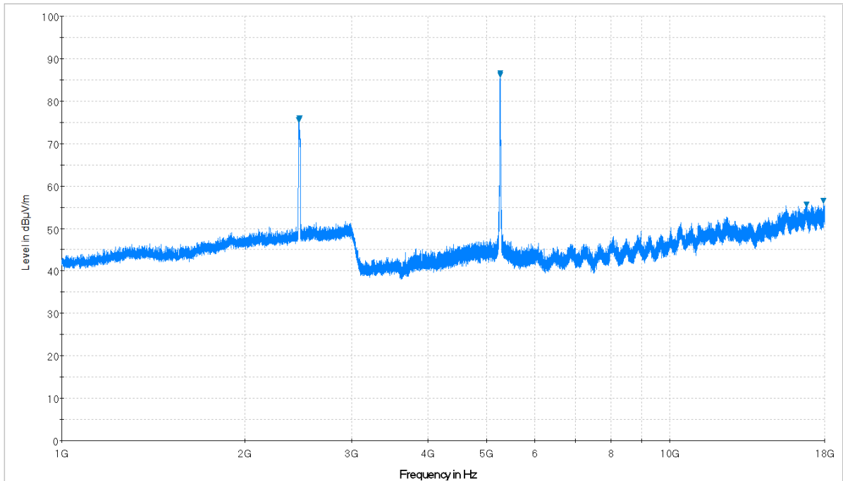
Plot 6-175. Radiated Spurious Plot above 1GHz (Simultaneous Tx 5GHz – 2.4GHz, Ant. Pol. H)
