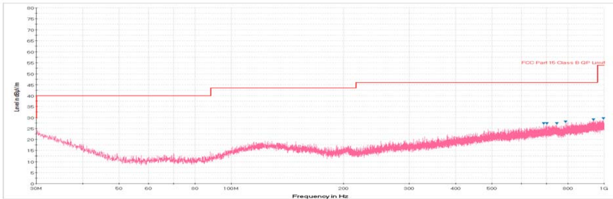
Plot 6-246. Radiated Spurious Plot below 1GHz (802.11a – U3 Ch. 157, Ant. Pol. H)
