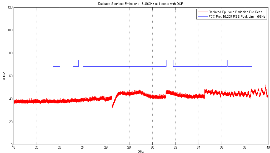
Plot 6-180. Radiated Spurious Plot above 18GHz (Simultaneous Tx 5 GHz – 2.4 GHz, Ant. Pol. V)
