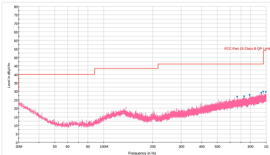
Plot 6-248. Radiated Spurious Plot below 1GHz (Simultaneous Tx 2.4GHz – 5 GHz, Ant. Pol. H)
