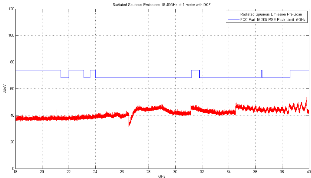
Plot 6-177. Radiated Spurious Plot above 18GHz (Simultaneous Tx 2.4GHz – 5 GHz, Ant. Pol. H)
