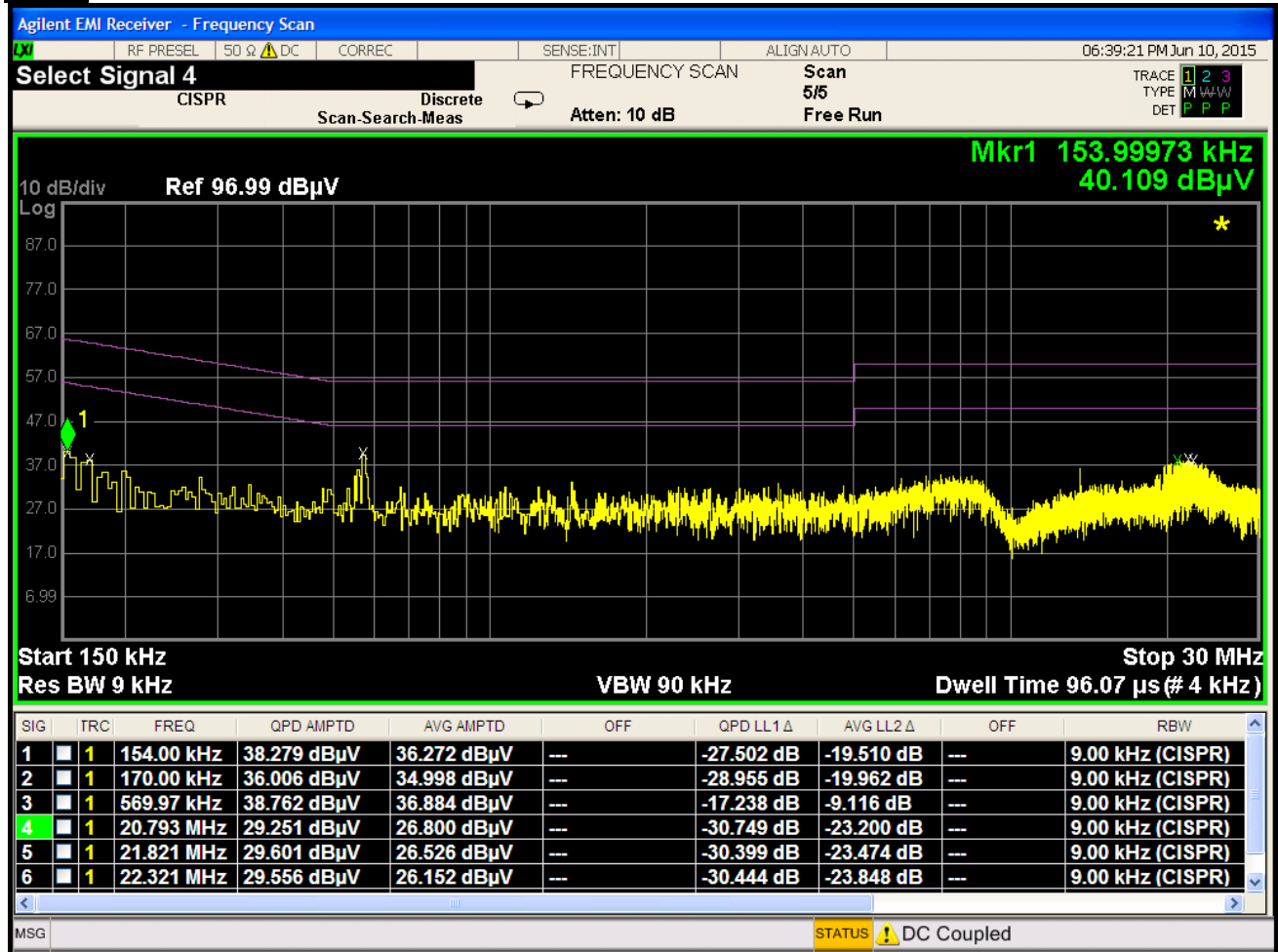
Plot 6-256. Line Conducted Plot with 802.11a UNII Band 2C (L1)
