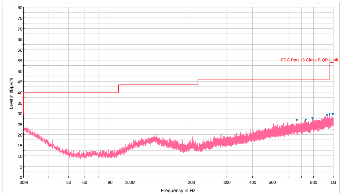
Plot 6-249. Radiated Spurious Plot below 1GHz (Simultaneous Tx 2.4GHz – 5 GHz, Ant. Pol. V)
