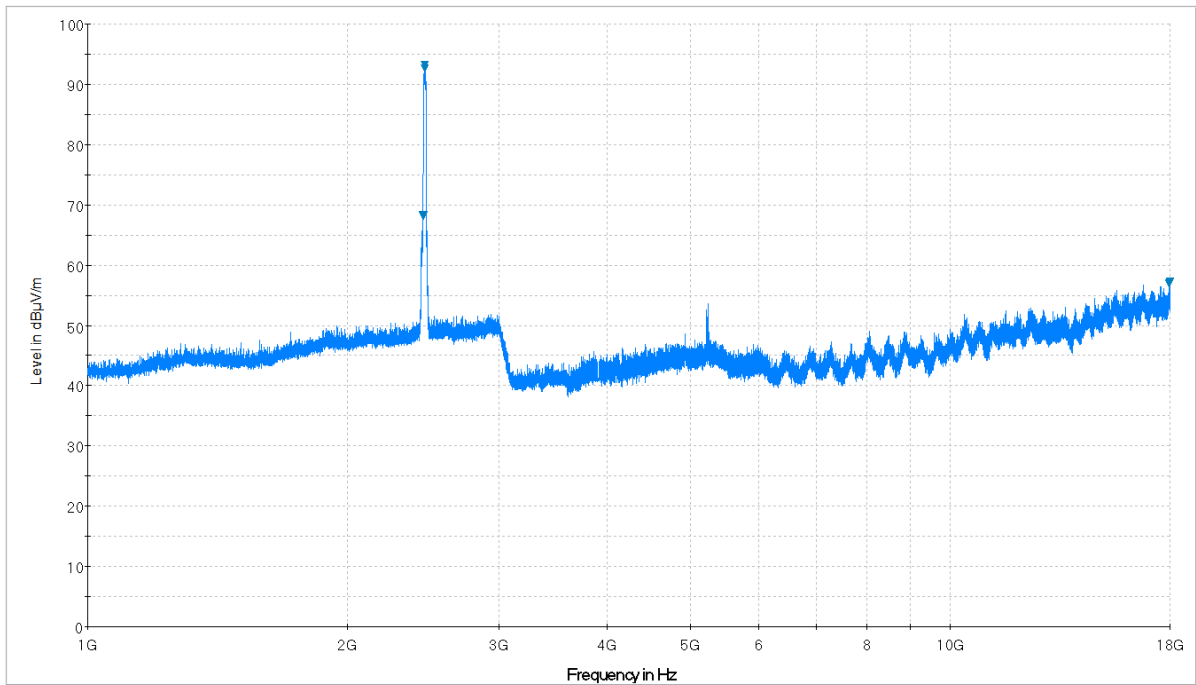
Plot 6-174. Radiated Spurious Plot above 1GHz (Simultaneous Tx 2.4GHz – 5GHz, Ant. Pol. V)
