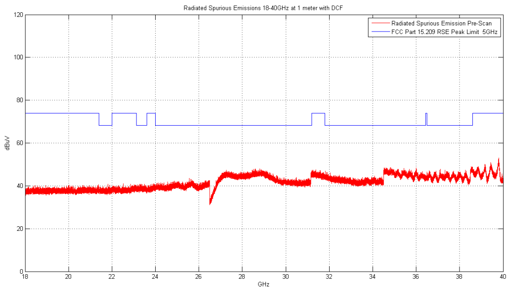
Plot 6-179. Radiated Spurious Plot above 18GHz (Simultaneous Tx 5 GHz – 2.4 GHz, Ant. Pol. H)
