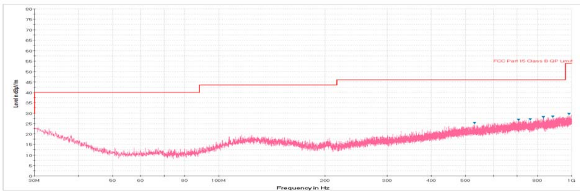
Plot 6-247. Radiated Spurious Plot below 1GHz (802.11a – U3 Ch. 157, Ant. Pol. V)
