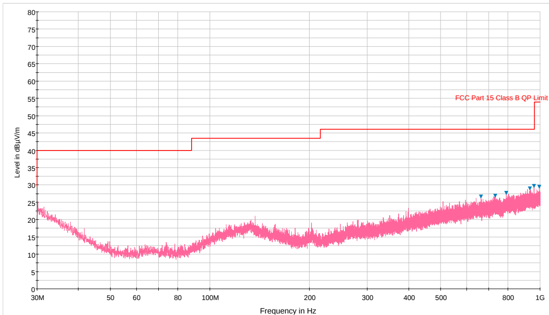
Plot 6-251. Radiated Spurious Plot below 1GHz (Simultaneous Tx 5GHz – 2.4GHz, Ant. Pol. V)
