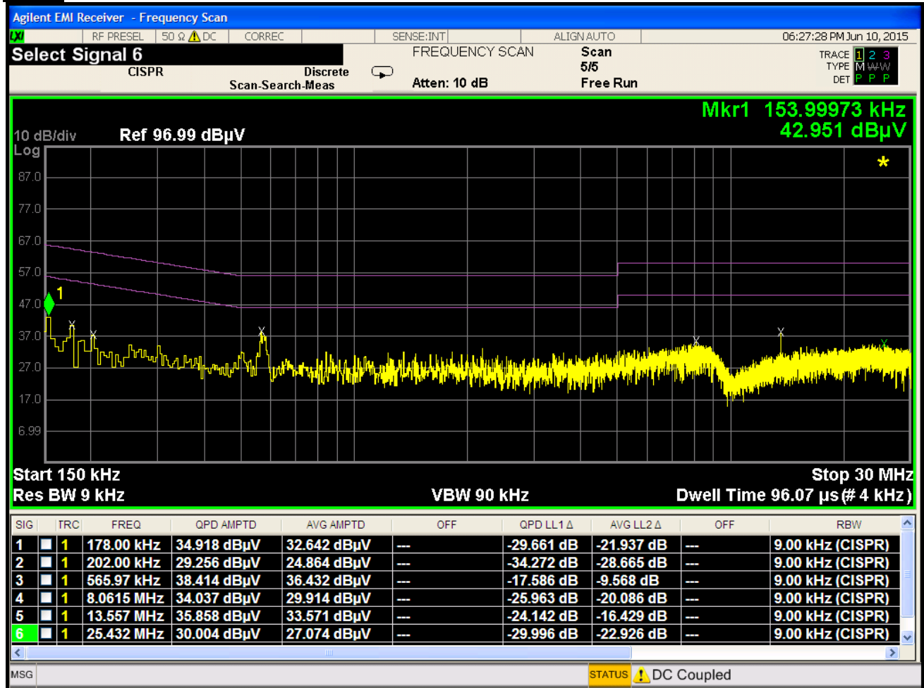
Plot 6-252. Line Conducted Plot with 802.11a UNII Band 1 (L1)
