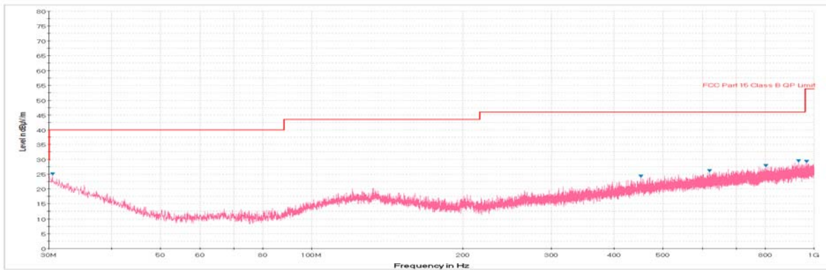
Plot 6-245. Radiated Spurious Plot below 1GHz (802.11a – U3 Ch. 157, Ant. Pol. V)
