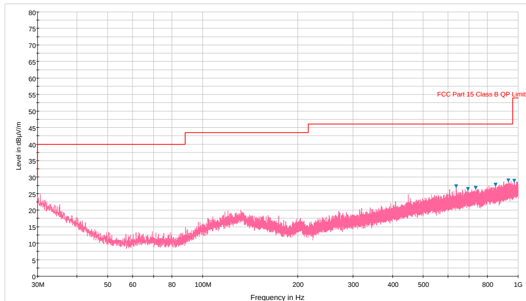
Plot 6-250. Radiated Spurious Plot below 1GHz (Simultaneous Tx 5GHz – 2.4GHz, Ant. Pol. H)
