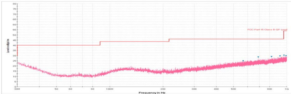
Plot 6-244. Radiated Spurious Plot below 1GHz (802.11a – U3 Ch. 157, Ant. Pol. H)
