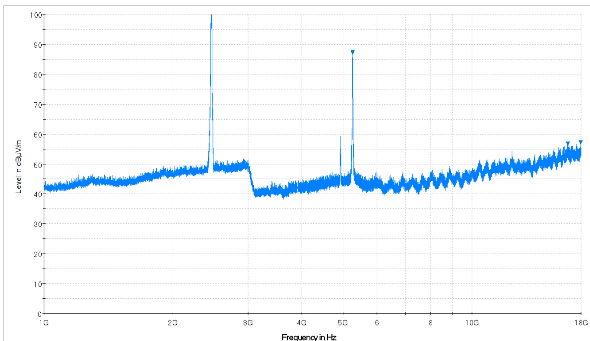
Plot 6-173. Radiated Spurious Plot above 1GHz (Simultaneous Tx 2.4GHz – 5GHz, Ant. Pol. H)
