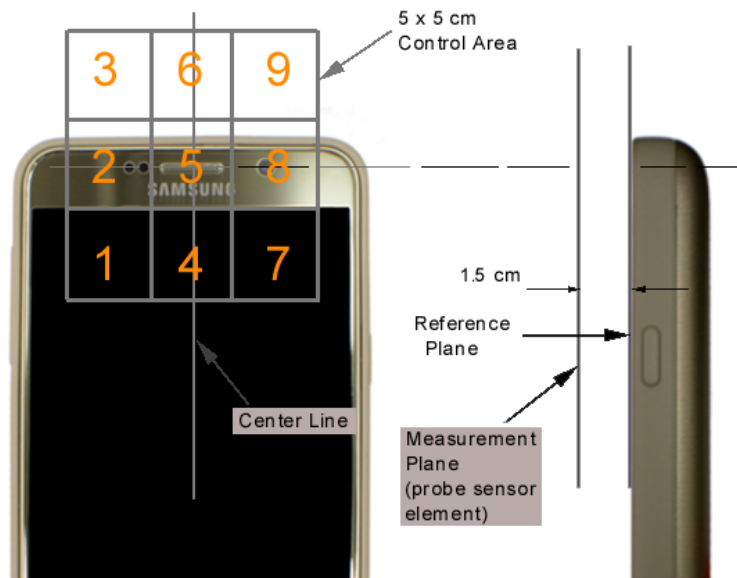
Figure 15-3 5x5 Scan grid above WD
