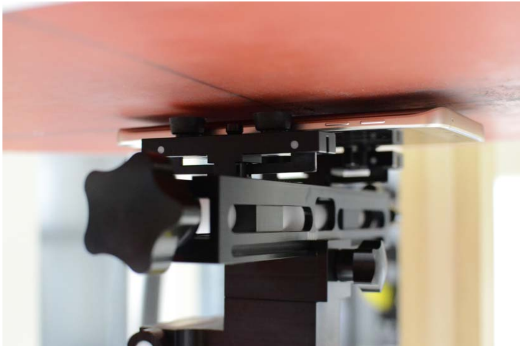
SAR Test Setup Photo 6– Back Side at 0.3 cm (Extremity)
