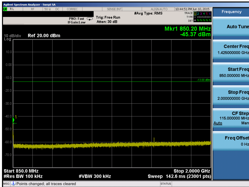
Plot 6-59. Conducted Spurious Plot (Band 5/26 – 5.0MHz QPSK – RB Size 1, RB Offset 0 – High Channel)
