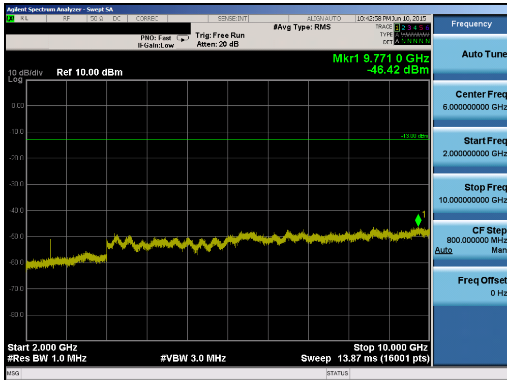
Plot 6-57. Conducted Spurious Plot (Band 5/26 – 5.0MHz QPSK – RB Size 1, RB Offset 0 – Mid Channel)
