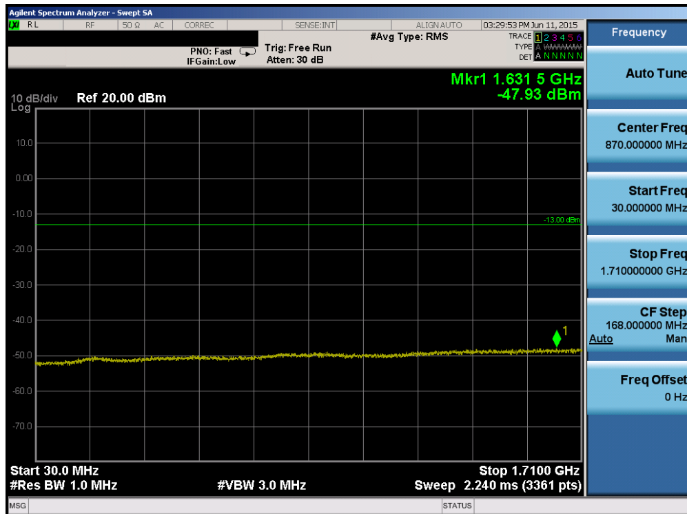
Plot 6-64. Conducted Spurious Plot (Band 4 – 5.0MHz QPSK – RB Size 1, RB Offset 0 – Mid Channel)
