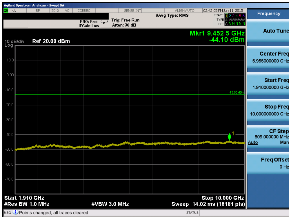
Plot 6-71. Conducted Spurious Plot (Band 2 – 5.0MHz QPSK – RB Size 1, RB Offset 0 – Low Channel)
