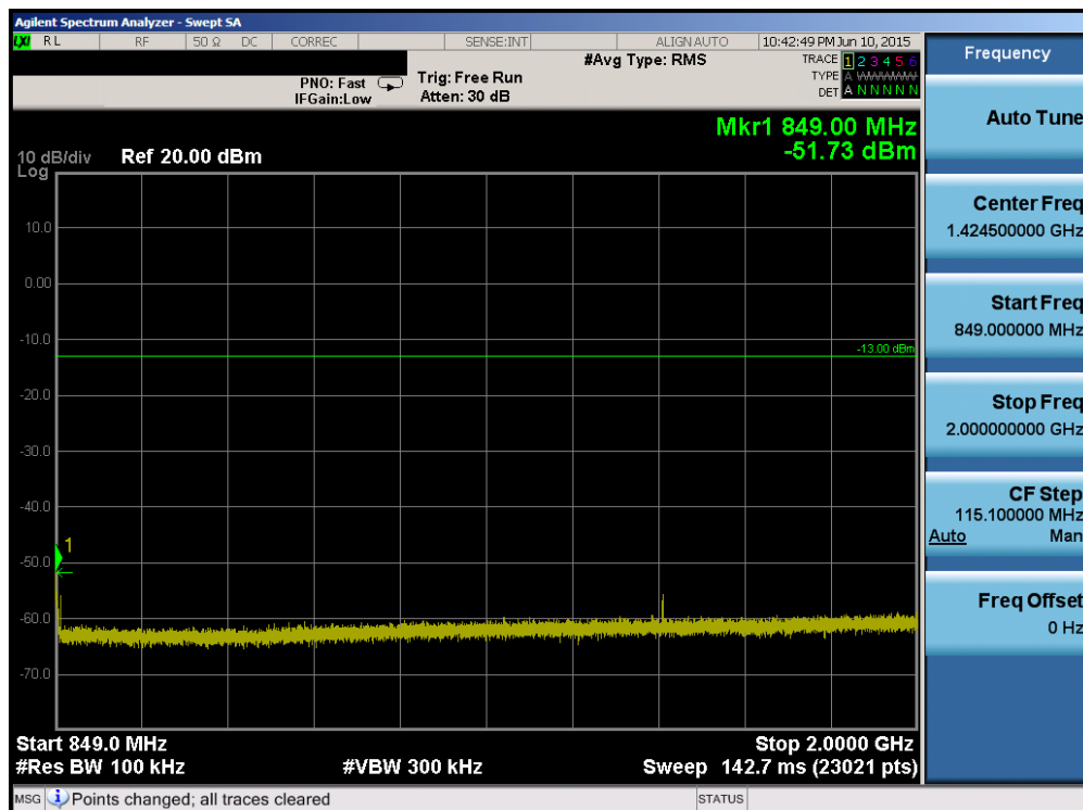
Plot 6-56. Conducted Spurious Plot (Band 5/26 – 5.0MHz QPSK – RB Size 1, RB Offset 0 – Mid Channel)
