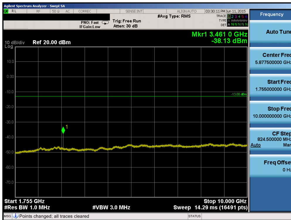
Plot 6-65. Conducted Spurious Plot (Band 4 – 5.0MHz QPSK – RB Size 1, RB Offset 0 – Mid Channel)
