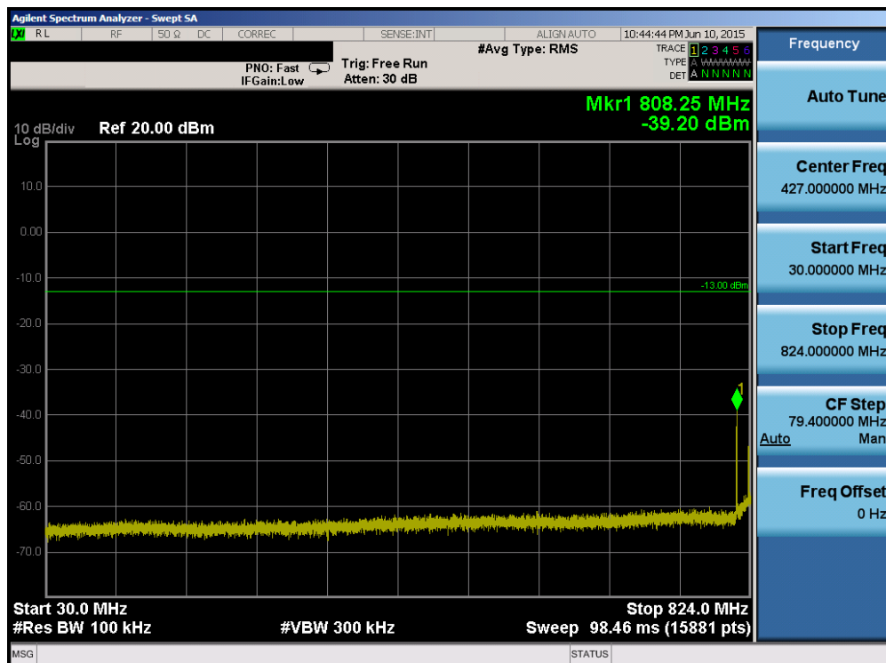
Plot 6-58. Conducted Spurious Plot (Band 5/26 – 5.0MHz QPSK – RB Size 1, RB Offset 0 – High Channel)
