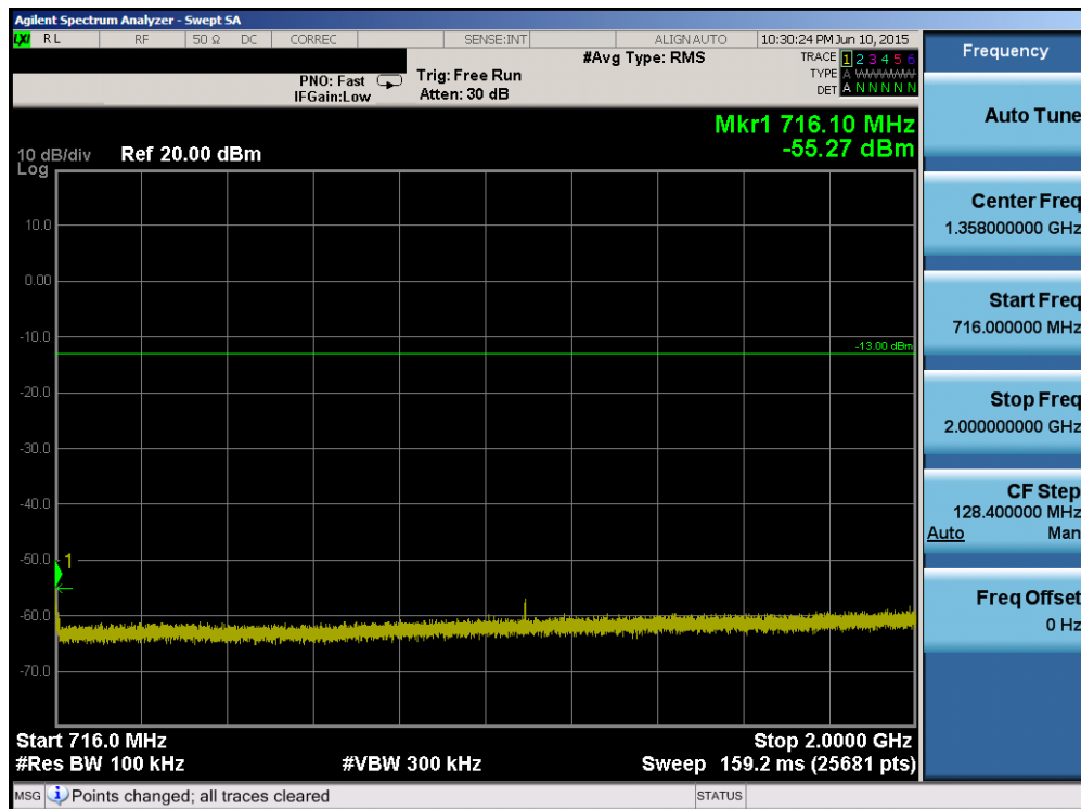
Plot 6-44. Conducted Spurious Plot (Band 12/17 – 10.0MHz QPSK – RB Size 1, RB Offset 0 – Low Channel)
