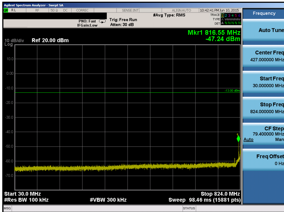
Plot 6-55. Conducted Spurious Plot (Band 5/26 – 5.0MHz QPSK – RB Size 1, RB Offset 0 – Mid Channel)
