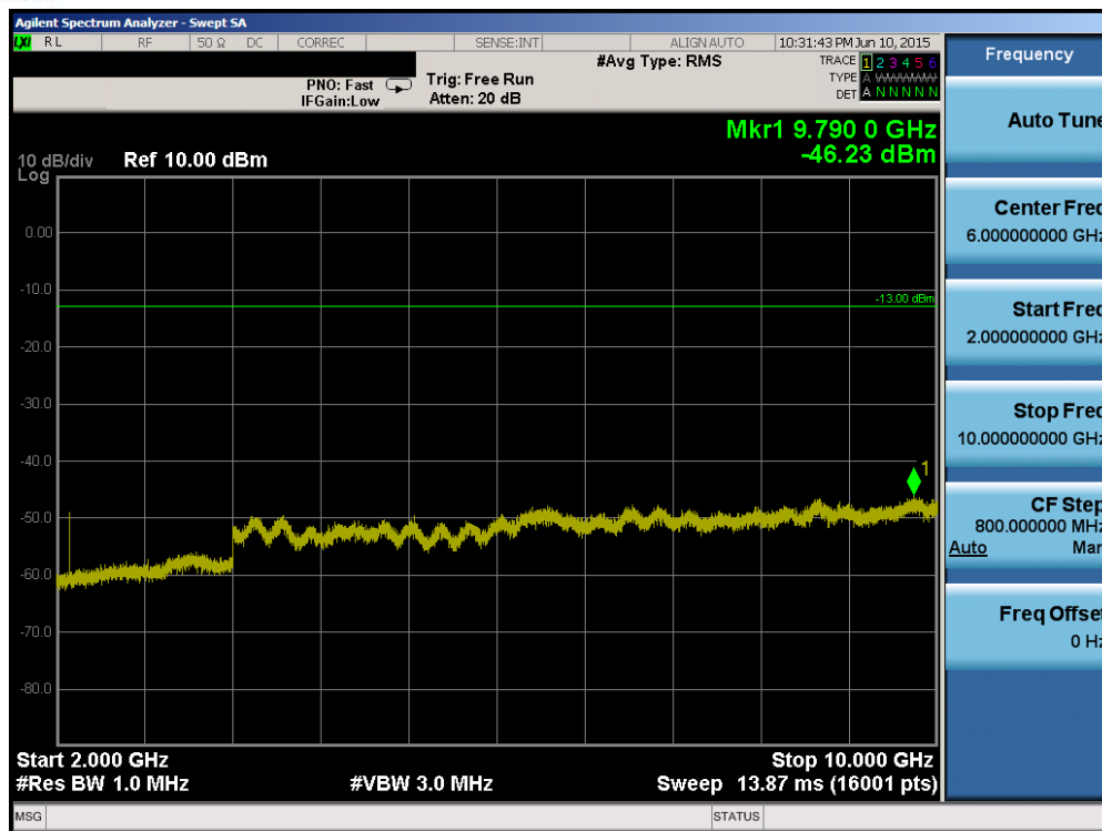
Plot 6-51. Conducted Spurious Plot (Band 12/17 – 10.0MHz QPSK – RB Size 1, RB Offset 0 – High Channel)
