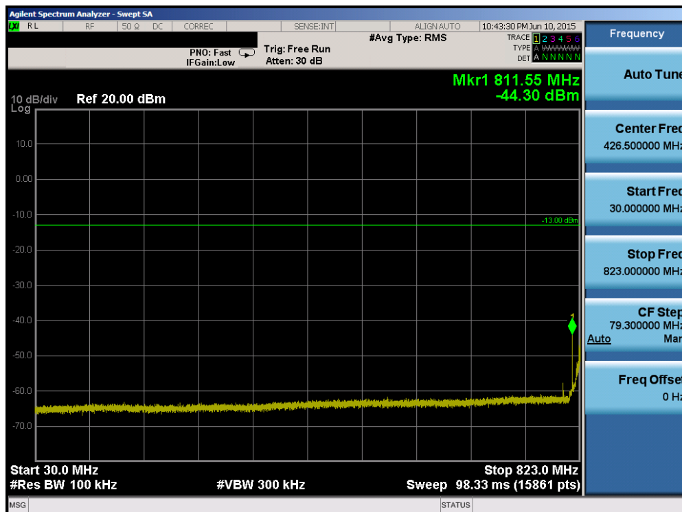
Plot 6-52. Conducted Spurious Plot (Band 5/26 – 5.0MHz QPSK – RB Size 1, RB Offset 0 – Low Channel)
