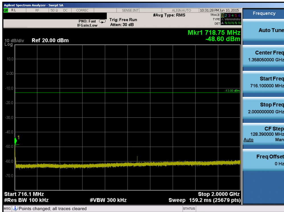
Plot 6-50. Conducted Spurious Plot (Band 12/17 – 10.0MHz QPSK – RB Size 1, RB Offset 0 – High Channel)
