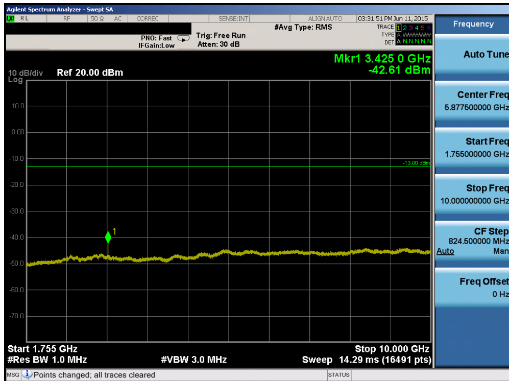
Plot 6-62. Conducted Spurious Plot (Band 4 – 5.0MHz QPSK – RB Size 1, RB Offset 0 – Low Channel)
