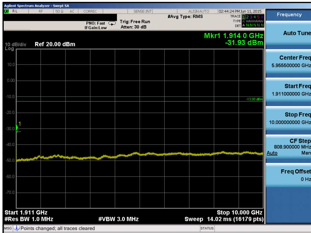
Plot 6-77. Conducted Spurious Plot (Band 2 – 5.0MHz QPSK – RB Size 1, RB Offset 0 – High Channel)
