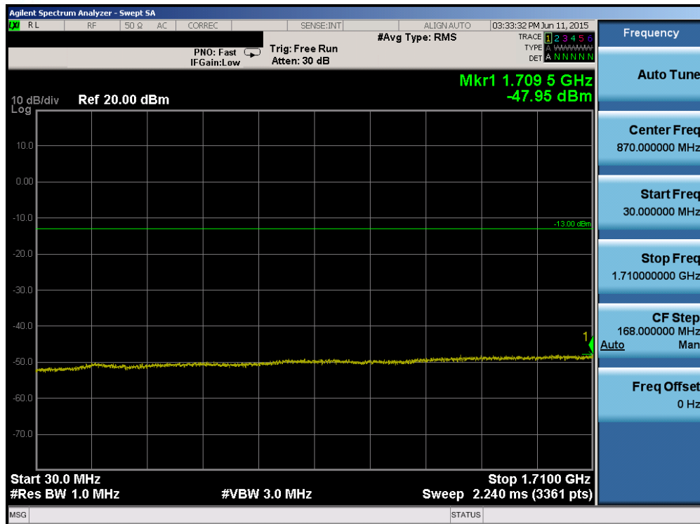
Plot 6-67. Conducted Spurious Plot (Band 4 – 5.0MHz QPSK – RB Size 1, RB Offset 0 – High Channel)
