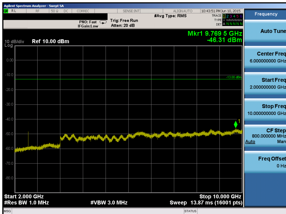
Plot 6-54. Conducted Spurious Plot (Band 5/26 – 5.0MHz QPSK – RB Size 1, RB Offset 0 – Low Channel)
