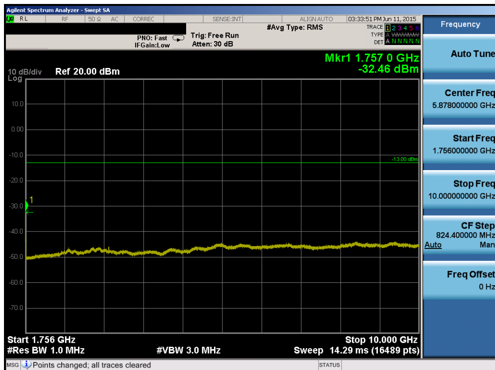
Plot 6-68. Conducted Spurious Plot (Band 4 – 5.0MHz QPSK – RB Size 1, RB Offset 0 – High Channel)
