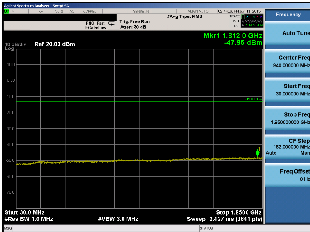
Plot 6-76. Conducted Spurious Plot (Band 2 – 5.0MHz QPSK – RB Size 1, RB Offset 0 – High Channel)
