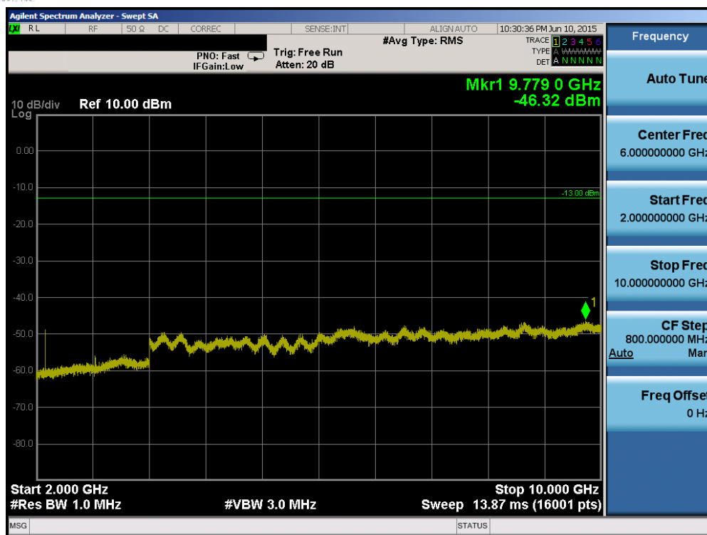
Plot 6-45. Conducted Spurious Plot (Band 12/17 – 10.0MHz QPSK – RB Size 1, RB Offset 0 – Low Channel)
