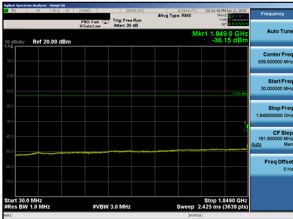
Plot 6-70. Conducted Spurious Plot (Band 2 – 5.0MHz QPSK – RB Size 1, RB Offset 0 – Low Channel)
