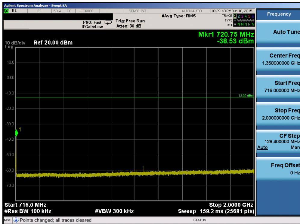
Plot 6-47. Conducted Spurious Plot (Band 12/17 – 10.0MHz QPSK – RB Size 1, RB Offset 0 – Mid Channel)
