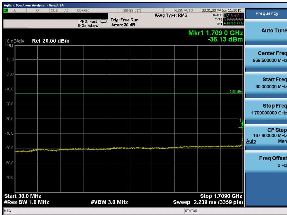
Plot 6-61. Conducted Spurious Plot (Band 4 – 5.0MHz QPSK – RB Size 1, RB Offset 0 – Low Channel)
