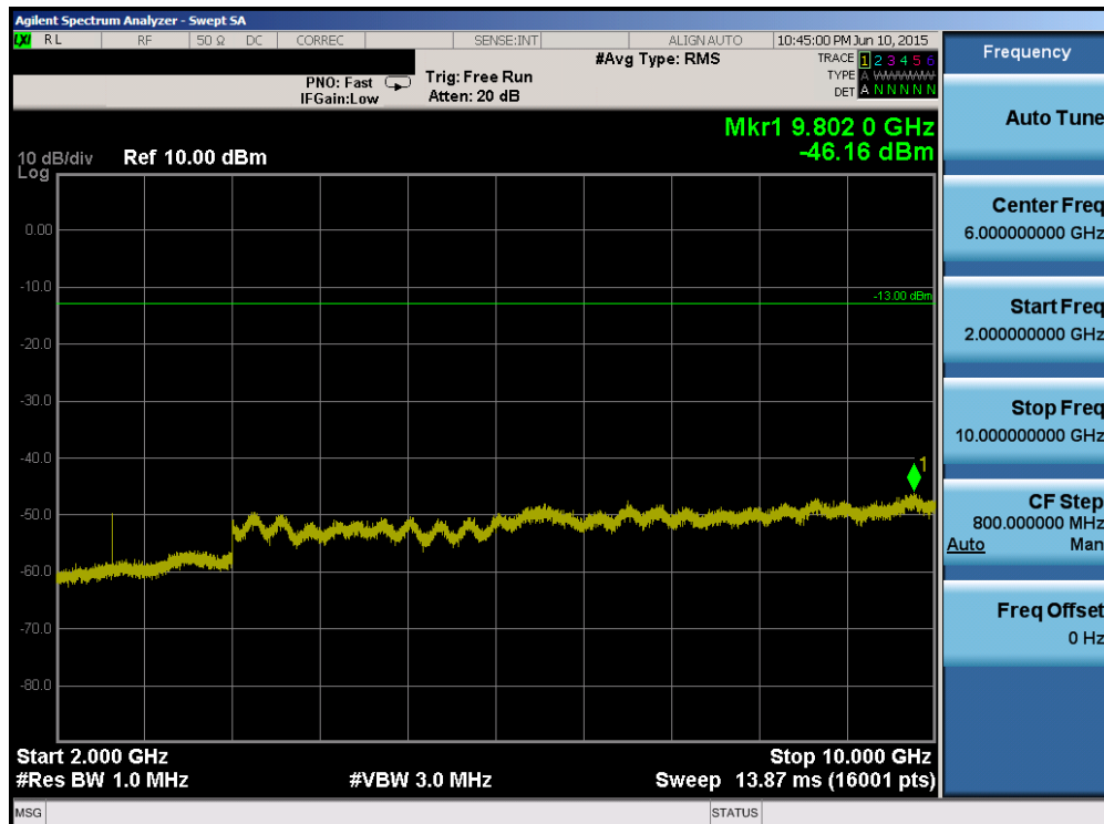
Plot 6-60. Conducted Spurious Plot (Band 5/26 – 5.0MHz QPSK – RB Size 1, RB Offset 0 – High Channel)
