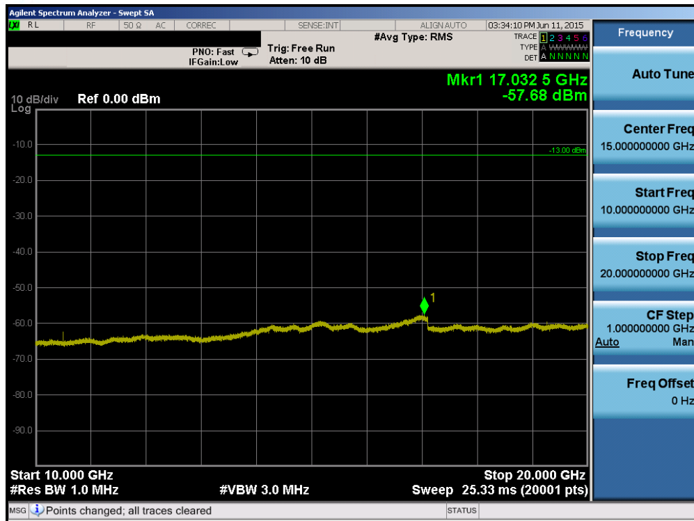
Plot 6-69. Conducted Spurious Plot (Band 4 – 5.0MHz QPSK – RB Size 1, RB Offset 0 – High Channel)
