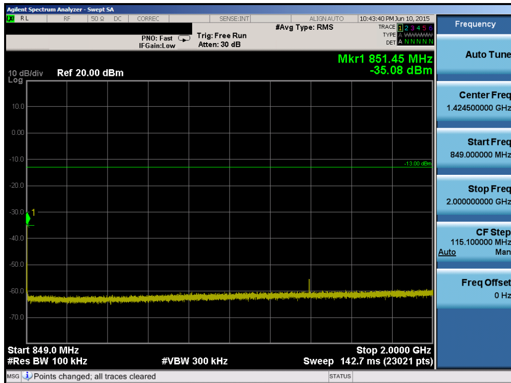
Plot 6-53. Conducted Spurious Plot (Band 5/26 – 5.0MHz QPSK – RB Size 1, RB Offset 0 – Low Channel)
