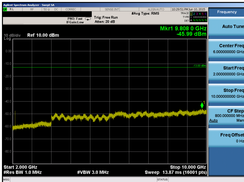
Plot 6-48. Conducted Spurious Plot (Band 12/17 – 10.0MHz QPSK – RB Size 1, RB Offset 0 – Mid Channel)
