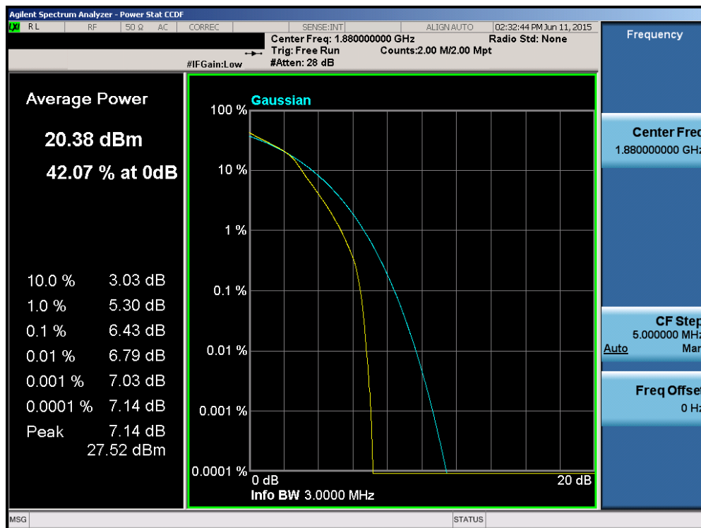
Plot 6-160. PAR Plot (Band 2 – 3.0MHz 16-QAM – RB Size 15)
