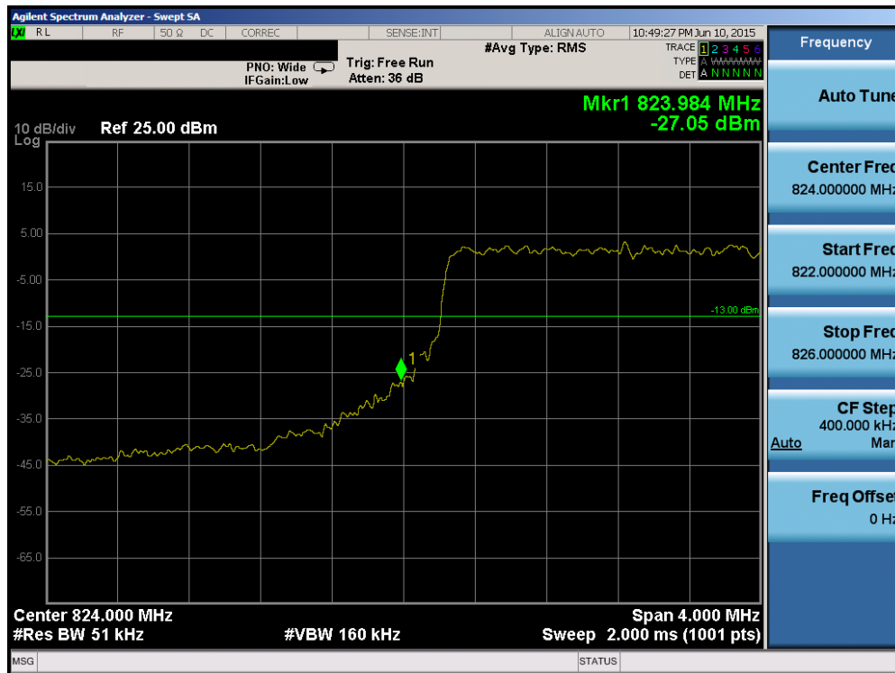
Plot 6-101. Lower Band Edge Plot (Band 5/26 – 5.0MHz QPSK – RB Size 25)
