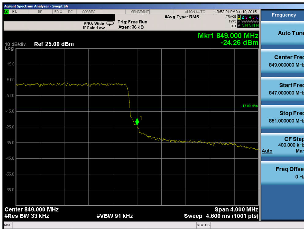
Plot 6-99. Upper Band Edge Plot (Band 5/26 - 3.0MHz QPSK - RB Size 15)
