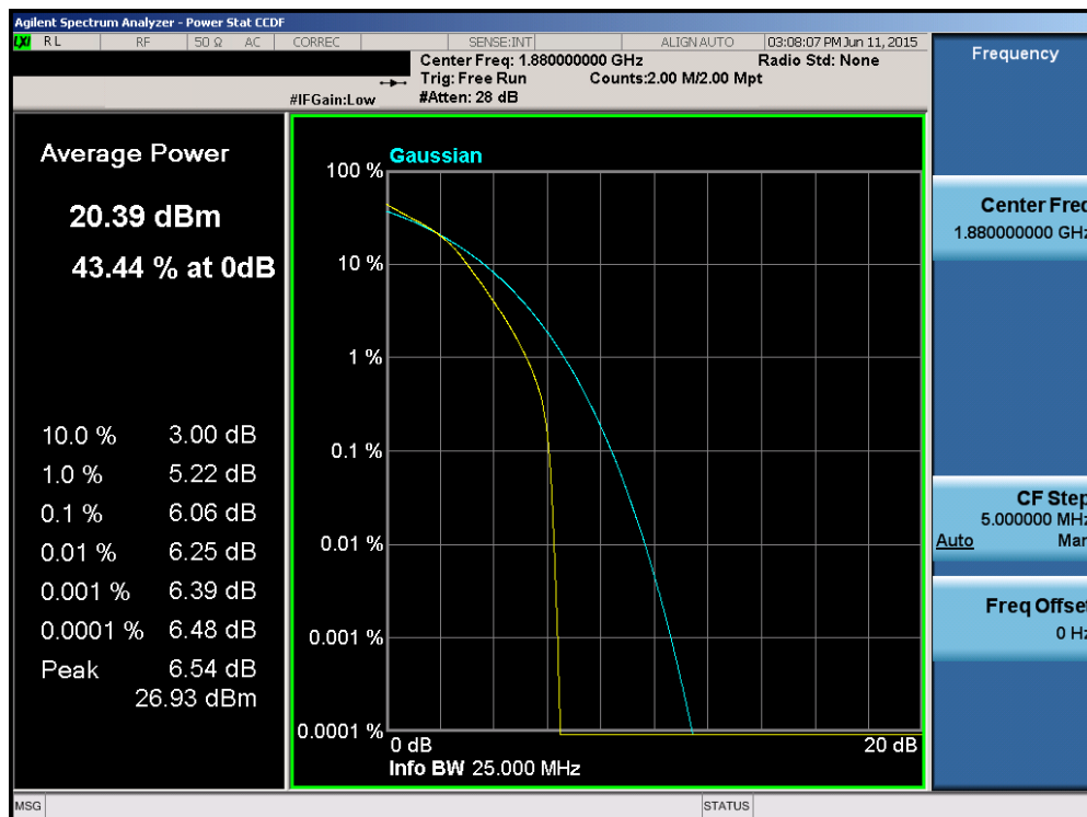
Plot 6-168. PAR Plot (Band 2 – 20.0MHz 16-QAM – RB Size 100)
