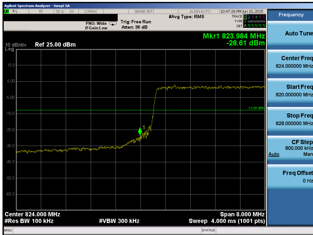
Plot 6-105. Lower Band Edge Plot (Band 5/26 – 10.0MHz QPSK – RB Size 50)
