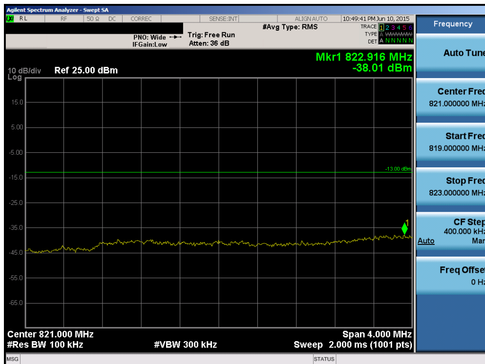
Plot 6-102. Lower Extended Band Edge Plot (Band 5/26 – 5.0MHz QPSK – RB Size 25)
