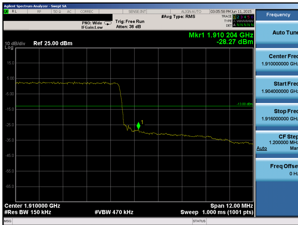
Plot 6-151. Upper Band Edge Plot (Band 2 – 15.0MHz QPSK – RB Size 75)
