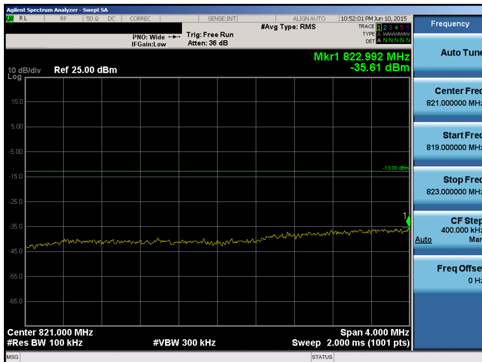
Plot 6-98. Lower Extended Band Edge Plot (Band 5/26 – 3.0MHz QPSK – RB Size 15)
