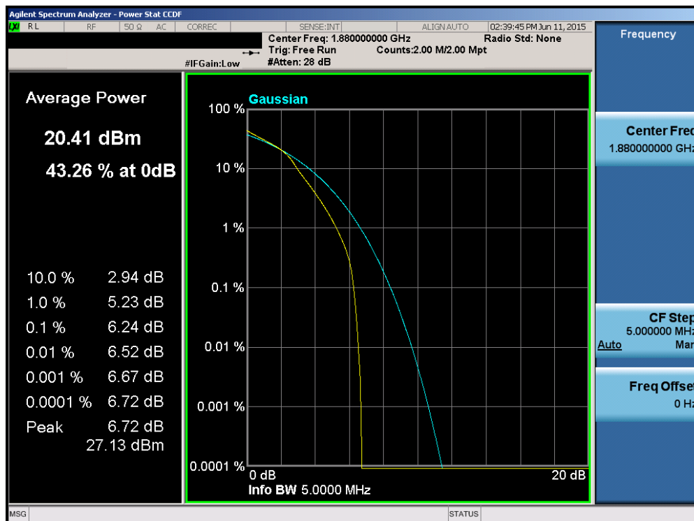
Plot 6-162. PAR Plot (Band 2 – 5.0MHz 16-QAM – RB Size 25)
