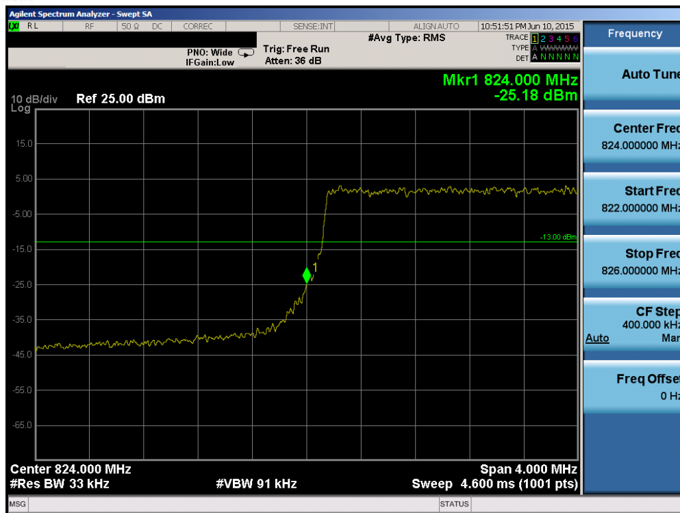
Plot 6-97. Lower Band Edge Plot (Band 5/26 – 3.0MHz QPSK – RB Size 15)
