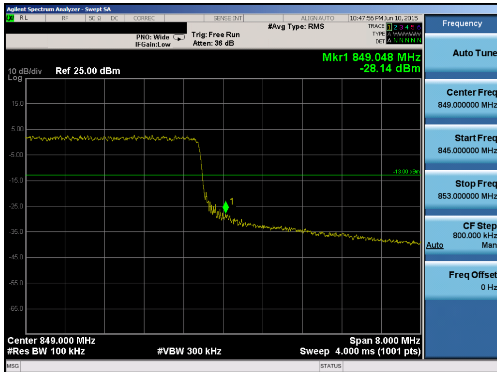
Plot 6-106. Upper Band Edge Plot (Band 5/26 – 10.0MHz QPSK – RB Size 50)
