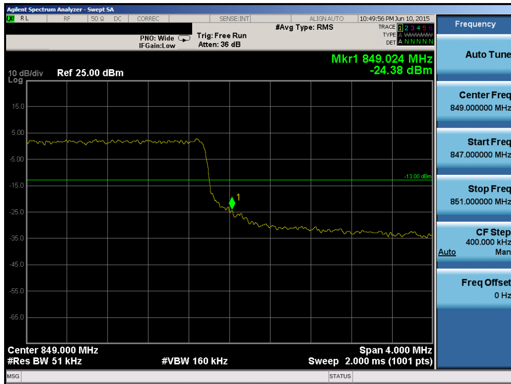
Plot 6-103. Upper Band Edge Plot (Band 5/26 – 5.0MHz QPSK – RB Size 25)
