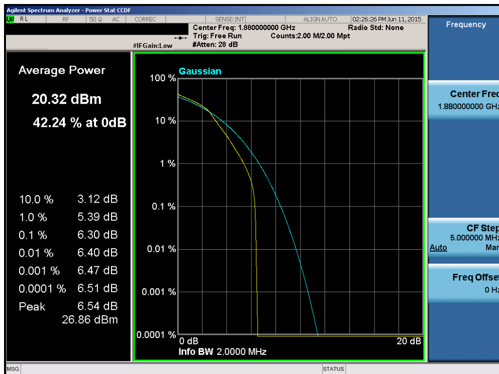
Plot 6-158. PAR Plot (Band 2 – 1.4MHz 16-QAM – RB Size 6)
