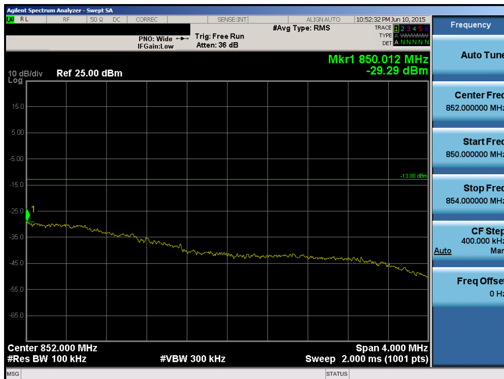
Plot 6-100. Upper Extended Band Edge Plot (Band 5/26 - Band 5 - 3.0MHz QPSK - RB Size 15)
