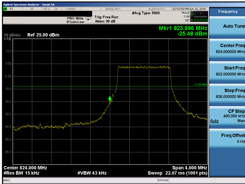
Plot 6-93. Lower Band Edge Plot (Band 5/26 – 1.4MHz QPSK – RB Size 6)
