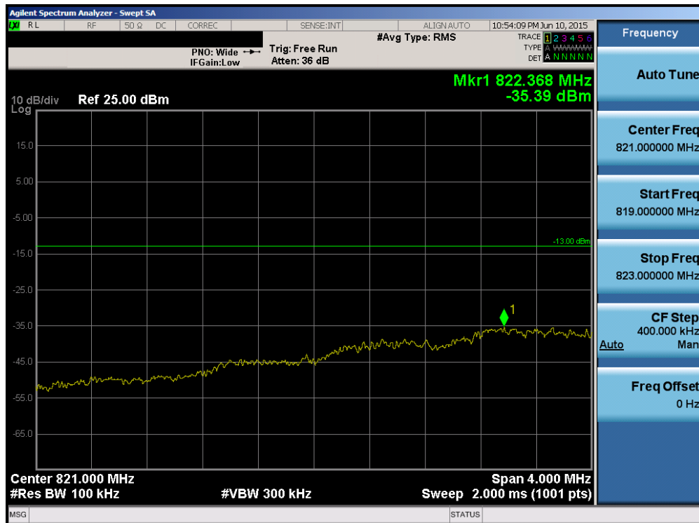
Plot 6-94. Lower Extended Band Edge Plot (Band 5/26 – 1.4MHz QPSK – RB Size 6)
