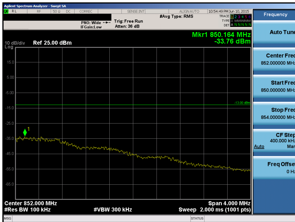
Plot 6-96. Upper Extended Band Edge Plot (Band 5/26 – 1.4MHz QPSK – RB Size 6)
