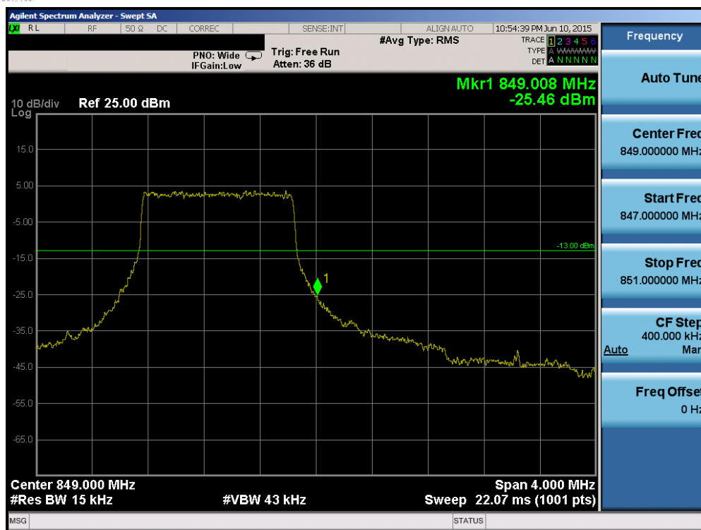
Plot 6-95. Upper Band Edge Plot (Band 5/26 – 1.4MHz QPSK – RB Size 6)
