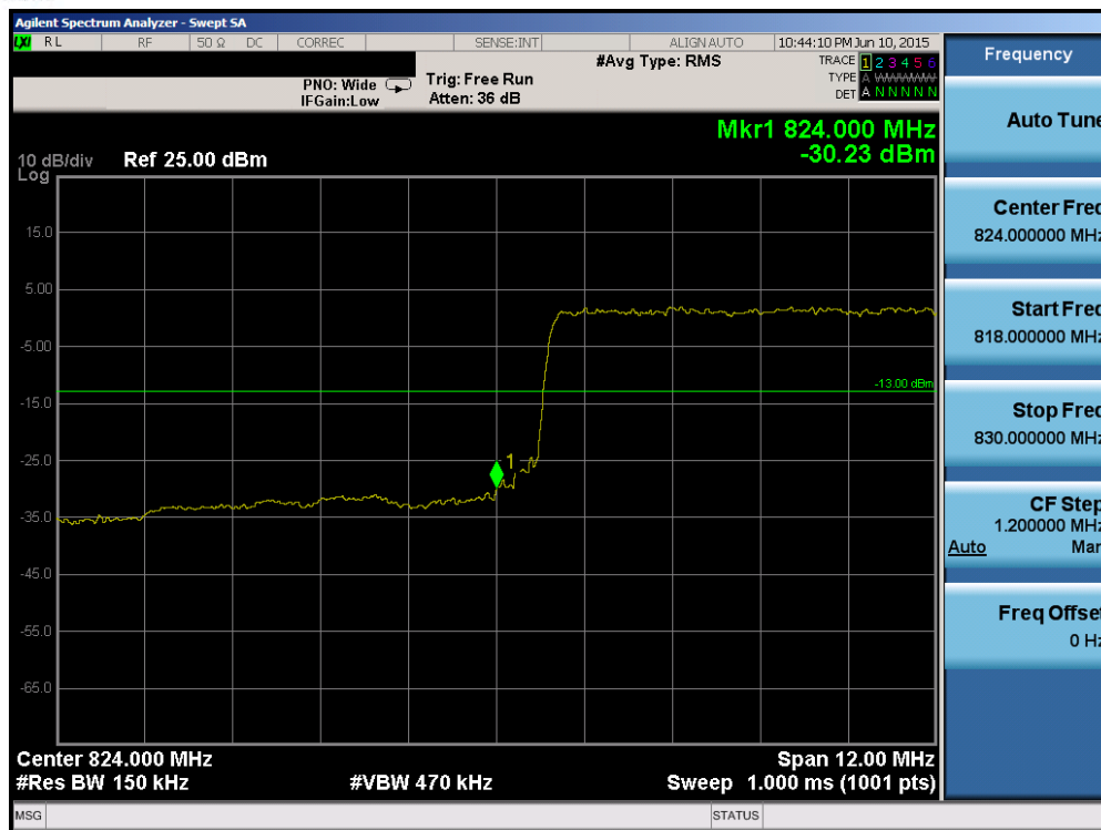
Plot 6-107. Lower Band Edge Plot (Band 26 – 15.0MHz QPSK – RB Size 75)
