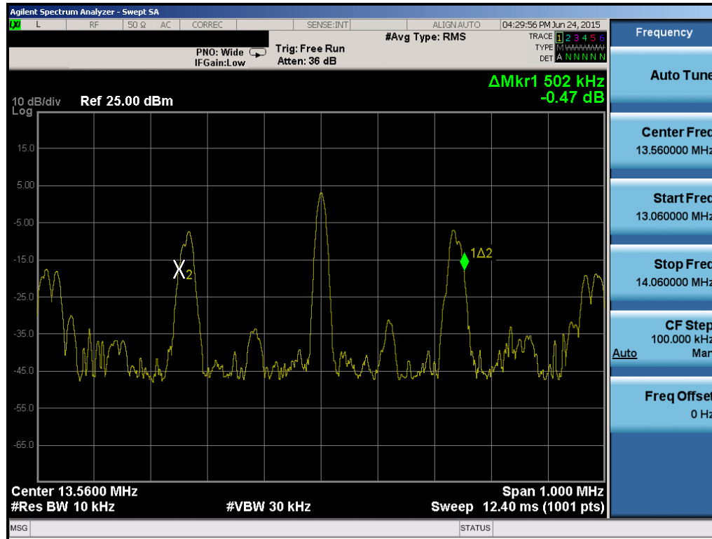
Figure 7-3. 20dB Bandwidth Plot with WCP
