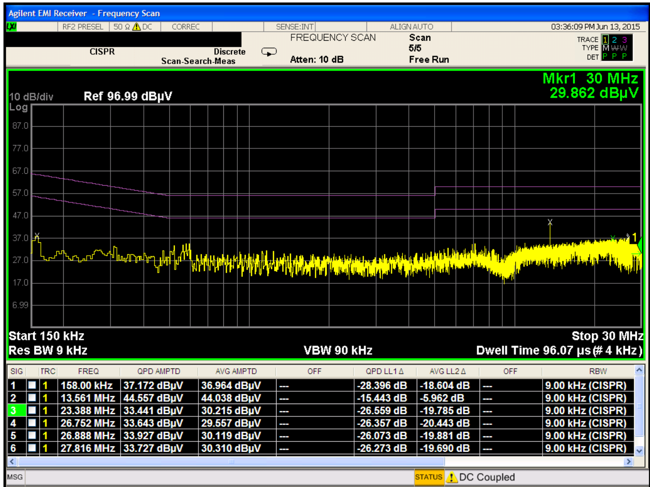
Plot 7-2. Line-Conducted Test Plot (N)
