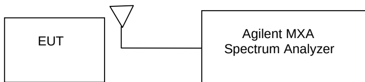
Figure 7-1. Test Instrument & Measurement Setup
