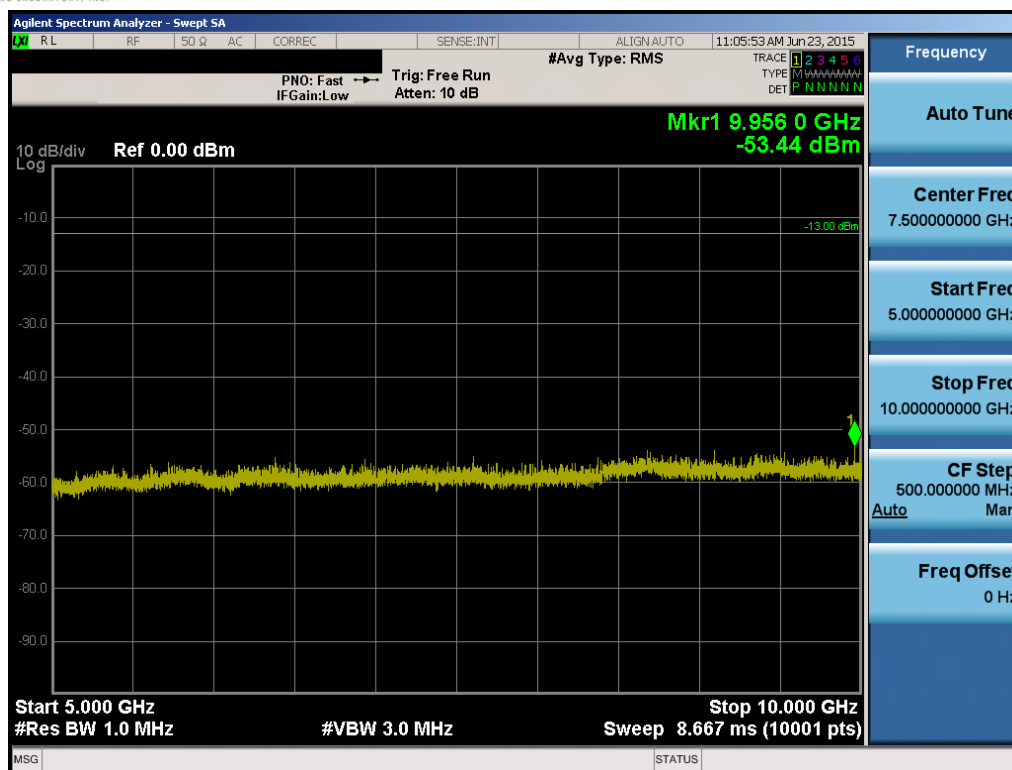
Plot 7-7. Conducted Spurious Plot (1.4MHz QPSK – RB Size 1, RB Offset 0 – High Channel)
