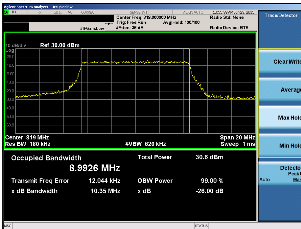
Plot 7-17. Occupied Bandwidth Plot (10MHz QPSK – RB Size 50)
