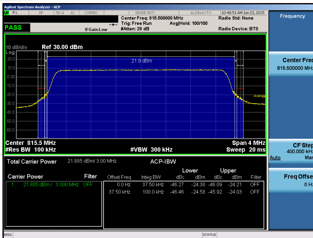
Plot 7-9. Channel Edge Plot (3MHz QPSK – RB Size 15– Low Channel)
