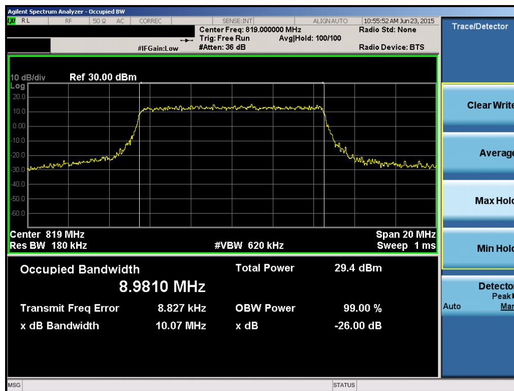
Plot 7-18. Occupied Bandwidth Plot (10MHz 16-QAM – RB Size 50)
