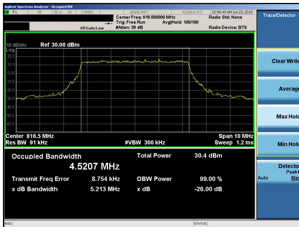
Plot 7-14. Occupied Bandwidth Plot (5MHz QPSK – RB Size 25– Low Channel)
