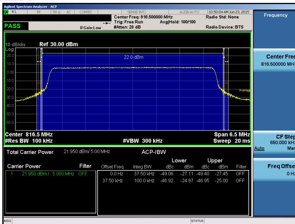
Plot 7-13. Channel Edge Plot (5MHz QPSK – RB Size 25– Low Channel)
