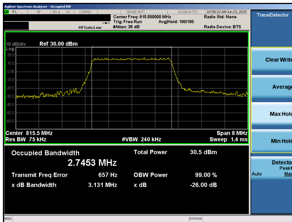
Plot 7-10. Occupied Bandwidth Plot (3MHz QPSK – RB Size 15– Low Channel)
