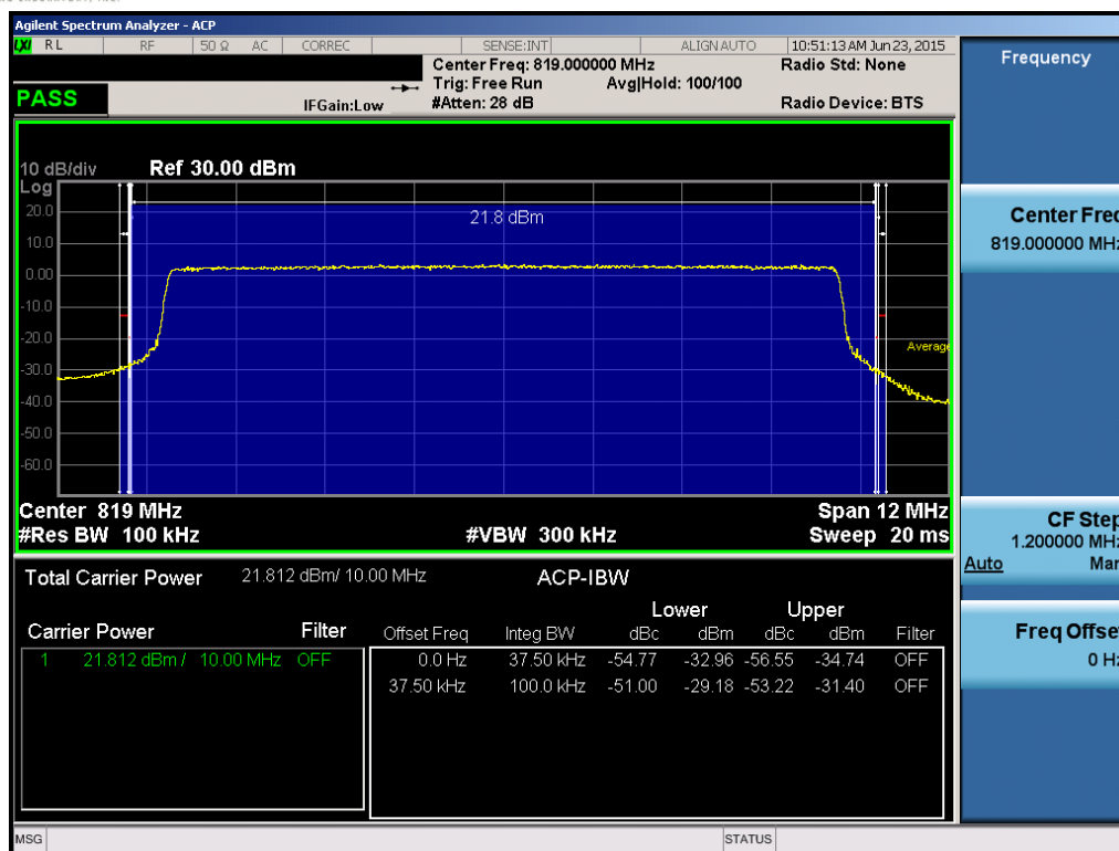
Plot 7-19. Channel Edge Plot (10MHz QPSK – RB Size 50)
