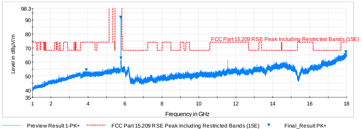
Plot 6-160. Radiated Spurious Plot above 1GHz (802.11a – U3 Ch. 157, Ant. Pol. V)
