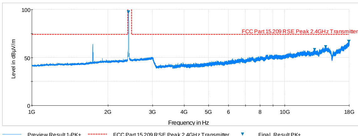
Plot 6-73. Radiated Spurious Plot above 1GHz (802.11b – Ch. 1, Ant. Pol. H)
