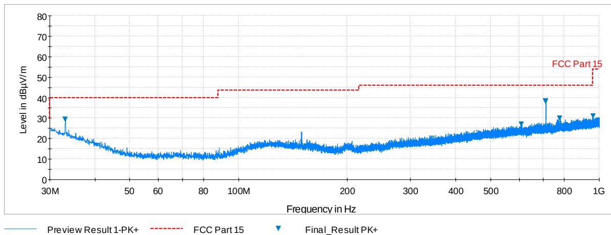
Plot 6-104. Radiated Spurious Plot below 1GHz (Pol. V)
