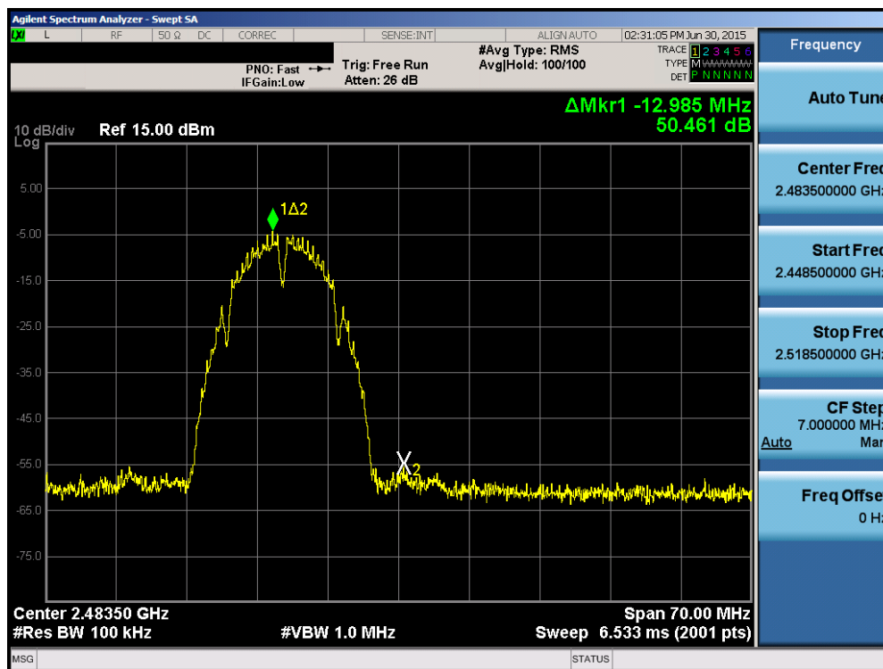
Plot 6-52. Band Edge Plot (802.11b – Ch. 13)
