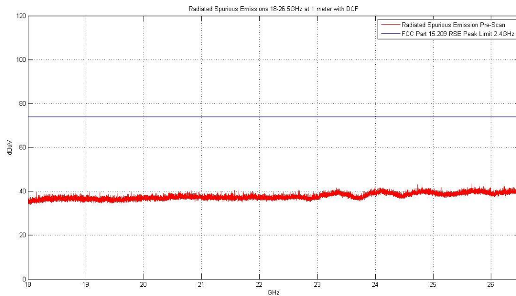
Plot 6-80. Radiated Spurious Plot above 18GHz (Pol. V)
