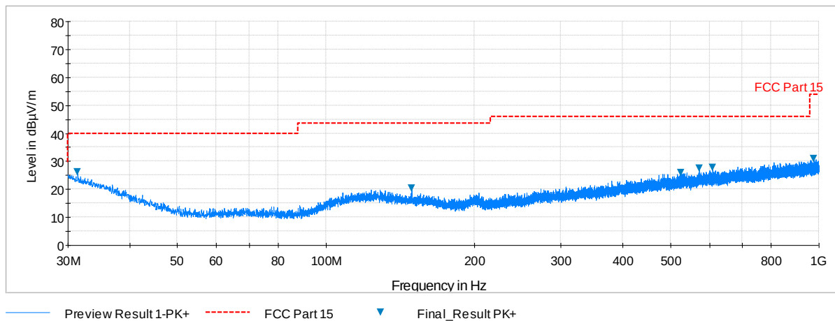
Plot 6-102. Radiated Spurious Plot below 1GHz (Pol. V)
