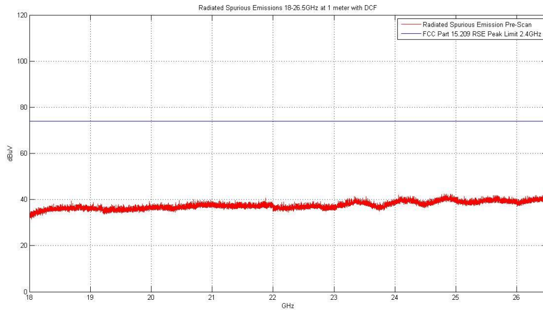
Plot 6-88. Radiated Spurious Plot above 18GHz (Pol. V)
