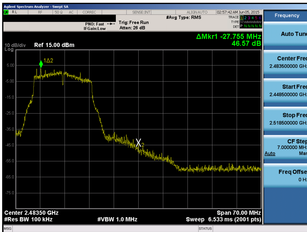
Plot 6-54. Band Edge Plot (802.11g – Ch. 11)
