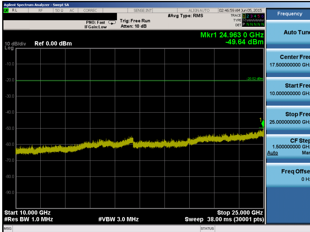
Plot 6-68. Conducted Spurious Plot (802.11b – Ch. 1)
