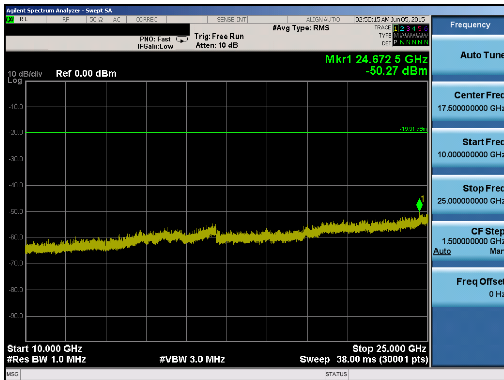
Plot 6-72. Conducted Spurious Plot (802.11b – Ch. 11)
