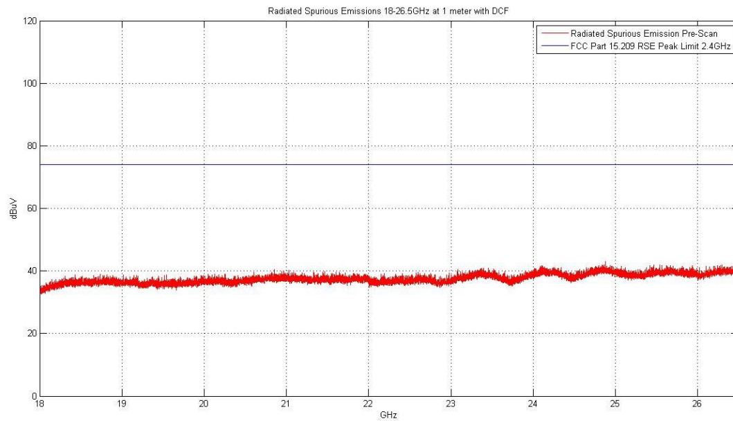
Plot 6-79. Radiated Spurious Plot above 18GHz (Pol. H)
