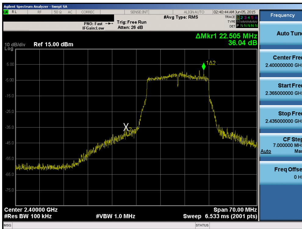
Plot 6-45. Band Edge Plot (802.11n (2.4GHz) – Ch. 1)
