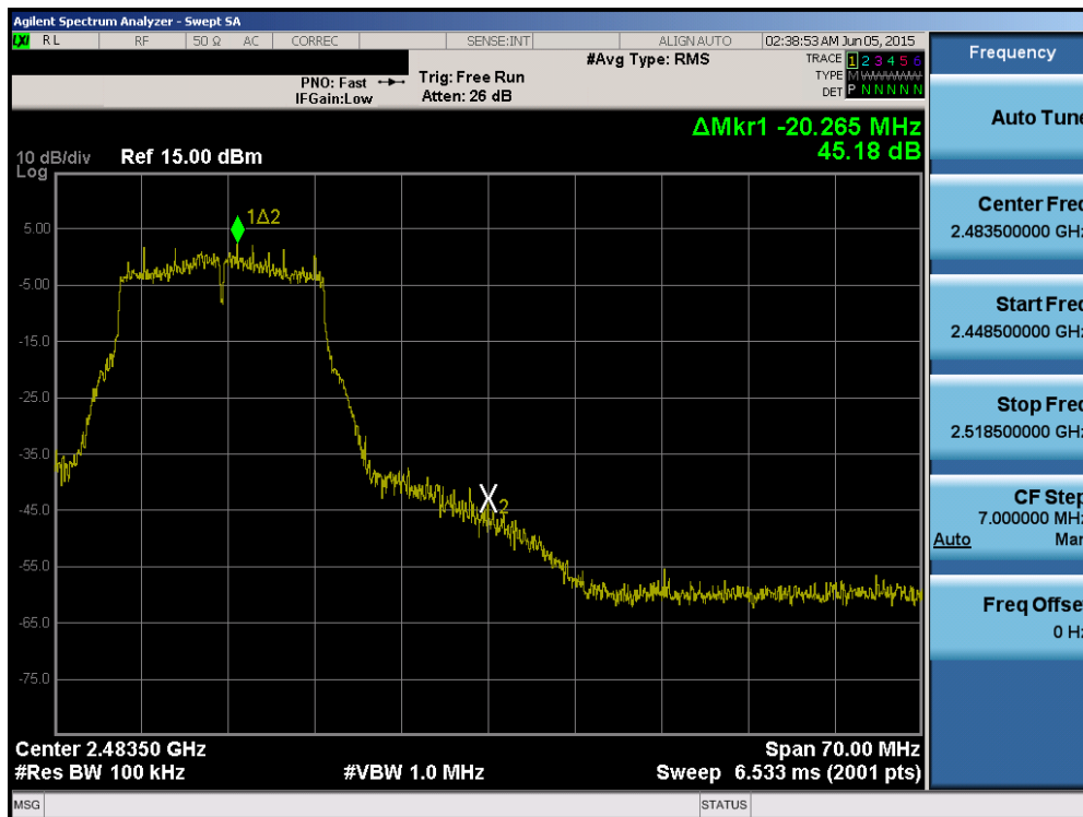
Plot 6-42. Band Edge Plot (802.11g – Ch. 11)
