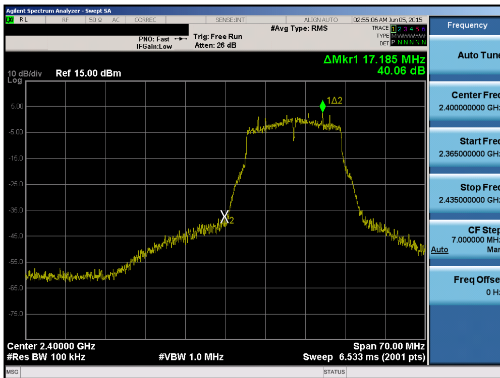
Plot 6-53. Band Edge Plot (802.11g– Ch. 1)
