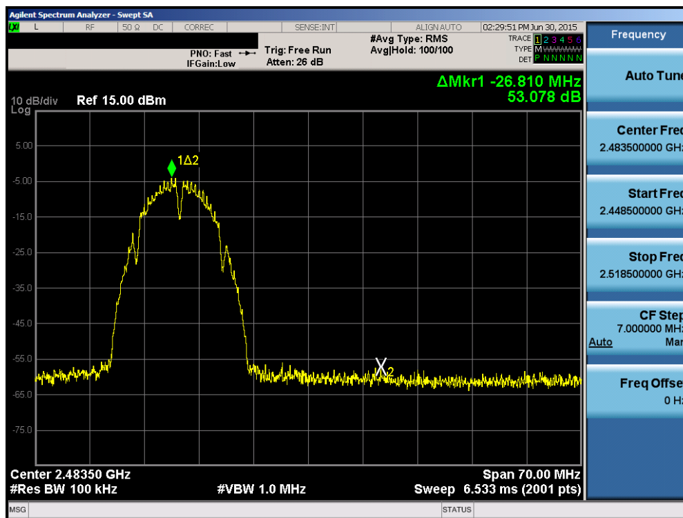
Plot 6-51. Band Edge Plot (802.11b – Ch. 12)
