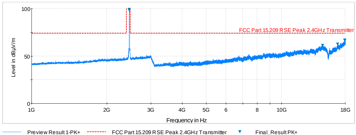
Plot 6-77. Radiated Spurious Plot above 1GHz (802.11b – Ch. 11, Ant. Pol. H)
