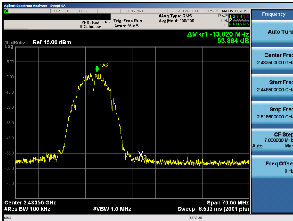
Plot 6-40. Band Edge Plot (802.11b – Ch. 13)
