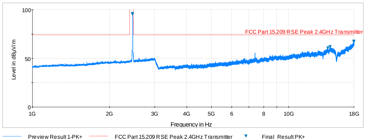
Plot 6-86. Radiated Spurious Plot above 1GHz (802.11b – Ch. 11, Ant. Pol. V)
