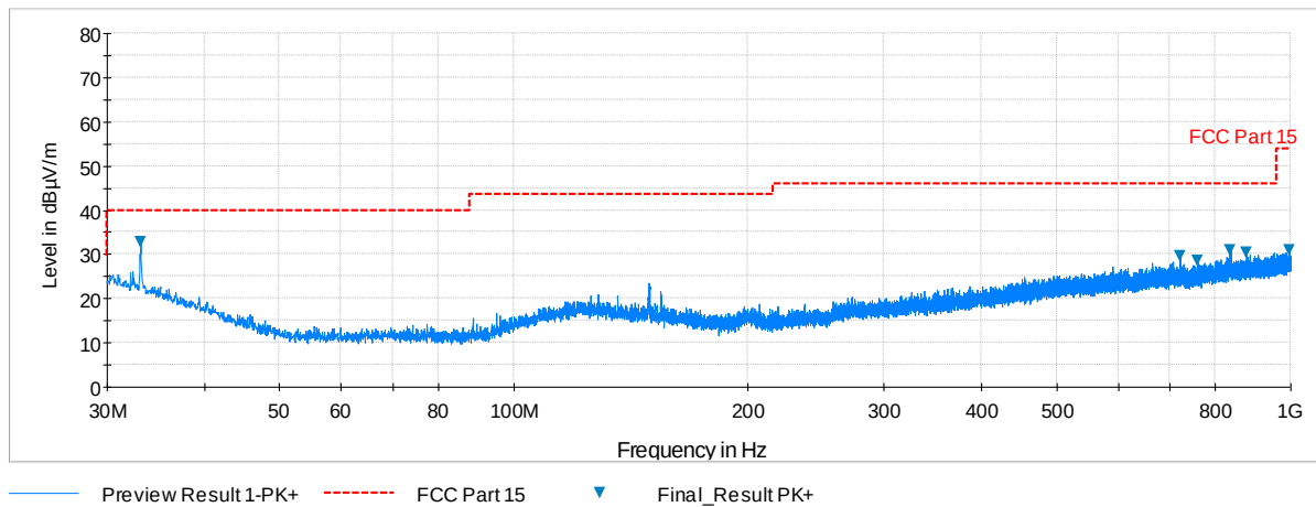
Plot 6-101. Radiated Spurious Plot below 1GHz (Pol. H)
