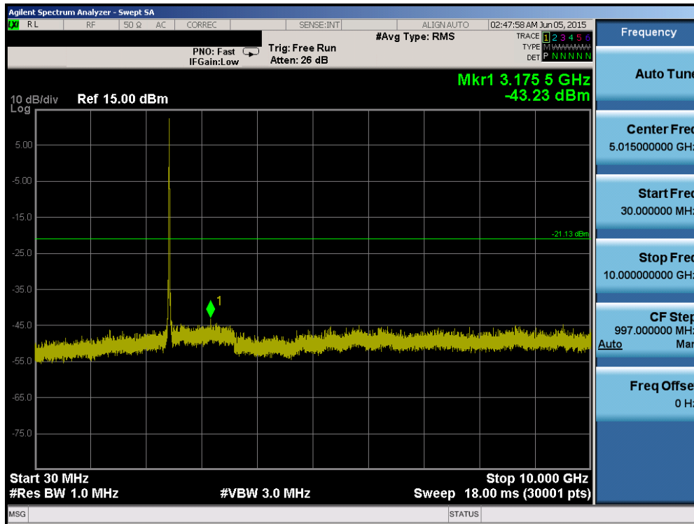
Plot 6-69. Conducted Spurious Plot (802.11b – Ch. 6)
