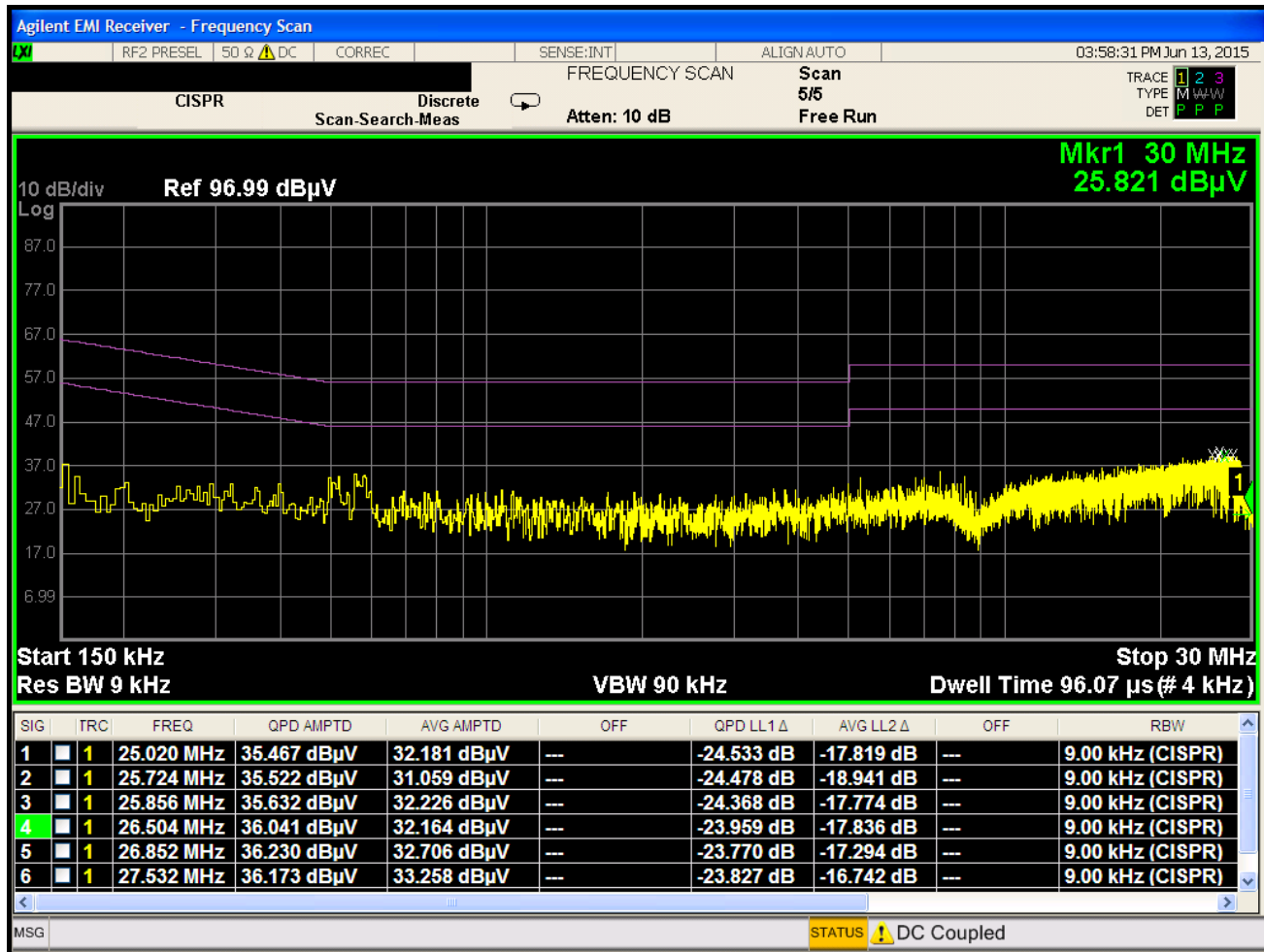
Plot 6-106. Line Conducted Plot with 802.11b (N)
