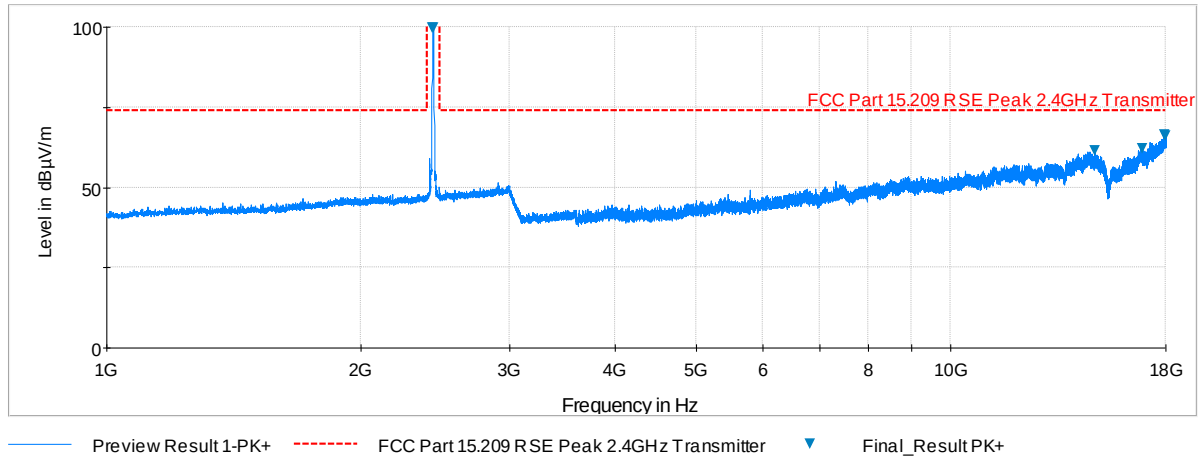
Plot 6-76. Radiated Spurious Plot above 1GHz (802.11b – Ch. 6, Ant. Pol. V)
