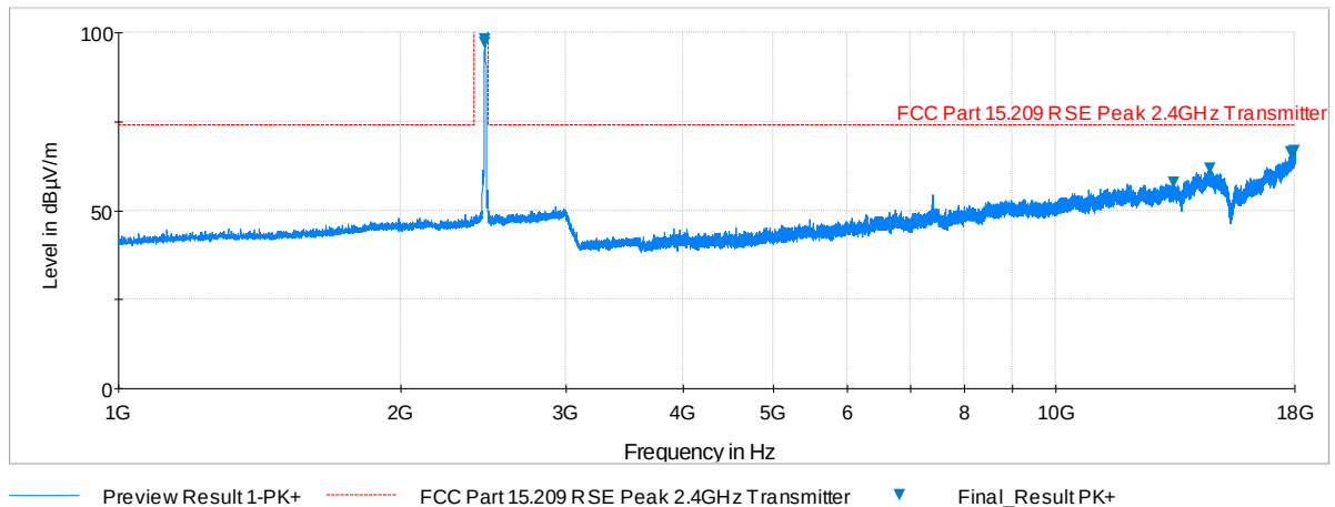
Plot 6-85. Radiated Spurious Plot above 1GHz (802.11b – Ch. 11, Ant. Pol. H)
