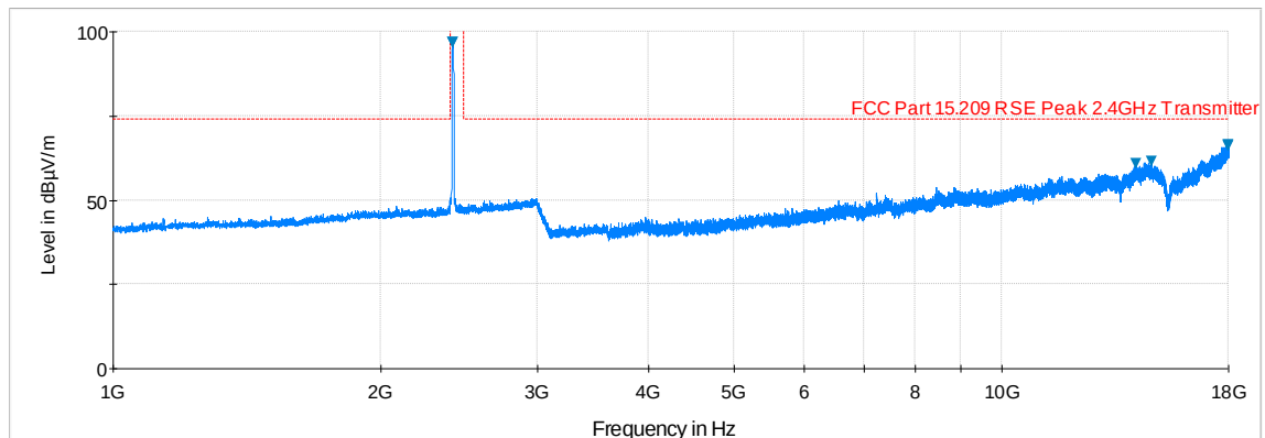
Plot 6-82. Radiated Spurious Plot above 1GHz (802.11b – Ch. 1, Ant. Pol. V)
