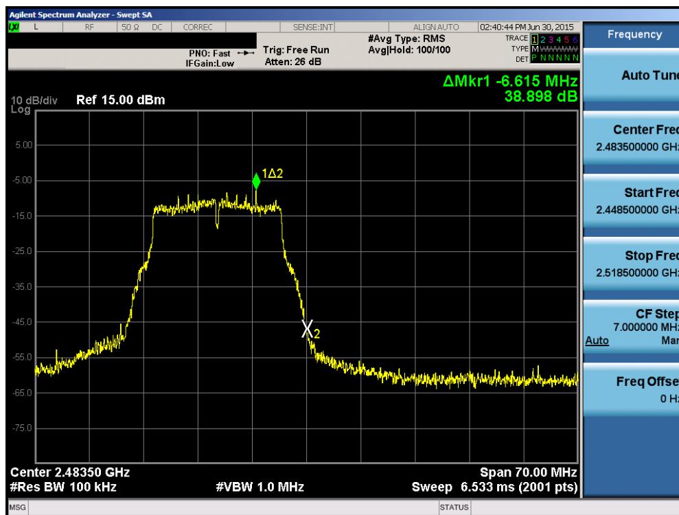
Plot 6-56. Band Edge Plot (802.11g – Ch. 13)
