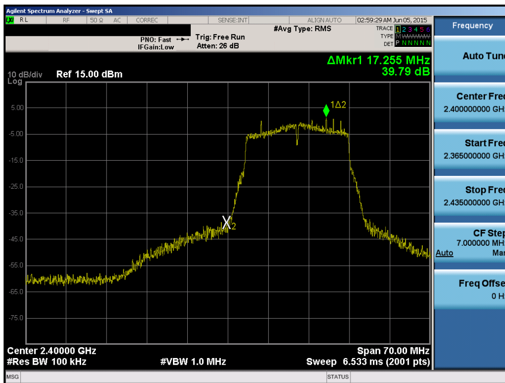
Plot 6-57. Band Edge Plot (802.11n (2.4GHz) – Ch. 1)
