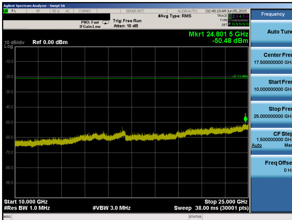
Plot 6-70. Conducted Spurious Plot (802.11b – Ch. 6)
