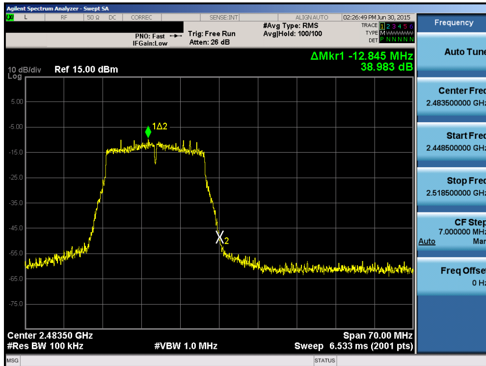
Plot 6-48. Band Edge Plot (802.11n (2.4GHz) – Ch. 13)
