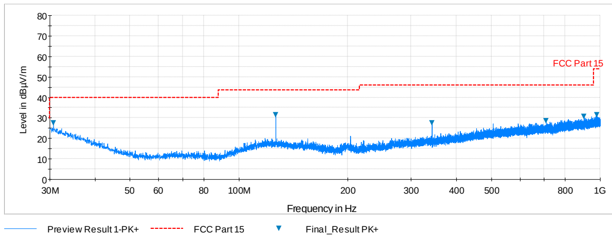
Plot 6-103. Radiated Spurious Plot below 1GHz (Pol. H)
