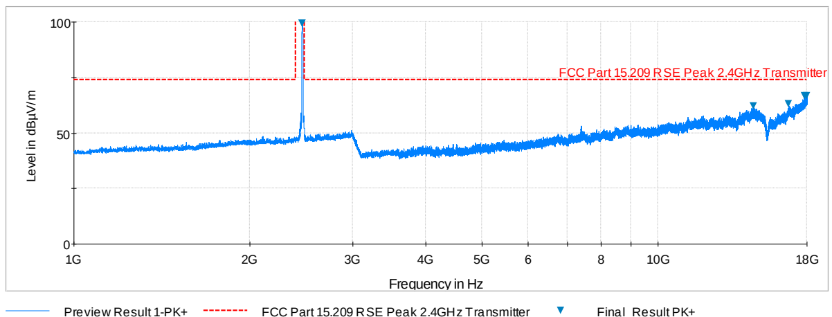
Plot 6-78. Radiated Spurious Plot above 1GHz (802.11b – Ch. 11, Ant. Pol. V)
