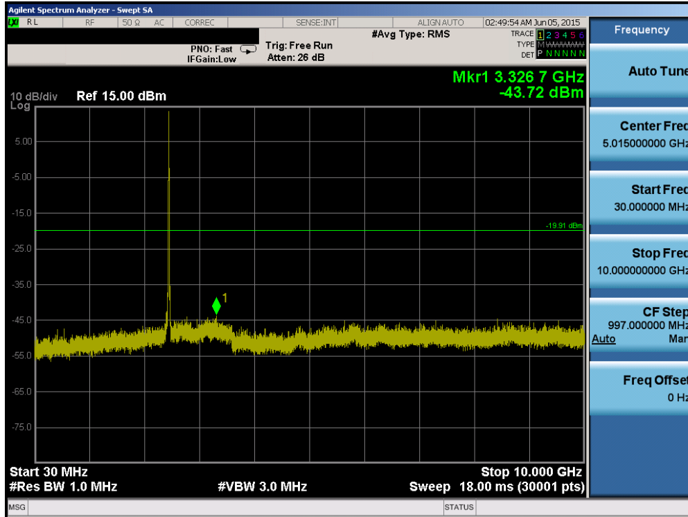
Plot 6-71. Conducted Spurious Plot (802.11b – Ch. 11)
