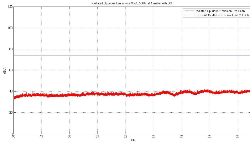
Plot 6-87. Radiated Spurious Plot above 18GHz (Pol. H)
