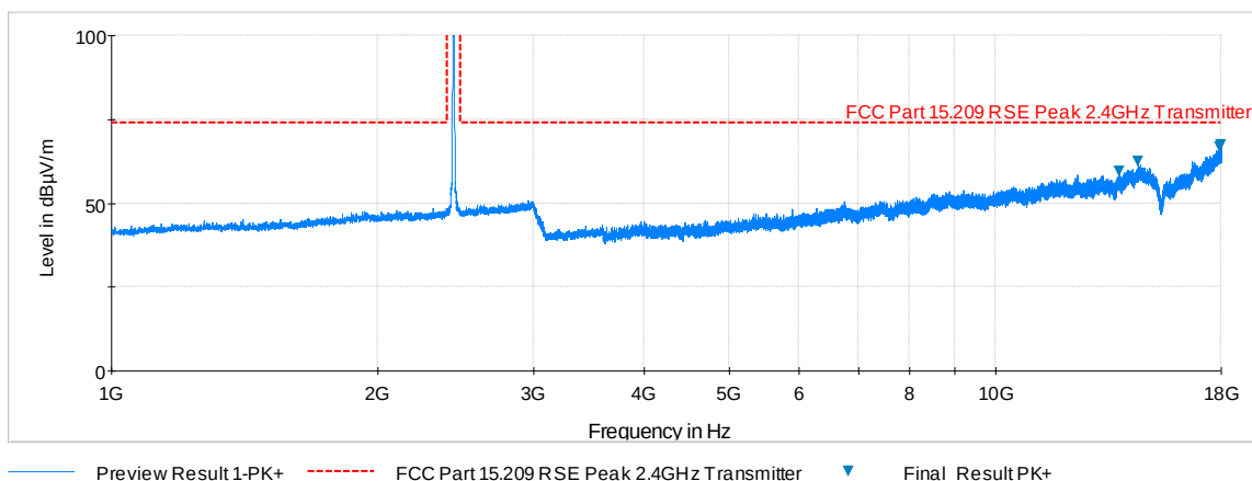
Plot 6-75. Radiated Spurious Plot above 1GHz (802.11b – Ch. 6, Ant. Pol. H)
