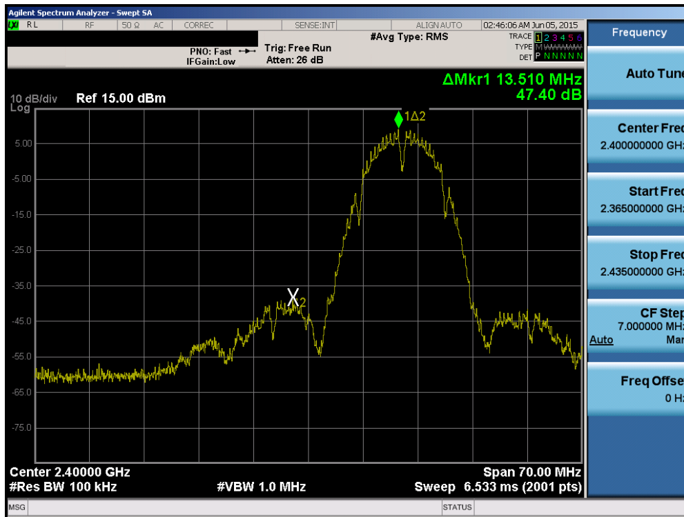
Plot 6-49. Band Edge Plot (802.11b – Ch. 1)
