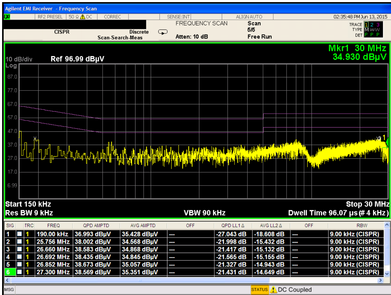
Plot 6-105. Line Conducted Plot with 802.11b (L1)
