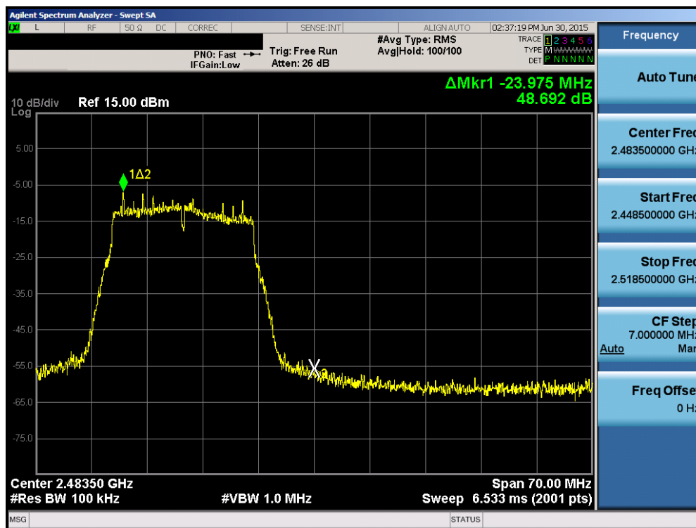
Plot 6-59. Band Edge Plot (802.11n (2.4GHz) – Ch. 12)
