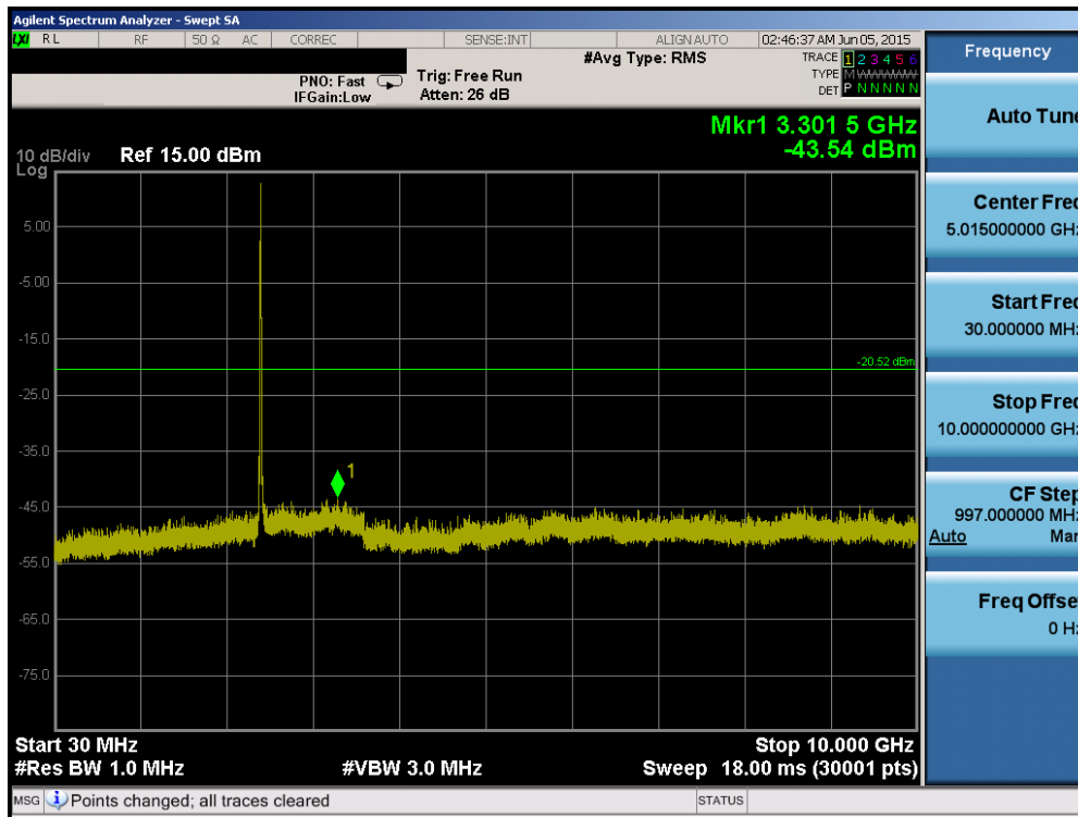
Plot 6-67. Conducted Spurious Plot (802.11b – Ch. 1)
