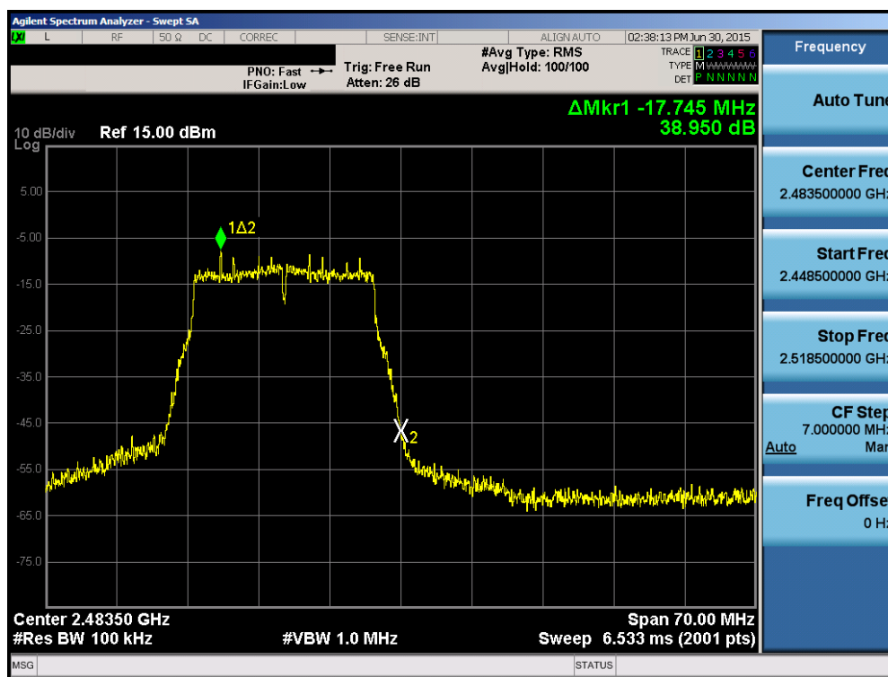
Plot 6-60. Band Edge Plot (802.11n (2.4GHz) – Ch. 13)
