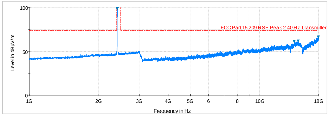
Plot 6-81. Radiated Spurious Plot above 1GHz (802.11b – Ch. 1, Ant. Pol. H)
