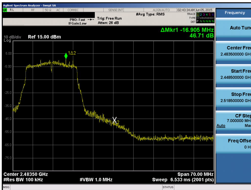
Plot 6-46. Band Edge Plot (802.11n (2.4GHz) – Ch. 11)
