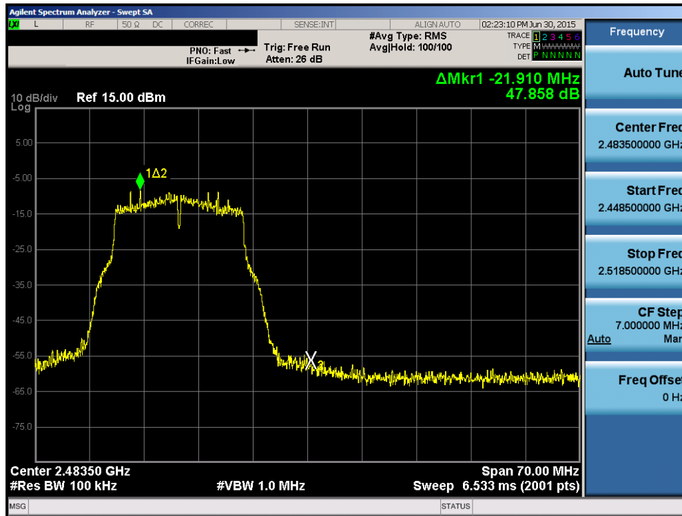
Plot 6-43. Band Edge Plot (802.11g – Ch. 12)
