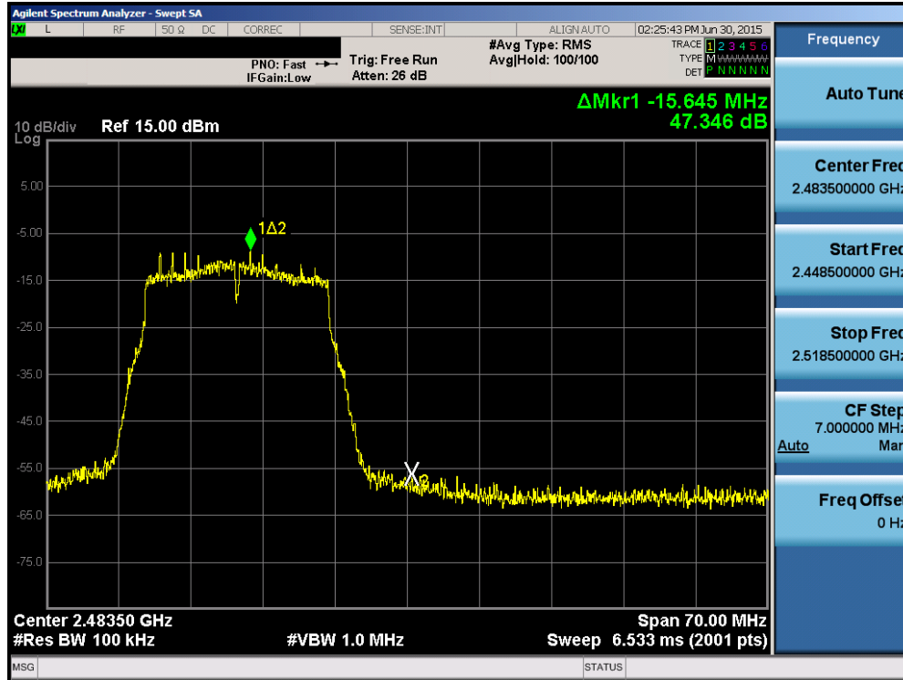
Plot 6-47. Band Edge Plot (802.11n (2.4GHz) – Ch. 12)
