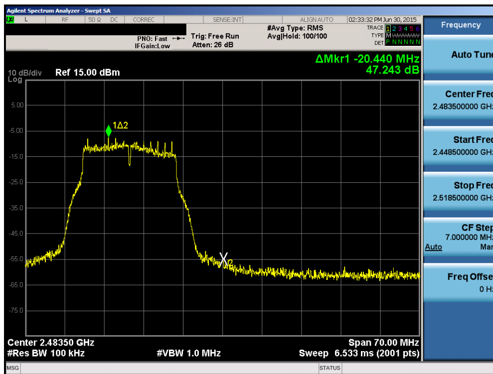
Plot 6-55. Band Edge Plot (802.11g – Ch. 12)
