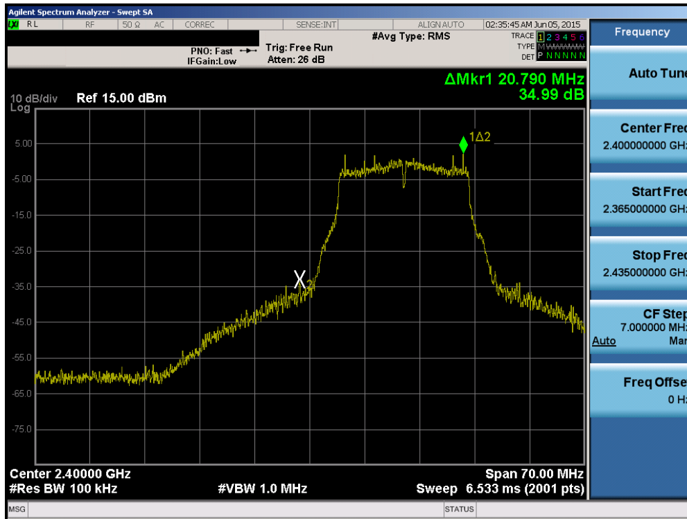
Plot 6-41. Band Edge Plot (802.11g– Ch. 1)
