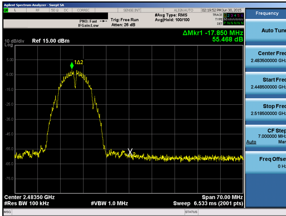
Plot 6-39. Band Edge Plot (802.11b – Ch. 12)
