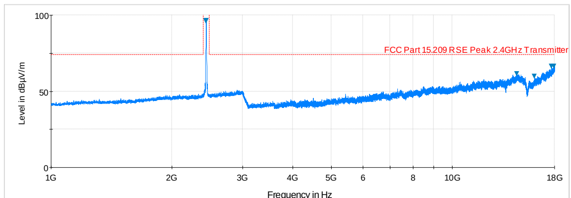
Plot 6-83. Radiated Spurious Plot above 1GHz (802.11b – Ch. 6, Ant. Pol. H)
