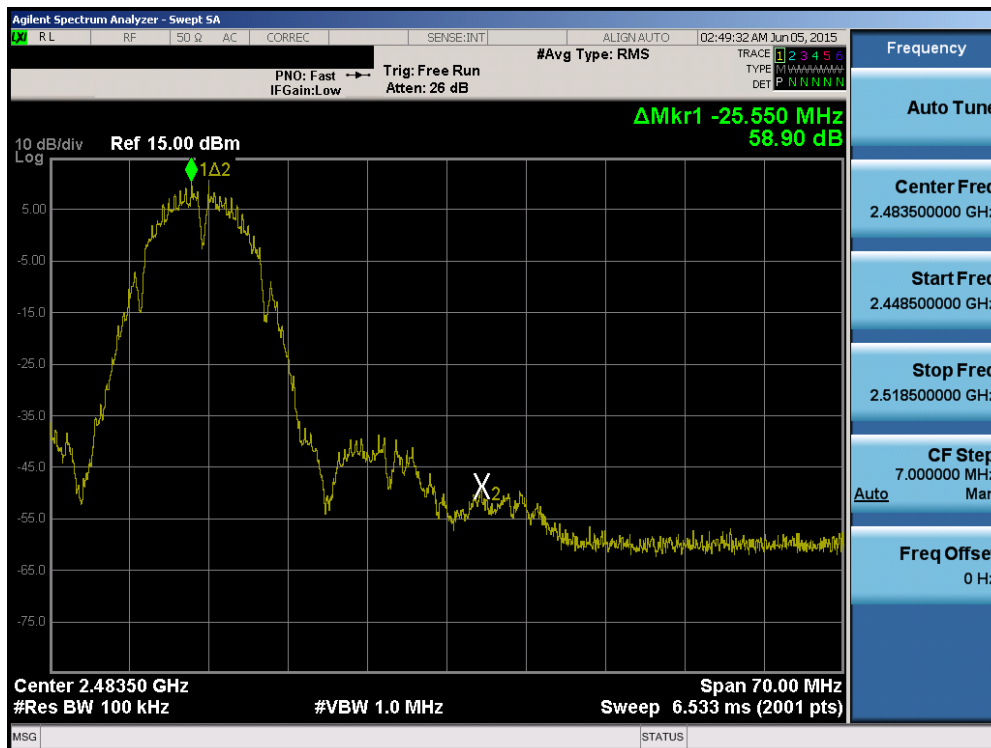
Plot 6-50. Band Edge Plot (802.11b – Ch. 11)
