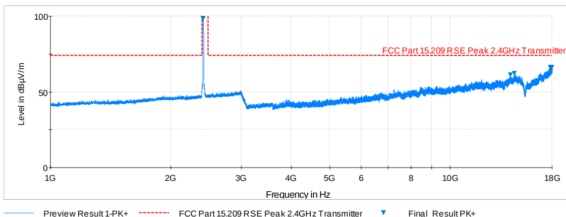
Plot 6-74. Radiated Spurious Plot above 1GHz (802.11b – Ch. 1, Ant. Pol. V)
