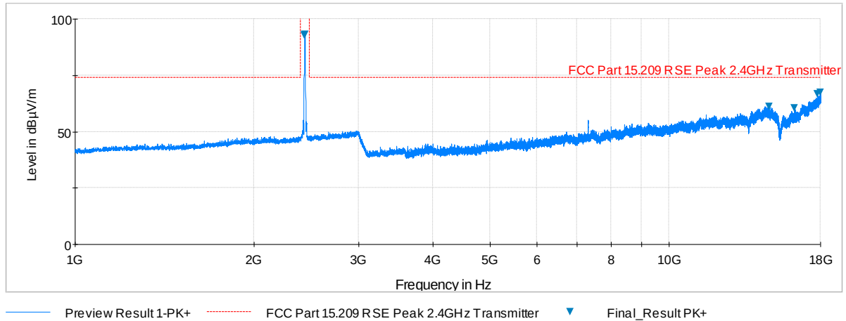
Plot 6-84. Radiated Spurious Plot above 1GHz (802.11b – Ch. 6, Ant. Pol. V)
