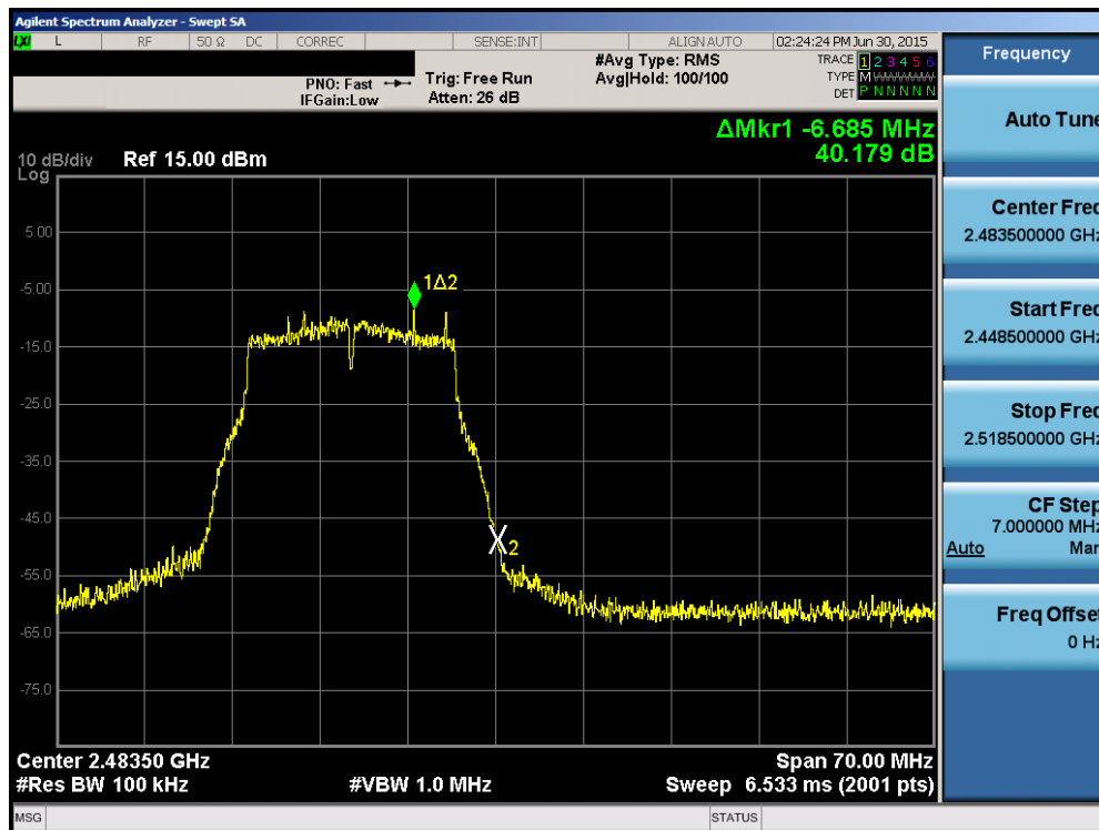
Plot 6-44. Band Edge Plot (802.11g – Ch. 13)
