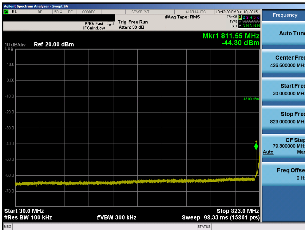
Plot 6-52. Conducted Spurious Plot (Band 5/26 – 10.0MHz QPSK – RB Size 1, RB Offset 0 – Low Channel)
