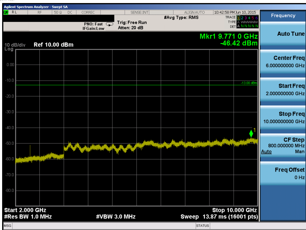
Plot 6-57. Conducted Spurious Plot (Band 5/26 – 10.0MHz QPSK – RB Size 1, RB Offset 0 – Mid Channel)
