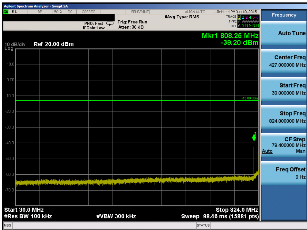
Plot 6-58. Conducted Spurious Plot (Band 5/26 – 10.0MHz QPSK – RB Size 1, RB Offset 0 – High Channel)
