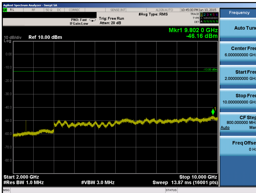
Plot 6-60. Conducted Spurious Plot (Band 5/26 – 10.0MHz QPSK – RB Size 1, RB Offset 0 – High Channel)
