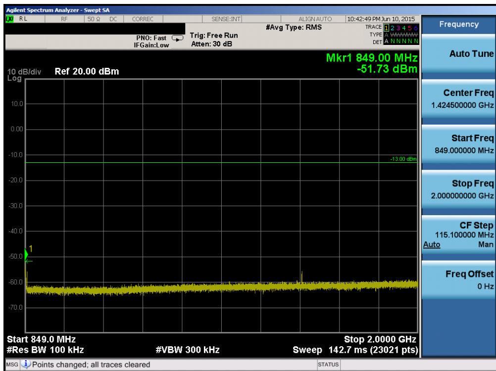
Plot 6-56. Conducted Spurious Plot (Band 5/26 – 10.0MHz QPSK – RB Size 1, RB Offset 0 – Mid Channel)
