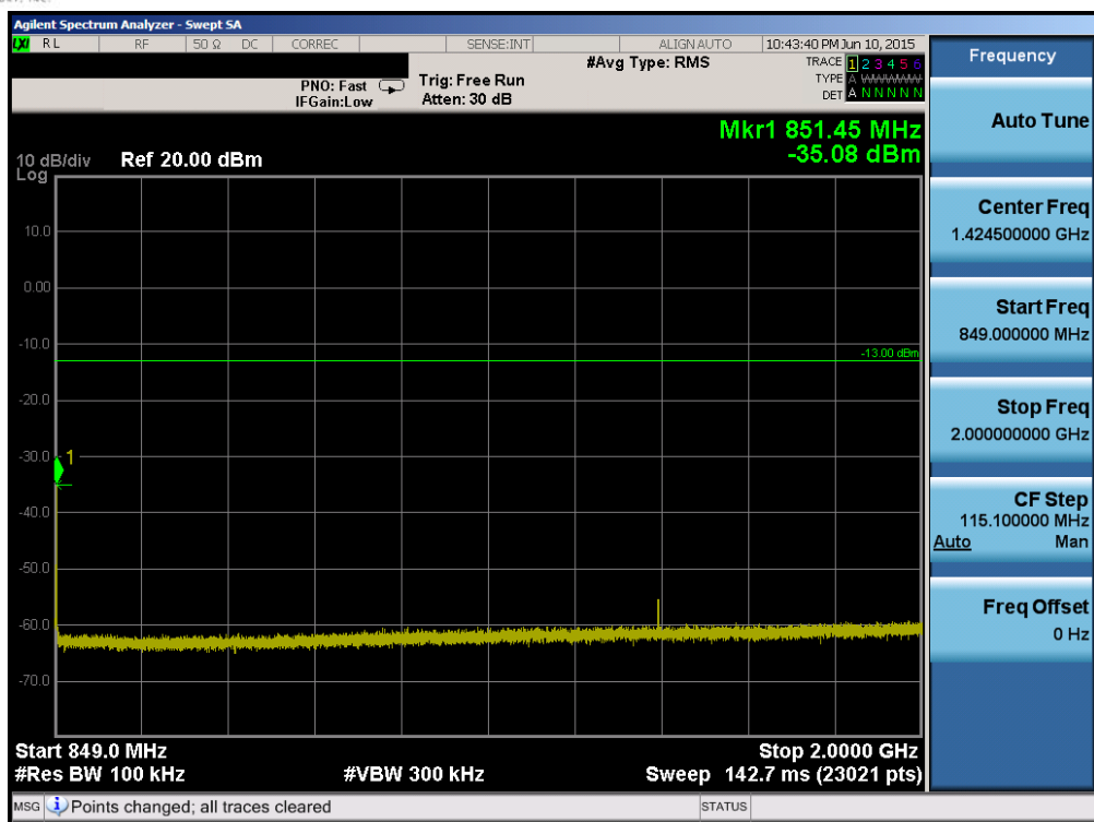
Plot 6-53. Conducted Spurious Plot (Band 5/26 – 10.0MHz QPSK – RB Size 1, RB Offset 0 – Low Channel)
