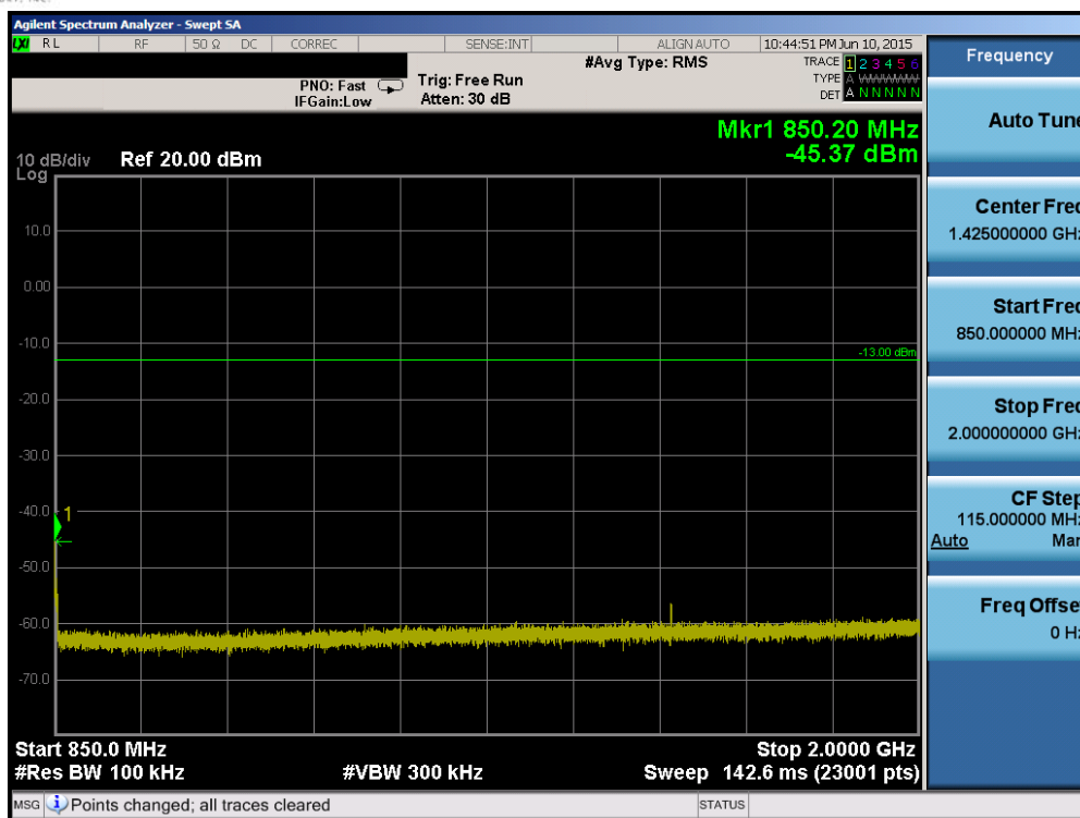
Plot 6-59. Conducted Spurious Plot (Band 5/26 – 10.0MHz QPSK – RB Size 1, RB Offset 0 – High Channel)
