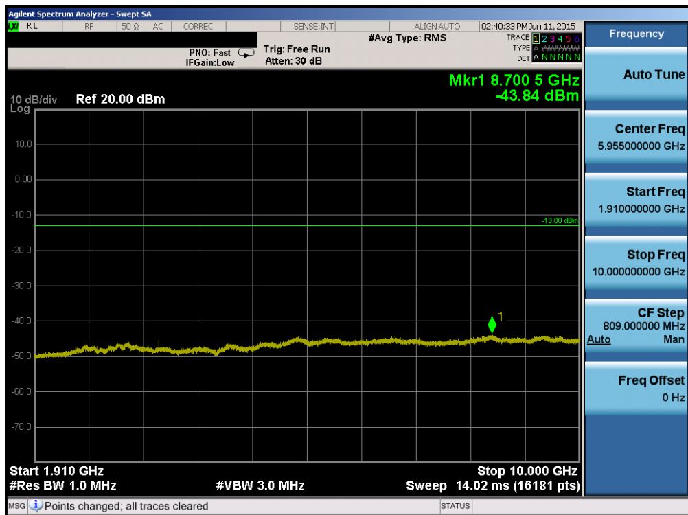
Plot 6-74. Conducted Spurious Plot (Band 2 – 5.0MHz QPSK – RB Size 1, RB Offset 0 – Mid Channel)
