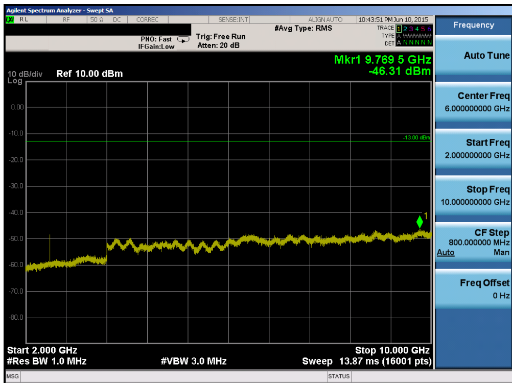
Plot 6-54. Conducted Spurious Plot (Band 5/26 – 10.0MHz QPSK – RB Size 1, RB Offset 0 – Low Channel)
