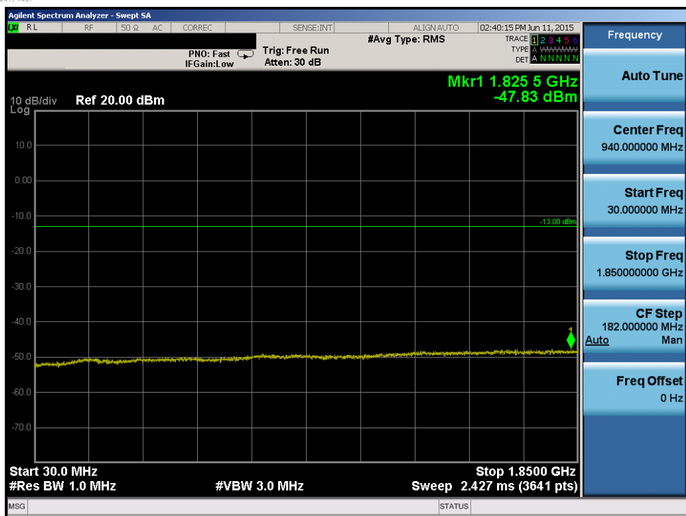
Plot 6-73. Conducted Spurious Plot (Band 2 – 5.0MHz QPSK – RB Size 1, RB Offset 0 – Mid Channel)
