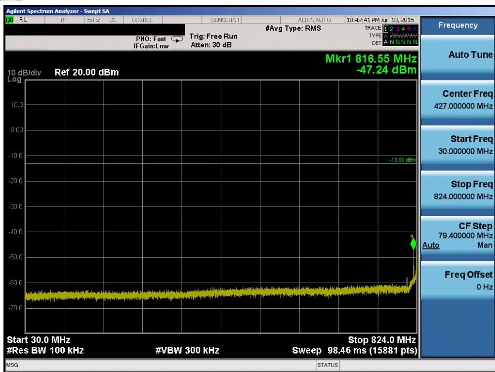
Plot 6-55. Conducted Spurious Plot (Band 5/26 – 10.0MHz QPSK – RB Size 1, RB Offset 0 – Mid Channel)
