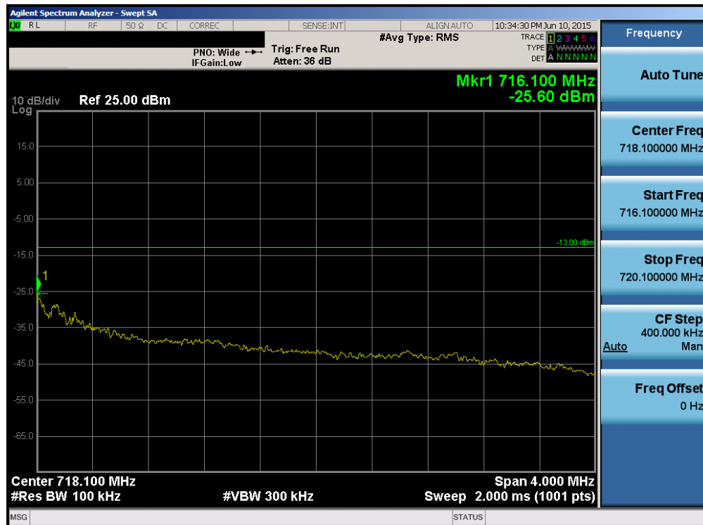
Plot 6-90. Upper Extended Band Edge Plot (Band 12/17 – 5.0MHz QPSK – RB Size 25)
