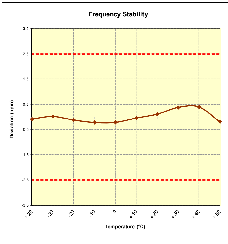
Figure 6-7. Frequency Stability Graph (Band 12/17)
