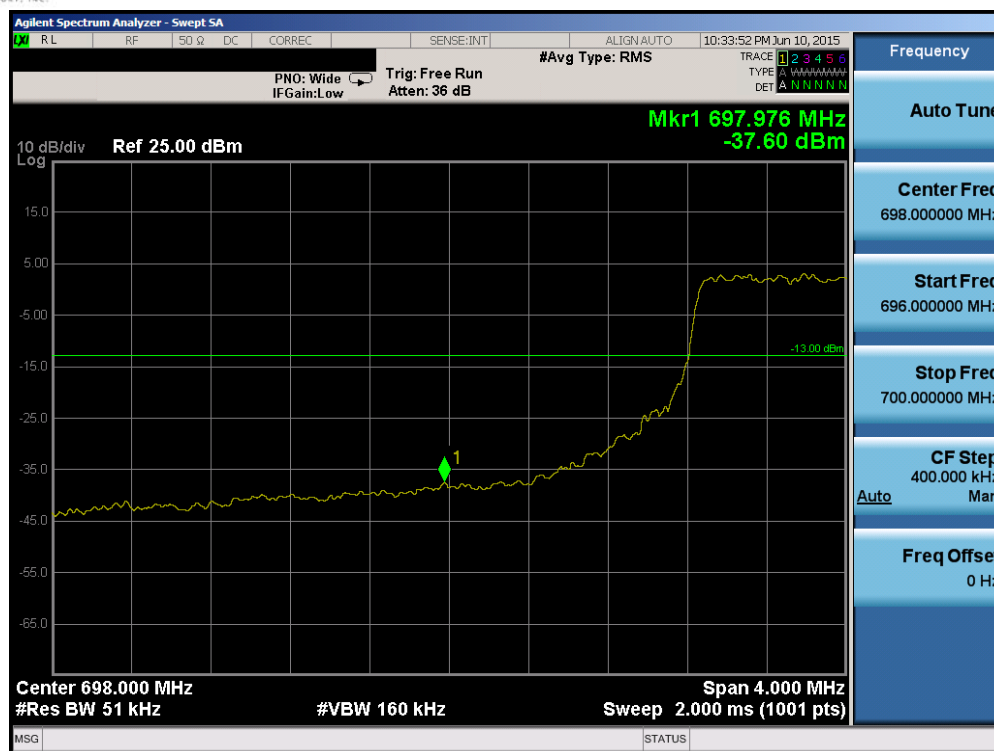
Plot 6-87. Lower Band Edge Plot (Band 12/17 – 5.0MHz QPSK – RB Size 25)
