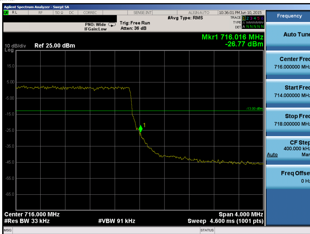
Plot 6-85. Upper Band Edge Plot (Band 12 – 3.0MHz QPSK – RB Size 15)
