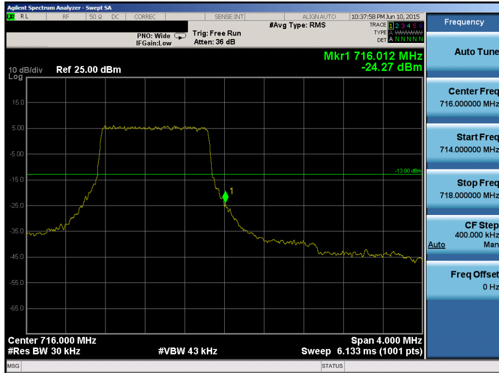
Plot 6-81. Upper Band Edge Plot (Band 12 – 1.4MHz QPSK – RB Size 6)
