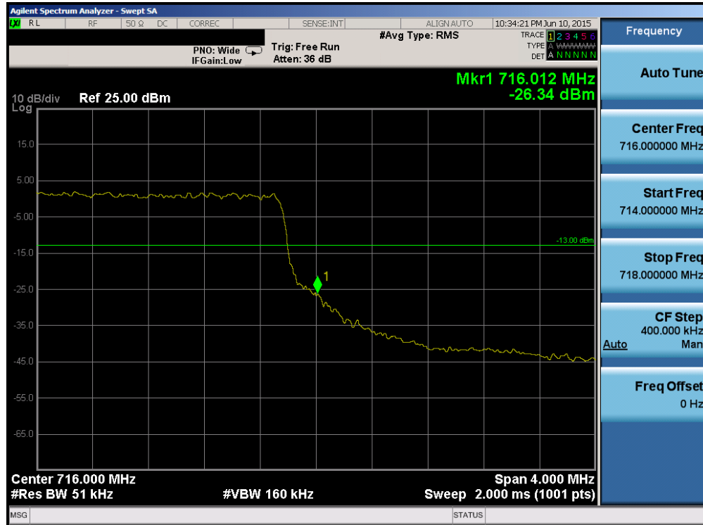
Plot 6-89. Upper Band Edge Plot (Band 12/17 – 5.0MHz QPSK – RB Size 25)
