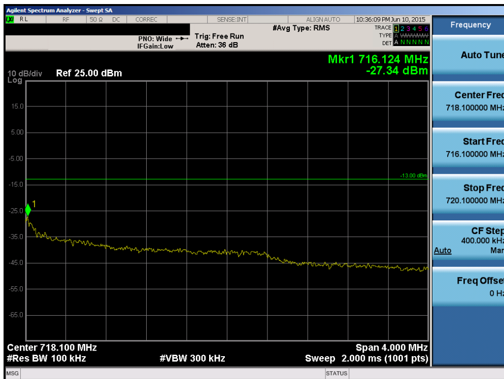
Plot 6-86. Upper Extended Band Edge Plot (Band 12 – 3.0MHz QPSK – RB Size 15)
