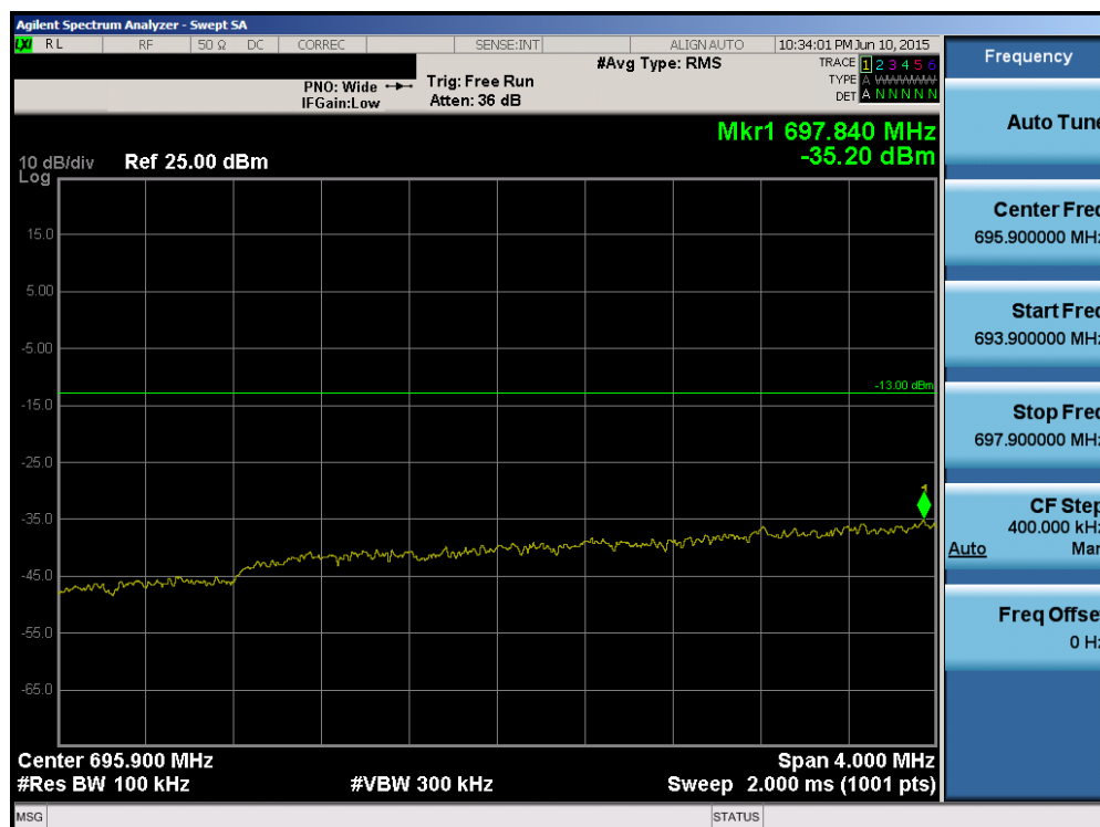
Plot 6-88. Lower Extended Band Edge Plot (Band 12/17 – 5.0MHz QPSK – RB Size 25)
