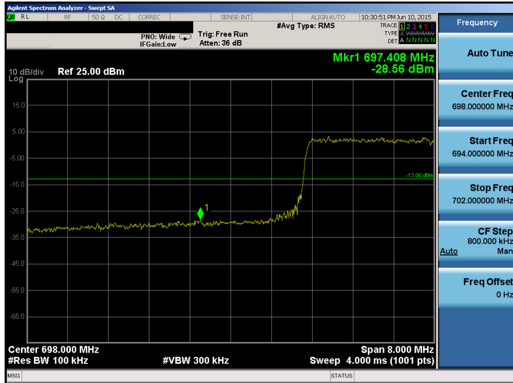
Plot 6-91. Lower Band Edge Plot (Band 12/17 – 10.0MHz QPSK – RB Size 50)
