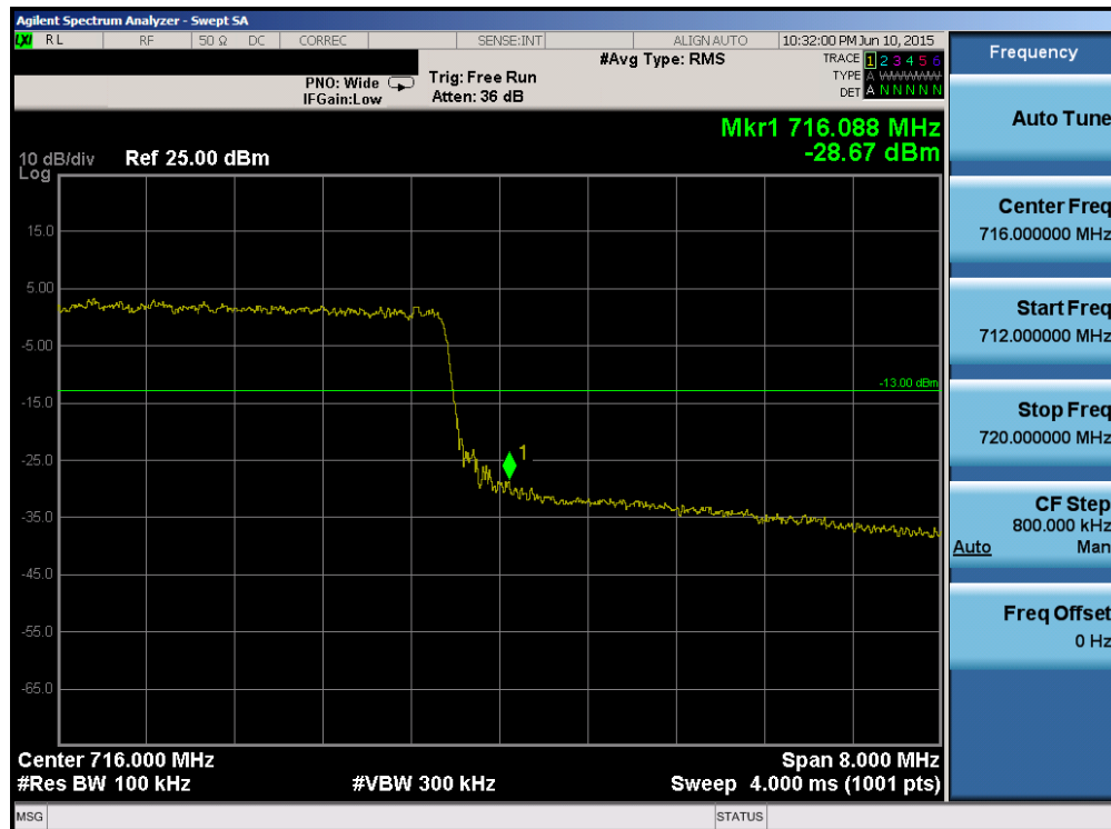
Plot 6-92. Upper Band Edge Plot (Band 12/17 – 10.0MHz QPSK – RB Size 50)
