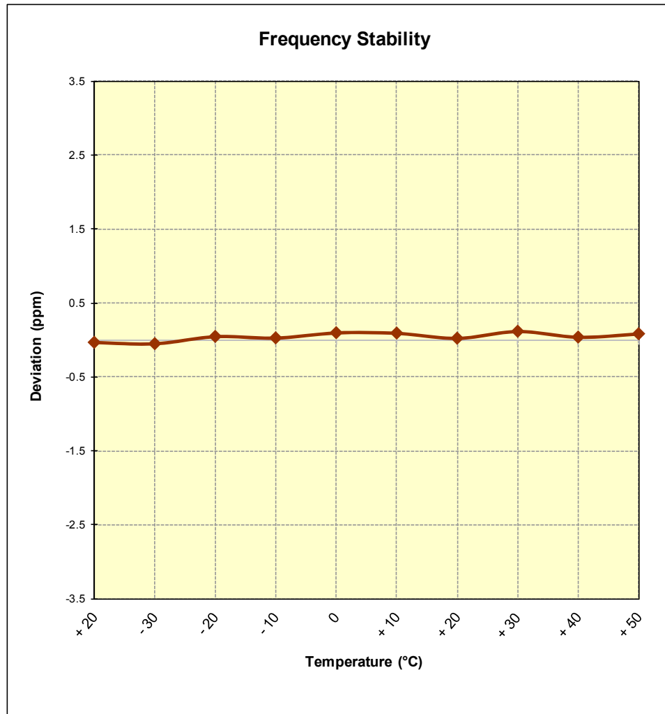
Figure 6-9. Frequency Stability Graph (PCS GSM Mode – Ch. 661)
