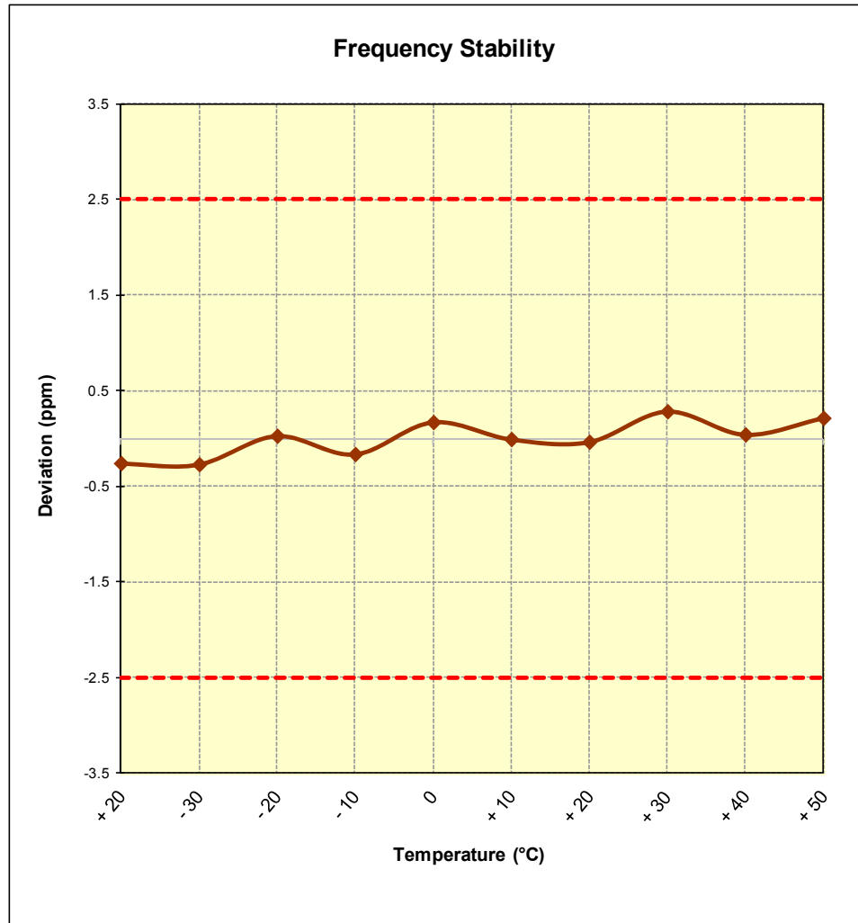
Figure 6-8. Frequency Stability Graph (Cellular WCDMA Mode – Ch. 4183)
