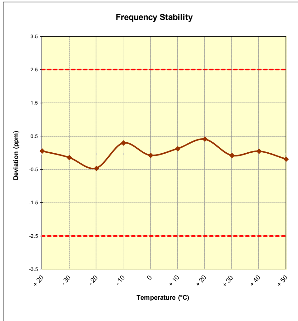
Figure 6-7. Frequency Stability Graph (Cellular GSM Mode – Ch. 190)
