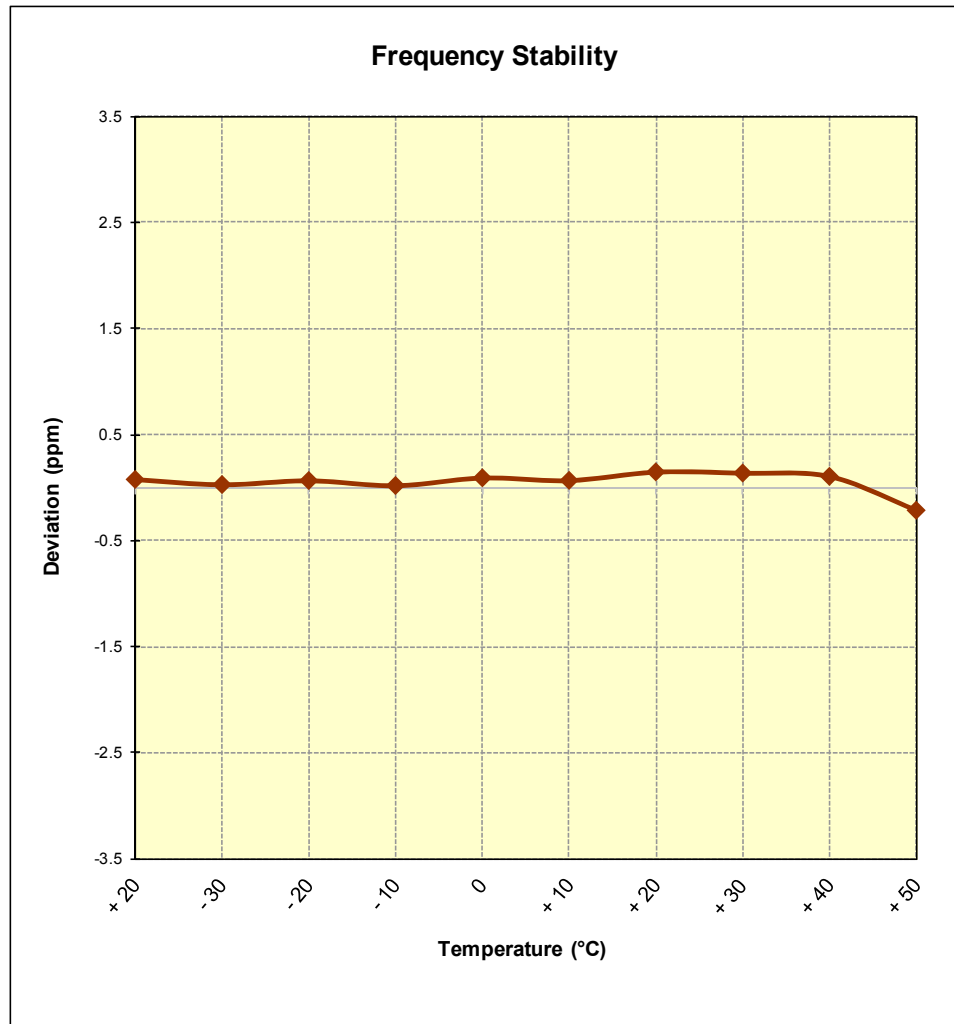
Figure 6-10. Frequency Stability Graph (PCS WCDMA Mode – Ch. 9400)
