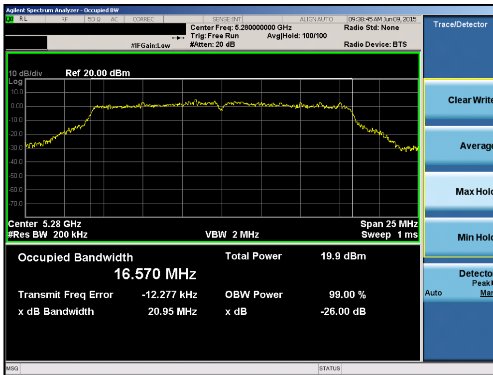
Plot 6-40. 26dB Bandwidth Plot (802.11a (UNII Band 2A) – Ch. 56)
