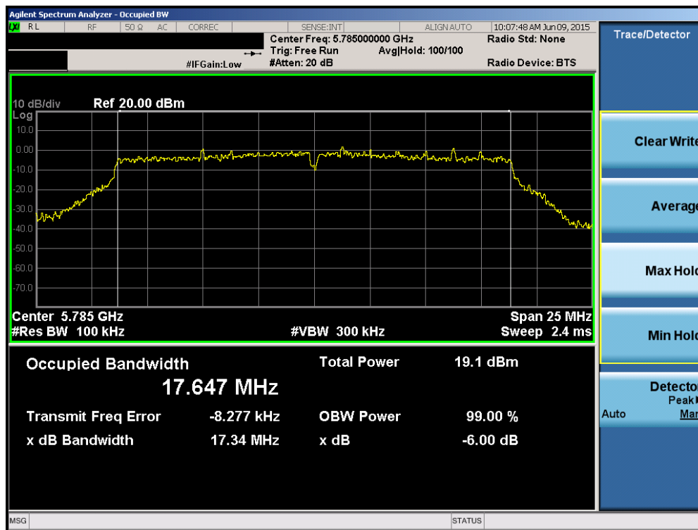
Plot 6-72. 6dB Bandwidth Plot (20MHz BW 802.11n (UNII Band 3) – Ch. 157)
