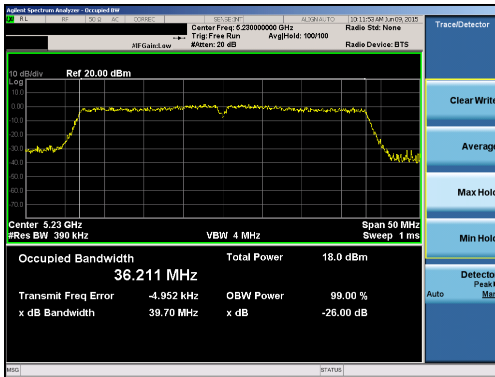
Plot 6-37. 26dB Bandwidth Plot (40MHz BW 802.11n (UNII Band 1) – Ch. 46)
