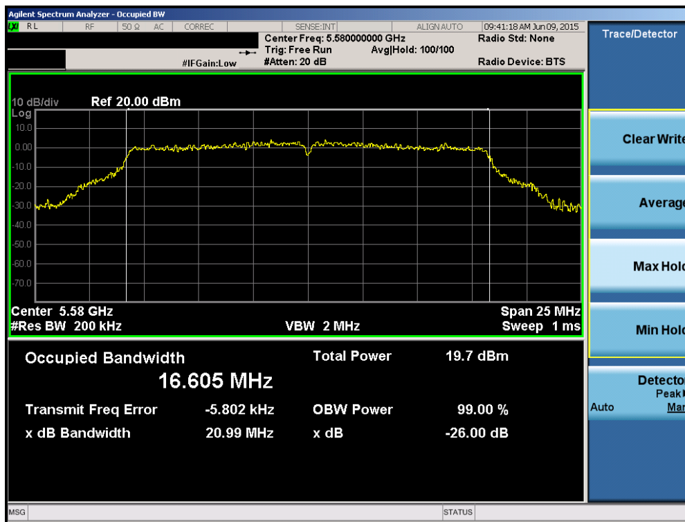
Plot 6-49. 26dB Bandwidth Plot (802.11a (UNII Band 2C) – Ch. 116)
