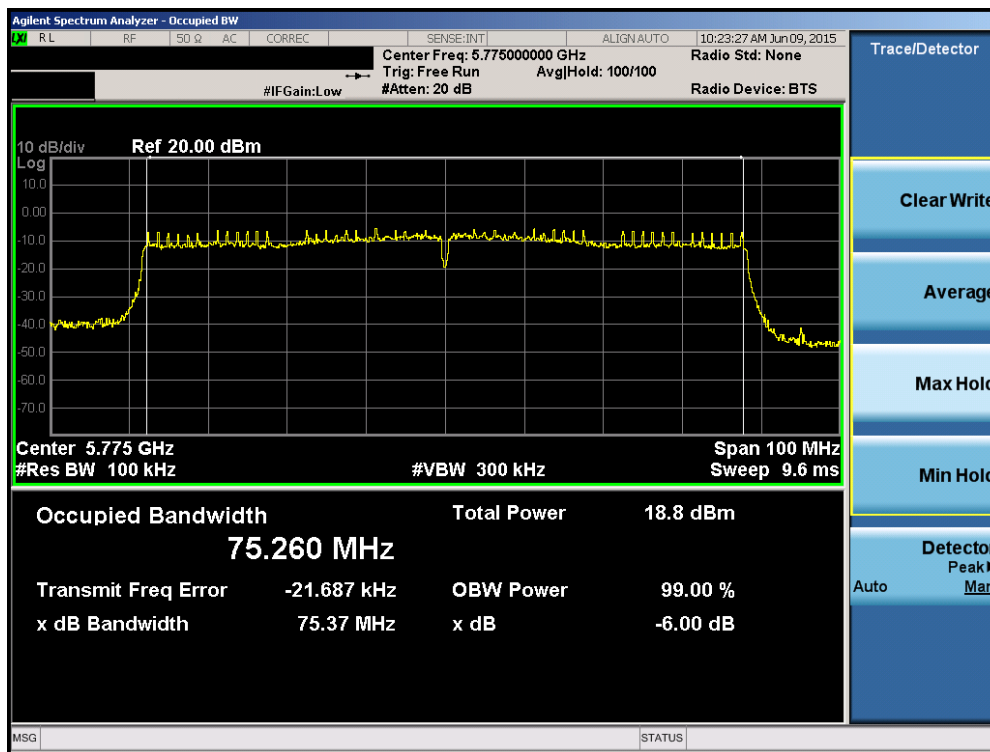
Plot 6-76. 6dB Bandwidth Plot (80MHz BW 802.11ac (UNII Band 3) – Ch. 155)
