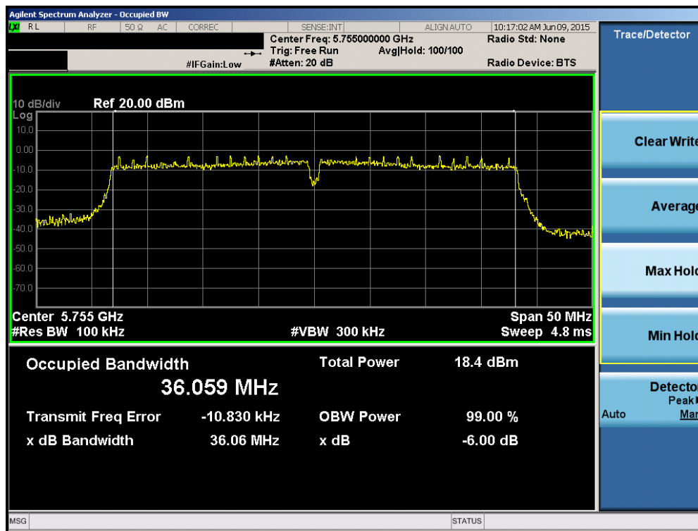
Plot 6-74. 6dB Bandwidth Plot (40MHz BW 802.11n (UNII Band 3) – Ch. 151)
