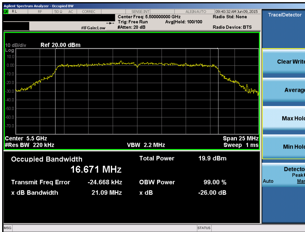
Plot 6-48. 26dB Bandwidth Plot (802.11a (UNII Band 2C) – Ch. 100)
