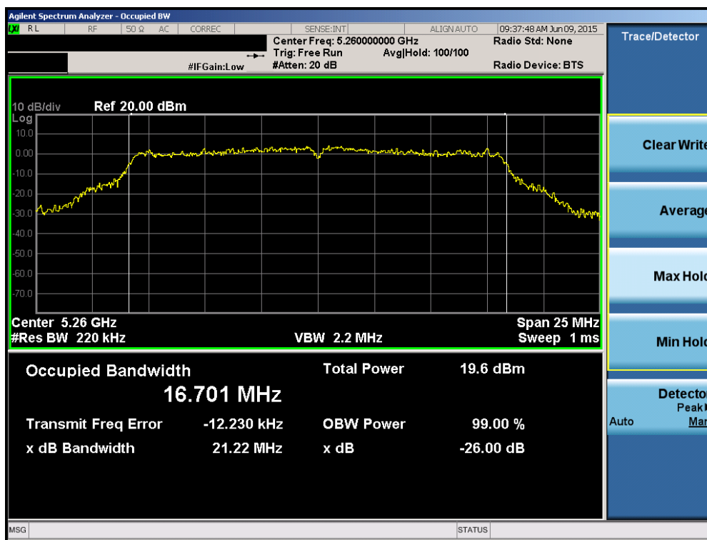
Plot 6-39. 26dB Bandwidth Plot (802.11a (UNII Band 2A) – Ch. 52)
