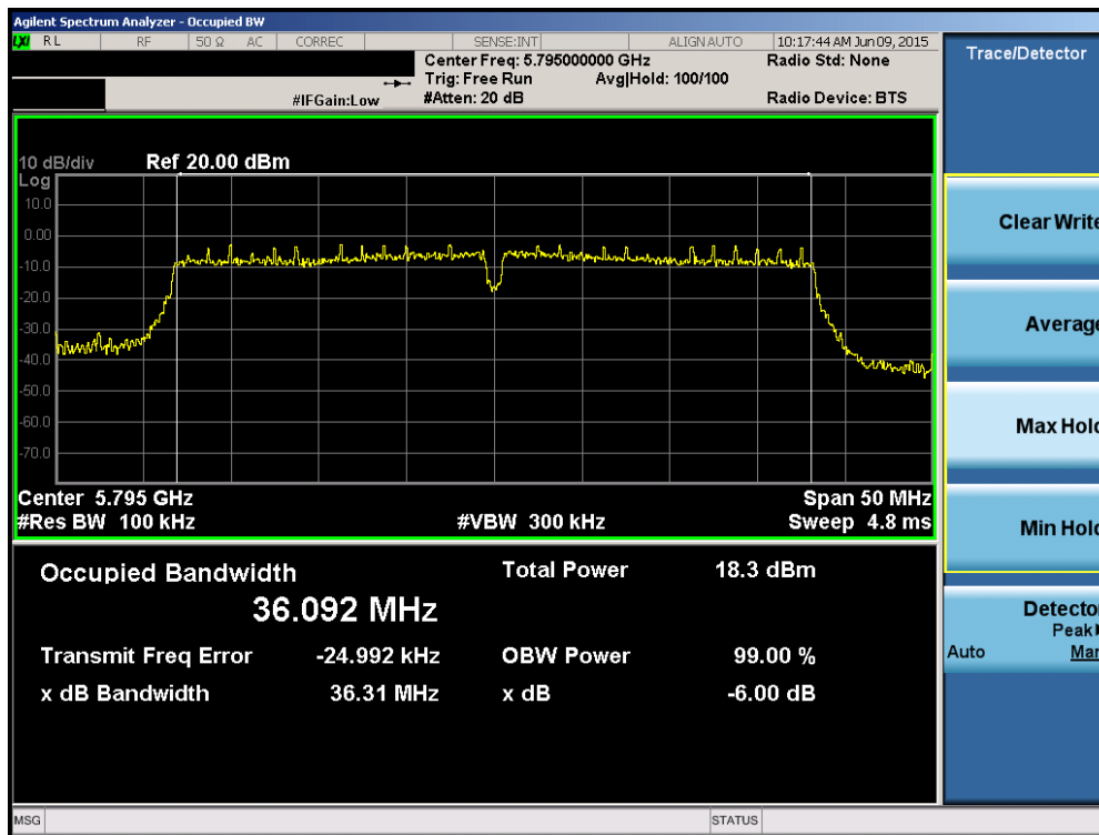
Plot 6-75. 6dB Bandwidth Plot (40MHz BW 802.11n (UNII Band 3) – Ch. 159)
