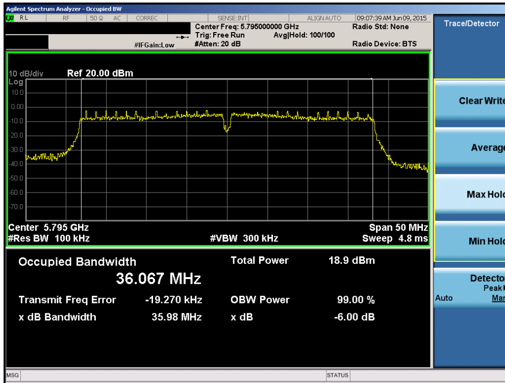
Plot 6-66. 6dB Bandwidth Plot (40MHz BW 802.11n (UNII Band 3) – Ch. 159)
