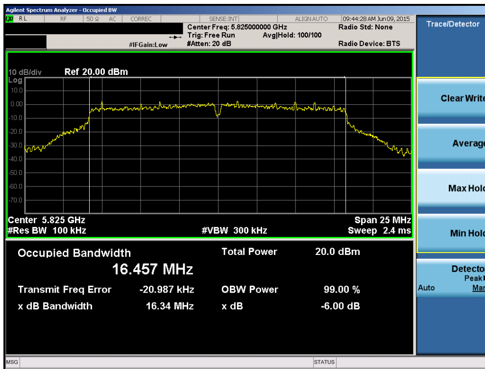
Plot 6-70. 6dB Bandwidth Plot (802.11a (UNII Band 3) – Ch. 165)
