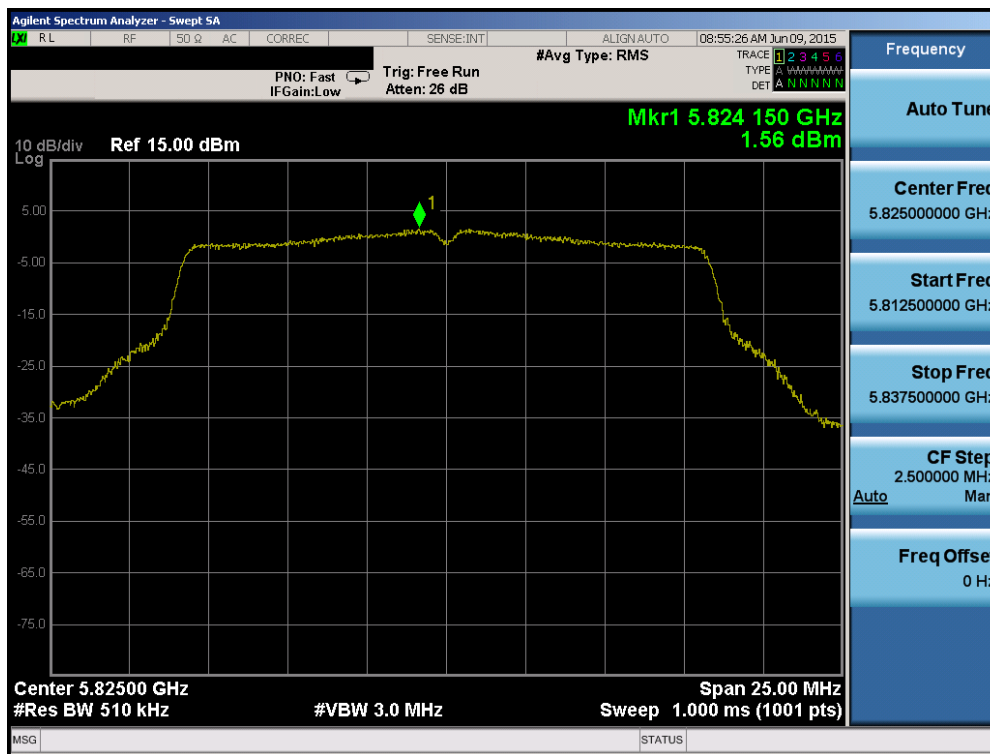
Plot 6-108. Power Spectral Density Plot (802.11a (UNII Band 3) – Ch. 165)
