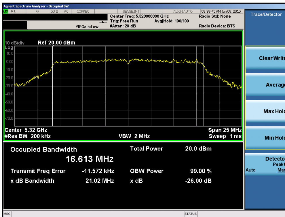
Plot 6-41. 26dB Bandwidth Plot (802.11a (UNII Band 2A) – Ch. 64)
