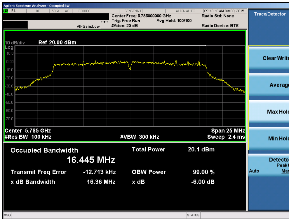
Plot 6-69. 6dB Bandwidth Plot (802.11a (UNII Band 3) – Ch. 157)
