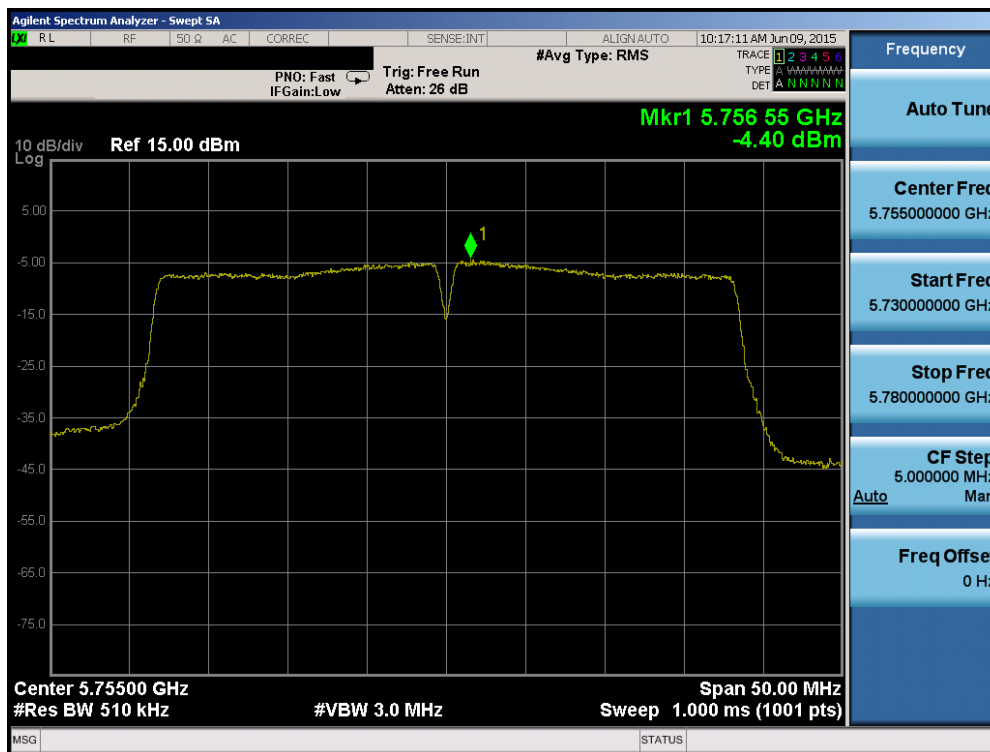
Plot 6-150. Power Spectral Density Plot (40MHz BW 802.11n (UNII Band 3) – Ch. 151)
