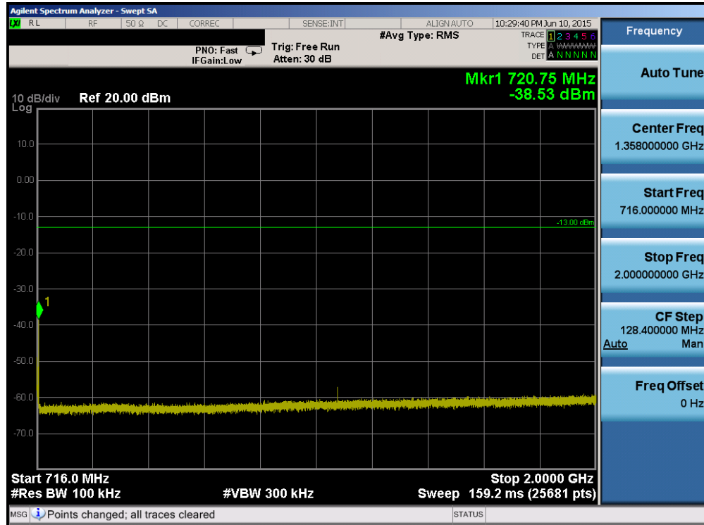
Plot 6-47. Conducted Spurious Plot (Band 12/17 – 5.0MHz QPSK – RB Size 1, RB Offset 0 – Mid Channel)
