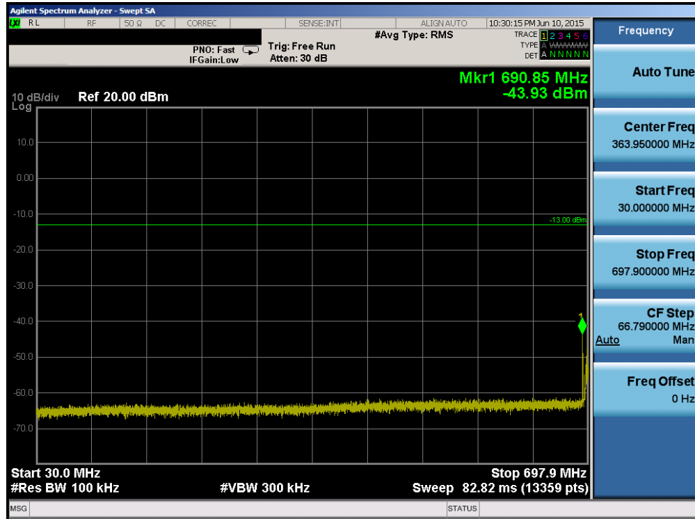
Plot 6-43. Conducted Spurious Plot (Band 12/17 – 5.0MHz QPSK – RB Size 1, RB Offset 0 – Low Channel)
