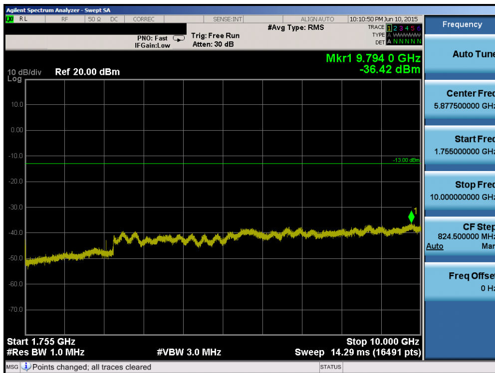
Plot 6-62. Conducted Spurious Plot (Band 4 – 20.0MHz QPSK – RB Size 1, RB Offset 0 – Low Channel)
