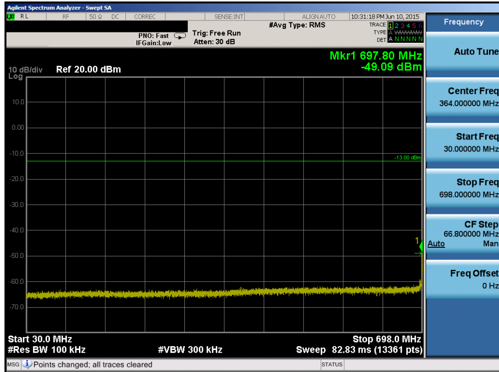
Plot 6-49. Conducted Spurious Plot (Band 12/17 – 5.0MHz QPSK – RB Size 1, RB Offset 0 – High Channel)
