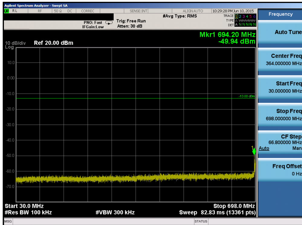
Plot 6-46. Conducted Spurious Plot (Band 12/17 – 5.0MHz QPSK – RB Size 1, RB Offset 0 – Mid Channel)
