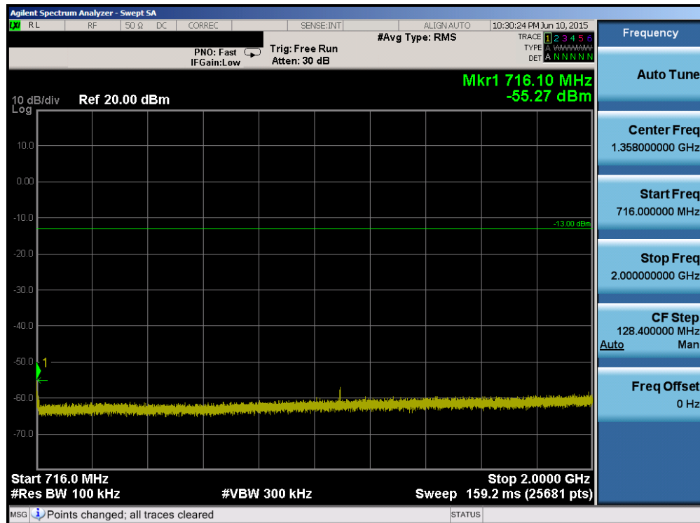
Plot 6-44. Conducted Spurious Plot (Band 12/17 – 5.0MHz QPSK – RB Size 1, RB Offset 0 – Low Channel)
