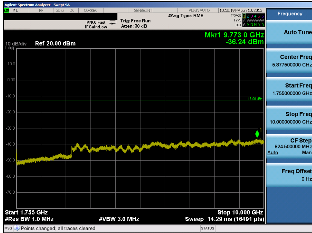
Plot 6-65. Conducted Spurious Plot (Band 4 – 20.0MHz QPSK – RB Size 1, RB Offset 0 – Mid Channel)
