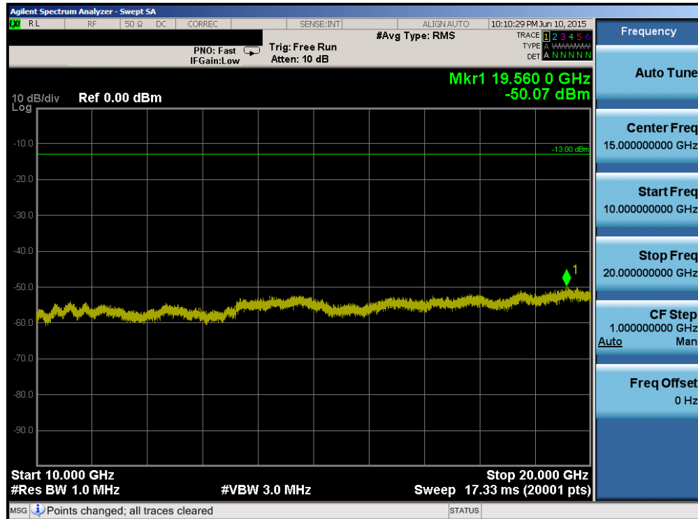
Plot 6-66. Conducted Spurious Plot (Band 4 – 20.0MHz QPSK – RB Size 1, RB Offset 0 – Mid Channel)
