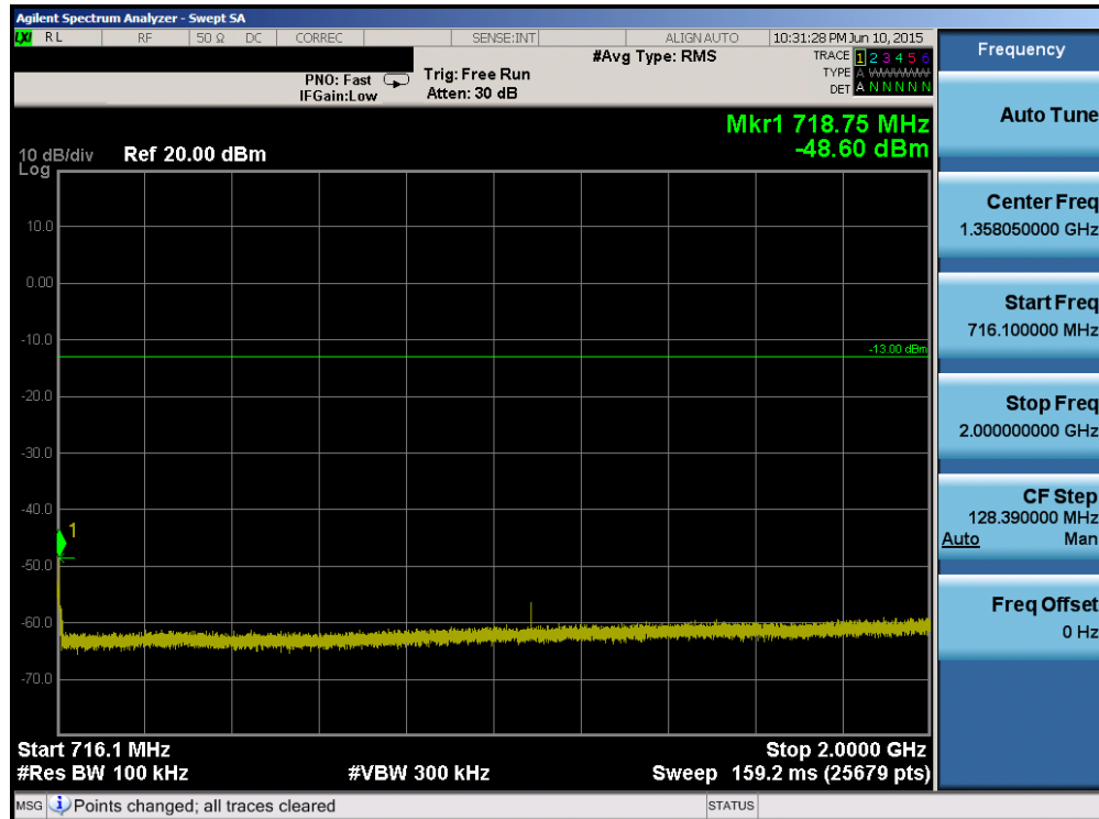
Plot 6-50. Conducted Spurious Plot (Band 12/17 – 5.0MHz QPSK – RB Size 1, RB Offset 0 – High Channel)
