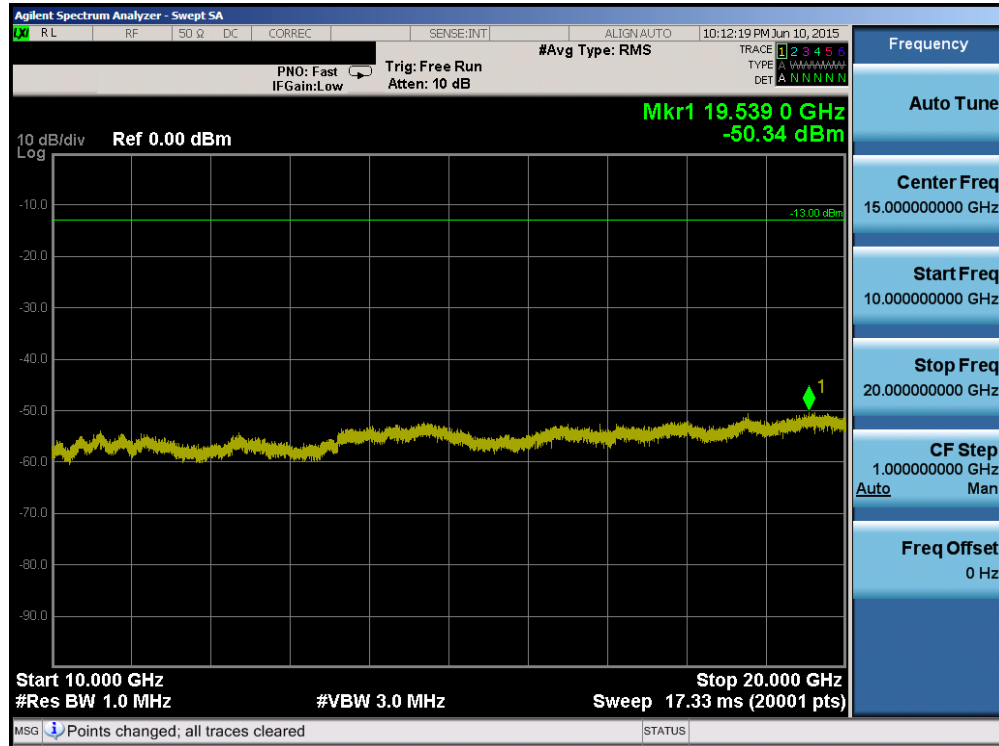
Plot 6-69. Conducted Spurious Plot (Band 4 – 20.0MHz QPSK – RB Size 1, RB Offset 0 – High Channel)
