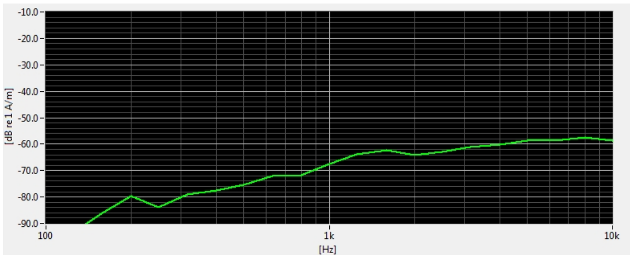
Figure 7-3 Worst-case ABM2 Plot for UMTS
