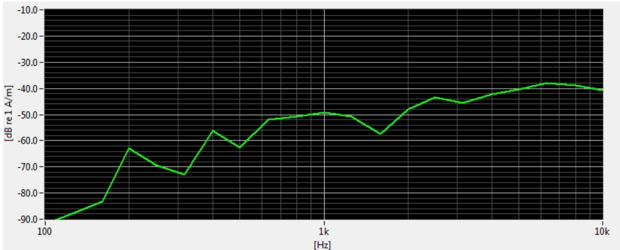
Figure 7-2 Worst-case ABM2 Plot for GSM
