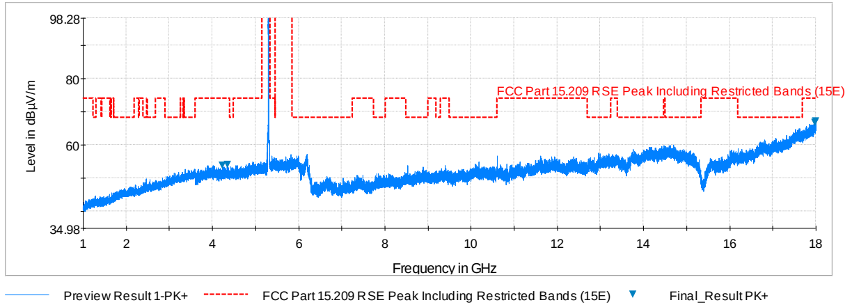
Plot 6-166. Radiated Spurious Plot above 1GHz (802.11a – U2A Ch. 56, Ant. Pol. V)
