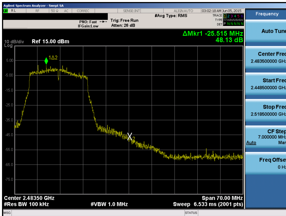
Plot 6-58. Band Edge Plot (802.11n (2.4GHz) – Ch. 11)
