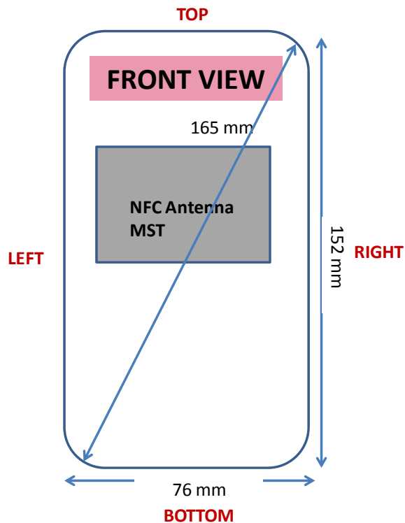
Figure F-2 NFC and MST Antenna Locations
